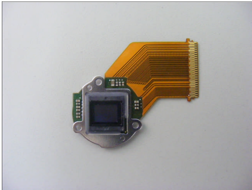
Top view of Cmos FPCB
