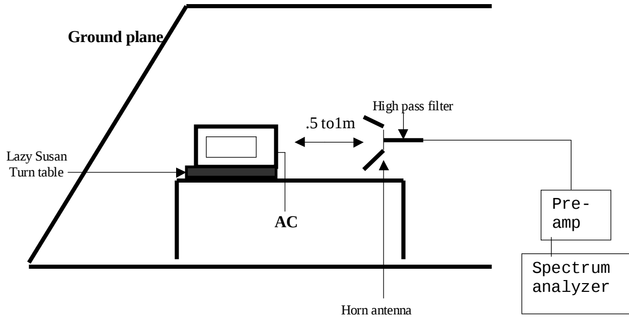
Figure 2. Radiated Emissions Configuration
