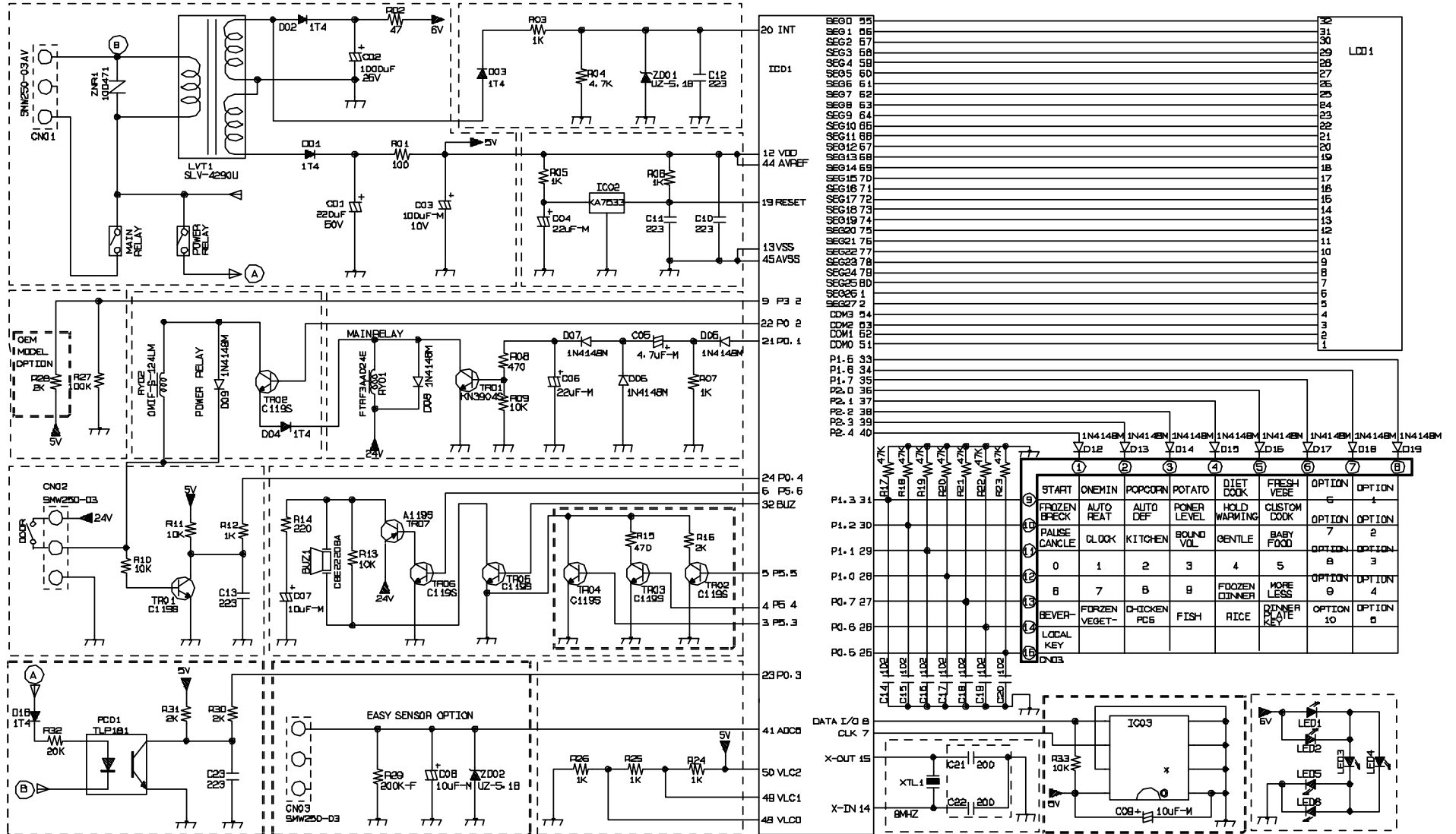
22LCD2 SCHEMATIC
