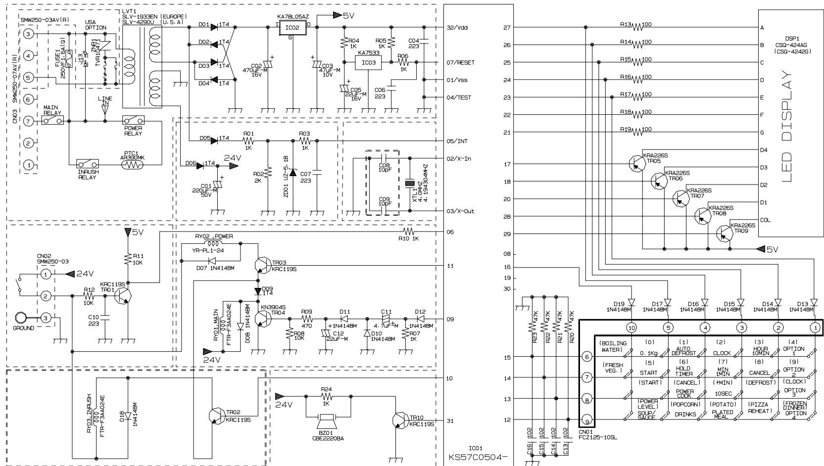
ELECTRIC DIAGRAM RC-22LED/(RA-22LED)
