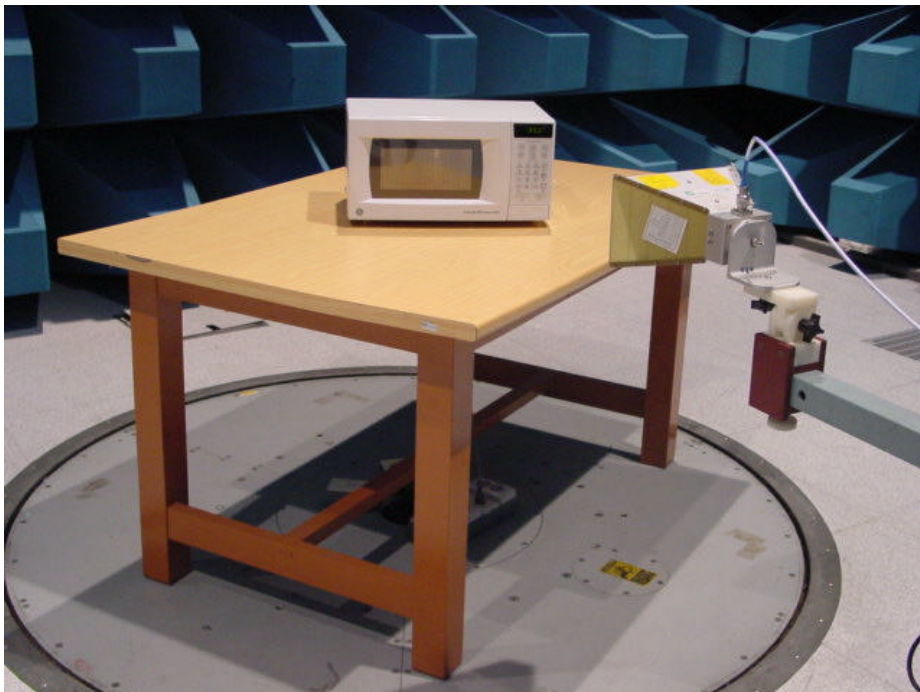
Fig. 9 Radiated Emission setup(1 - 25GHz)
