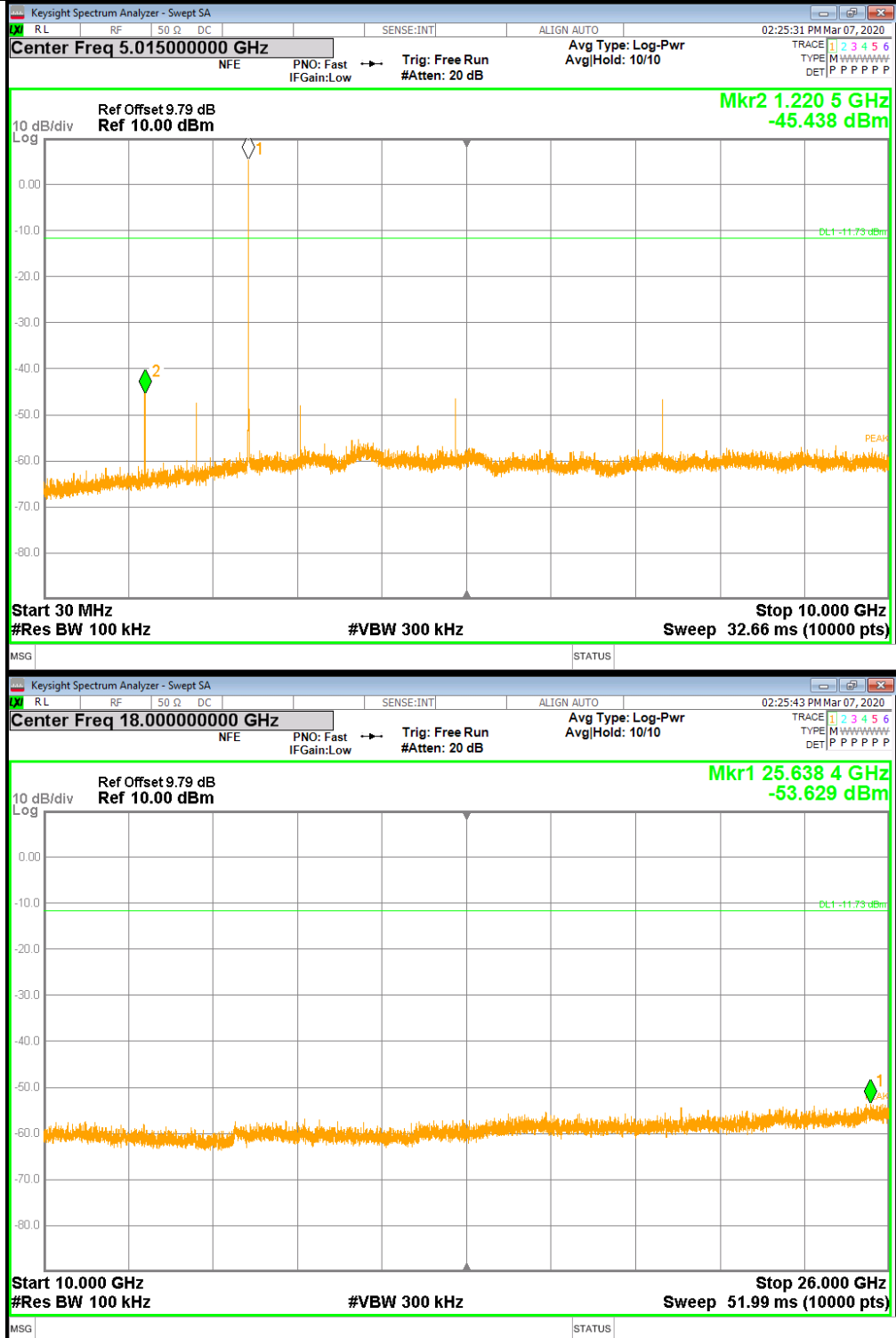
8DPSK_HCH_Graphs
