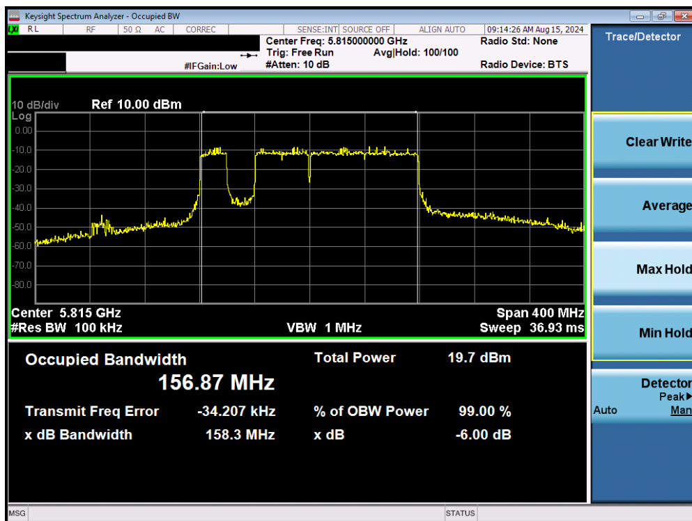
Plot 7-95. 6dB Bandwidth Plot MIMO ANT1 (160MHz BW 802.11be – Punctured (UNII Band 3/4) – Ch. 163)
