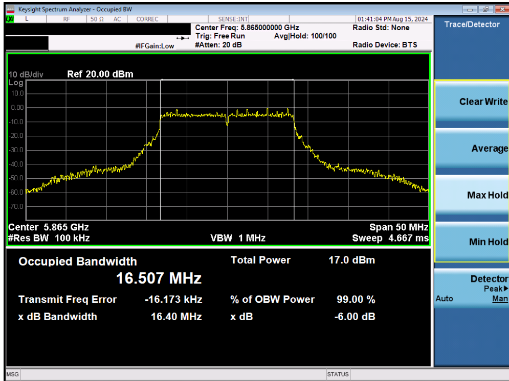
Plot 7-84. 6dB Bandwidth Plot MIMO ANT2 (802.11a (UNII Band 4) – Ch. 173)
