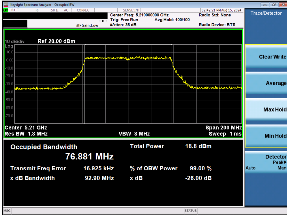
Plot 7-32. 26dB Bandwidth Plot MIMO ANT2 (80MHz BW 802.11be (UNII Band 1) – Ch. 42)
