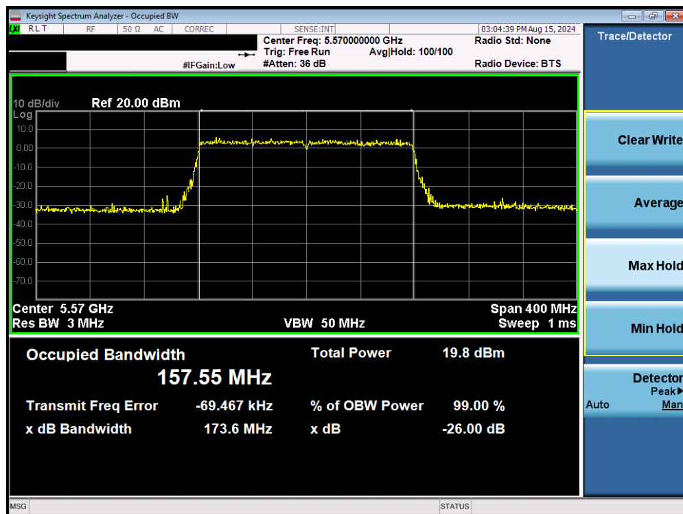
Plot 7-50. 26dB Bandwidth Plot MIMO ANT2 (160MHz BW 802.11be (UNII Band 2C) – Ch. 114)
