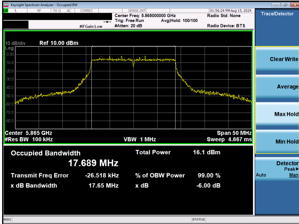
Plot 7-85. 6dB Bandwidth Plot MIMO ANT2 (20MHz BW 802.11n (UNII Band 3/4) – Ch. 173)
