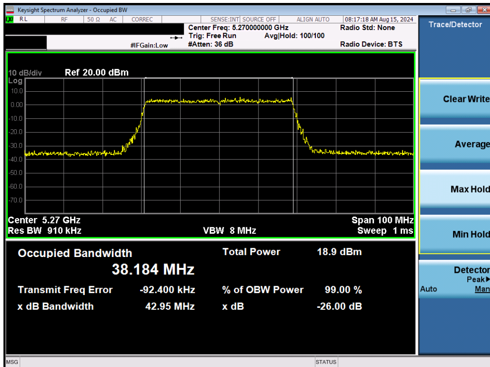
Plot 7-14. 26dB Bandwidth Plot MIMO ANT1 (40MHz BW 802.11be (UNII Band 2A) – Ch. 54)
