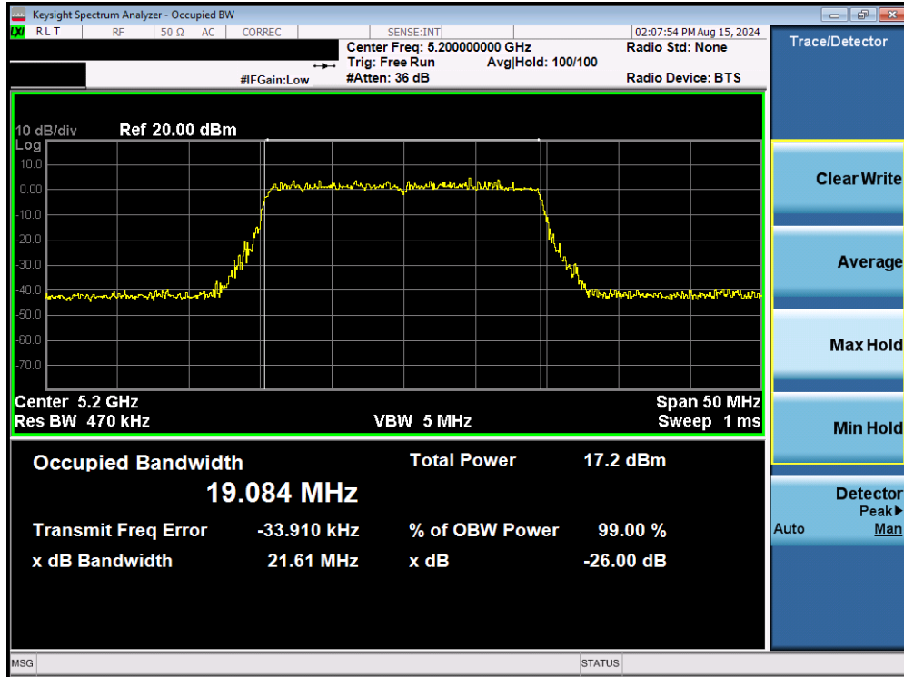
Plot 7-28. 26dB Bandwidth Plot MIMO ANT2 (20MHz BW 802.11be (UNII Band 1) – Ch. 40)
