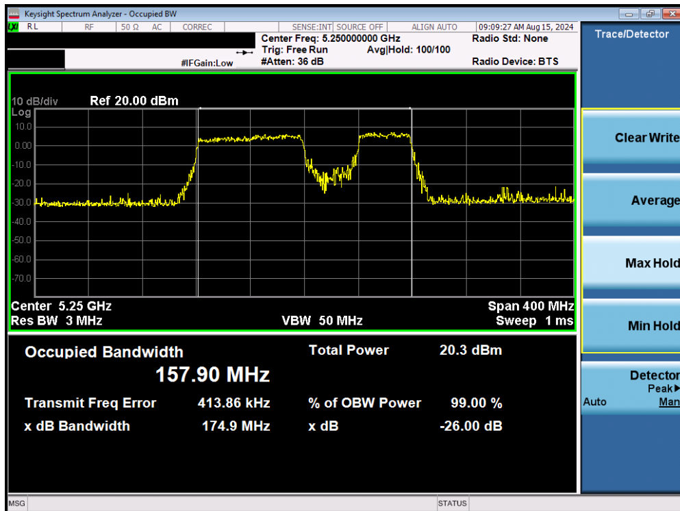
Plot 7-52. 26dB Bandwidth Plot MIMO ANT1 (160MHz BW 802.11be – Punctured (UNII Band 1/2A) – Ch. 50)
