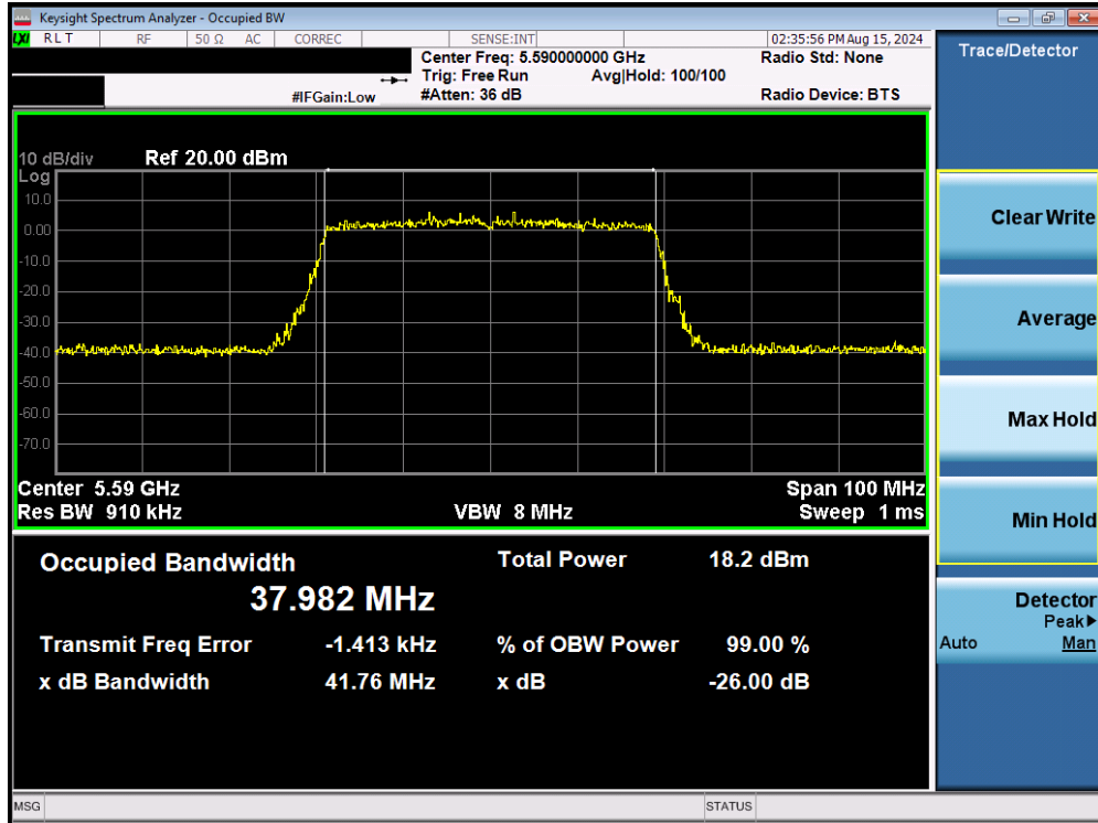
Plot 7-46. 26dB Bandwidth Plot MIMO ANT2 (40MHz BW 802.11be (UNII Band 2C) – Ch. 118)
