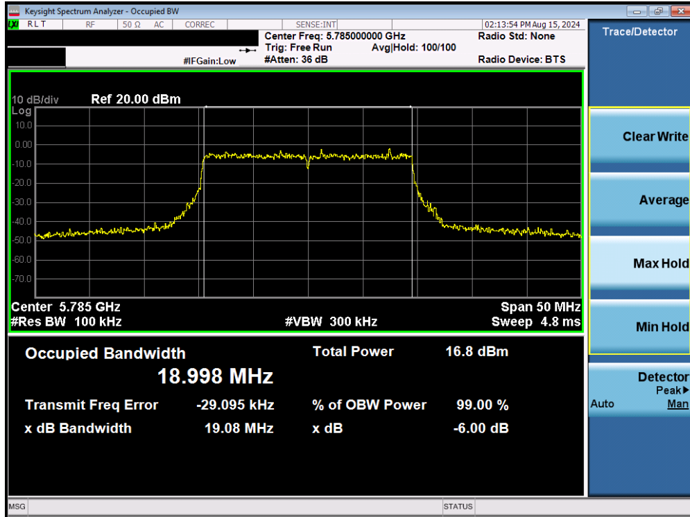
Plot 7-79. 6dB Bandwidth Plot MIMO ANT2 (20MHz BW 802.11be (UNII Band 3) – Ch. 157)
