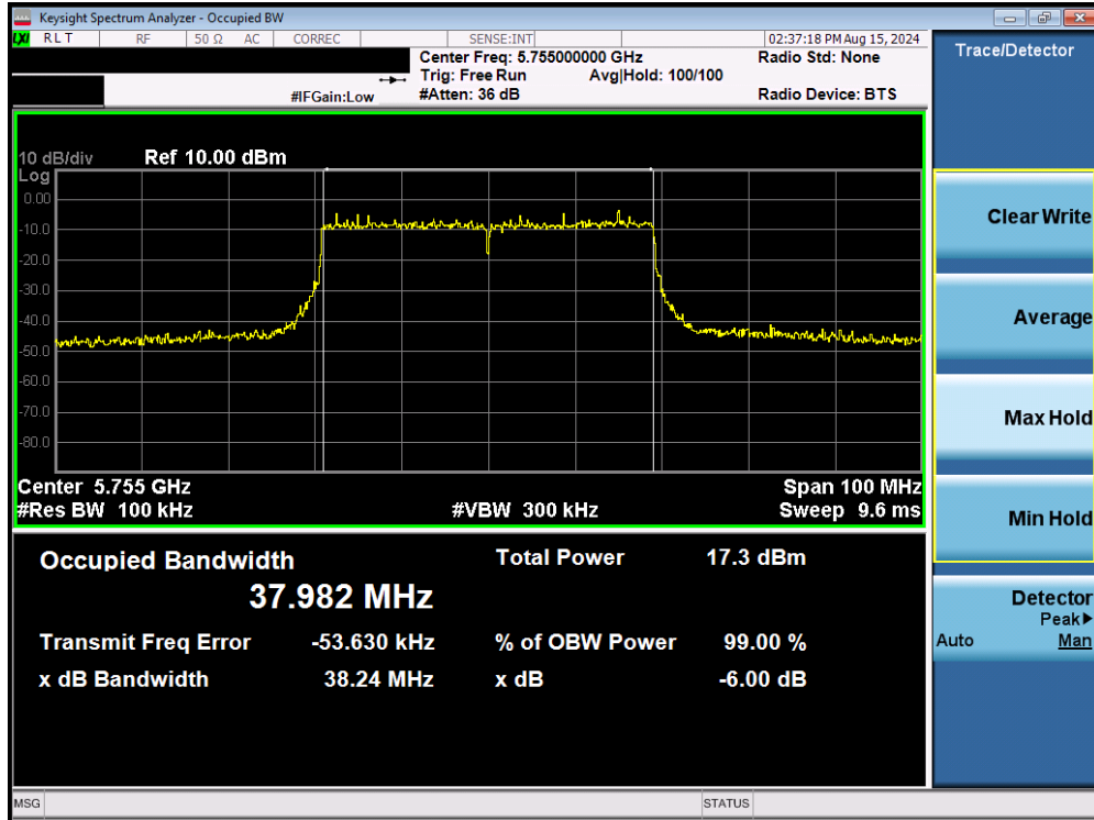
Plot 7-81. 6dB Bandwidth Plot MIMO ANT2 (40MHz BW 802.11be (UNII Band 3) – Ch. 151)
