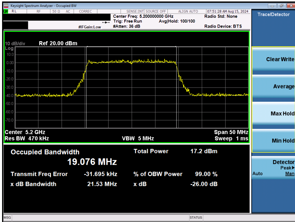
Plot 7-3. 26dB Bandwidth Plot MIMO ANT1 (20MHz BW 802.11be(UNII Band 1) – Ch. 40)
