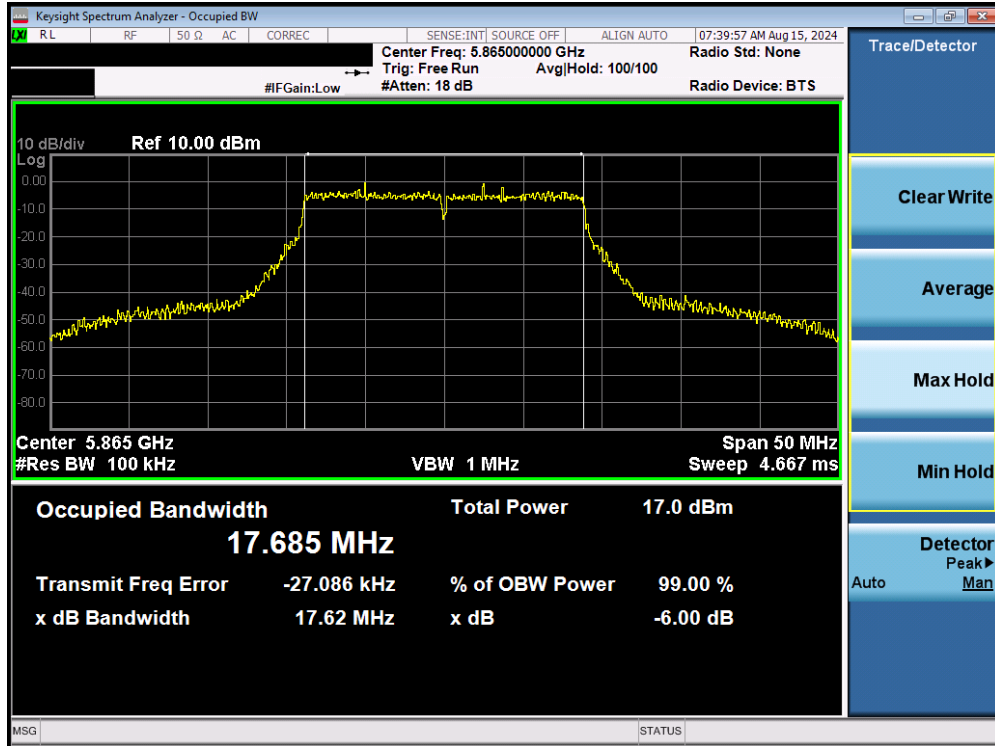
Plot 7-69. 6dB Bandwidth Plot MIMO ANT1 (20MHz BW 802.11n (UNII Band 4) – Ch. 173)
