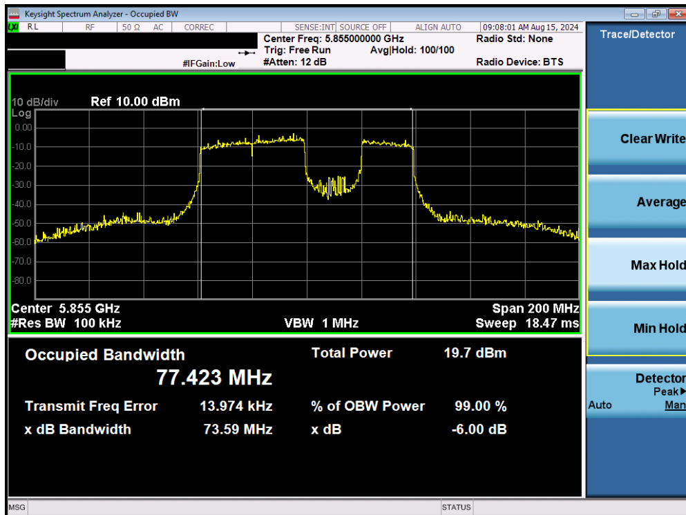
Plot 7-94. 6dB Bandwidth Plot MIMO ANT1 (80MHz BW 802.11be – Punctured (UNII Band 3/4) – Ch. 171)
