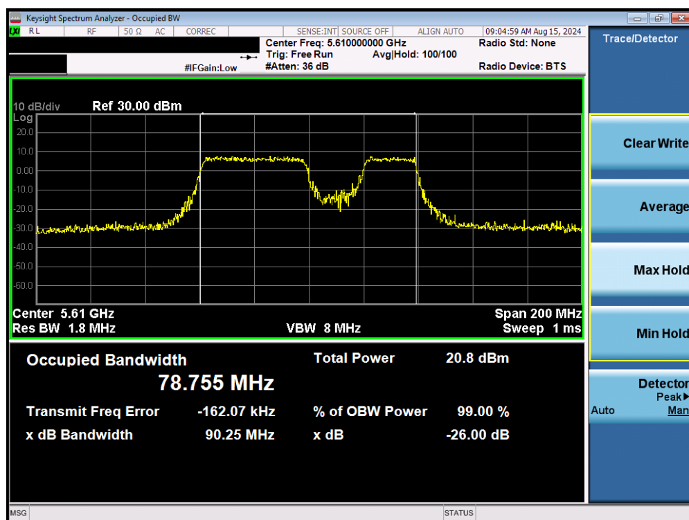
Plot 7-54. 26dB Bandwidth Plot MIMO ANT1 (80MHz BW 802.11be – Punctured (UNII Band 2C) – Ch. 122)
