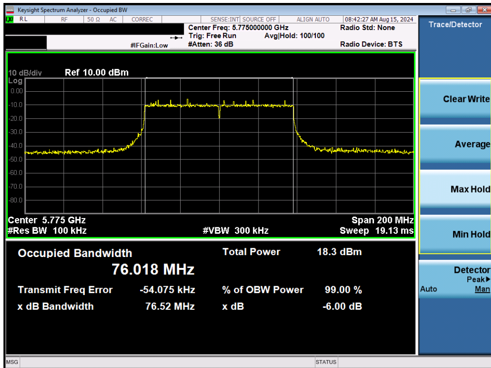
Plot 7-66. 6dB Bandwidth Plot MIMO ANT1 (80MHz BW 802.11ac (UNII Band 3) – Ch. 155)
