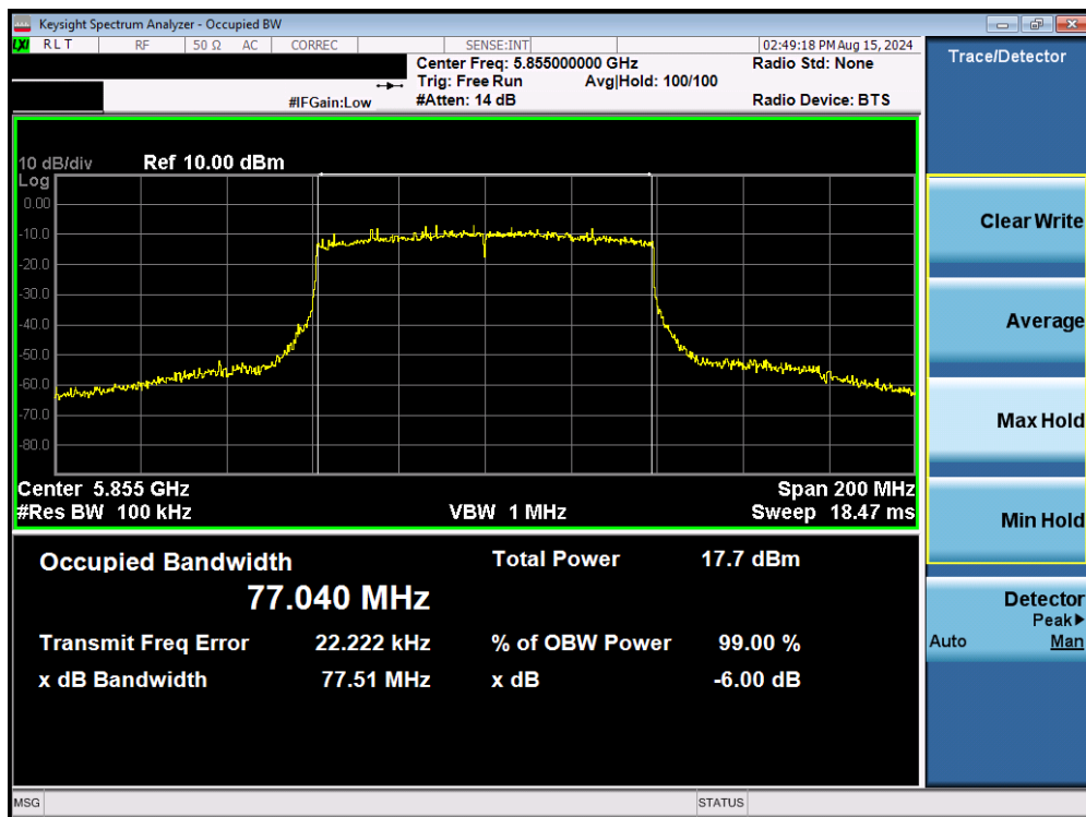
Plot 7-90. 6dB Bandwidth Plot MIMO ANT2 (80MHz BW 802.11be (UNII Band 3/4) – Ch. 171)
