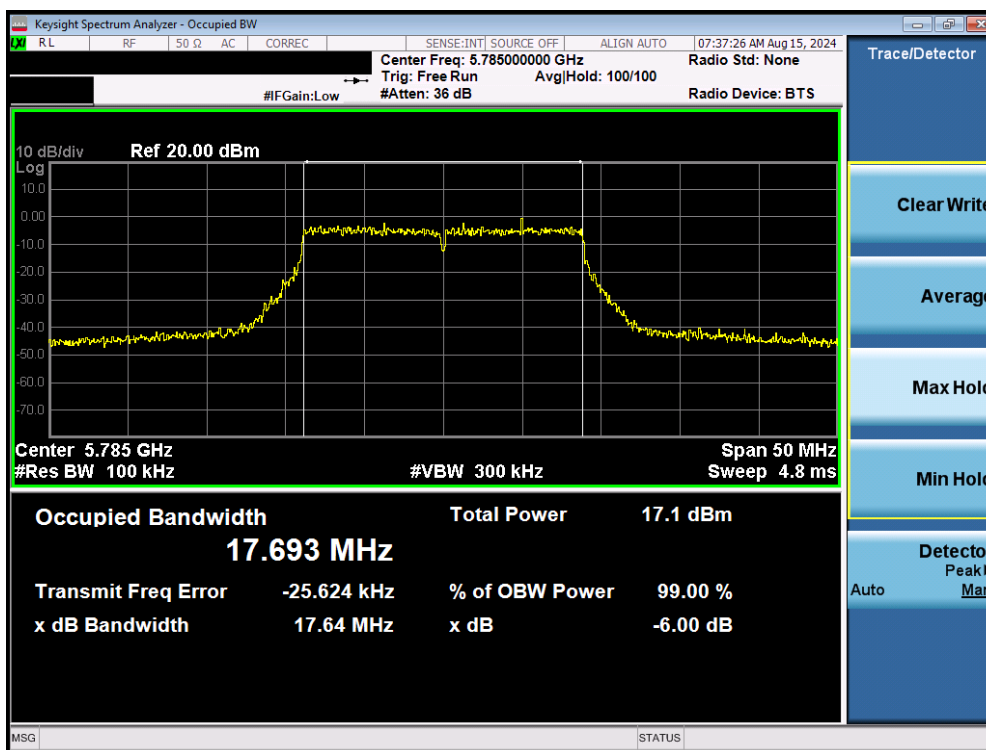
Plot 7-62. 6dB Bandwidth Plot MIMO ANT1 (20MHz BW 802.11n (UNII Band 3) – Ch. 157)
