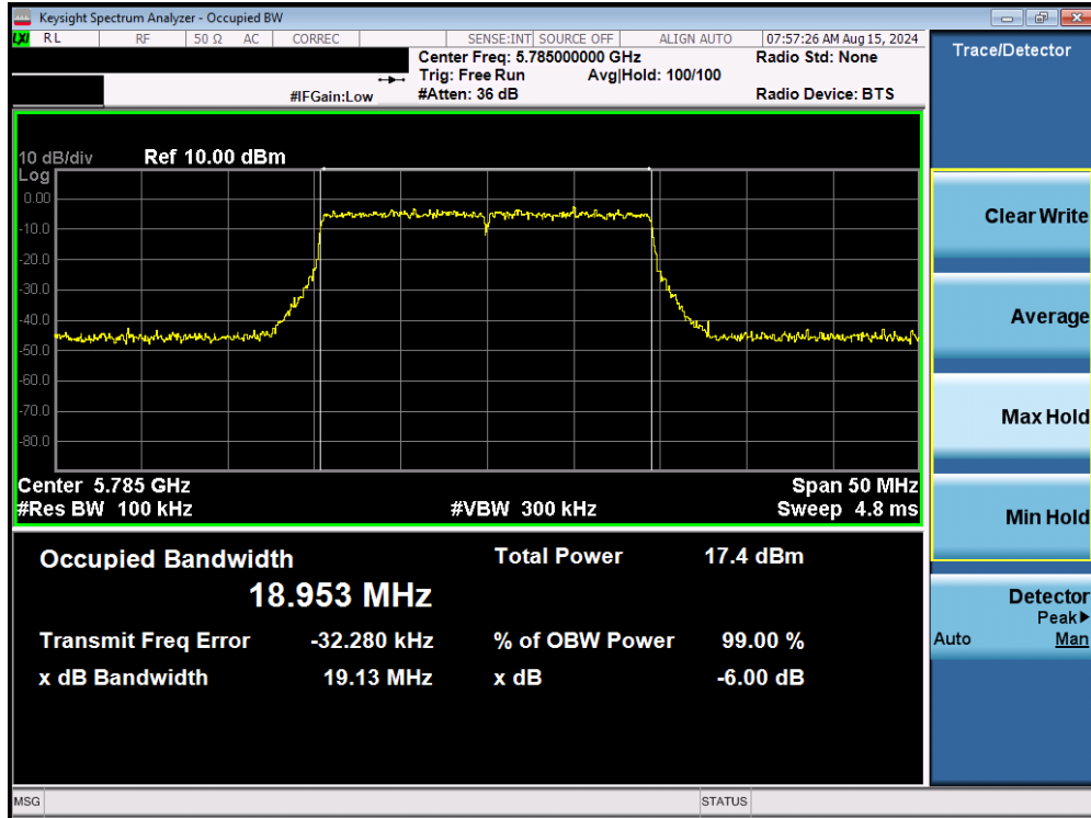
Plot 7-63. 6dB Bandwidth Plot MIMO ANT1 (20MHz BW 802.11be (UNII Band 3) – Ch. 157)
