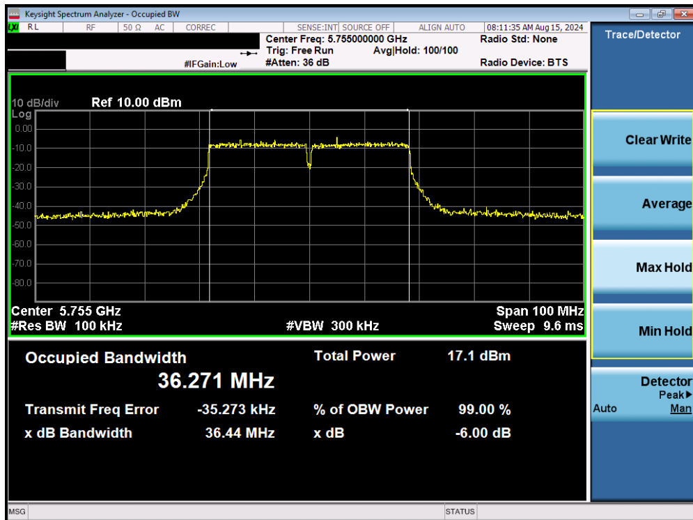
Plot 7-64. 6dB Bandwidth Plot MIMO ANT1 (40MHz BW 802.11n (UNII Band 3) – Ch. 151)
