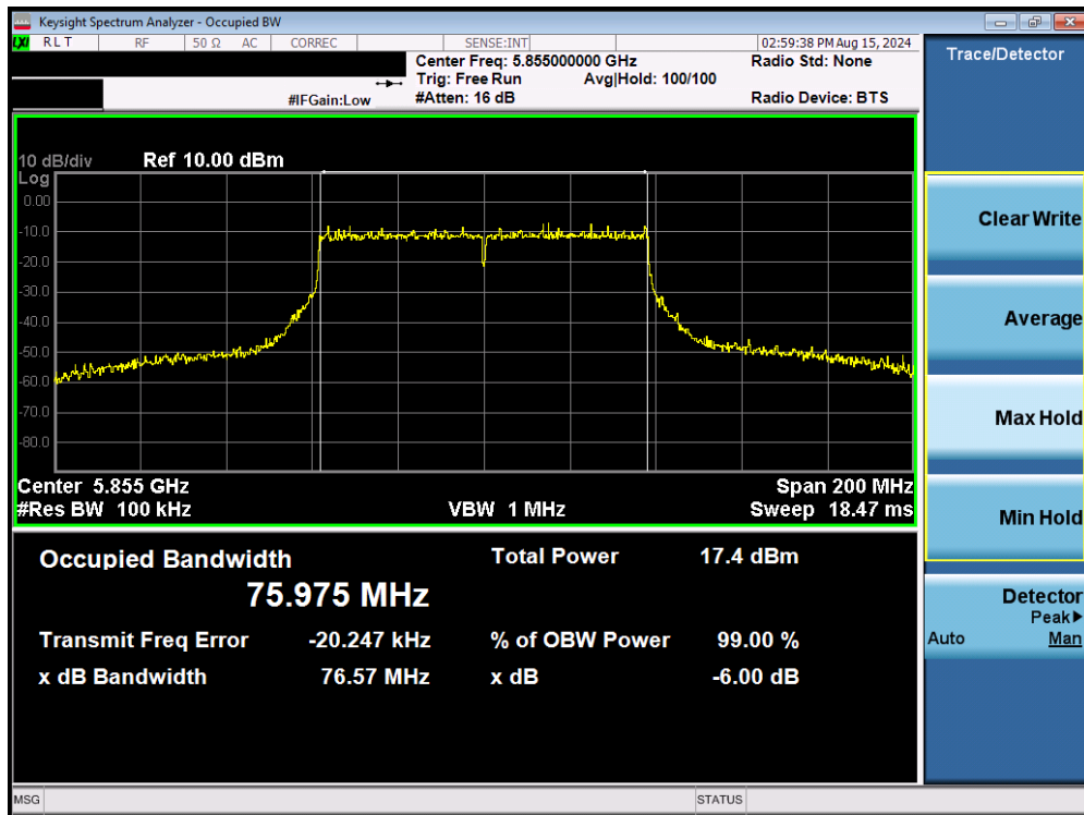
Plot 7-89. 6dB Bandwidth Plot MIMO ANT2 (80MHz BW 802.11ac (UNII Band 3/4) – Ch. 171)
