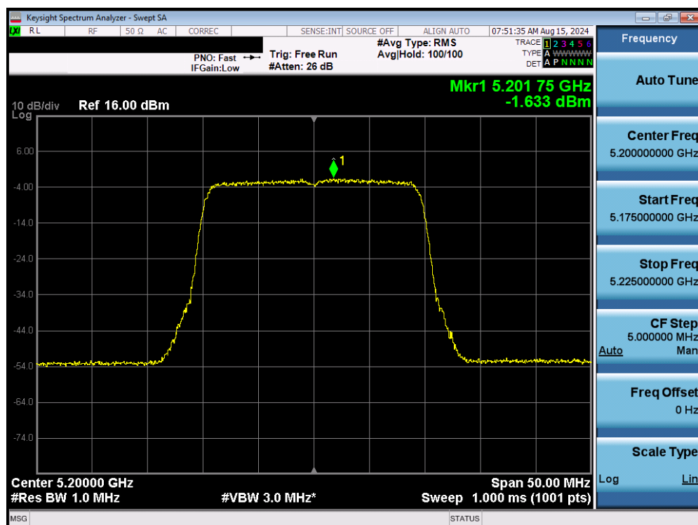
Plot 7-101. Power Spectral Density Plot MIMO ANT1 (20MHz BW 802.11be (UNII Band 1) – Ch. 40)
