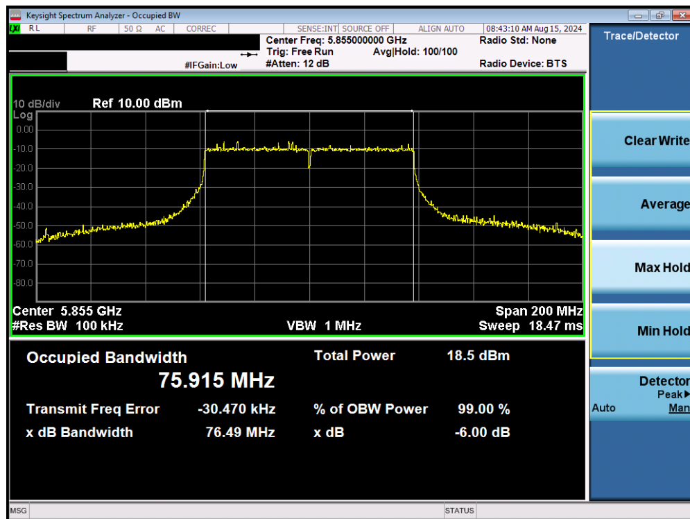
Plot 7-73. 6dB Bandwidth Plot MIMO ANT1 (80MHz BW 802.11ac (UNII Band 3/4) – Ch. 171)
