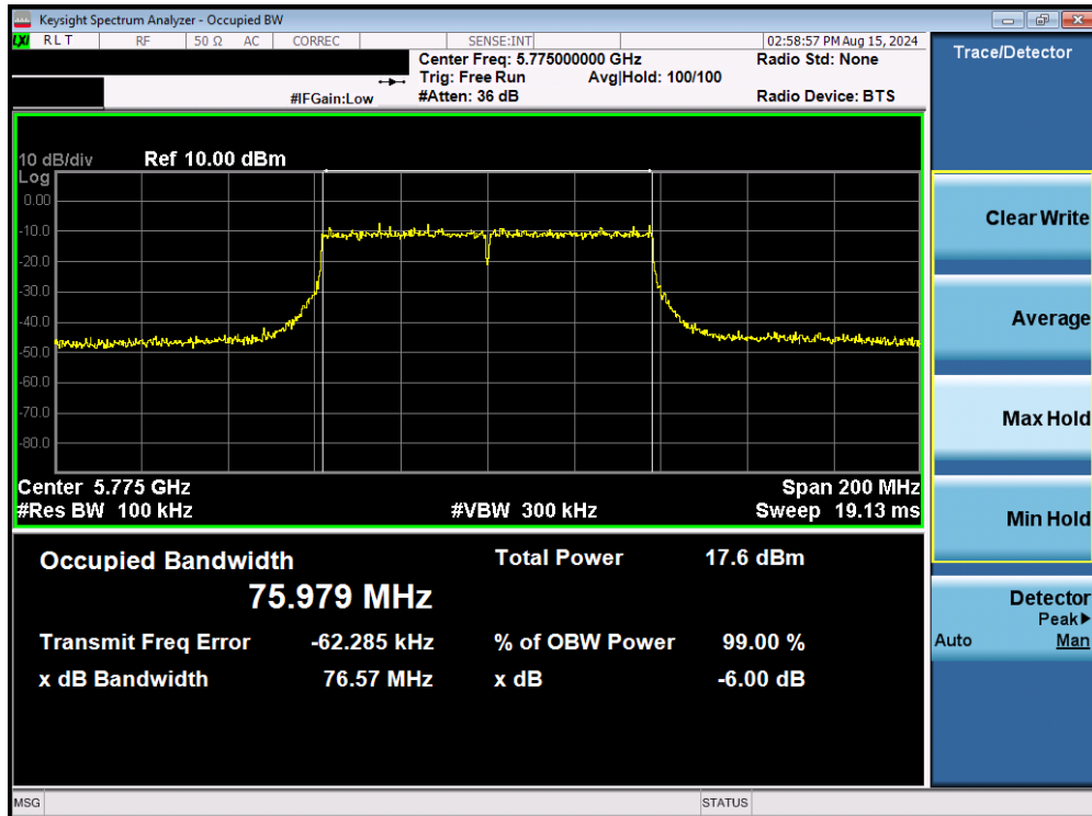
Plot 7-82. 6dB Bandwidth Plot MIMO ANT2 (80MHz BW 802.11ac (UNII Band 3) – Ch. 155)
