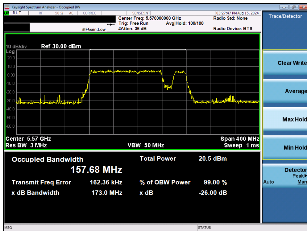
Plot 7-60. 26dB Bandwidth Plot MIMO ANT2 (160MHz BW 802.11be – Punctured (UNII Band 2C) – Ch. 114)
