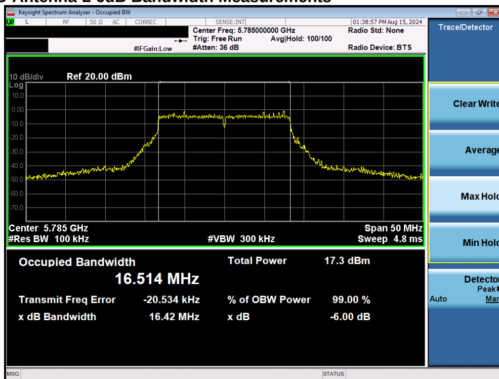
Plot 7-77. 6dB Bandwidth Plot MIMO ANT2 (802.11a (UNII Band 3) – Ch. 157)
