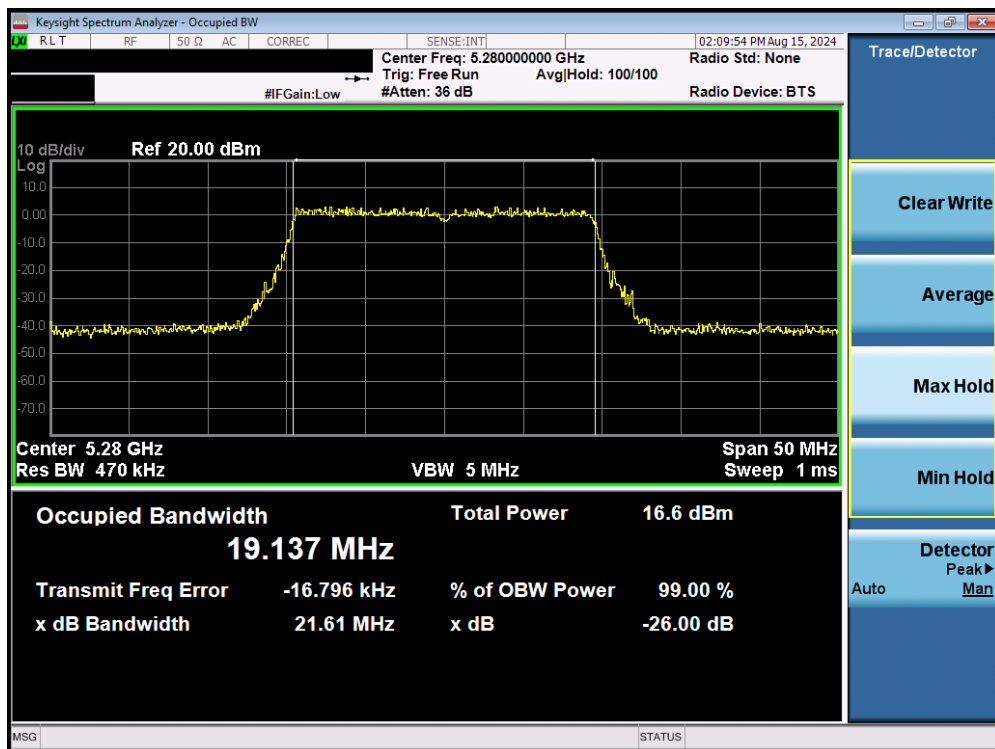
Plot 7-37. 26dB Bandwidth Plot MIMO ANT2 (20MHz BW 802.11be (UNII Band 2A) – Ch. 56)
