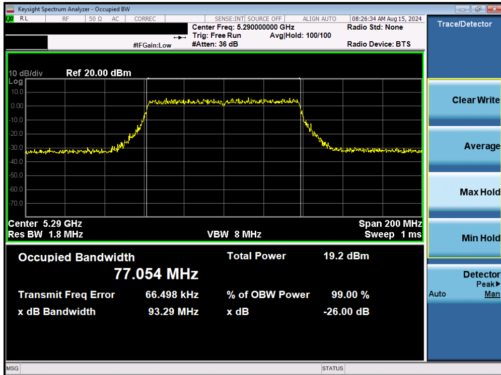
Plot 7-16. 26dB Bandwidth Plot MIMO ANT1 (80MHz BW 802.11be (UNII Band 2A) – Ch. 58)
