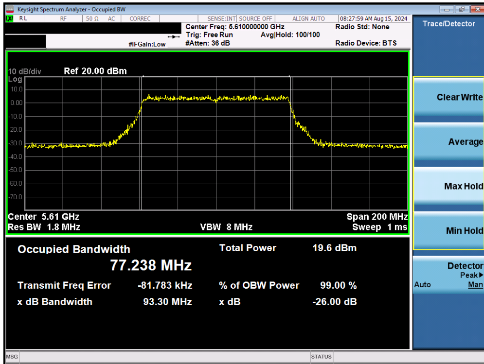
Plot 7-23. 26dB Bandwidth Plot MIMO ANT1 (80MHz BW 802.11be (UNII Band 2C) – Ch. 122)
