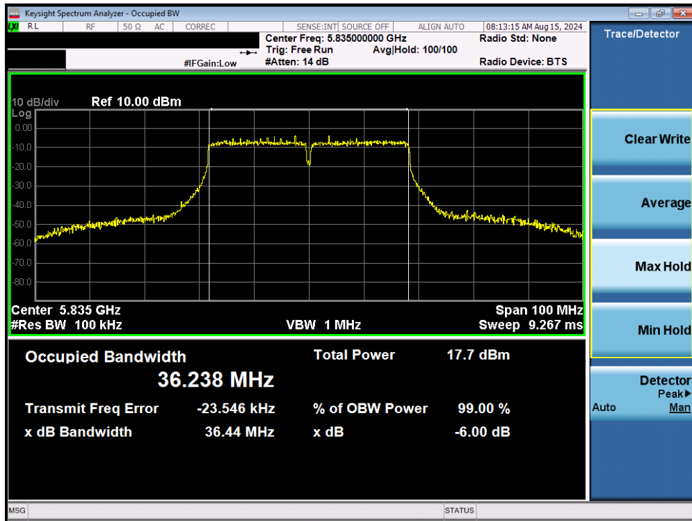
Plot 7-71. 6dB Bandwidth Plot MIMO ANT1 (40MHz BW 802.11n (UNII Band 3/4) – Ch. 167)
