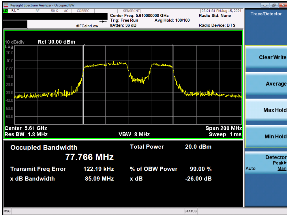
Plot 7-59. 26dB Bandwidth Plot MIMO ANT2 (80MHz BW 802.11be – Punctured (UNII Band 2C) – Ch. 122)
