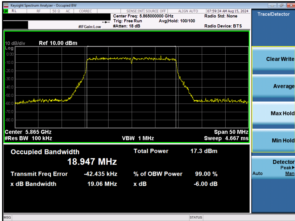
Plot 7-70. 6dB Bandwidth Plot MIMO ANT1 (20MHz BW 802.11be (UNII Band 4) – Ch. 173)
