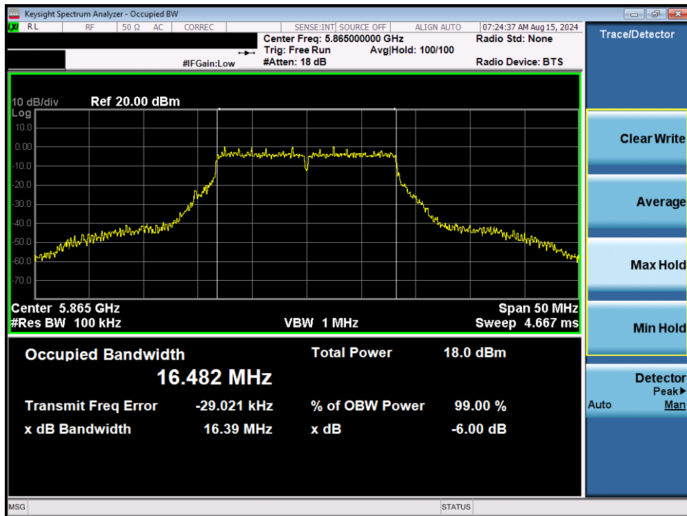
Plot 7-68. 6dB Bandwidth Plot MIMO ANT1 (802.11a (UNII Band 4) – Ch. 173)
