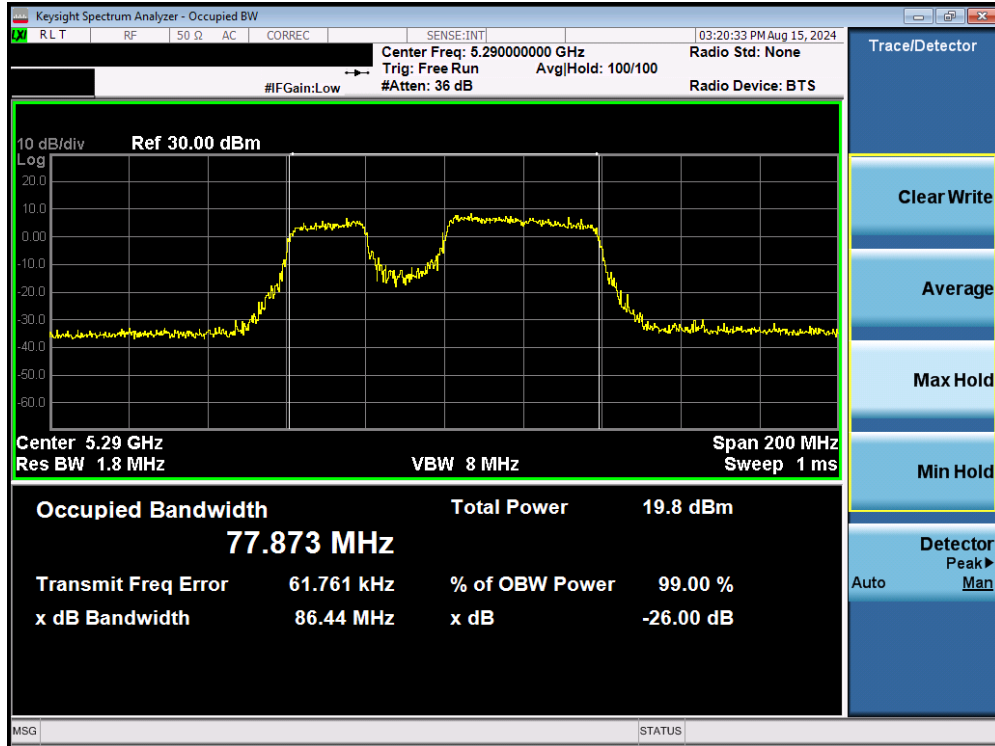
Plot 7-58. 26dB Bandwidth Plot MIMO ANT2 (80MHz BW 802.11be – Punctured (UNII Band 2A) – Ch. 58)
