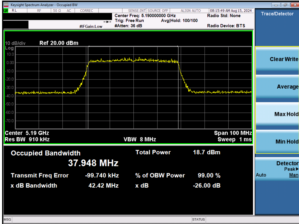
Plot 7-5. 26dB Bandwidth Plot MIMO ANT1 (40MHz BW 802.11be (UNII Band 1) – Ch. 38)
