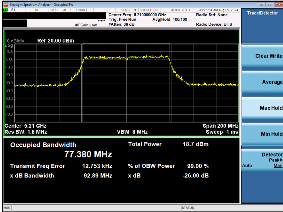
Plot 7-7. 26dB Bandwidth Plot MIMO ANT1 (80MHz BW 802.11be (UNII Band 1) – Ch. 42)
