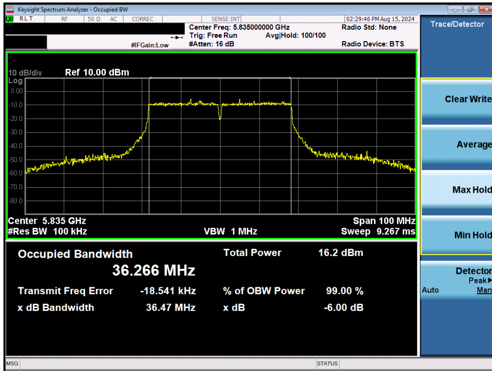
Plot 7-87. 6dB Bandwidth Plot MIMO ANT2 (40MHz BW 802.11n (UNII Band 3/4) – Ch. 167)
