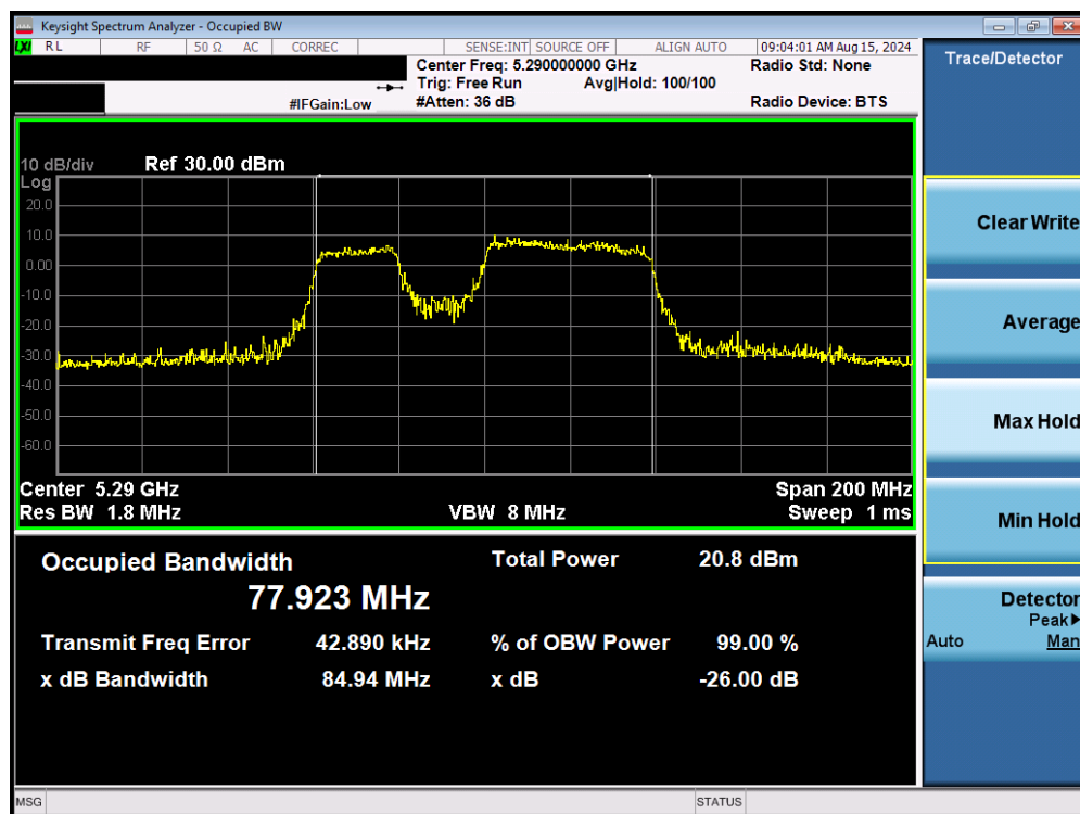
Plot 7-53. 26dB Bandwidth Plot MIMO ANT1 (80MHz BW 802.11be – Punctured (UNII Band 2A) – Ch. 58)
