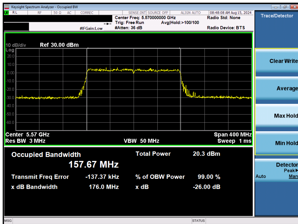
Plot 7-25. 26dB Bandwidth Plot MIMO ANT1 (160MHz BW 802.11be (UNII Band 2C) – Ch. 114)
