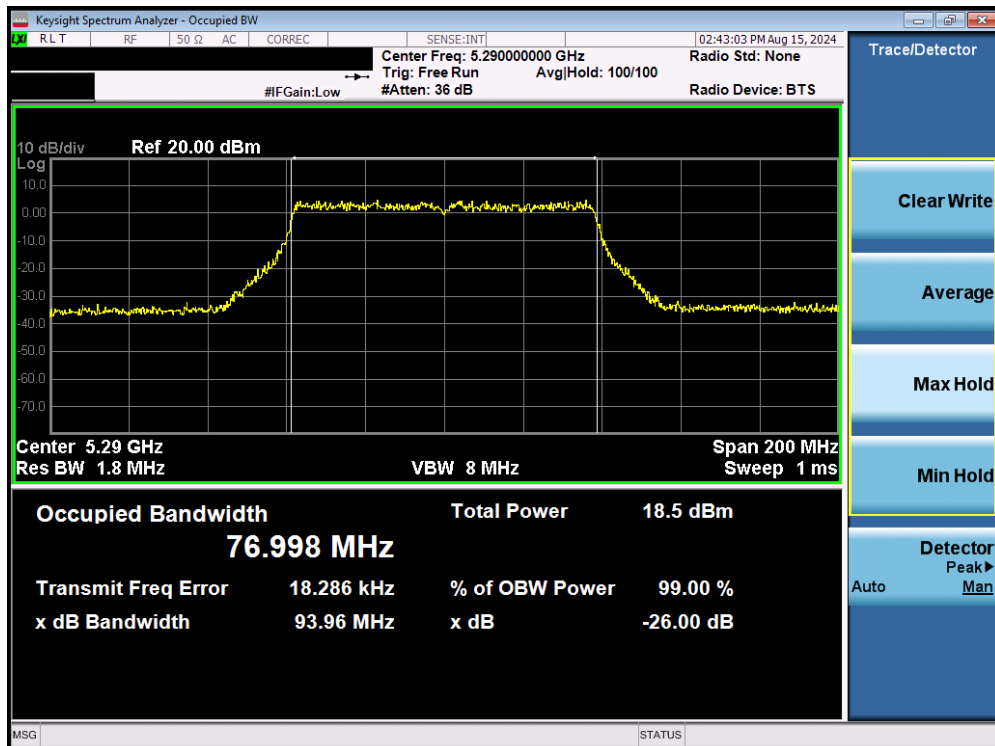
Plot 7-41. 26dB Bandwidth Plot MIMO ANT2 (80MHz BW 802.11be (UNII Band 2A) – Ch. 58)
