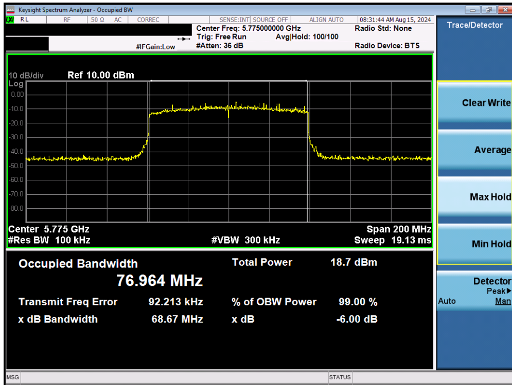
Plot 7-67. 6dB Bandwidth Plot MIMO ANT1 (80MHz BW 802.11be (UNII Band 3) – Ch. 155)
