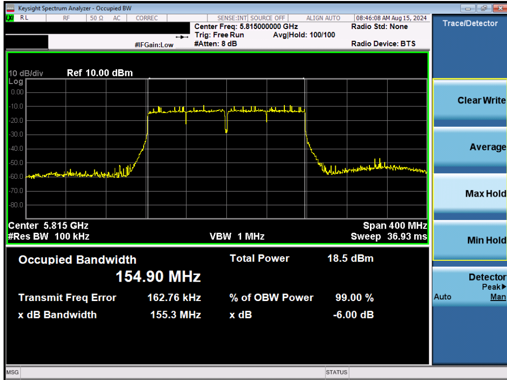
Plot 7-75. 6dB Bandwidth Plot MIMO ANT1 (160MHz BW 802.11ac (UNII Band 3/4) – Ch. 163)
