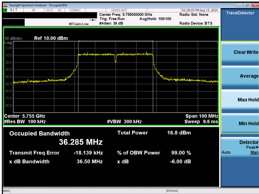
Plot 7-80. 6dB Bandwidth Plot MIMO ANT2 (40MHz BW 802.11n (UNII Band 3) – Ch. 151)
