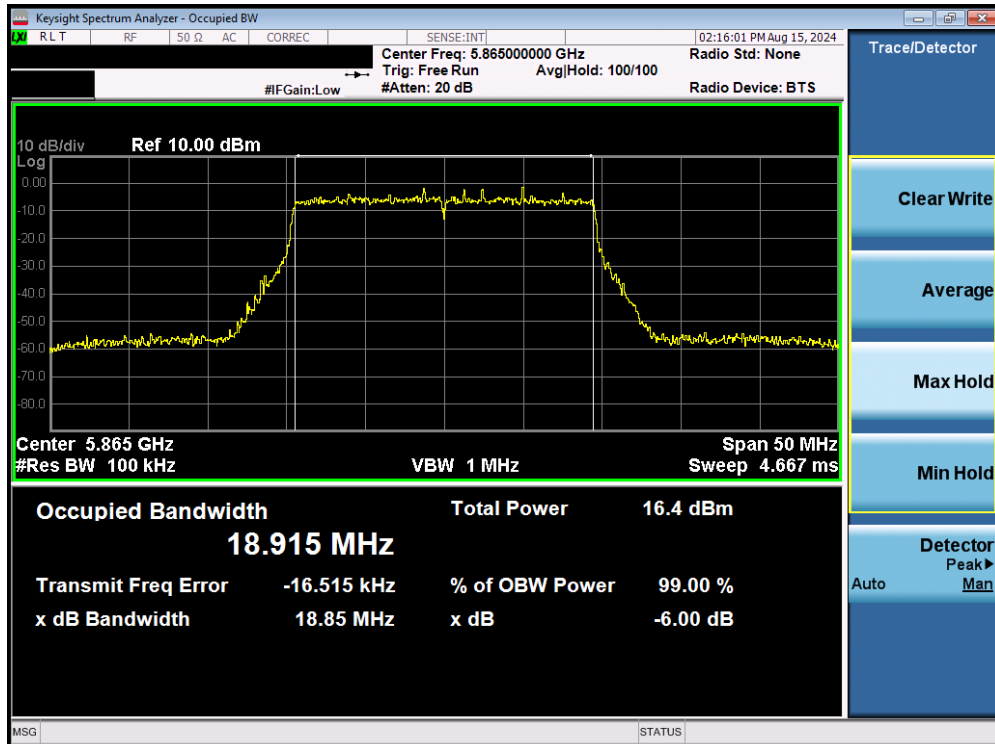
Plot 7-86. 6dB Bandwidth Plot MIMO ANT2 (20MHz BW 802.11be (UNII Band 3/4) – Ch. 173)
