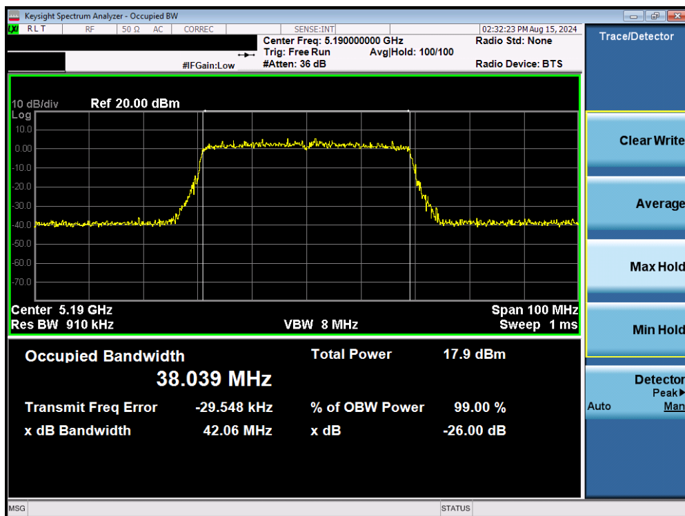
Plot 7-30. 26dB Bandwidth Plot MIMO ANT2 (40MHz BW 802.11be (UNII Band 1) – Ch. 38)
