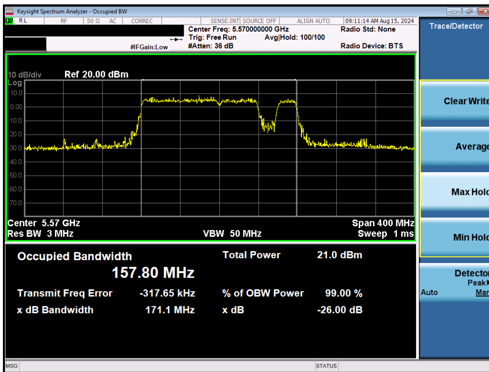
Plot 7-55 26dB Bandwidth Plot MIMO ANT1 (160MHz BW 802.11be – Punctured (UNII Band 2C) – Ch. 114)
