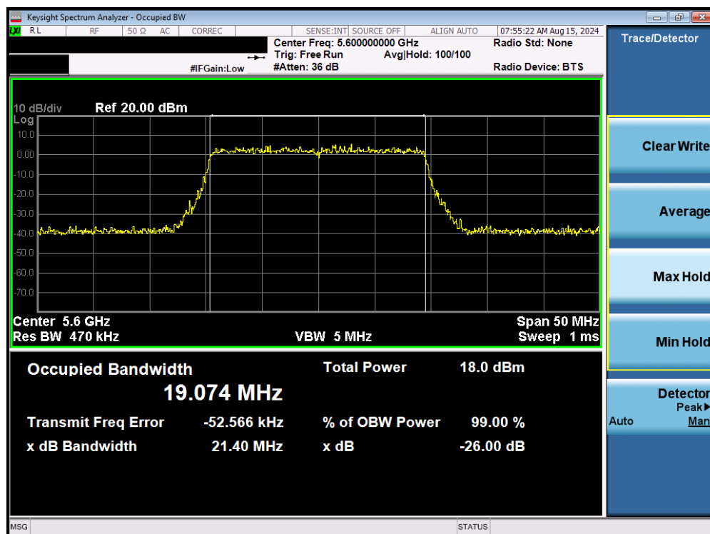
Plot 7-19. 26dB Bandwidth Plot MIMO ANT1 (20MHz BW 802.11be (UNII Band 2C) – Ch. 120)
