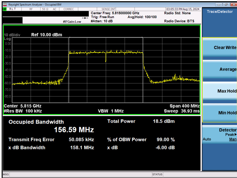
Plot 7-91. 6dB Bandwidth Plot MIMO ANT2 (160MHz BW 802.11ac (UNII Band 3/4) – Ch. 163)
