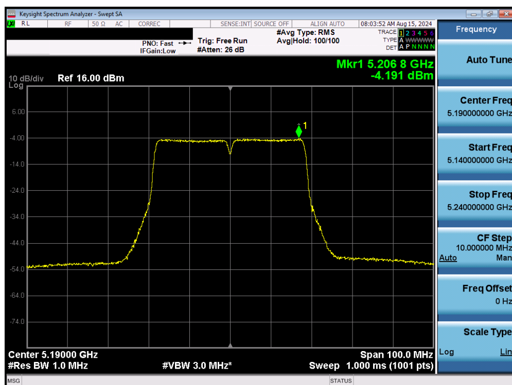
Plot 7-102. Power Spectral Density Plot MIMO ANT1 (40MHz BW 802.11n (UNII Band 1) – Ch. 38)
