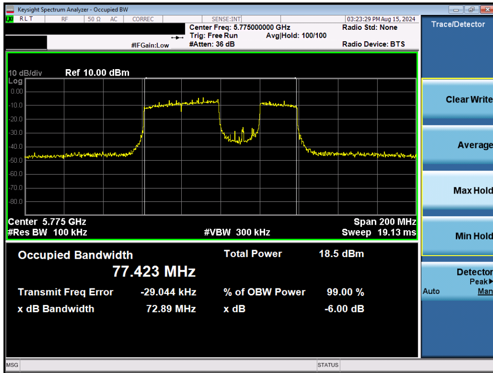
Plot 7-96. 6dB Bandwidth Plot MIMO ANT2 (80MHz BW 802.11be – Punctured (UNII Band 3) – Ch. 155)
