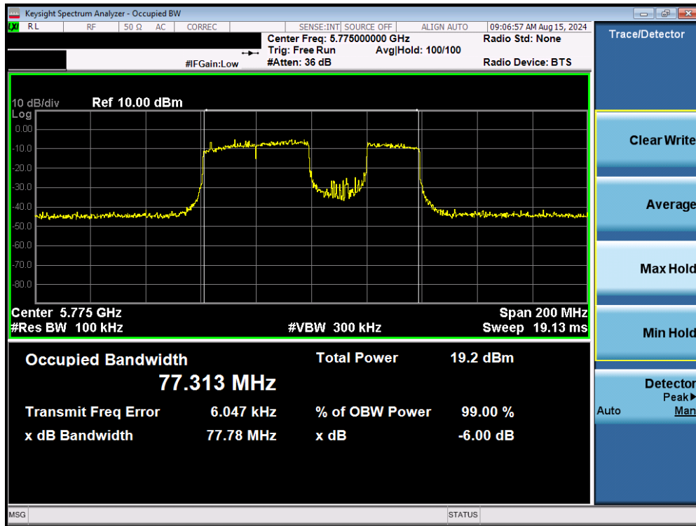
Plot 7-93. 6dB Bandwidth Plot MIMO ANT1 (80MHz BW 802.11be – Punctured (UNII Band 3) – Ch. 155)
