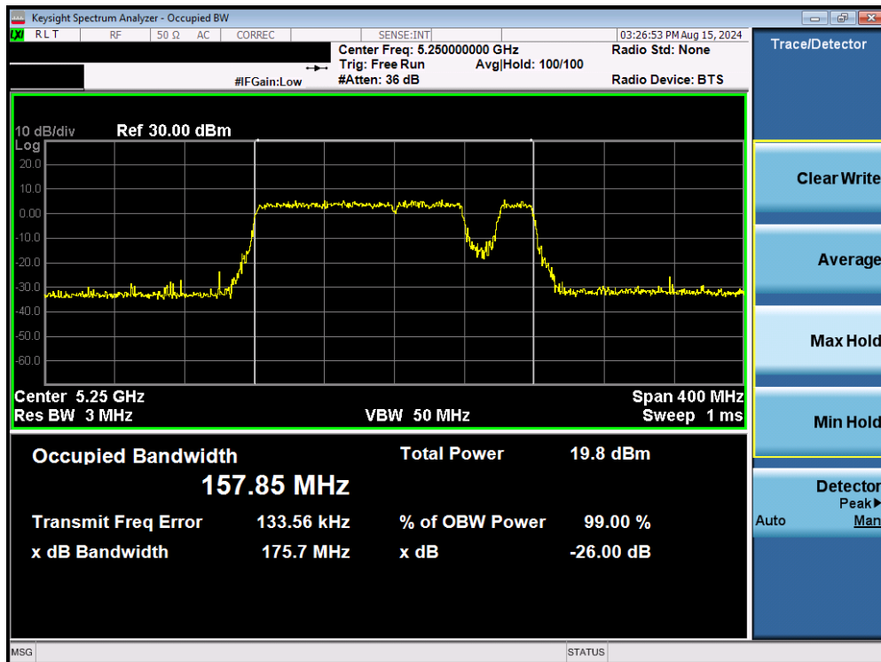
Plot 7-57. 26dB Bandwidth Plot MIMO ANT2 (160MHz BW 802.11be – Punctured (UNII Band 1/2A) – Ch. 50)
