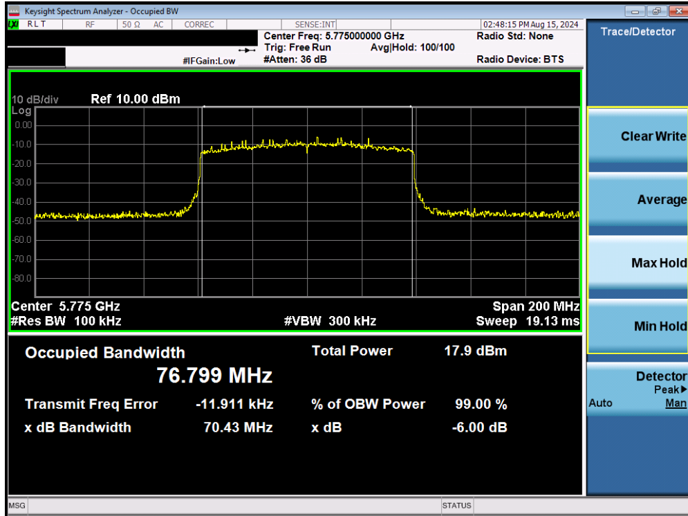
Plot 7-83. 6dB Bandwidth Plot MIMO ANT2 (80MHz BW 802.11be (UNII Band 3) – Ch. 155)
