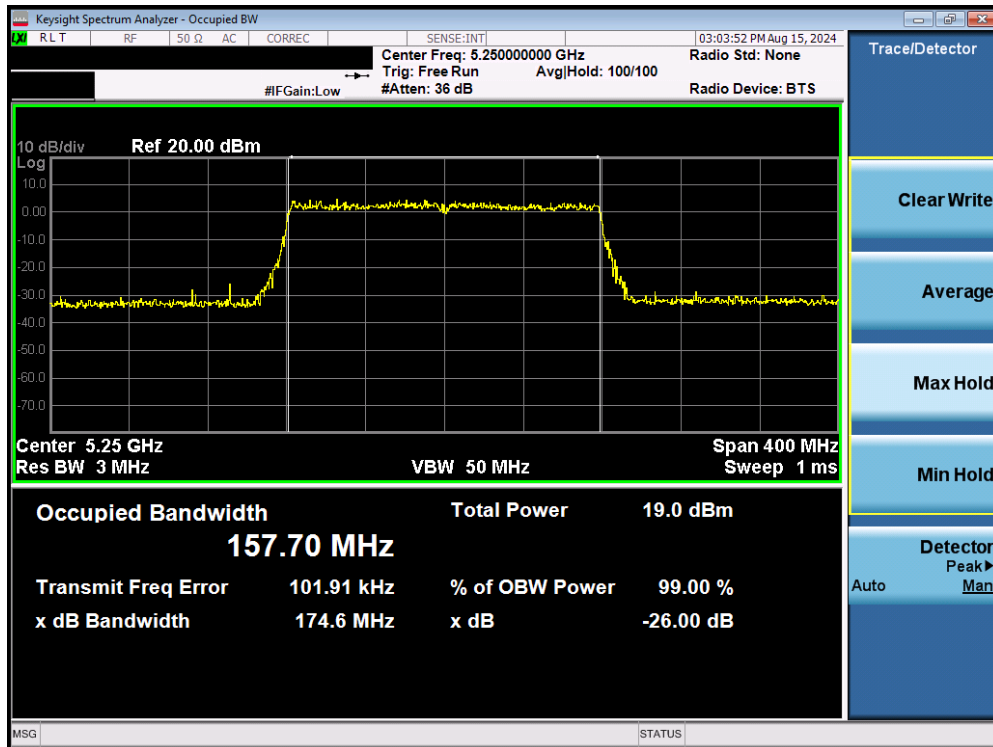
Plot 7-34. 26dB Bandwidth Plot MIMO ANT2 (160MHz BW 802.11be (UNII Band 1/2A) – Ch. 50)
