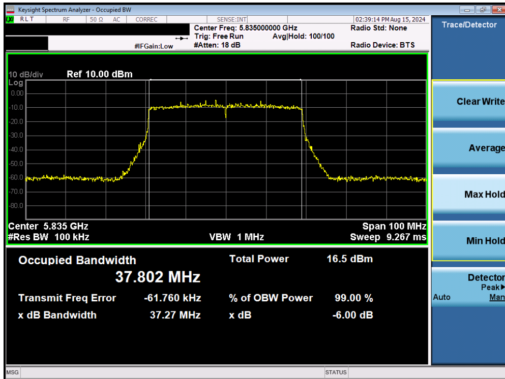
Plot 7-88. 6dB Bandwidth Plot MIMO ANT2 (40MHz BW 802.11be (UNII Band 3/4) – Ch. 167)
