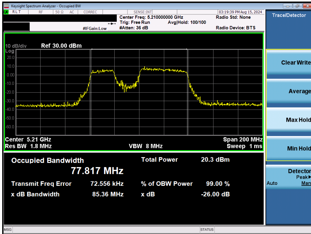
Plot 7-56. 26dB Bandwidth Plot MIMO ANT2 (80MHz BW 802.11be – Punctured (UNII Band 1) – Ch. 42)
