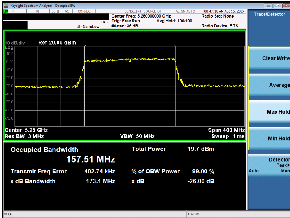
Plot 7-9. 26dB Bandwidth Plot MIMO ANT1 (160MHz BW 802.11be (UNII Band 1/2A) – Ch. 50)
