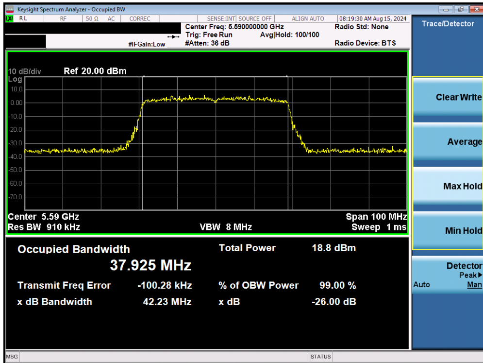
Plot 7-21. 26dB Bandwidth Plot MIMO ANT1 (40MHz BW 802.11be (UNII Band 2C) – Ch. 118)
