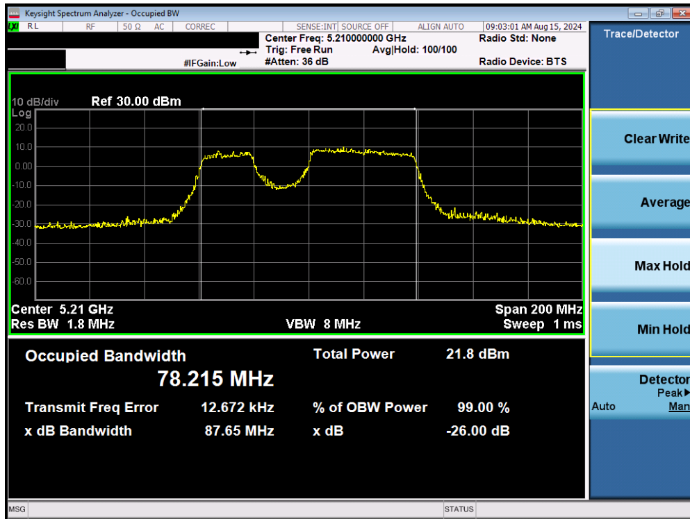
Plot 7-51. 26dB Bandwidth Plot MIMO ANT1 (80MHz BW 802.11be – Punctured (UNII Band 1) – Ch. 42)
