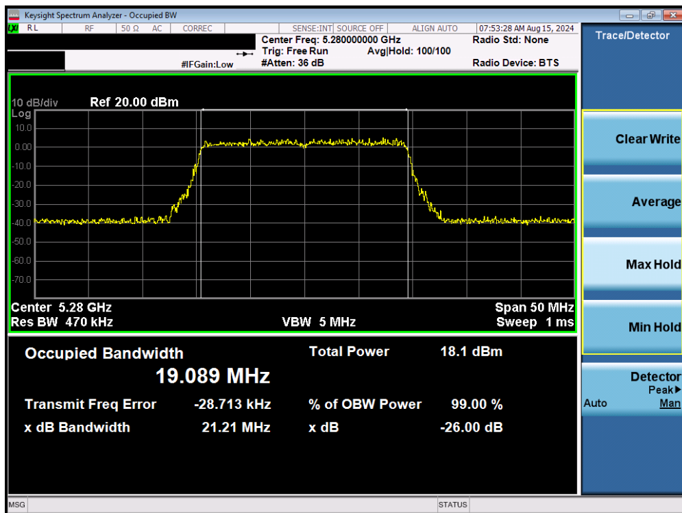
Plot 7-12. 26dB Bandwidth Plot MIMO ANT1 (20MHz BW 802.11be (UNII Band 2A) – Ch. 56)
