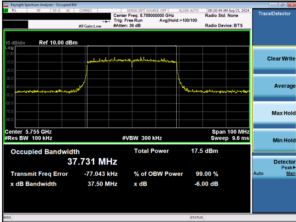
Plot 7-65. 6dB Bandwidth Plot MIMO ANT1 (40MHz BW 802.11be (UNII Band 3) – Ch. 151)
