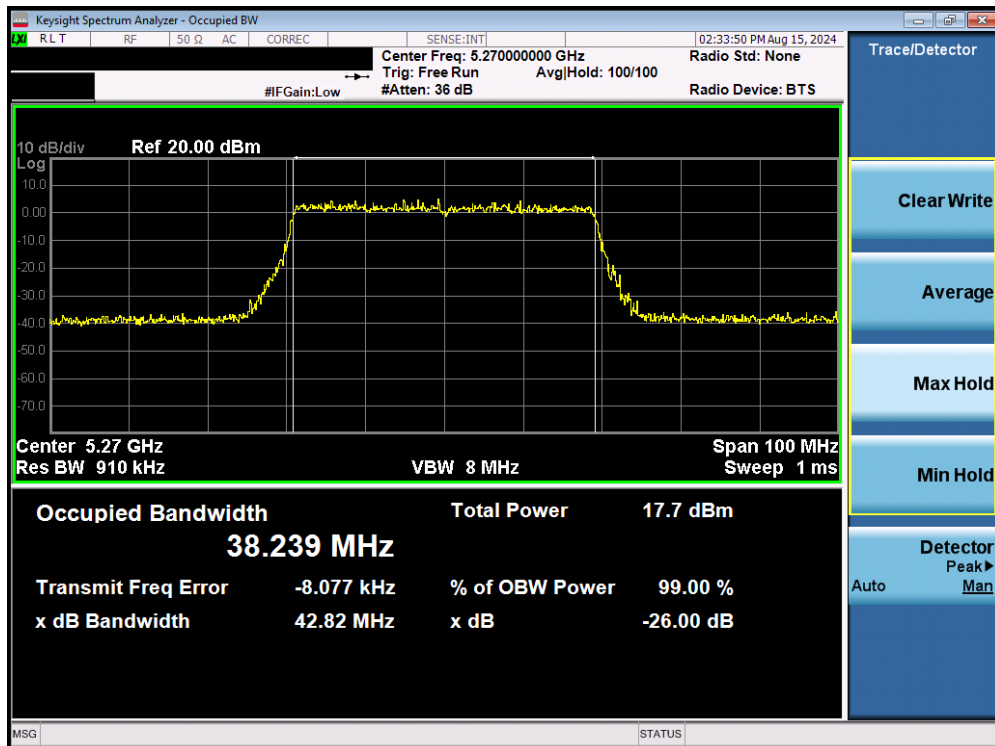
Plot 7-39. 26dB Bandwidth Plot MIMO ANT2 (40MHz BW 802.11be (UNII Band 2A) – Ch. 54)
