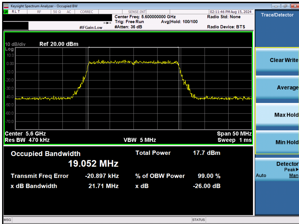
Plot 7-44. 26dB Bandwidth Plot MIMO ANT2 (20MHz BW 802.11be (UNII Band 2C) – Ch. 120)
