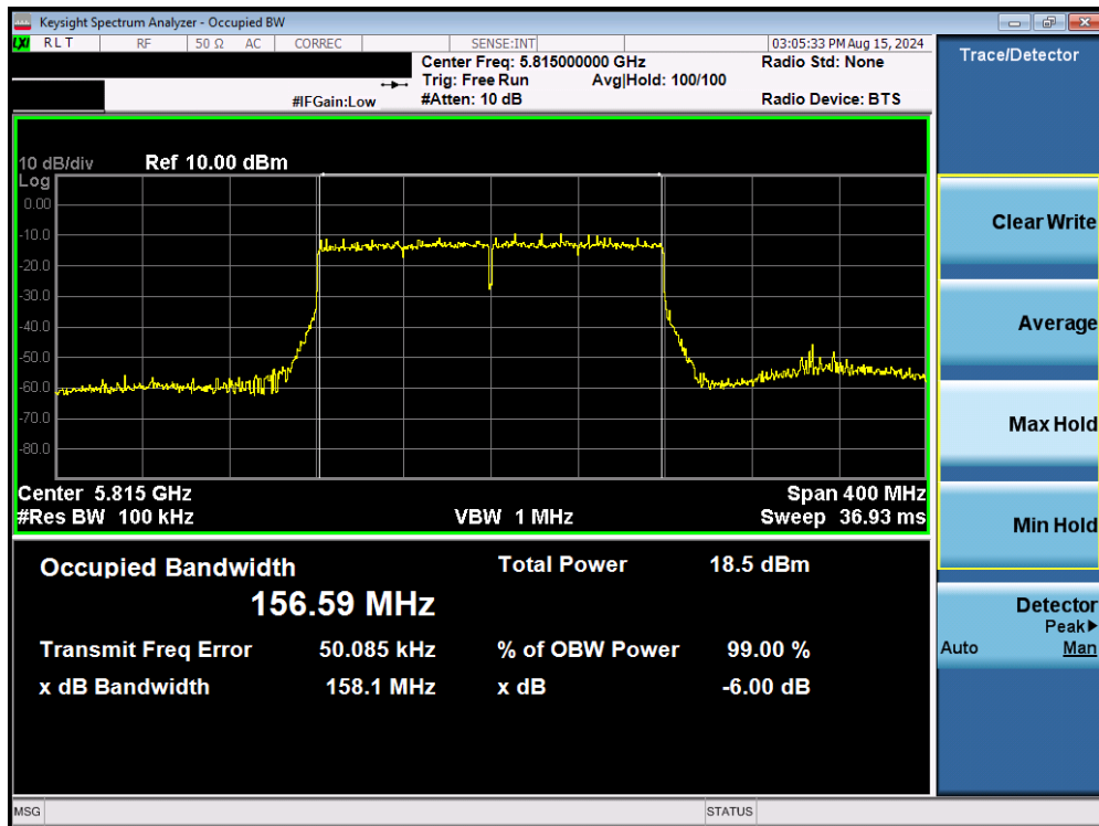
Plot 7-92. 6dB Bandwidth Plot MIMO ANT2 (160MHz BW 802.11be (UNII Band 3/4) – Ch. 163)
