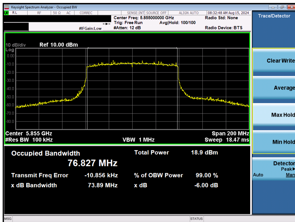
Plot 7-74. 6dB Bandwidth Plot MIMO ANT1 (80MHz BW 802.11be (UNII Band 3/4) – Ch. 171)
