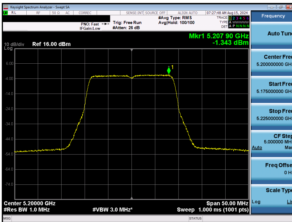
Plot 7-100. Power Spectral Density Plot MIMO ANT1 (20MHz BW 802.11n (UNII Band 1) – Ch. 40)
