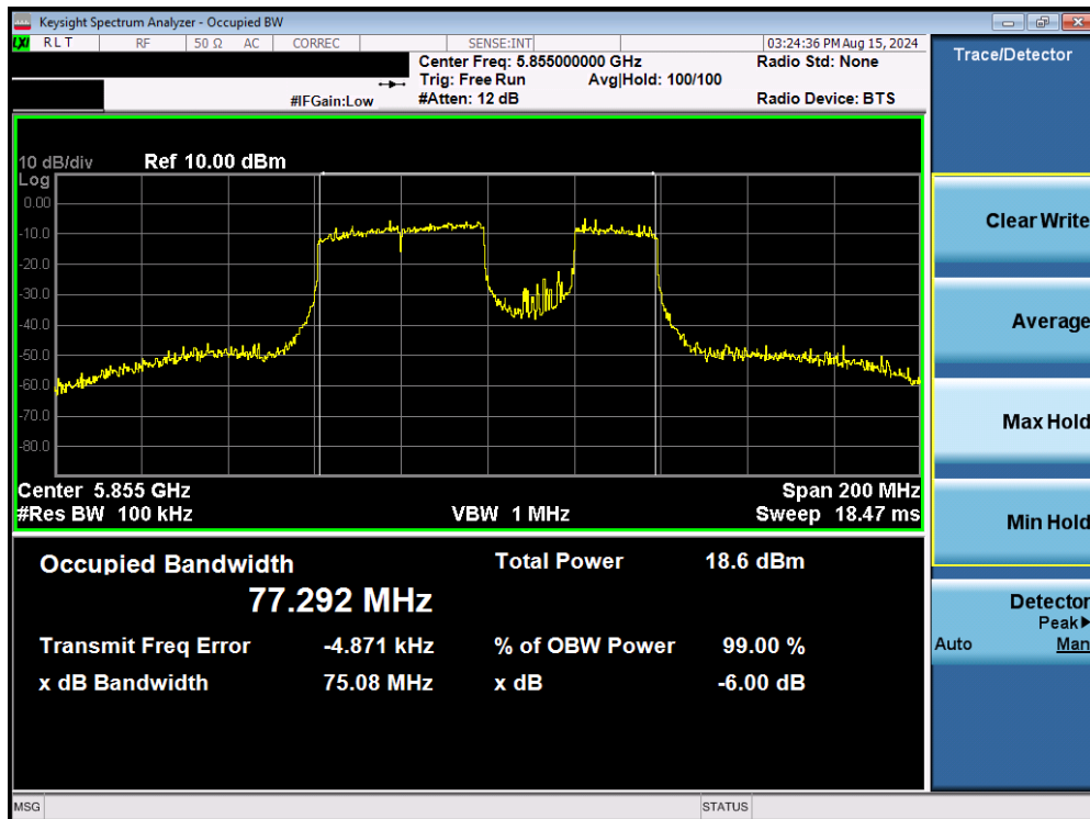
Plot 7-97. 6dB Bandwidth Plot MIMO ANT2 (80MHz BW 802.11be – Punctured (UNII Band 3/4) – Ch. 171)
