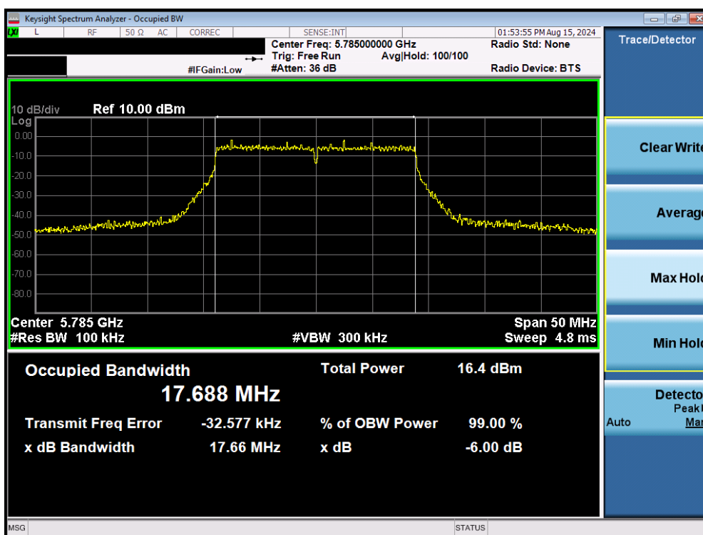
Plot 7-78. 6dB Bandwidth Plot MIMO ANT2 (20MHz BW 802.11n (UNII Band 3) – Ch. 157)
