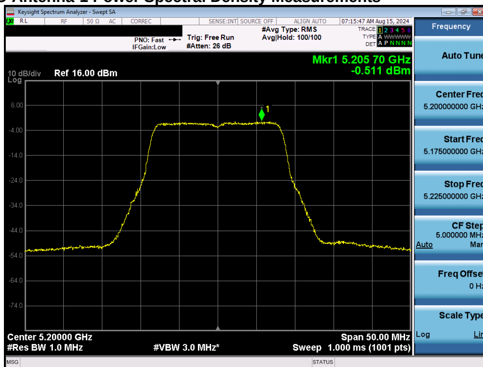
Plot 7-99. Power Spectral Density Plot MIMO ANT1 (802.11a (UNII Band 1) – Ch. 40)
