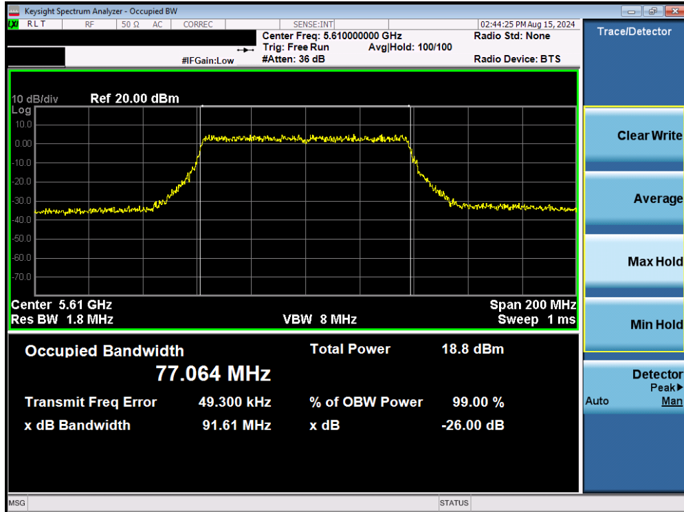
Plot 7-48. 26dB Bandwidth Plot MIMO ANT2 (80MHz BW 802.11be (UNII Band 2C)) –
