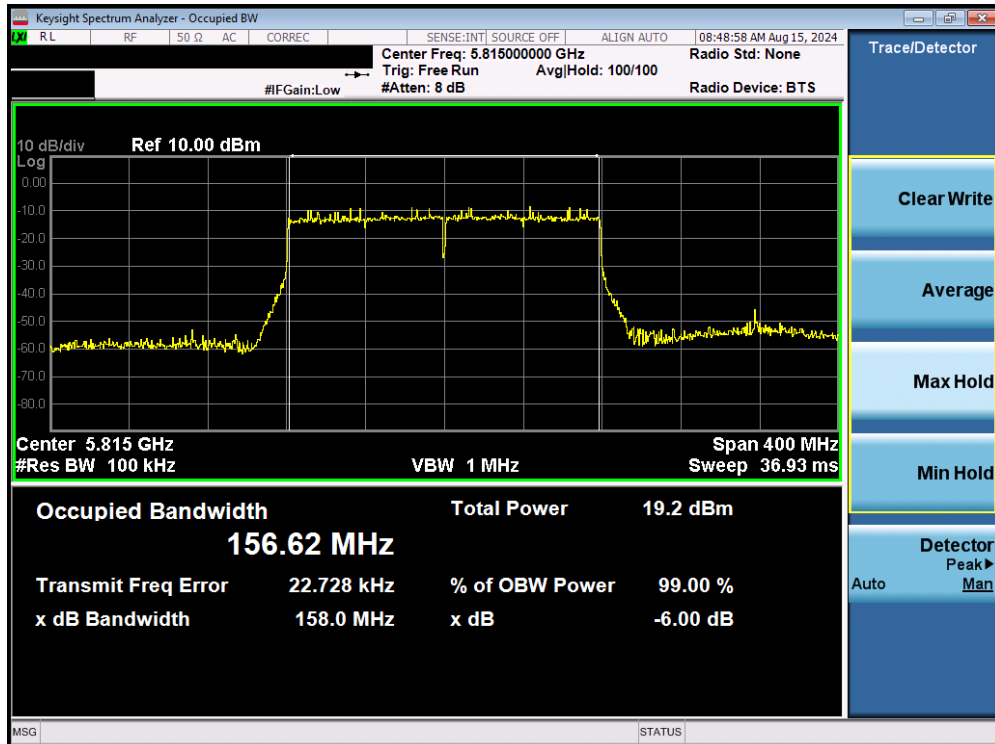
Plot 7-76. 6dB Bandwidth Plot MIMO ANT1 (160MHz BW 802.11be (UNII Band 3/4) – Ch. 163)
