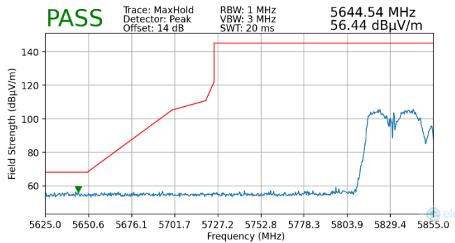
Plot 7-222. Radiated Lower Band Edge Plot MIMO (Peak – UNII Band 4)
