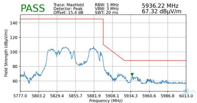
Plot 7-234. Radiated Upper Band Edge Plot MIMO (Peak – UNII Band 4)
