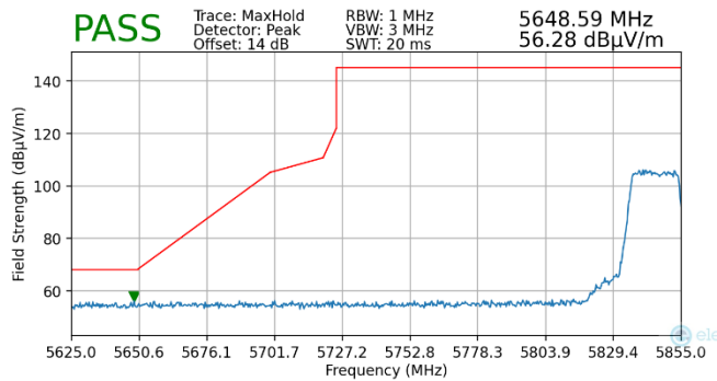
Plot 7-212. Radiated Lower Band Edge Plot MIMO (Peak – UNII Band 4)
