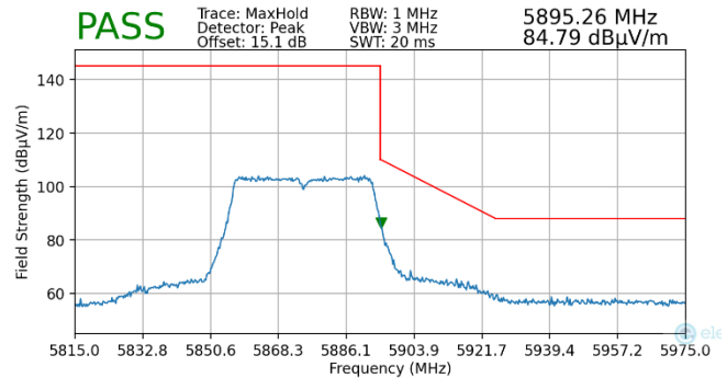
Plot 7-224. Radiated Upper Band Edge Plot MIMO (Peak – UNII Band 4)
