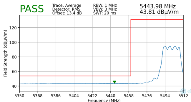
Plot 7-209. Radiated Lower Band Edge Plot MIMO (Average – UNII Band 2C)
