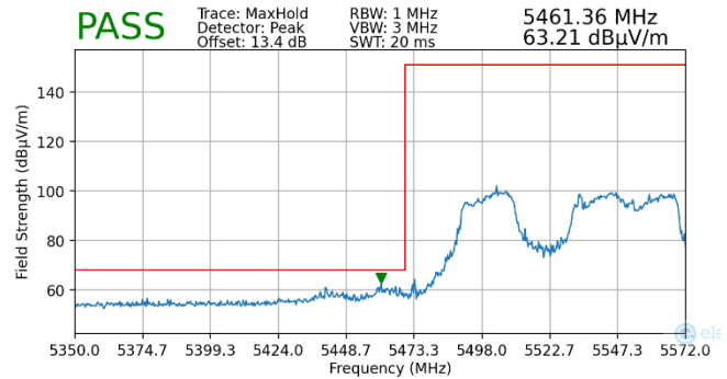
Plot 7-230. Radiated Lower Band Edge Plot MIMO (Peak – UNII Band 2C)
