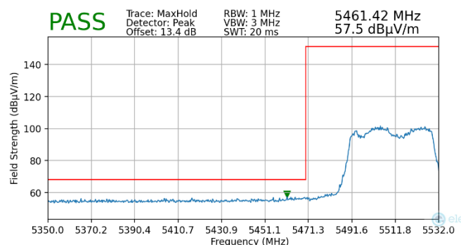
Plot 7-220. Radiated Lower Band Edge Plot MIMO (Peak – UNII Band 2C)
