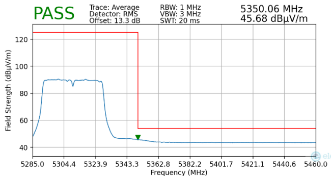
Plot 7-217. Radiated Upper Band Edge Plot MIMO (Average – UNII Band 2A)
