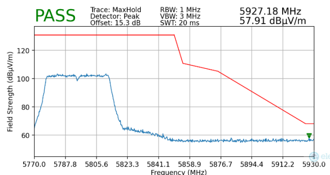
Plot 7-221. Radiated Upper Band Edge Plot MIMO (Peak – UNII Band 3)
