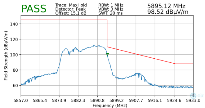
Plot 7-214. Radiated Upper Band Edge Plot MIMO (Peak – UNII Band 4)
