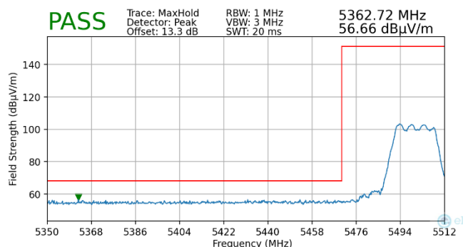
Plot 7-210. Radiated Lower Band Edge Plot MIMO (Peak – UNII Band 2C)
