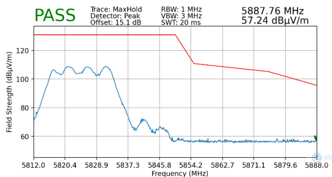
Plot 7-211. Radiated Upper Band Edge Plot MIMO (Peak – UNII Band 3)
