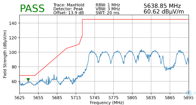
Plot 7-241. Radiated Lower Band Edge Plot MIMO (Peak – UNII Band 4)
