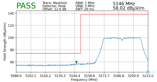
Plot 7-216. Radiated Lower Band Edge Plot MIMO (Peak – UNII Band 1)
