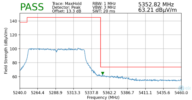
Plot 7-228. Radiated Upper Band Edge Plot MIMO (Peak – UNII Band 2A)
