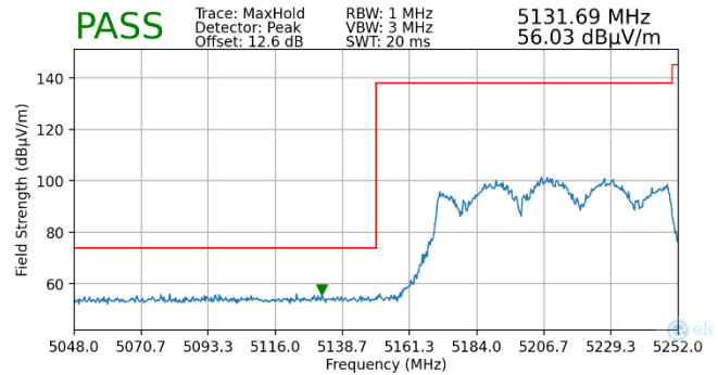
Plot 7-226. Radiated Lower Band Edge Plot MIMO (Peak – UNII Band 1)
