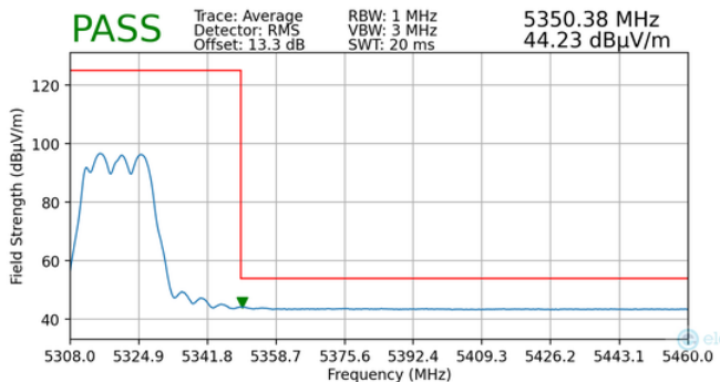
Plot 7-207. Radiated Upper Band Edge Plot MIMO (Average – UNII Band 2A)
