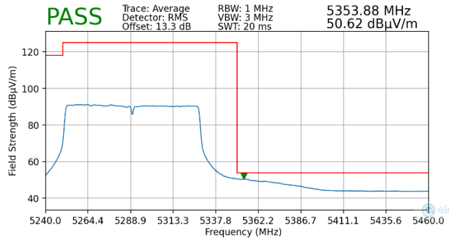
Plot 7-227. Radiated Upper Band Edge Plot MIMO (Average – UNII Band 2A)
