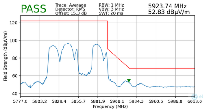
Plot 7-233. Radiated Upper Band Edge Plot MIMO (Average – UNII Band 4)
