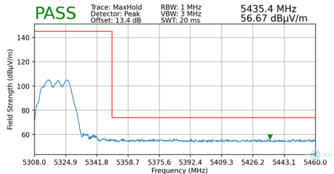
Plot 7-208. Radiated Upper Band Edge Plot MIMO (Peak – UNII Band 2A)
