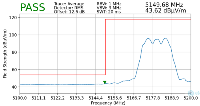
Plot 7-205. Radiated Lower Band Edge Plot MIMO (Average – UNII Band 1)
