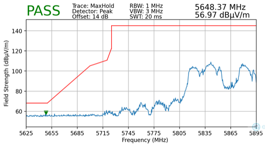
Plot 7-232. Radiated Lower Band Edge Plot MIMO (Peak – UNII Band 4)
