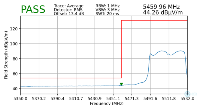
Plot 7-219. Radiated Lower Band Edge Plot MIMO (Average – UNII Band 2C)
