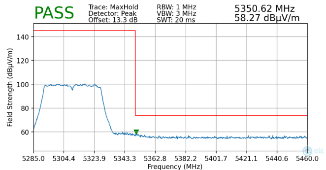
Plot 7-218. Radiated Upper Band Edge Plot MIMO (Peak – UNII Band 2A)
