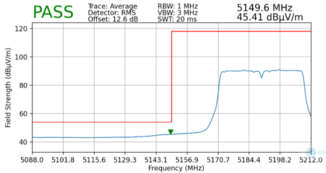
Plot 7-215. Radiated Lower Band Edge Plot MIMO (Average – UNII Band 1)
