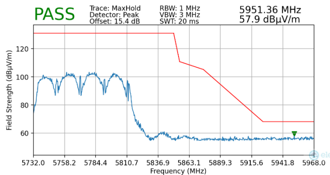
Plot 7-231. Radiated Upper Band Edge Plot MIMO (Peak – UNII Band 3)
