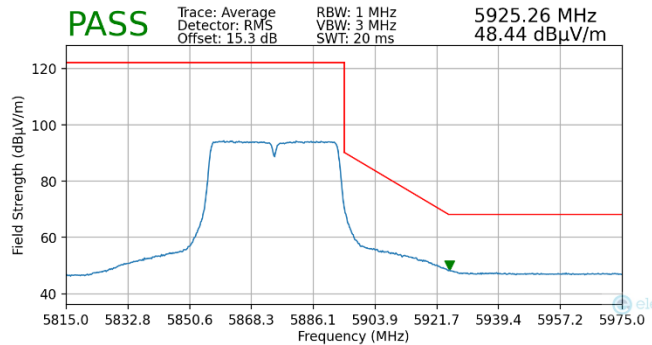
Plot 7-223. Radiated Upper Band Edge Plot MIMO (Average – UNII Band 4)
