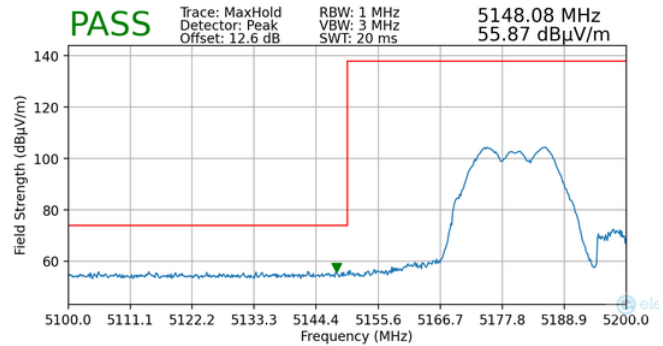
Plot 7-206. Radiated Lower Band Edge Plot MIMO (Peak – UNII Band 1)
