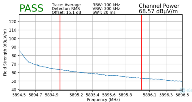
Plot 7-213. Radiated Upper Band Edge Plot MIMO (Average – UNII Band 4)
