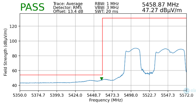
Plot 7-229. Radiated Lower Band Edge Plot MIMO (Average – UNII Band 2C)
