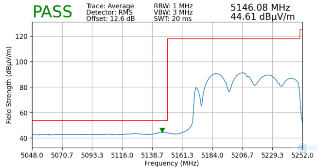
Plot 7-225. Radiated Lower Band Edge Plot MIMO (Average – UNII Band 1)
