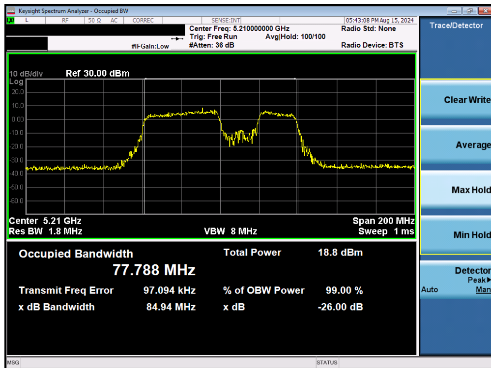
Plot 7-54. 26dB Bandwidth Plot MIMO ANT2 (80MHz BW 802.11be – 484+242 Tones (UNII Band 1) – Ch. 42)
