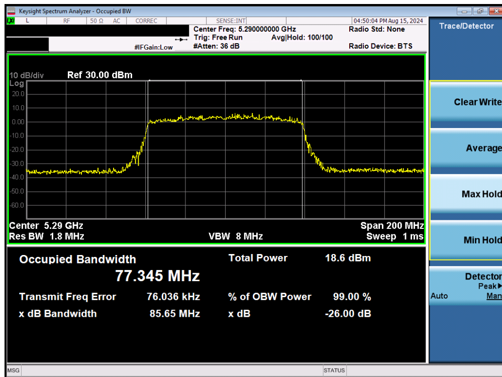
Plot 7-48. 26dB Bandwidth Plot MIMO ANT2 (80MHz BW 802.11be – 996 Tones (UNII Band 2A) – Ch. 58)
