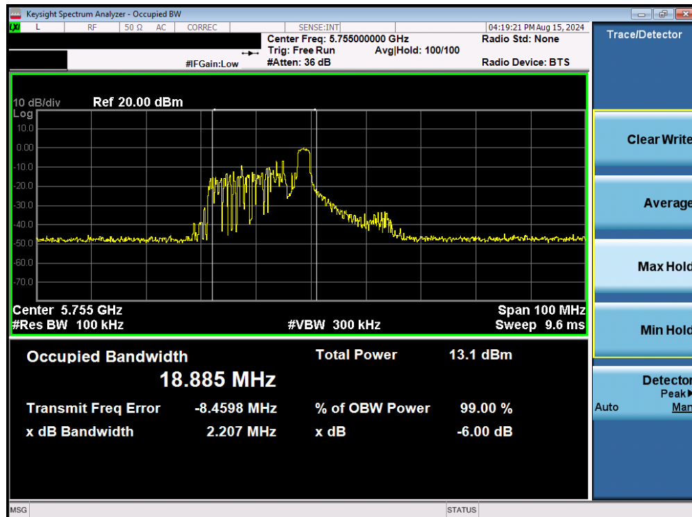
Plot 7-81. 6dB Bandwidth Plot MIMO ANT2 (40MHz BW 802.11be – 26 Tones (UNII Band 3) – Ch. 151)
