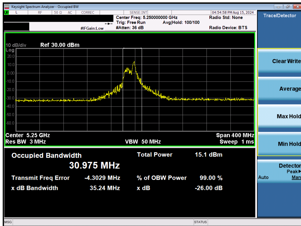
Plot 7-34. 26dB Bandwidth Plot MIMO ANT2 (160MHz BW 802.11be – 26 Tones (UNII Band 1/2A) – Ch. 50)
