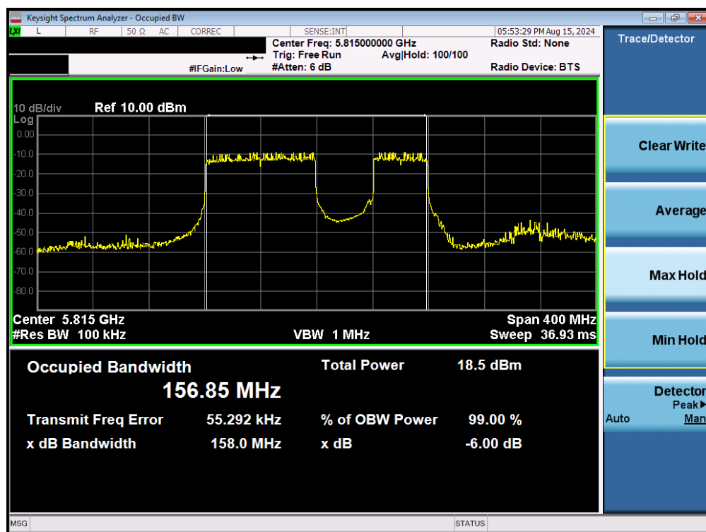
Plot 7-98. 6dB Bandwidth Plot MIMO ANT2 (160MHz BW 802.11be – 996+484T Tones (UNII Band 3/4) – Ch. 163)
