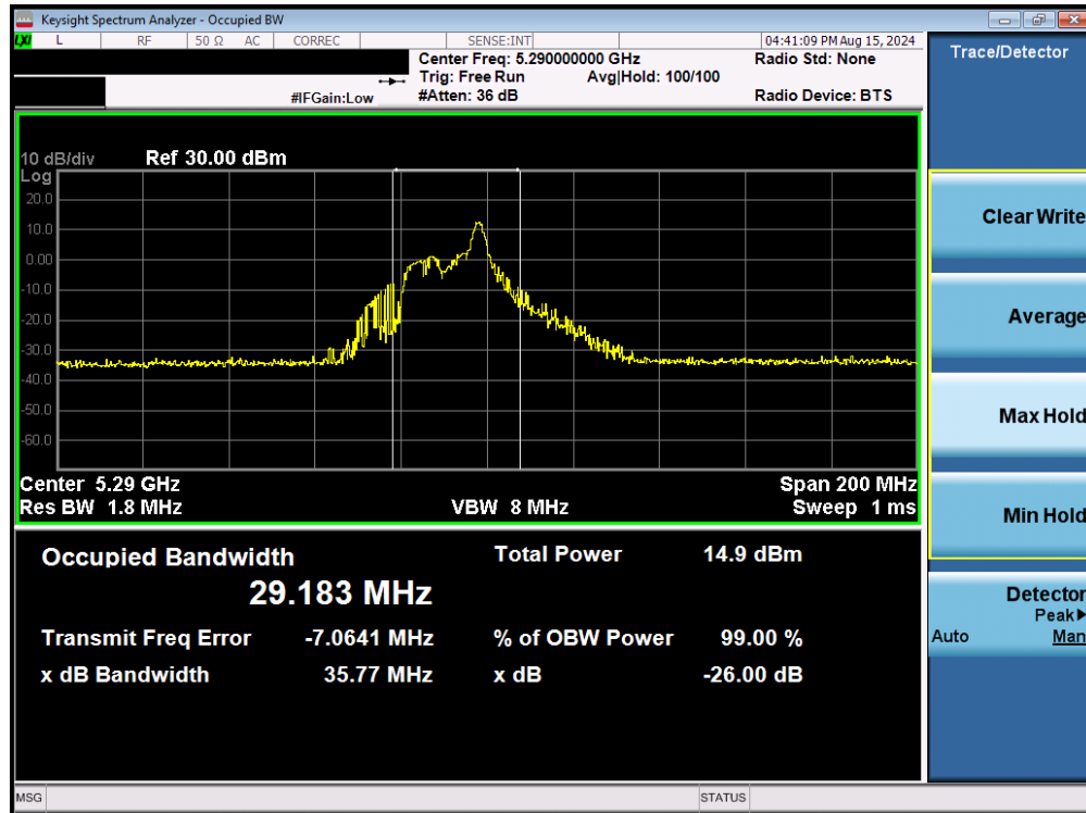
Plot 7-37. 26dB Bandwidth Plot MIMO ANT2 (80MHz BW 802.11be – 26 Tones (UNII Band 2A) – Ch. 58)
