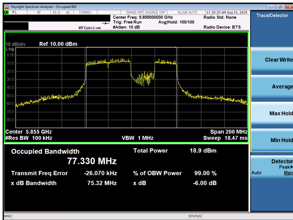
Plot 7-78. 6dB Bandwidth Plot MIMO ANT1 (80MHz BW 802.11be – 484+242 Tones (UNII Band 3/4) – Ch. 171)
