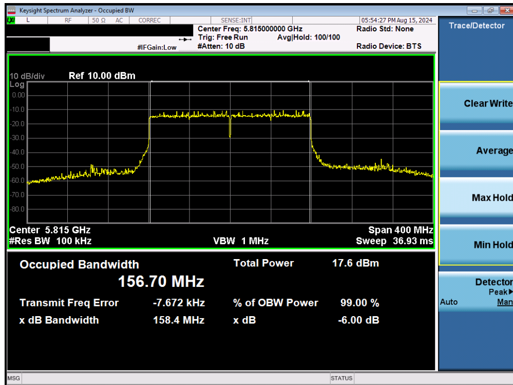
Plot 7-93. 6dB Bandwidth Plot MIMO ANT2 (160MHz BW 802.11be – 996*2 Tones (UNII Band 3/4) – Ch. 163)
