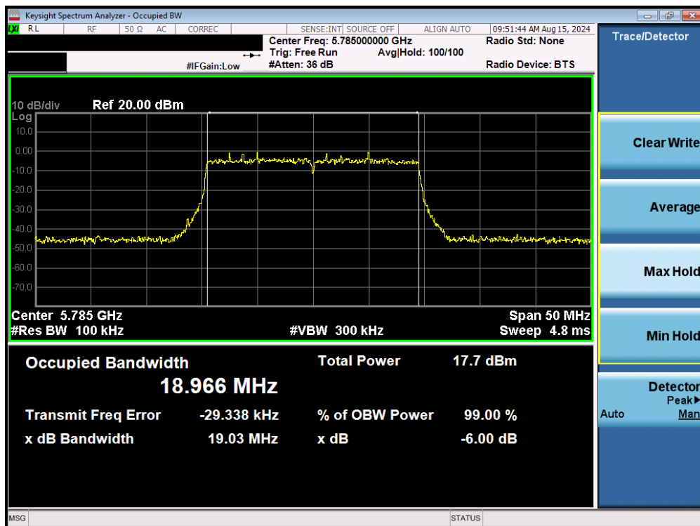
Plot 7-68. 6dB Bandwidth Plot MIMO ANT1 (20MHz BW 802.11be – 242 Tones (UNII Band 3) – Ch. 157)
