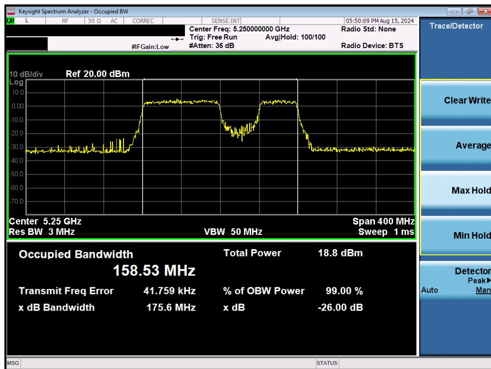
Plot 7-55. 26dB Bandwidth Plot MIMO ANT2 (160MHz BW 802.11be – 996+484 Tones (UNII Band 1/2A) – Ch. 50)
