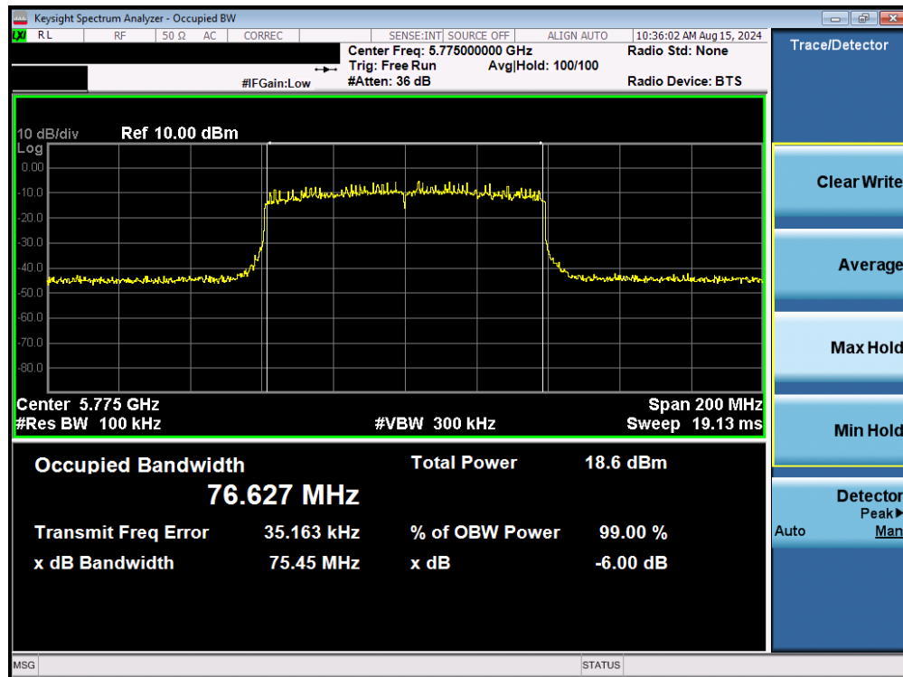
Plot 7-70. 6dB Bandwidth Plot MIMO ANT1 (80MHz BW 802.11be – 996 Tones (UNII Band 3) – Ch. 155)
