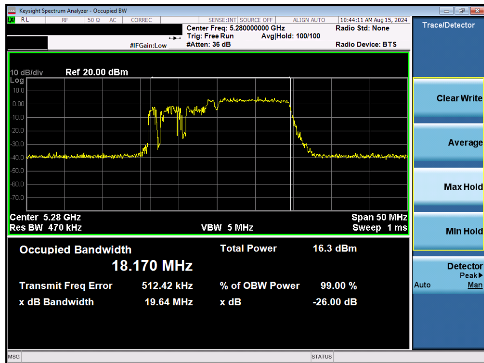
Plot 7-26. 26dB Bandwidth Plot MIMO ANT1 (20MHz BW 802.11be – 106+26 Tones (UNII Band 2A) – Ch. 56)
