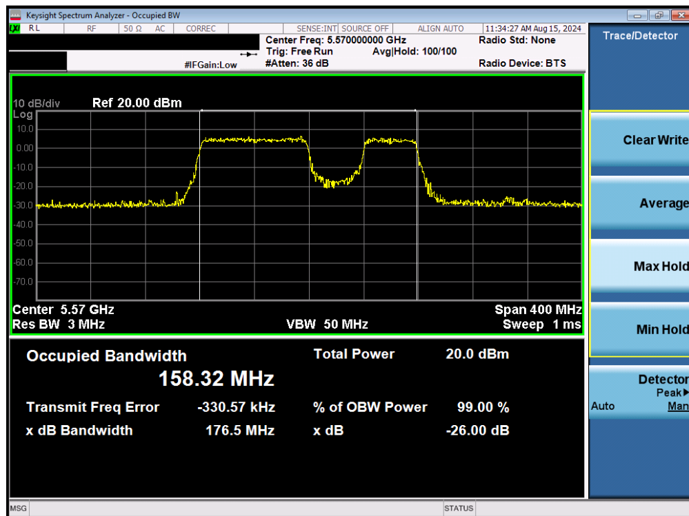
Plot 7-30. 26dB Bandwidth Plot MIMO ANT1 (160MHz BW 802.11be – 996+484 Tones (UNII Band 2C) – Ch. 114)
