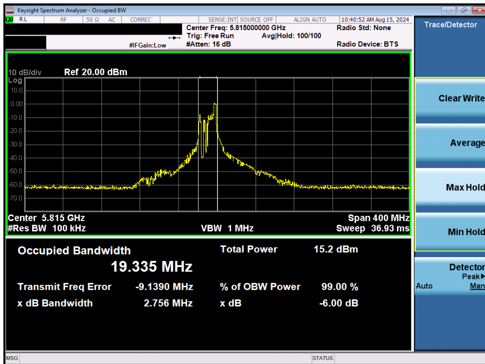
Plot 7-67. 6dB Bandwidth Plot MIMO ANT1 (160MHz BW 802.11be – 26 Tones (UNII Band 3/4) – Ch. 163)
