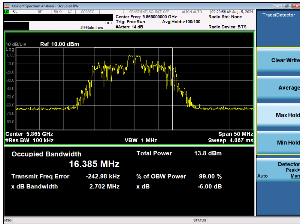
Plot 7-64. 6dB Bandwidth Plot MIMO ANT1 (20MHz BW 802.11be – 26 Tones (UNII Band 4) – Ch. 173)
