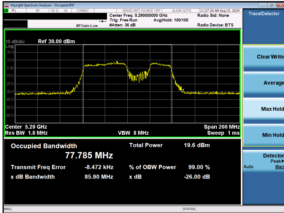
Plot 7-27. 26dB Bandwidth Plot MIMO ANT1 (80MHz BW 802.11be – 484+242 Tones (UNII Band 2A) – Ch. 58)
