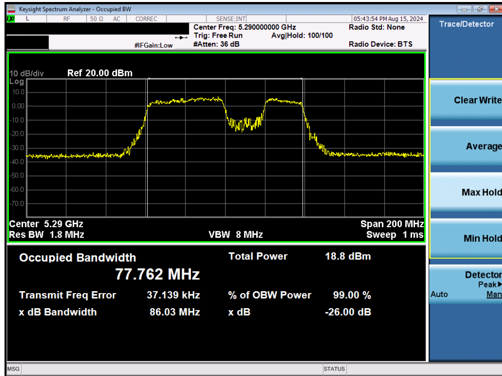
Plot 7-57. 26dB Bandwidth Plot MIMO ANT2 (80MHz BW 802.11be – 484+242 Tones (UNII Band 2A) – Ch. 58)
