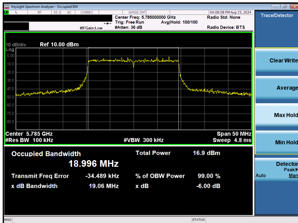
Plot 7-87. 6dB Bandwidth Plot MIMO ANT2 (20MHz BW 802.11be – 242 Tones (UNII Band 3) – Ch. 157)
