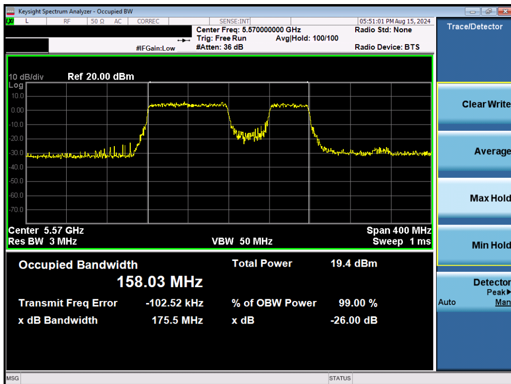
Plot 7-60. 26dB Bandwidth Plot MIMO ANT2 (160MHz BW 802.11be – 996+484 Tones (UNII Band 2C) – Ch. 114)
