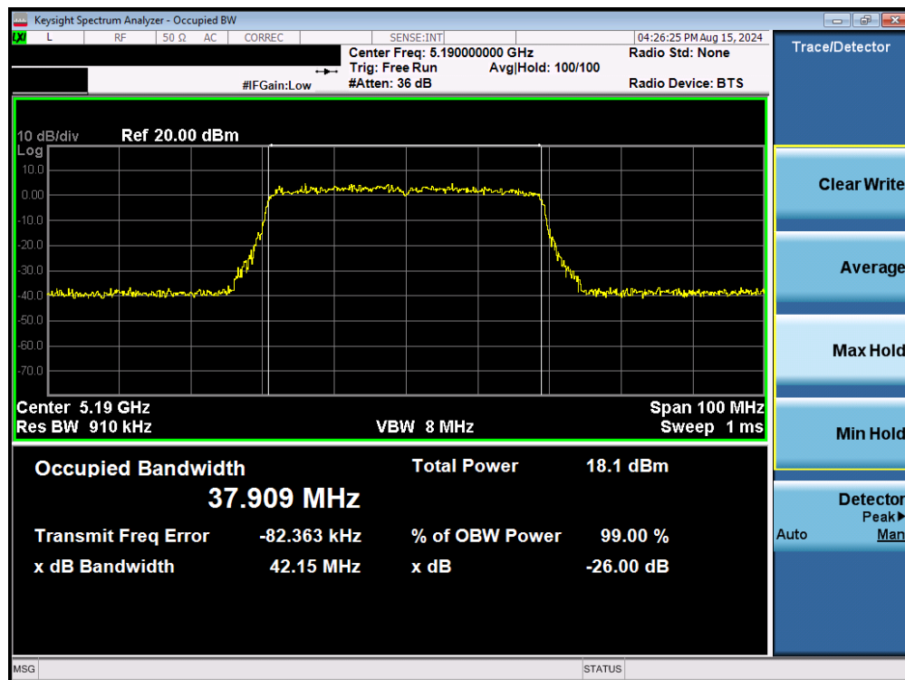
Plot 7-43. 26dB Bandwidth Plot MIMO ANT2 (40MHz BW 802.11be – 484 Tones (UNII Band 1) – Ch. 38)
