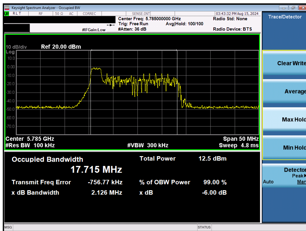
Plot 7-80. 6dB Bandwidth Plot MIMO ANT2 (20MHz BW 802.11be – 26 Tones (UNII Band 3) – Ch. 157)
