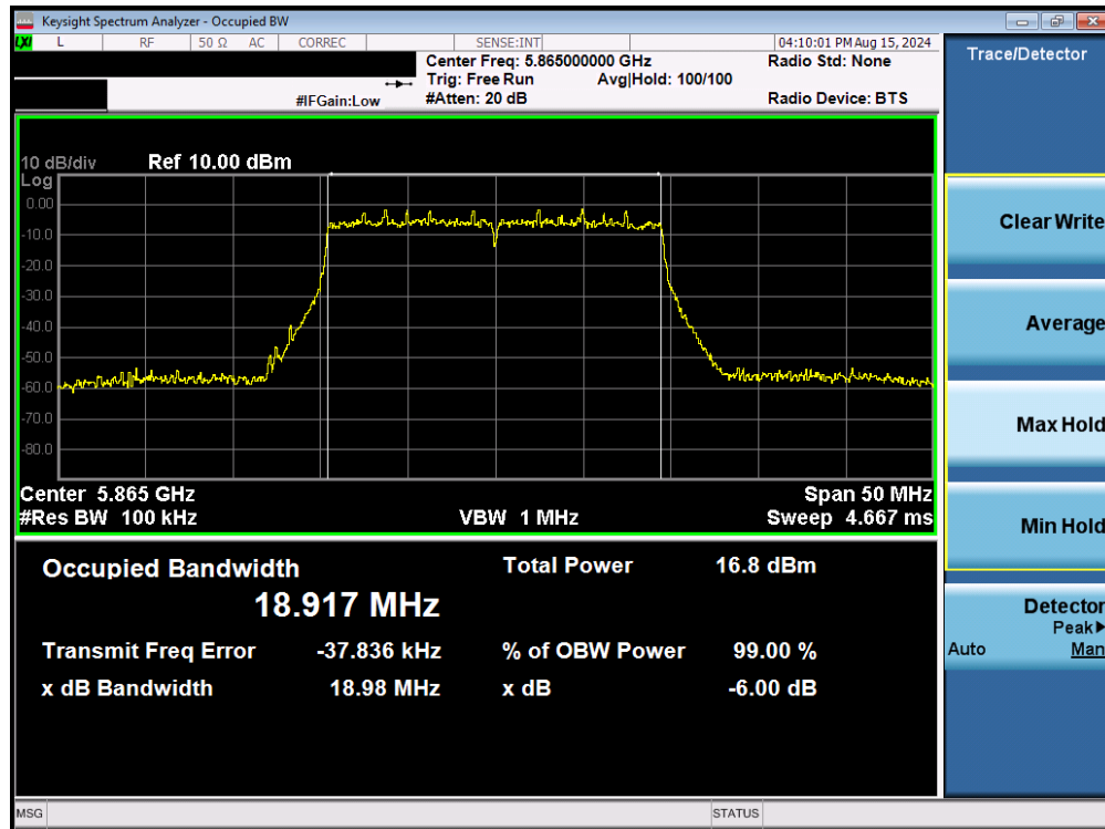
Plot 7-90. 6dB Bandwidth Plot MIMO ANT2 (20MHz BW 802.11be – 242 Tones (UNII Band 4) – Ch. 173)
