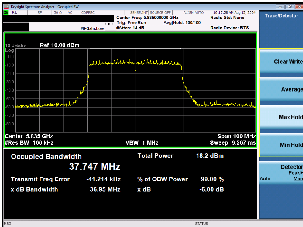
Plot 7-72. 6dB Bandwidth Plot MIMO ANT1 (40MHz BW 802.11be – 484 Tones (UNII Band 3/4) – Ch. 167)
