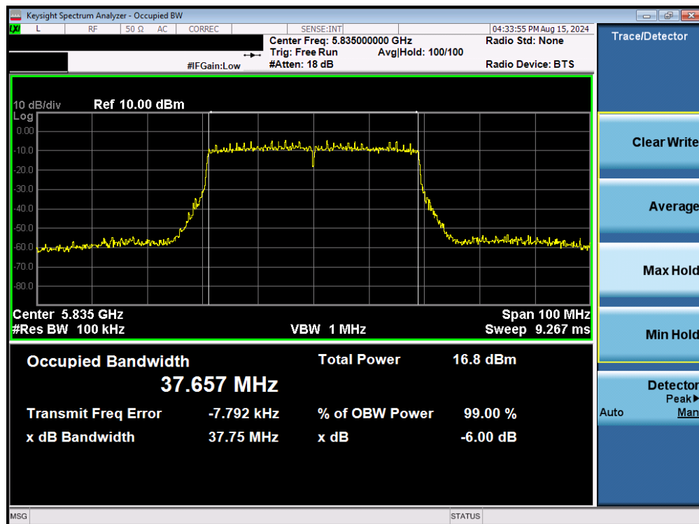
Plot 7-91. 6dB Bandwidth Plot MIMO ANT2 (40MHz BW 802.11be – 484 Tones (UNII Band 3/4) – Ch. 167)
