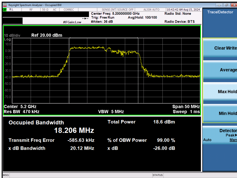
Plot 7-23. 26dB Bandwidth Plot MIMO ANT1 (20MHz BW 802.11be – 106+26T Tones (UNII Band 1) – Ch. 40)
