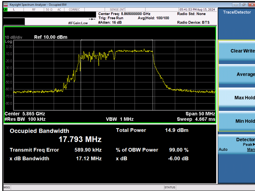
Plot 7-96. 6dB Bandwidth Plot MIMO ANT2 (20MHz BW 802.11be – 106+26 Tones (UNII Band 4) – Ch. 173)
