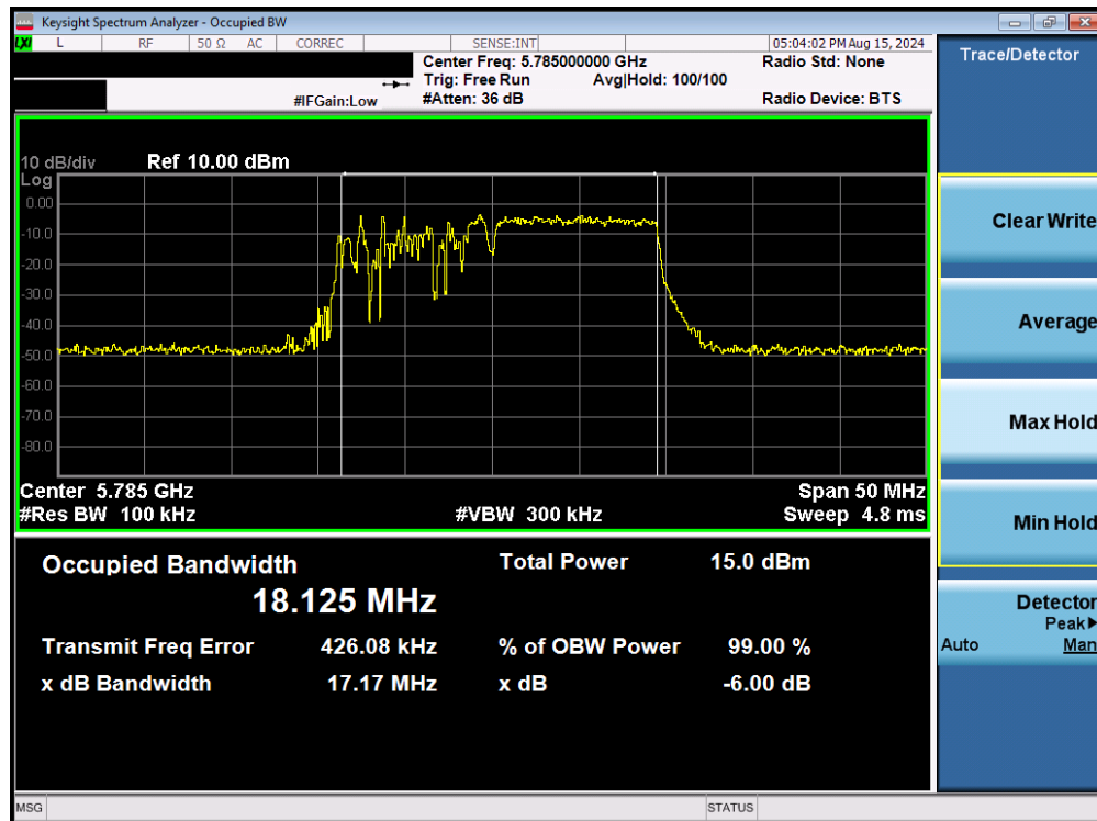
Plot 7-94. 6dB Bandwidth Plot MIMO ANT2 (20MHz BW 802.11be – 106+26 Tones (UNII Band 3) – Ch. 157)
