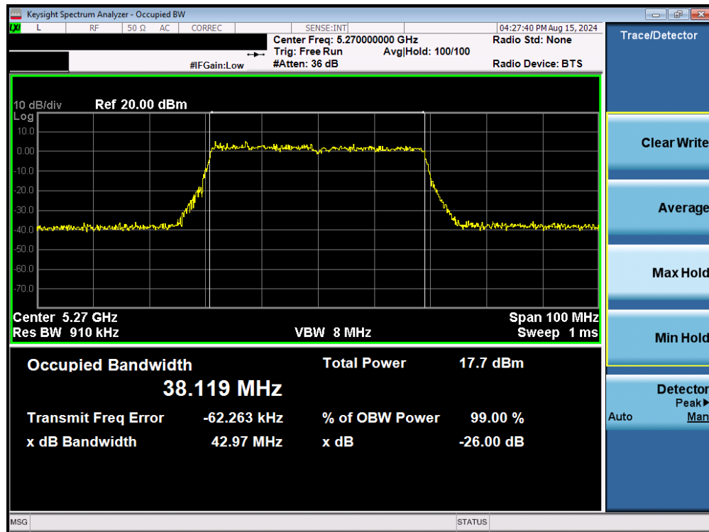
Plot 7-47. 26dB Bandwidth Plot MIMO ANT2 (40MHz BW 802.11be – 484 Tones (UNII Band 2A) – Ch. 54)
