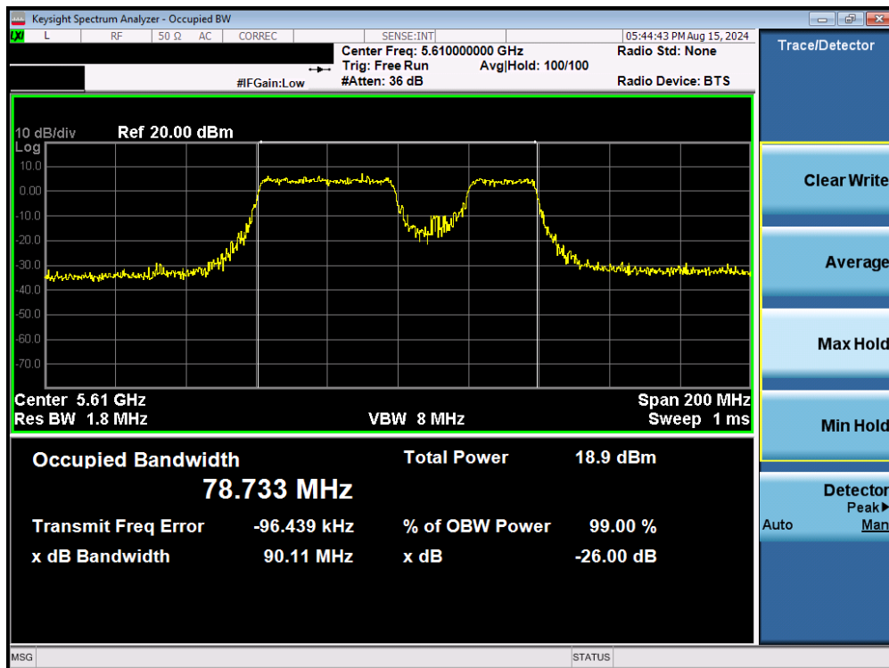
Plot 7-59. 26dB Bandwidth Plot MIMO ANT2 (80MHz BW 802.11be – 484+242 Tones (UNII Band 2C) – Ch. 122)
