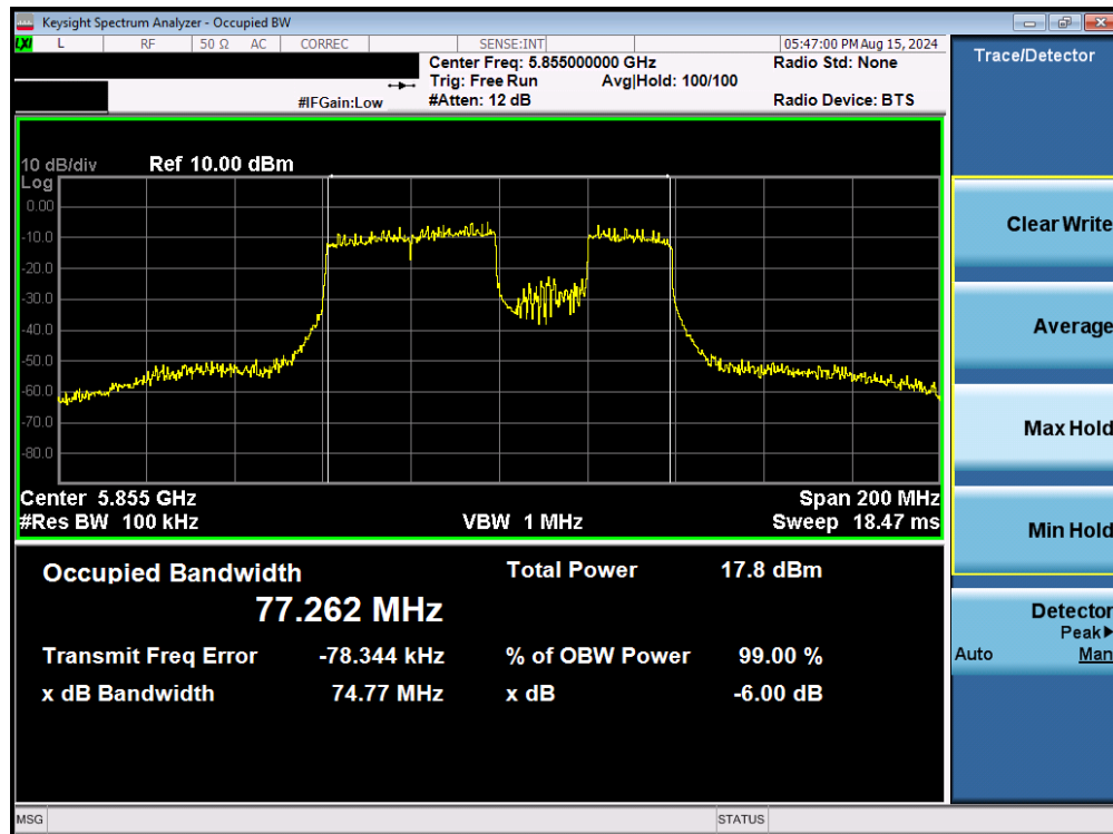
Plot 7-97. 6dB Bandwidth Plot MIMO ANT2 (80MHz BW 802.11be – 484+242 Tones (UNII Band 3/4) – Ch. 171)
