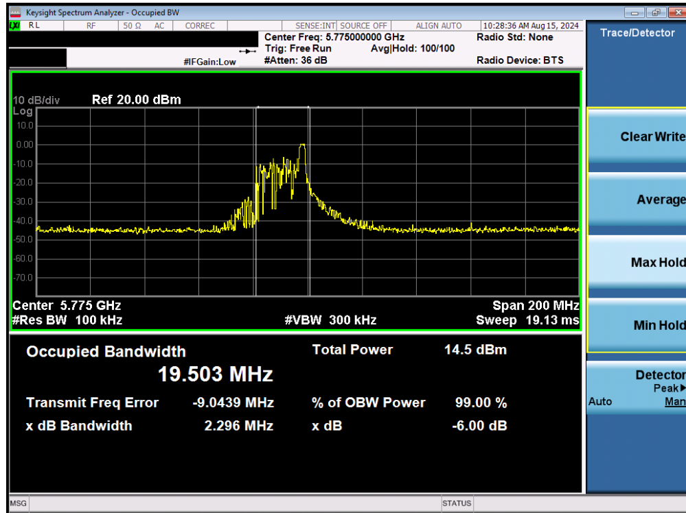
Plot 7-63. 6dB Bandwidth Plot MIMO ANT1 (80MHz BW 802.11be – 26 Tones (UNII Band 3) – Ch. 155)
