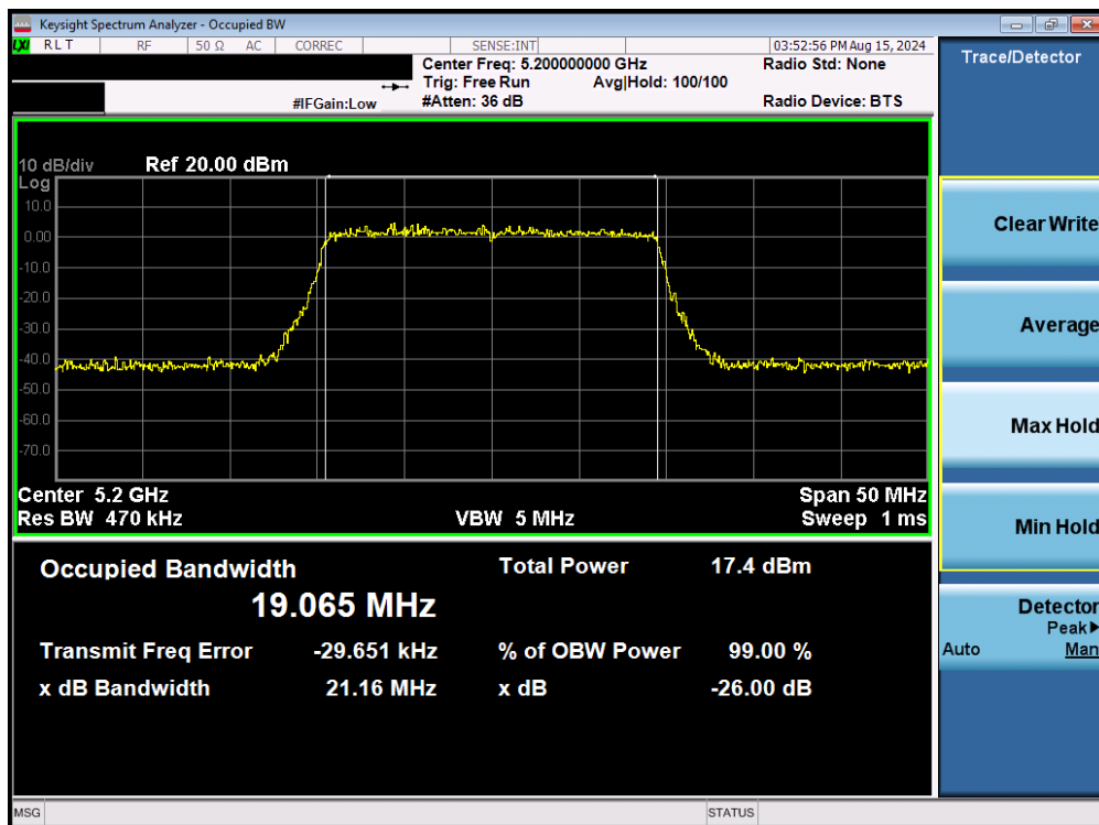
Plot 7-42. 26dB Bandwidth Plot MIMO ANT2 (20MHz BW 802.11be – 242 Tones (UNII Band 1) – Ch. 40)
