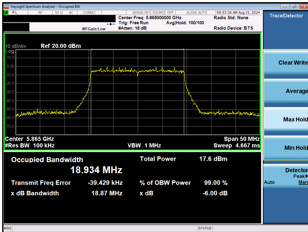
Plot 7-71. 6dB Bandwidth Plot MIMO ANT1 (20MHz BW 802.11be – 242 Tones (UNII Band 4) – Ch. 173)
