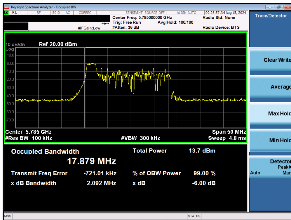
Plot 7-61. 6dB Bandwidth Plot MIMO ANT1 (20MHz BW 802.11be – 26 Tones (UNII Band 3) – Ch. 157)
