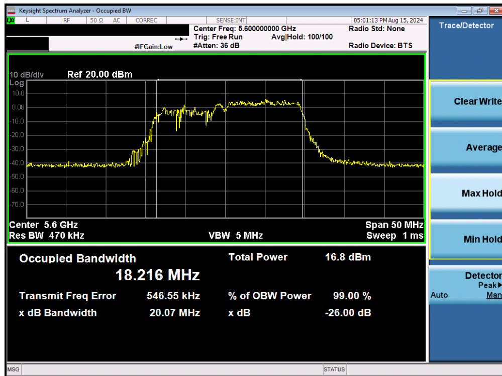
Plot 7-58. 26dB Bandwidth Plot MIMO ANT2 (20MHz BW 802.11be – 106+26 Tones (UNII Band 2C) – Ch. 120)
