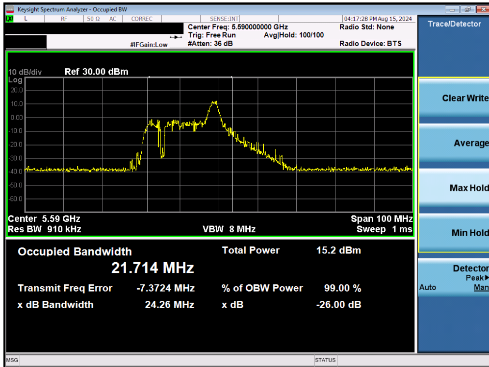
Plot 7-39. 26dB Bandwidth Plot MIMO ANT2 (40MHz BW 802.11be – 26 Tones (UNII Band 2C) – Ch. 118)
