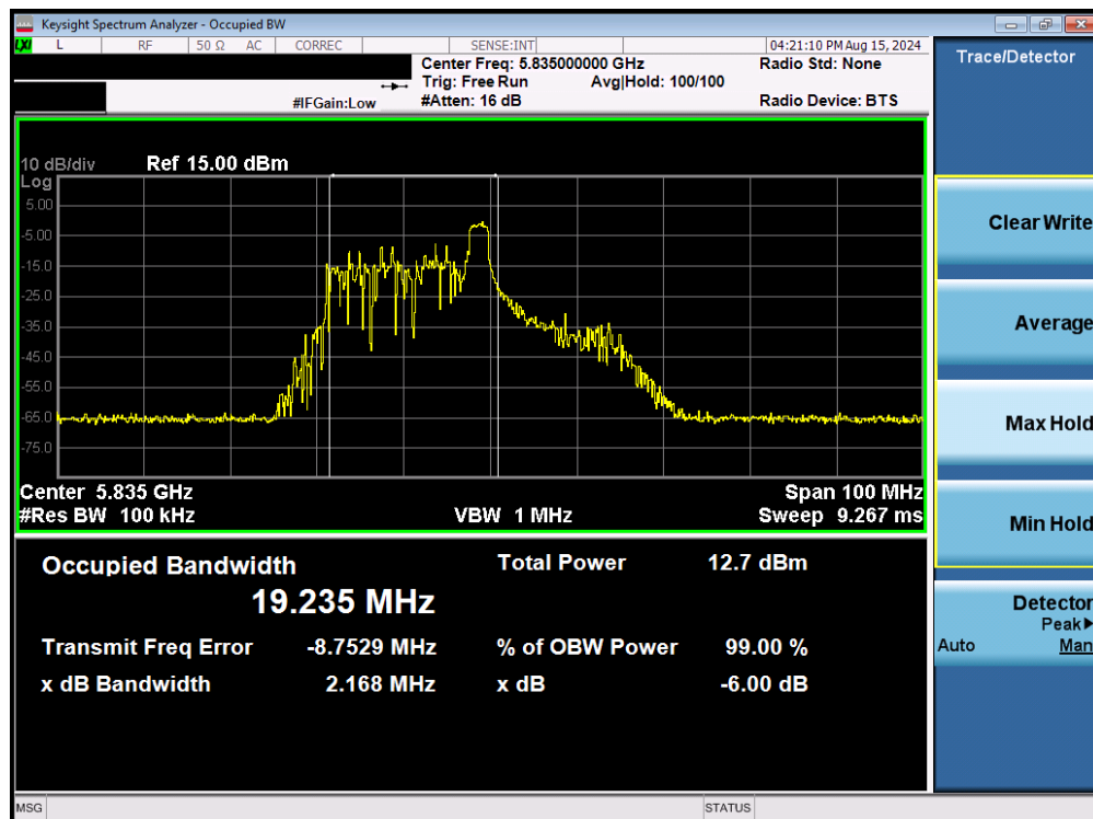
Plot 7-84. 6dB Bandwidth Plot MIMO ANT2 (40MHz BW 802.11be – 26 Tones (UNII Band 3/4) – Ch. 167)
