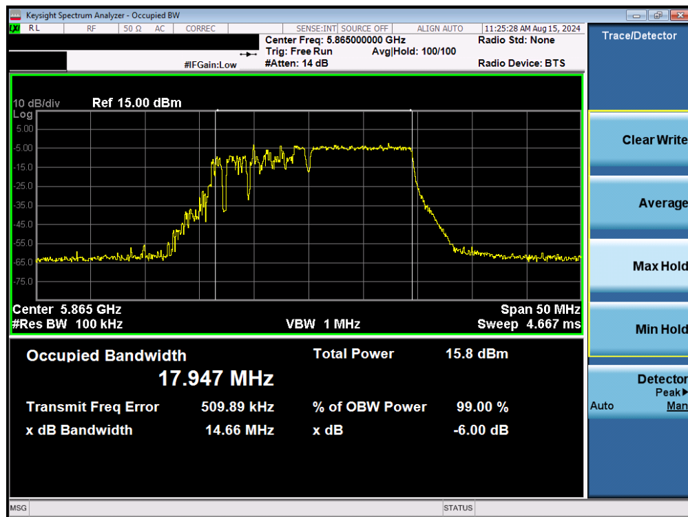
Plot 7-77. 6dB Bandwidth Plot MIMO ANT1 (20MHz BW 802.11be – 106+26 Tones (UNII Band 4) – Ch. 173)
