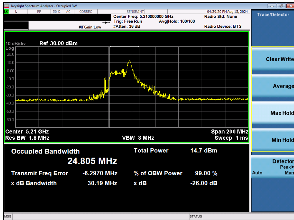
Plot 7-33. 26dB Bandwidth Plot MIMO ANT2 (80MHz BW 802.11be – 26 Tones (UNII Band 1) – Ch. 42)
