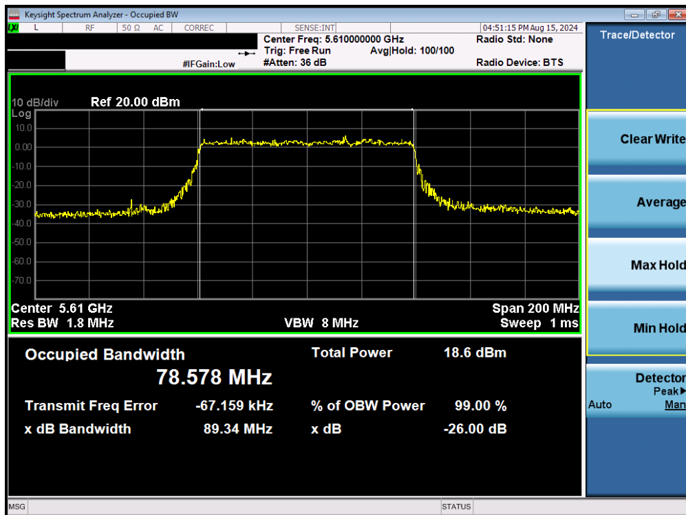
Plot 7-51. 26dB Bandwidth Plot MIMO ANT2 (80MHz BW 802.11be – 996 Tones (UNII Band 2C) – Ch. 122)
