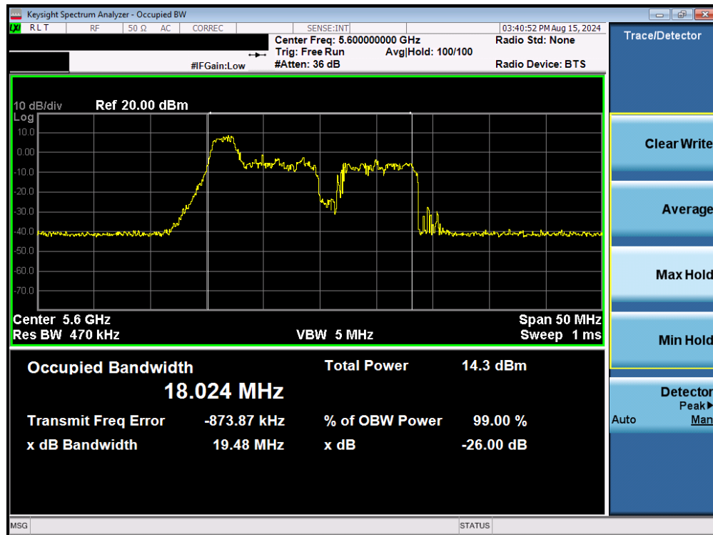
Plot 7-38. 26dB Bandwidth Plot MIMO ANT2 (20MHz BW 802.11be – 26 Tones (UNII Band 2C) – Ch. 120)
