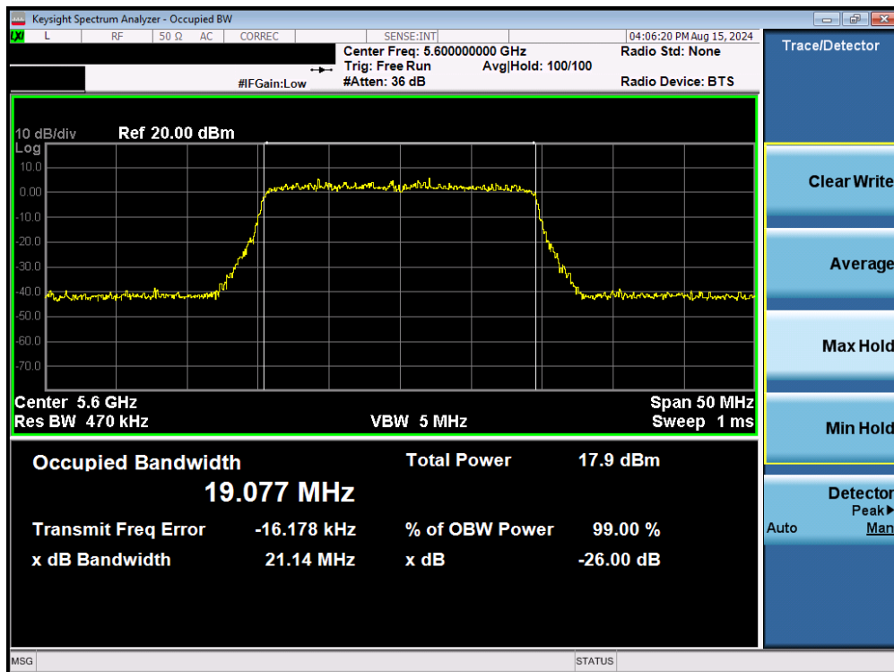
Plot 7-49. 26dB Bandwidth Plot MIMO ANT2 (20MHz BW 802.11be – 242 Tones (UNII Band 2C) – Ch. 120)
