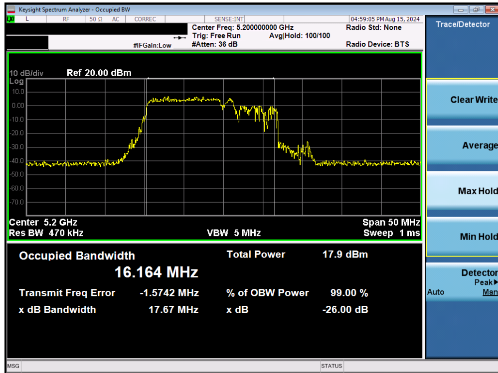
Plot 7-53. 26dB Bandwidth Plot MIMO ANT2 (20MHz BW 802.11be – 106+26T Tones (UNII Band 1) – Ch. 40)
