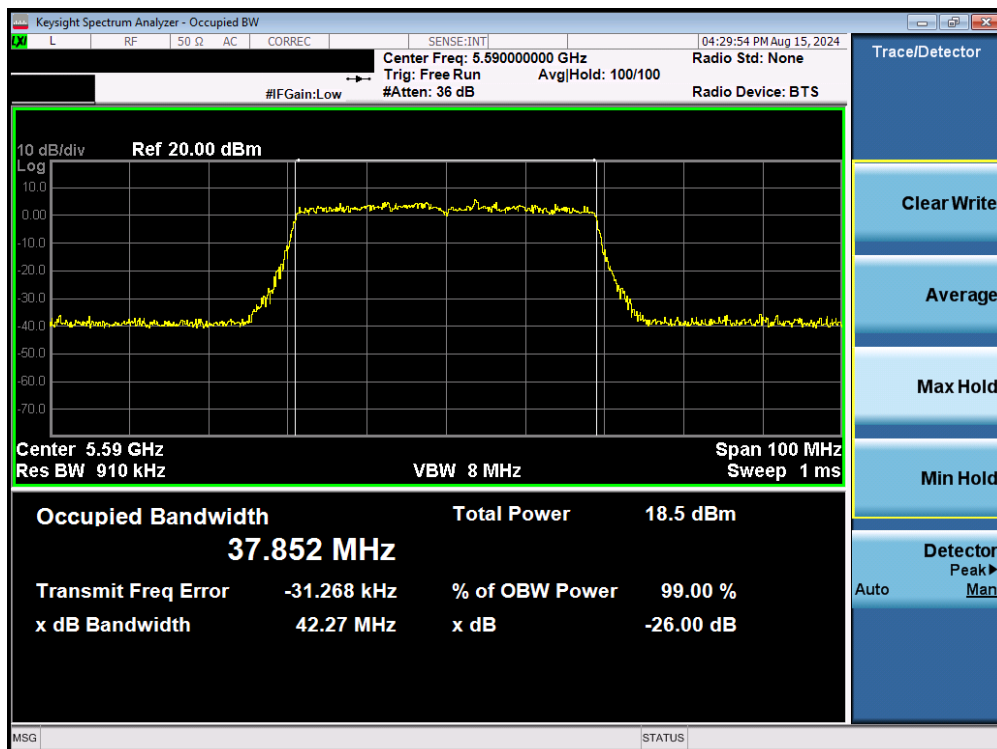
Plot 7-50. 26dB Bandwidth Plot MIMO ANT2 (40MHz BW 802.11be – 484 Tones (UNII Band 2C) – Ch. 118)
