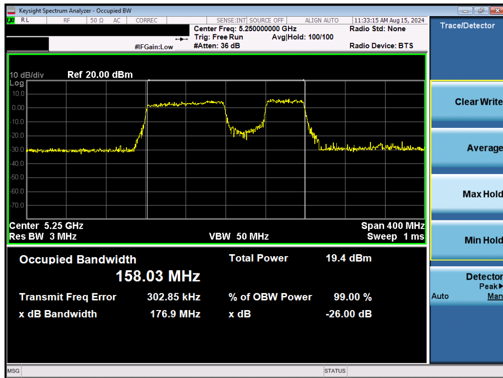
Plot 7-25. 26dB Bandwidth Plot MIMO ANT1 (160MHz BW 802.11be – 996+484 Tones (UNII Band 1/2A) – Ch. 50)
