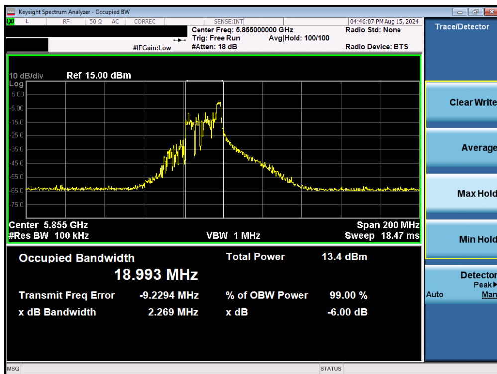
Plot 7-85. 6dB Bandwidth Plot MIMO ANT2 (80MHz BW 802.11be – 26 Tones (UNII Band 3/4) – Ch. 171)
