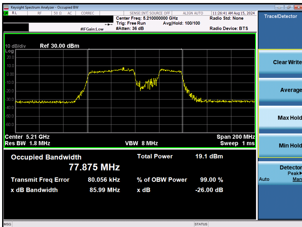
Plot 7-24. 26dB Bandwidth Plot MIMO ANT1 (80MHz BW 802.11be – 484+242 Tones (UNII Band 1) – Ch. 42)
