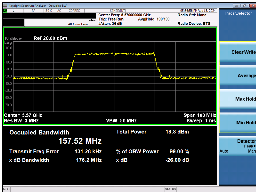
Plot 7-52. 26dB Bandwidth Plot MIMO ANT2 (160MHz BW 802.11be – 2x996 Tones (UNII Band 2C) – Ch. 114)
