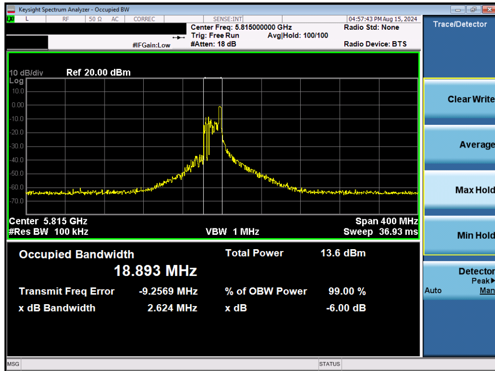
Plot 7-86. 6dB Bandwidth Plot MIMO ANT2 (160MHz BW 802.11be – 26 Tones (UNII Band 3/4) – Ch. 163)
