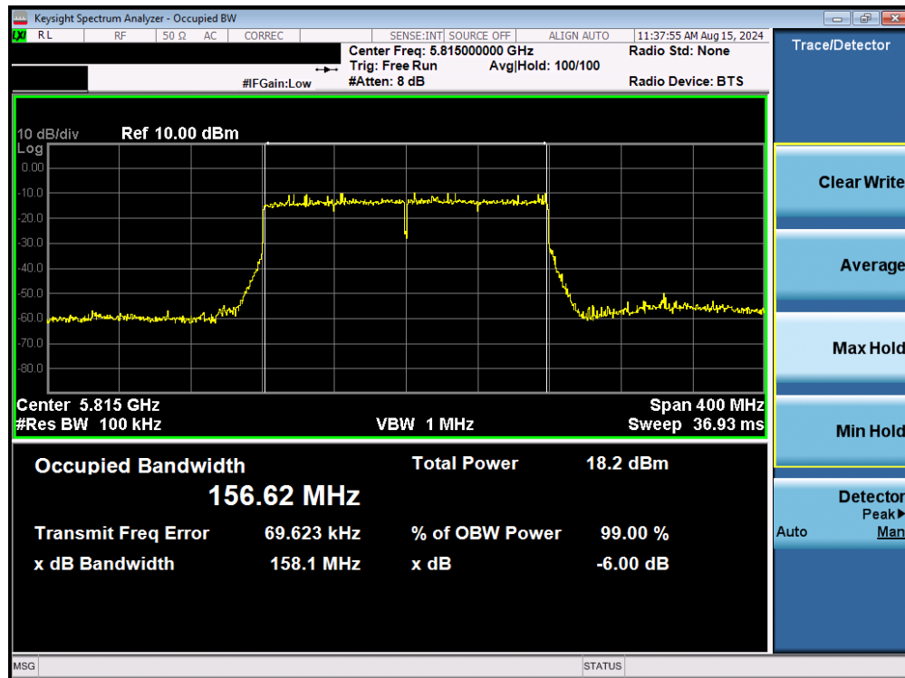
Plot 7-74. 6dB Bandwidth Plot MIMO ANT1 (160MHz BW 802.11be – 996*2 Tones (UNII Band 3/4) – Ch. 163)
