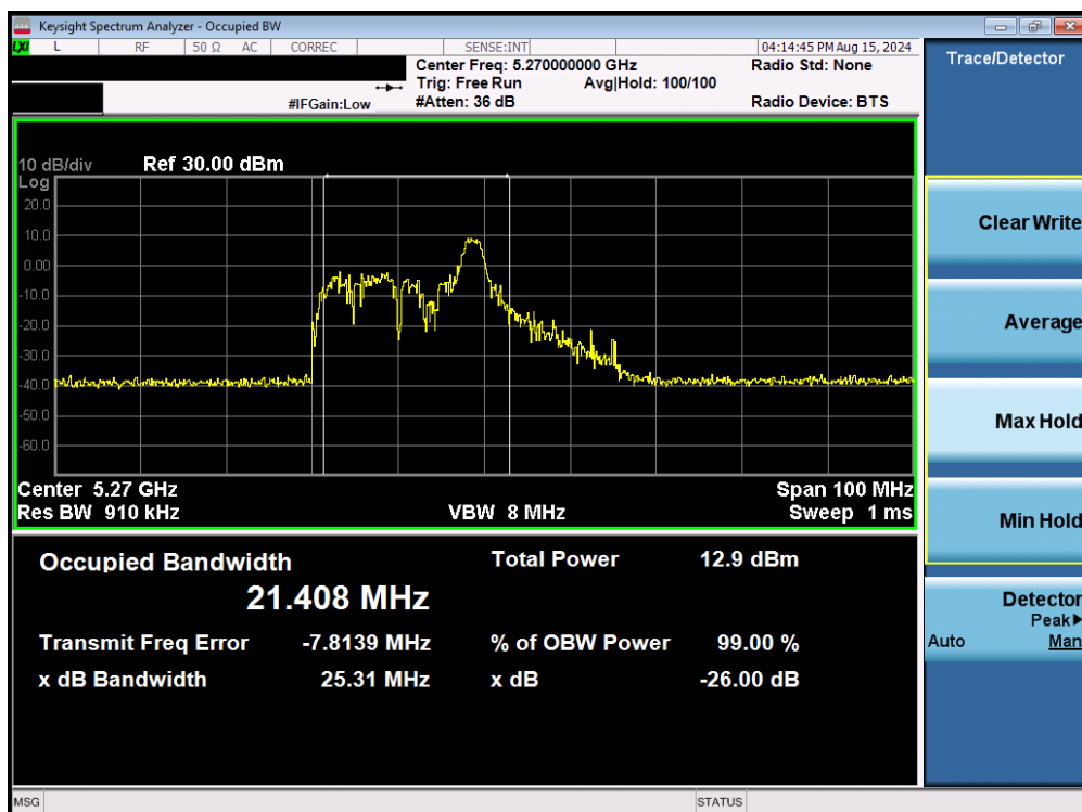
Plot 7-36. 26dB Bandwidth Plot MIMO ANT2 (40MHz BW 802.11be – 26 Tones (UNII Band 2A) – Ch. 54)
