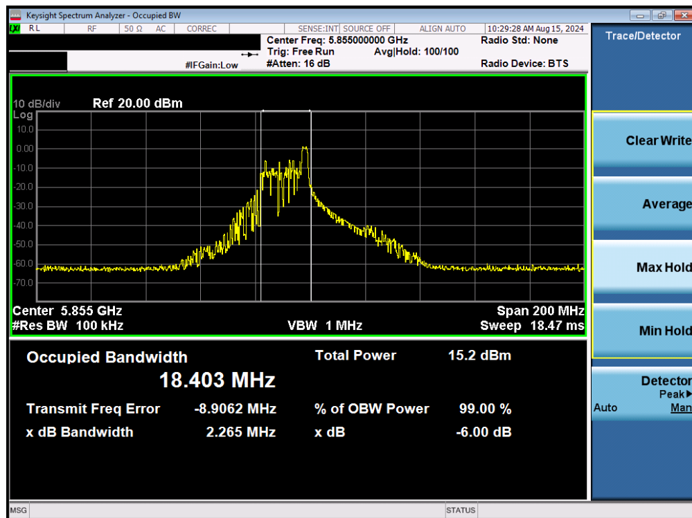
Plot 7-66. 6dB Bandwidth Plot MIMO ANT1 (80MHz BW 802.11be – 26 Tones (UNII Band 3/4) – Ch. 171)
