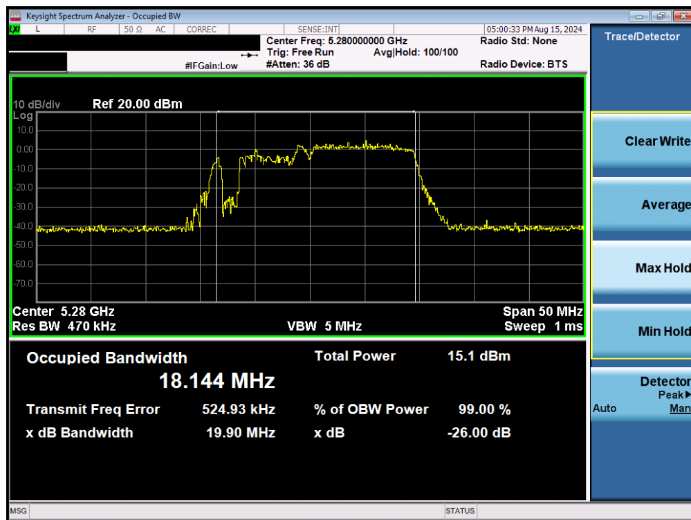
Plot 7-56. 26dB Bandwidth Plot MIMO ANT2 (20MHz BW 802.11be – 106+26 Tones (UNII Band 2A) – Ch. 56)
