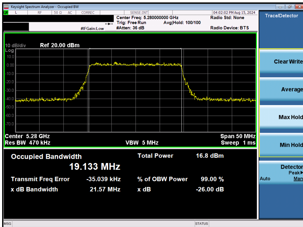
Plot 7-46. 26dB Bandwidth Plot MIMO ANT2 (20MHz BW 802.11be – 242 Tones (UNII Band 2A) – Ch. 56)
