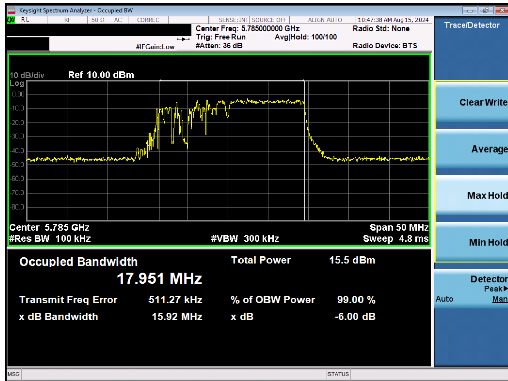
Plot 7-75. 6dB Bandwidth Plot MIMO ANT1 (20MHz BW 802.11be – 106+26 Tones (UNII Band 3) – Ch. 157)
