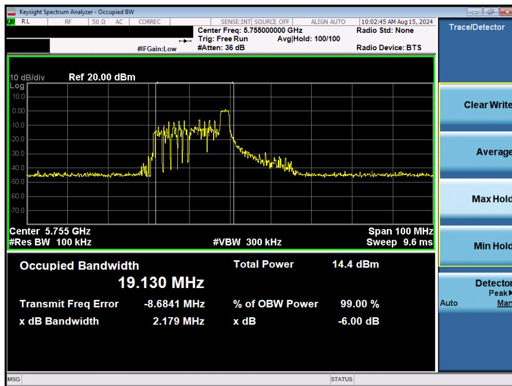
Plot 7-62. 6dB Bandwidth Plot MIMO ANT1 (40MHz BW 802.11be – 26 Tones (UNII Band 3) – Ch. 151)
