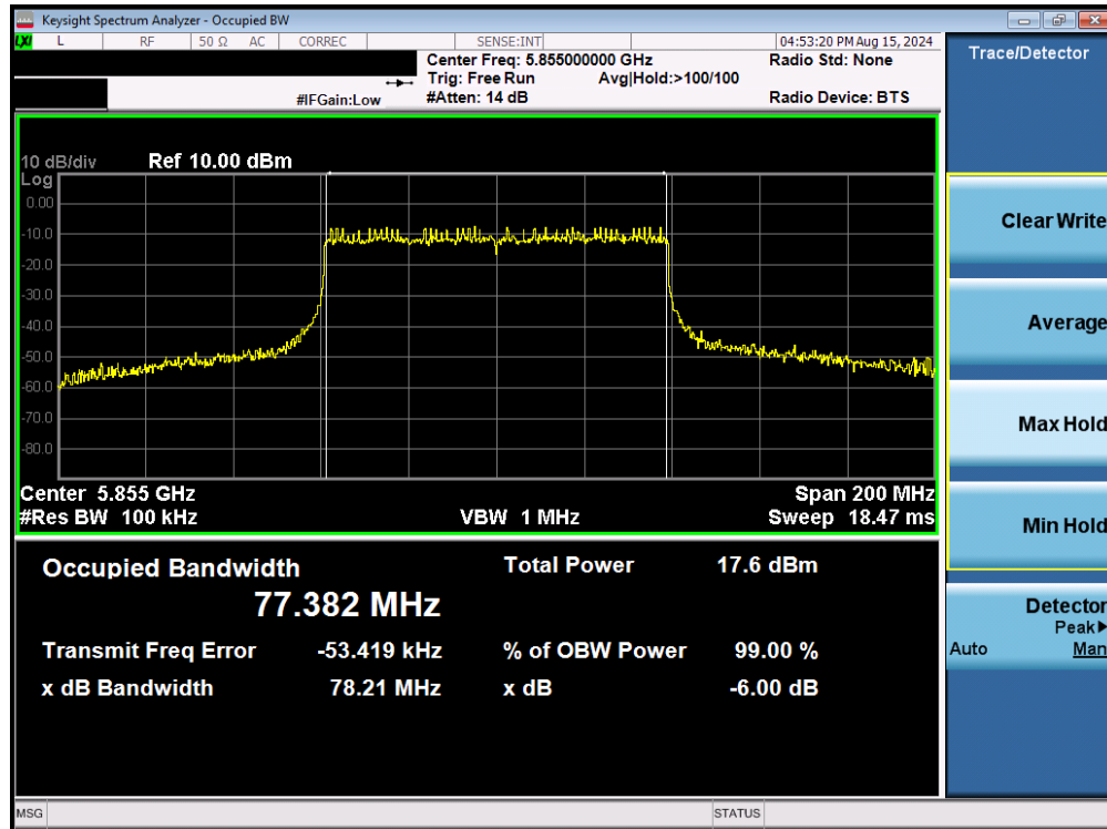
Plot 7-92. 6dB Bandwidth Plot MIMO ANT2 (80MHz BW 802.11be – 996 Tones (UNII Band 3/4) – Ch. 171)
