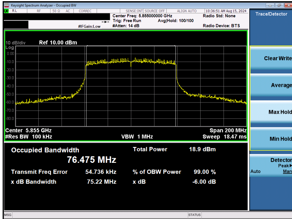
Plot 7-73. 6dB Bandwidth Plot MIMO ANT1 (80MHz BW 802.11be – 996 Tones (UNII Band 3/4) – Ch. 171)
