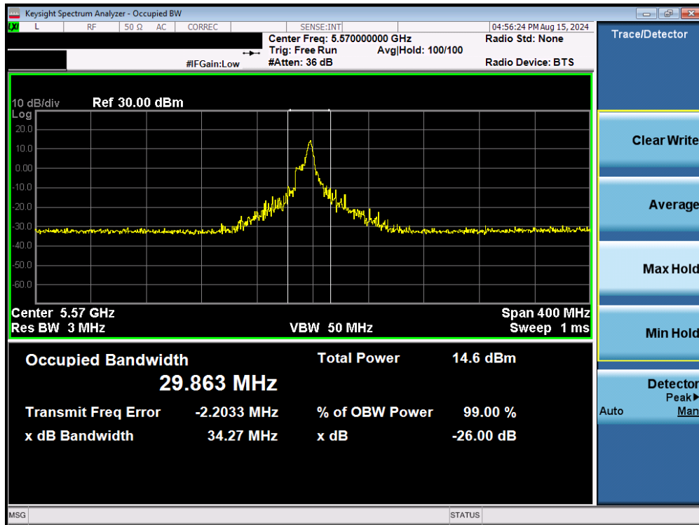
Plot 7-41. 26dB Bandwidth Plot MIMO ANT2 (160MHz BW 802.11be – 26 Tones (UNII Band 2C) – Ch. 114)
