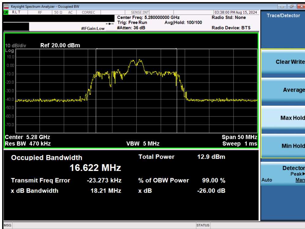
Plot 7-35. 26dB Bandwidth Plot MIMO ANT2 (20MHz BW 802.11be – 26 Tones (UNII Band 2A) – Ch. 56)
