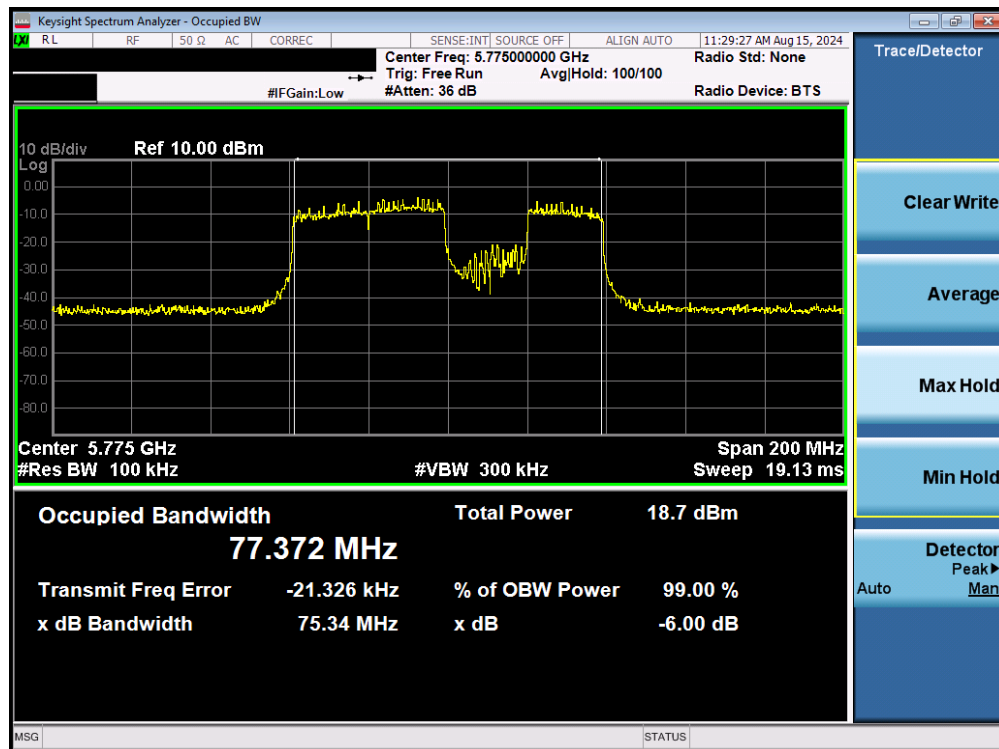
Plot 7-76. 6dB Bandwidth Plot MIMO ANT1 (80MHz BW 802.11be – 484+242 Tones (UNII Band 3) – Ch. 155)
