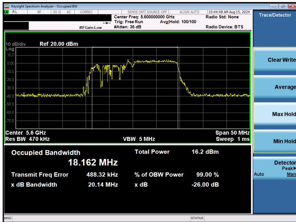
Plot 7-28. 26dB Bandwidth Plot MIMO ANT1 (20MHz BW 802.11be – 106+26 Tones (UNII Band 2C) – Ch. 120)
