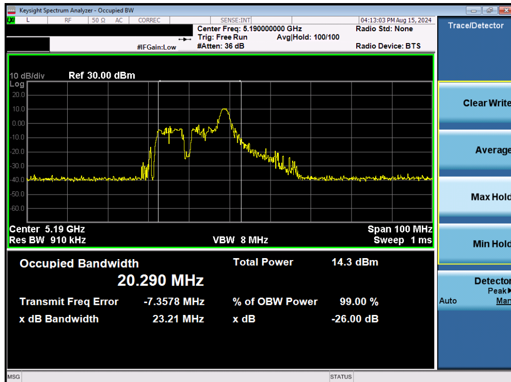
Plot 7-32. 26dB Bandwidth Plot MIMO ANT2 (40MHz BW 802.11be – 26 Tones (UNII Band 1) – Ch. 38)
