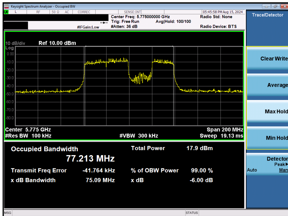
Plot 7-95. 6dB Bandwidth Plot MIMO ANT2 (80MHz BW 802.11be – 484+242 Tones (UNII Band 3) – Ch. 155)
