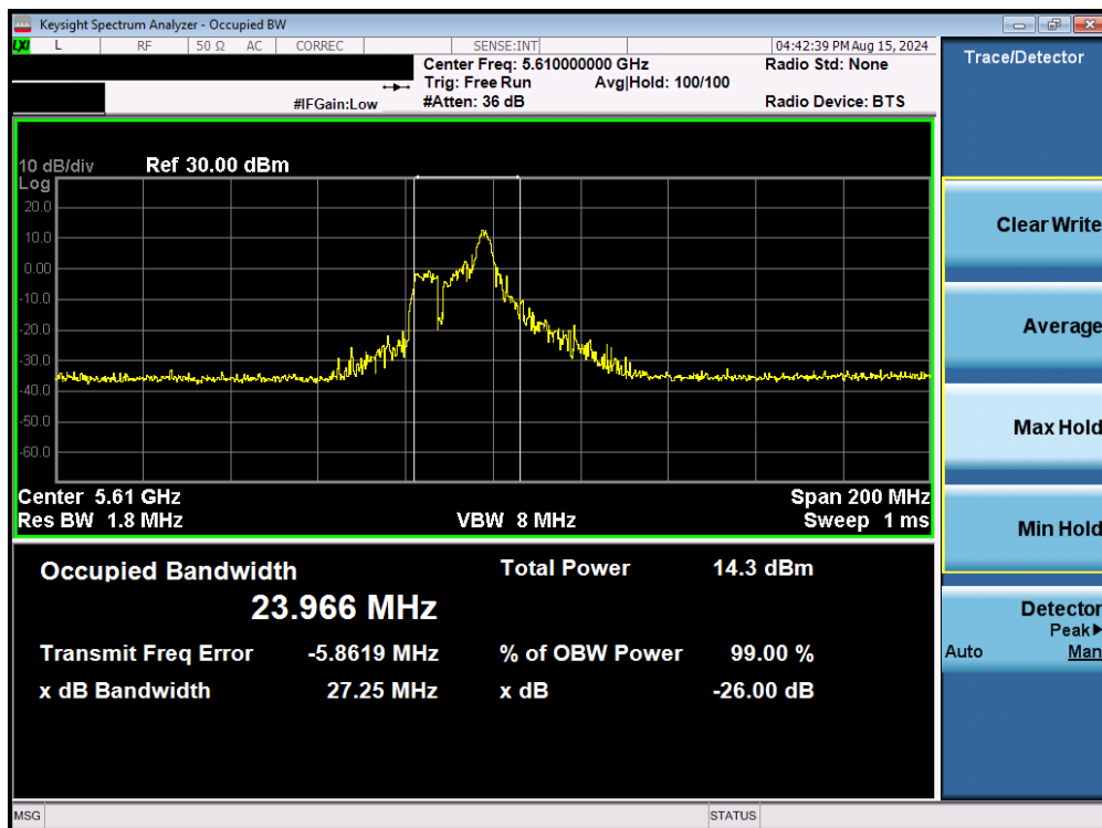
Plot 7-40. 26dB Bandwidth Plot MIMO ANT2 (80MHz BW 802.11be – 26 Tones (UNII Band 2C) – Ch. 122)
