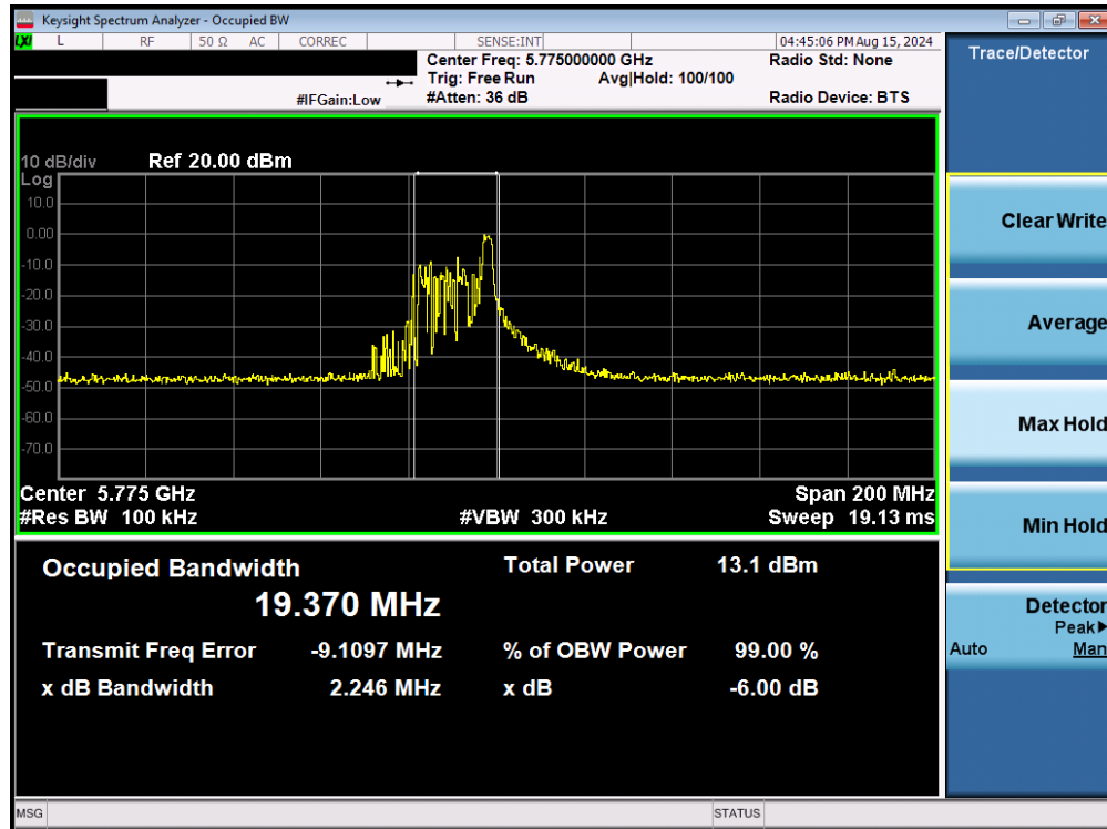
Plot 7-82. 6dB Bandwidth Plot MIMO ANT2 (80MHz BW 802.11be – 26 Tones (UNII Band 3) – Ch. 155)
