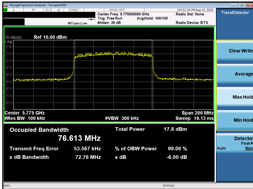
Plot 7-89. 6dB Bandwidth Plot MIMO ANT2 (80MHz BW 802.11be – 996 Tones (UNII Band 3) – Ch. 155)
