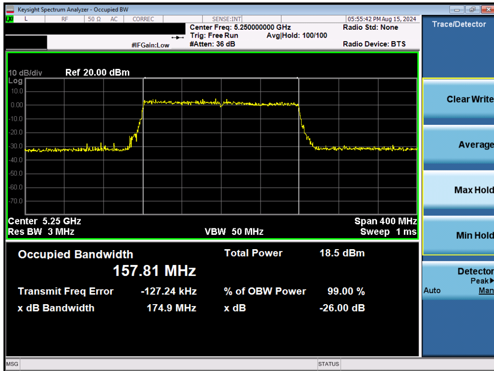
Plot 7-45. 26dB Bandwidth Plot MIMO ANT2 (160MHz BW 802.11be – 2x996 Tones (UNII Band 1/2A) – Ch. 50)
