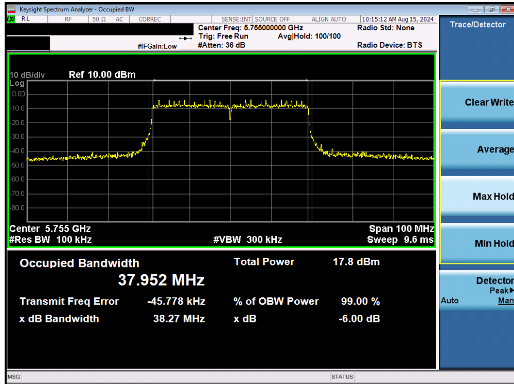
Plot 7-69. 6dB Bandwidth Plot MIMO ANT1 (40MHz BW 802.11be – 484 Tones (UNII Band 3) – Ch. 151)
