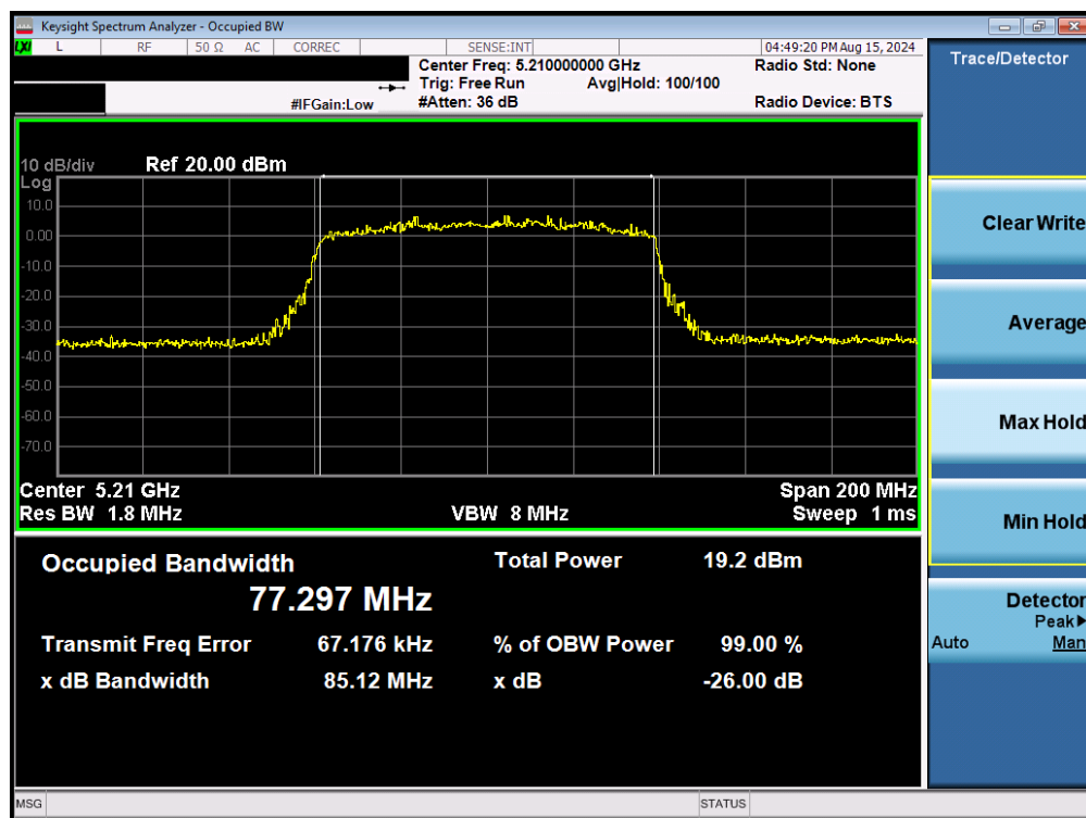
Plot 7-44. 26dB Bandwidth Plot MIMO ANT2 (80MHz BW 802.11be – 996 Tones (UNII Band 1) – Ch. 42)
