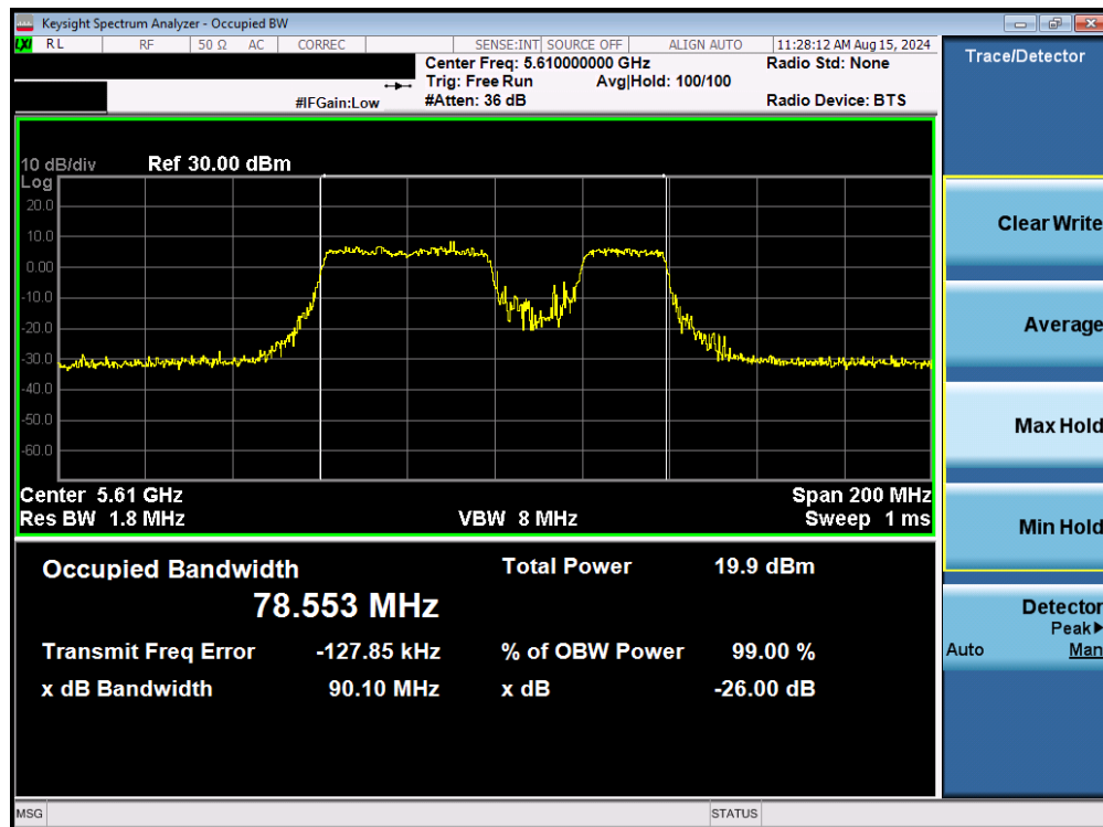
Plot 7-29. 26dB Bandwidth Plot MIMO ANT1 (80MHz BW 802.11be – 484+242 Tones (UNII Band 2C) – Ch. 122)
