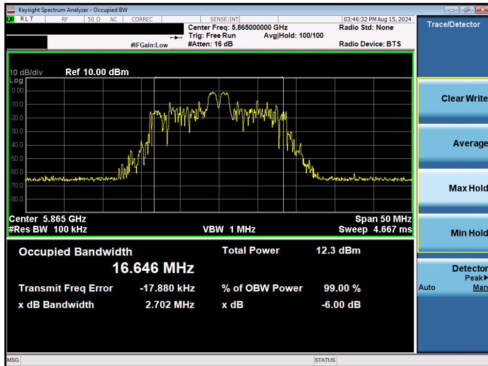
Plot 7-83. 6dB Bandwidth Plot MIMO ANT2 (20MHz BW 802.11be – 26 Tones (UNII Band 4) – Ch. 173)
