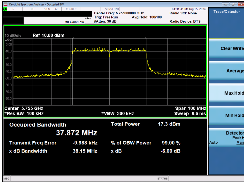
Plot 7-88. 6dB Bandwidth Plot MIMO ANT2 (40MHz BW 802.11be – 484 Tones (UNII Band 3) – Ch. 151)
