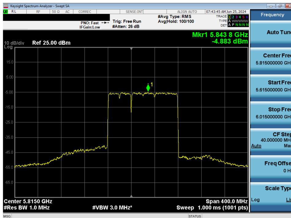
Plot 7-196. Power Spectral Density Plot MIMO ANT2 (160MHz BW 802.11be – 996+484 Tones (UNII Band 3/4) – Ch. 163)
