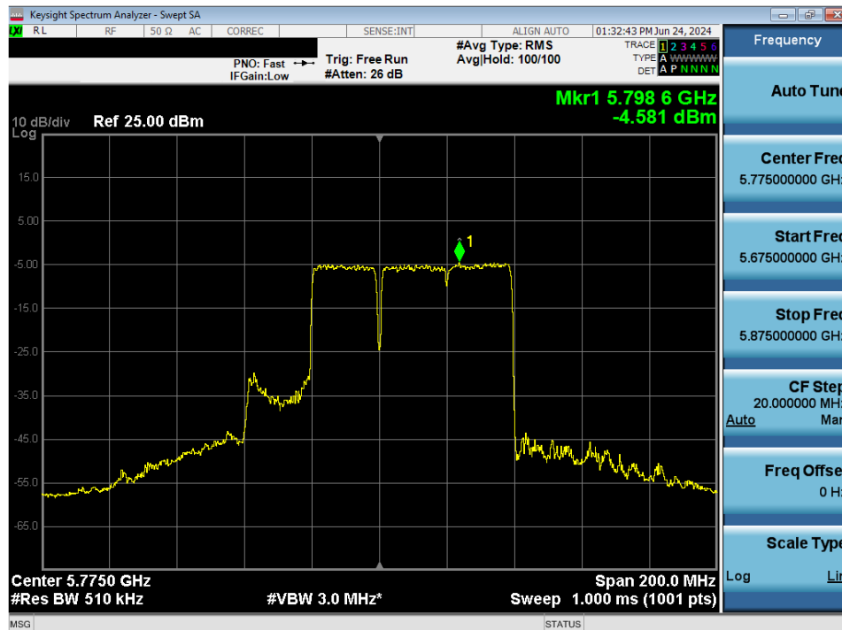
Plot 7-193. Power Spectral Density Plot MIMO ANT2 (80MHz BW 802.11be – 484+242Tones (UNII Band 3) – Ch. 155)
