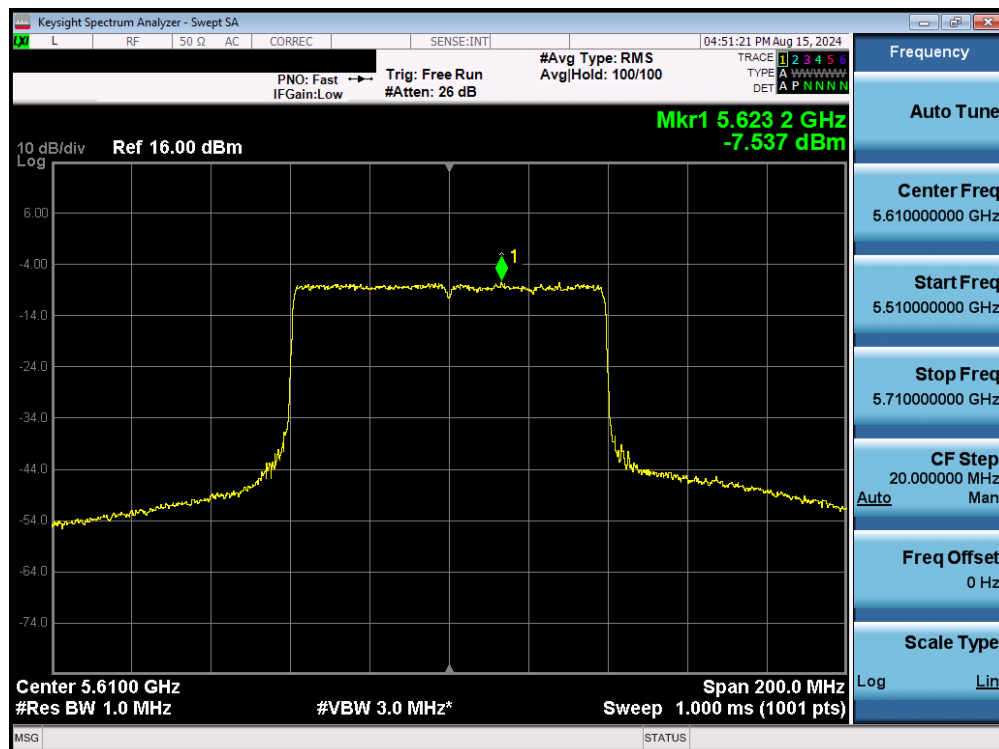
Plot 7-175. Power Spectral Density Plot MIMO ANT2 (80MHz BW 802.11be – 996 Tones (UNII Band 2C) – Ch. 122)
