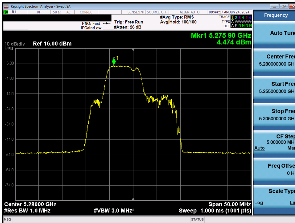
Plot 7-138. Power Spectral Density Plot MIMO ANT1 (20MHz BW 802.11be – 52+26 Tones (UNII Band 2A) – Ch. 56)
