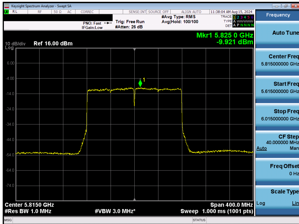
Plot 7-134. Power Spectral Density Plot MIMO ANT1 (160MHz BW 802.11be – 996*2 Tones (UNII Band 3/4) – Ch. 163)
