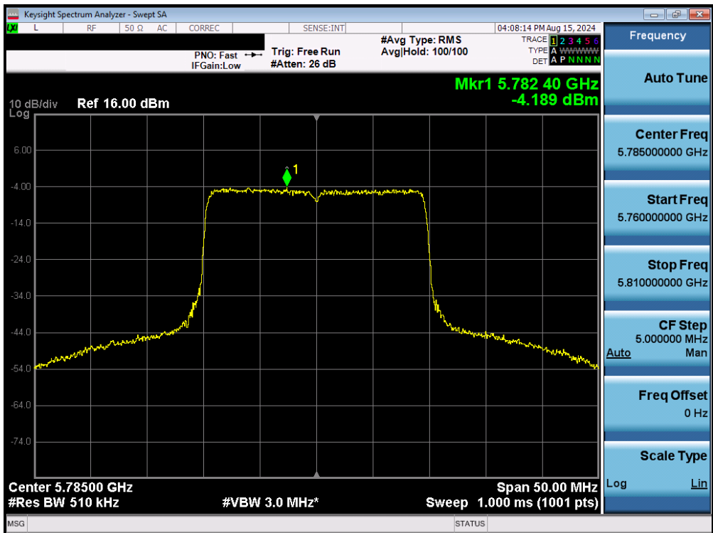
Plot 7-177. Power Spectral Density Plot MIMO ANT2 (20MHz BW 802.11be – 242 Tones (UNII Band 3) – Ch. 157)
