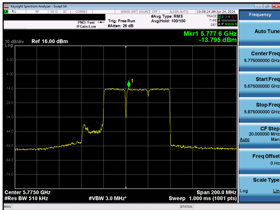
Plot 7-144. Power Spectral Density Plot MIMO ANT1 (80MHz BW 802.11be – 484+242Tones (UNII Band 3) – Ch. 155)
