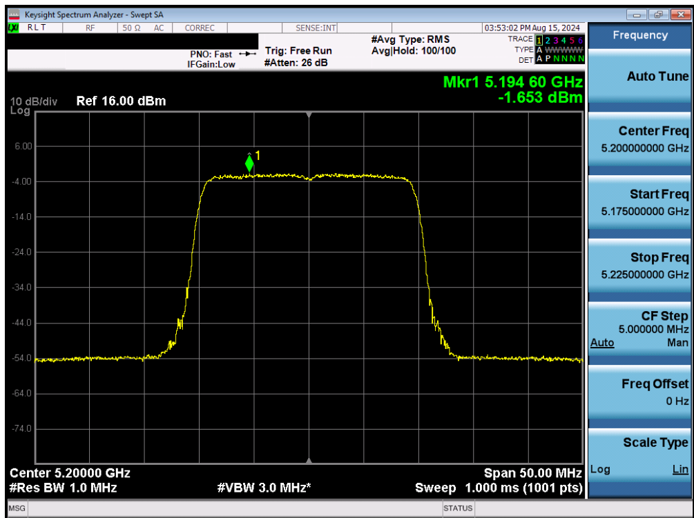
Plot 7-166. Power Spectral Density Plot MIMO ANT2 (20MHz BW 802.11be – 242 Tones (UNII Band 1) – Ch. 40)
