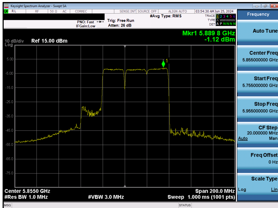
Plot 7-146. Power Spectral Density Plot MIMO ANT1 (80MHz BW 802.11be – 484+242Tones (UNII Band 3/4) – Ch. 171)
