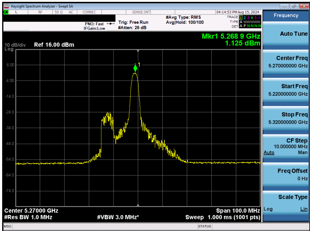
Plot 7-153. Power Spectral Density Plot MIMO ANT2 (40MHz BW 802.11be – 26 Tones (UNII Band 2A) – Ch. 54)
