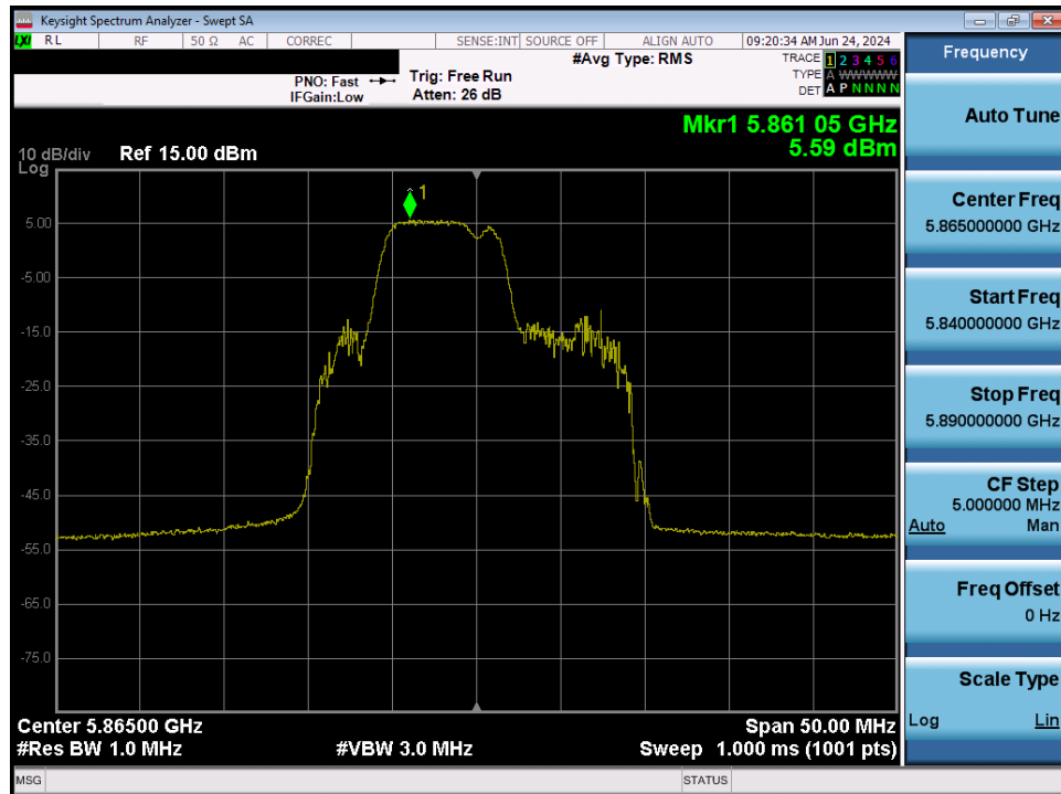
Plot 7-145. Power Spectral Density Plot MIMO ANT1 (20MHz BW 802.11be – 52+26 Tones (UNII Band 4) – Ch. 173)
