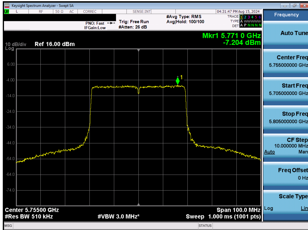
Plot 7-178. Power Spectral Density Plot MIMO ANT2 (40MHz BW 802.11be – 484 Tones (UNII Band 3) – Ch. 151)
