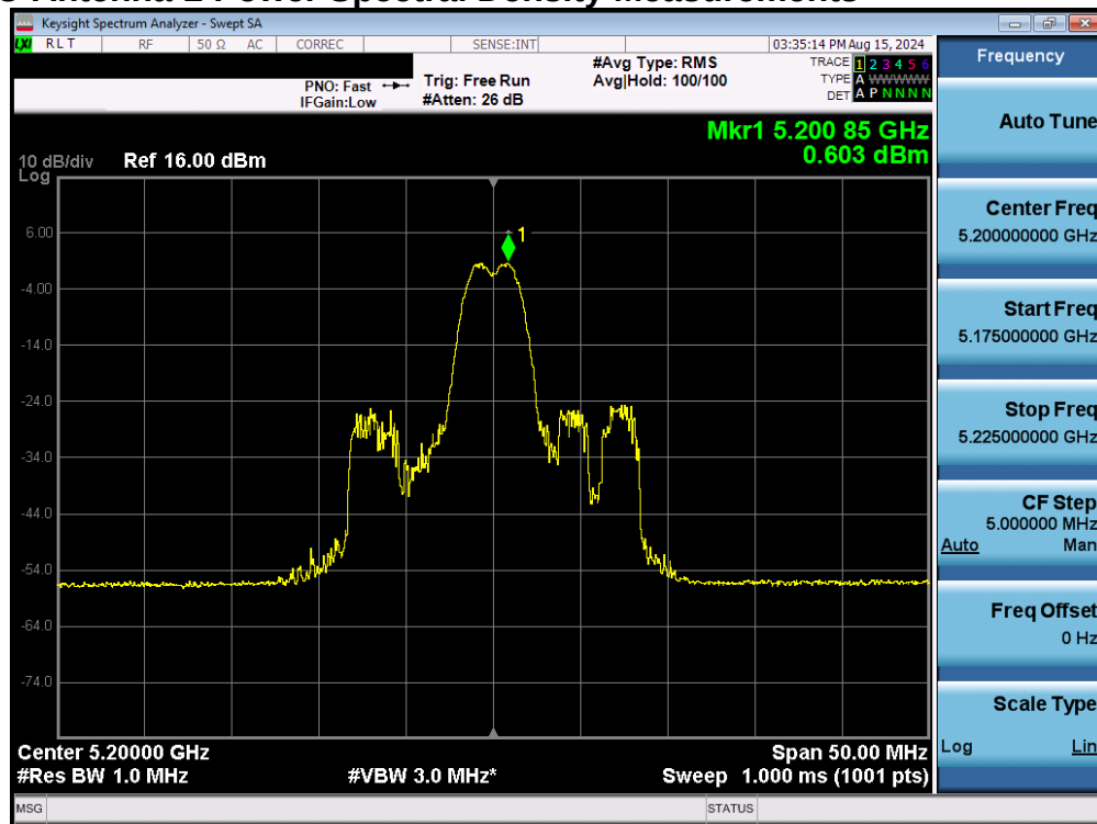
Plot 7-148. Power Spectral Density Plot MIMO ANT2 (20MHz BW 802.11be – 26 Tones (UNII Band 1) – Ch. 40)
