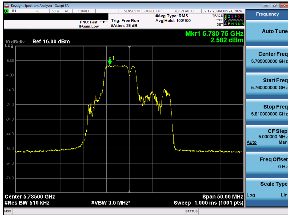
Plot 7-143. Power Spectral Density Plot MIMO ANT1 (20MHz BW 802.11be – 52+26 Tones (UNII Band 3) – Ch. 157)
