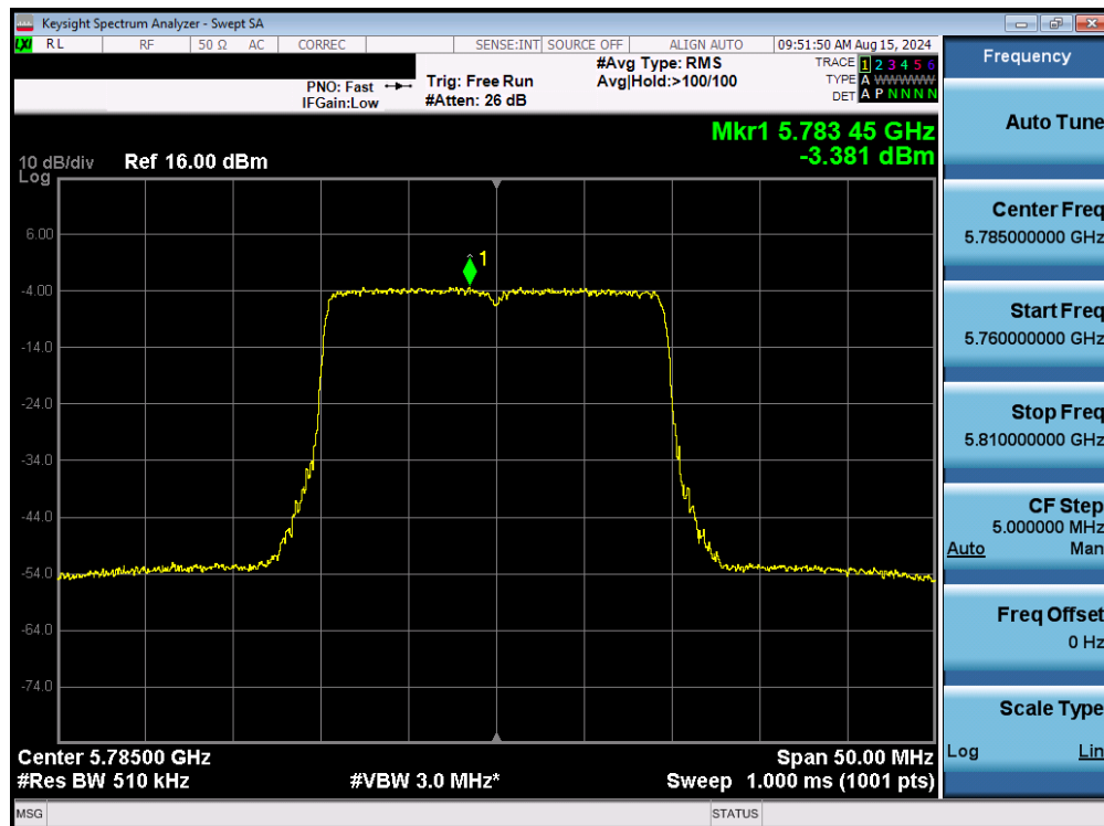
Plot 7-128. Power Spectral Density Plot MIMO ANT1 (20MHz BW 802.11be – 242 Tones (UNII Band 3) – Ch. 157)
