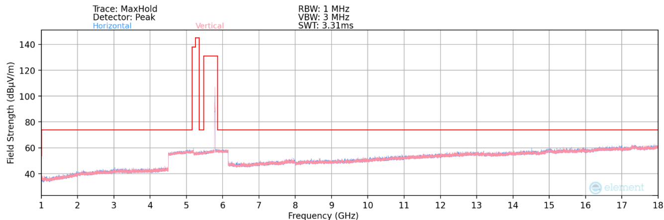
Plot 7-200. Radiated Spurious Plot above 1GHz MIMO (802.11be – UNII 3 Ch. 157)
