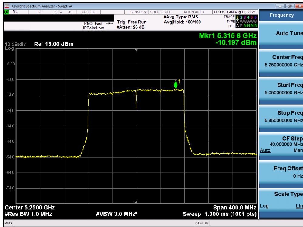
Plot 7-120. Power Spectral Density Plot MIMO ANT1 (160MHz BW 802.11be – 2x996 Tones (UNII Band 1/2A) – Ch. 50)
