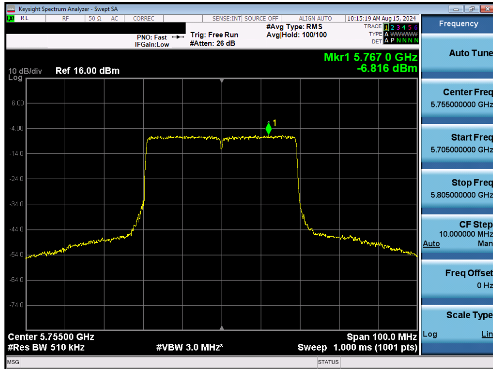
Plot 7-129. Power Spectral Density Plot MIMO ANT1 (40MHz BW 802.11be – 484 Tones (UNII Band 3) – Ch. 151)
