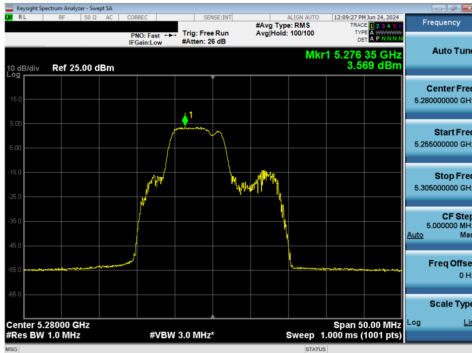
Plot 7-187. Power Spectral Density Plot MIMO ANT2 (20MHz BW 802.11be – 52+26 Tones (UNII Band 2A) – Ch. 56)
