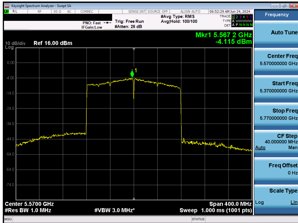
Plot 7-127. Power Spectral Density Plot MIMO ANT1 (160MHz BW 802.11be – 2x996 Tones (UNII Band 2C) – Ch. 114)
