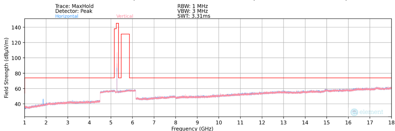
Plot 7-197. Radiated Spurious Plot above 1GHz MIMO (802.11be – UNII 1 Ch. 40)
