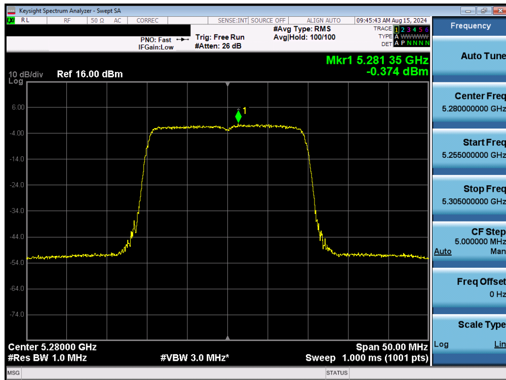
Plot 7-121. Power Spectral Density Plot MIMO ANT1 (20MHz BW 802.11be – 242 Tones (UNII Band 2A) – Ch. 56)
