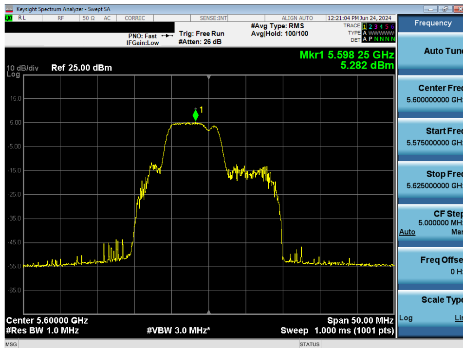
Plot 7-189. Power Spectral Density Plot MIMO ANT2 (20MHz BW 802.11be – 52+26 Tones (UNII Band 2C) – Ch. 120)
