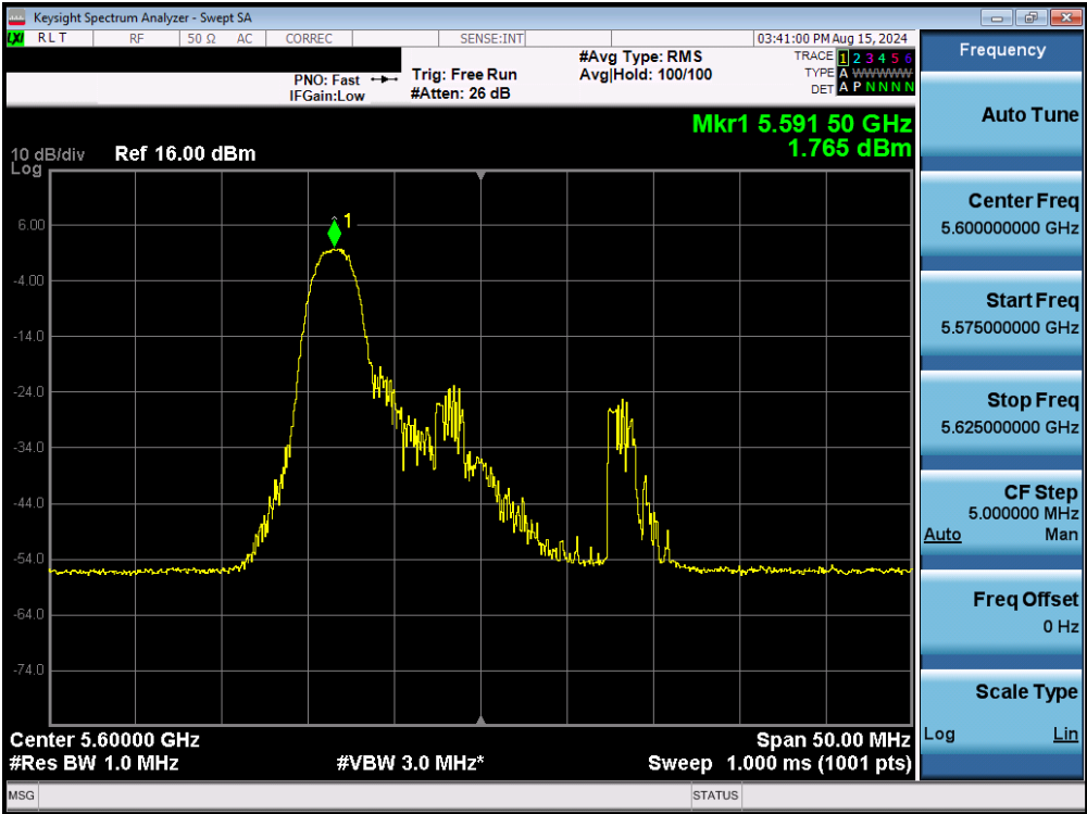
Plot 7-155. Power Spectral Density Plot MIMO ANT2 (20MHz BW 802.11be – 26 Tones (UNII Band 2C) – Ch. 120)
