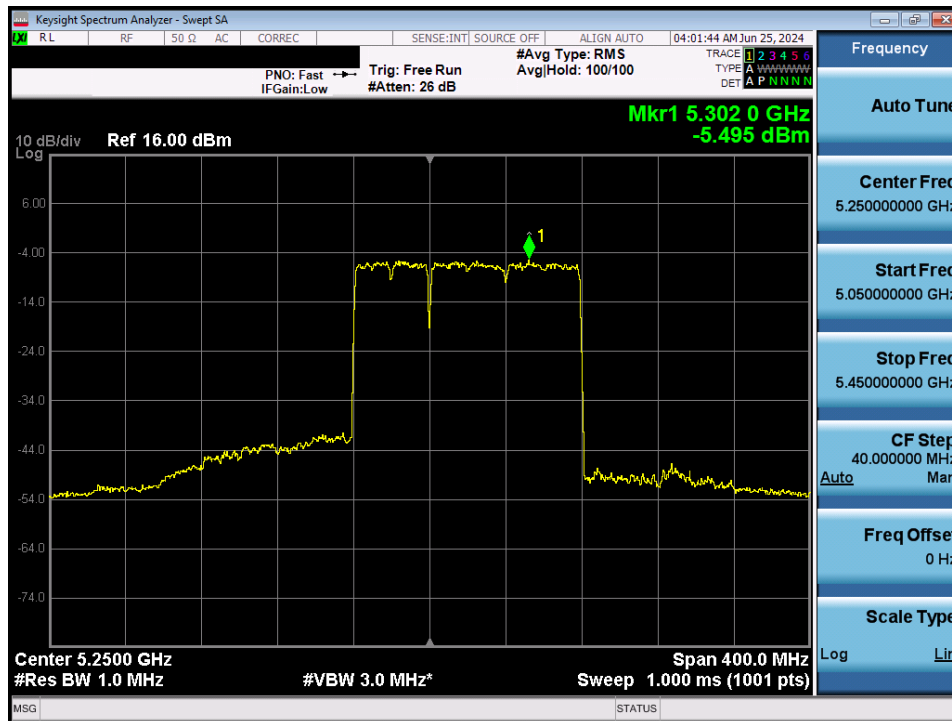
Plot 7-137. Power Spectral Density Plot MIMO ANT1(160MHz BW 802.11be – 996+484 Tones (UNII Band 1/2A) – Ch. 50)
