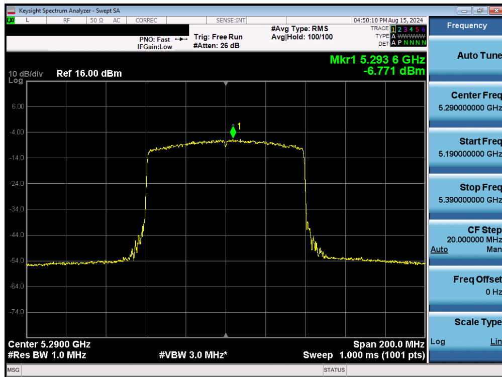
Plot 7-172. Power Spectral Density Plot MIMO ANT2 (80MHz BW 802.11be – 996 Tones (UNII Band 2A) – Ch. 58)
