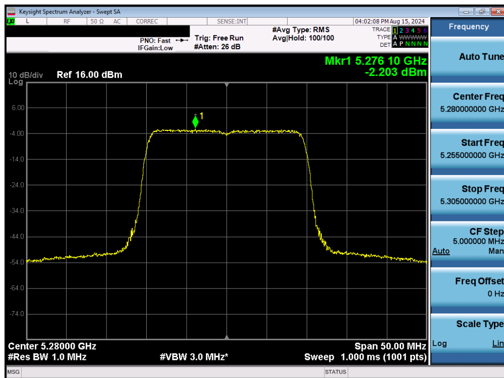
Plot 7-170. Power Spectral Density Plot MIMO ANT2 (20MHz BW 802.11be – 242 Tones (UNII Band 2A) – Ch. 56)
