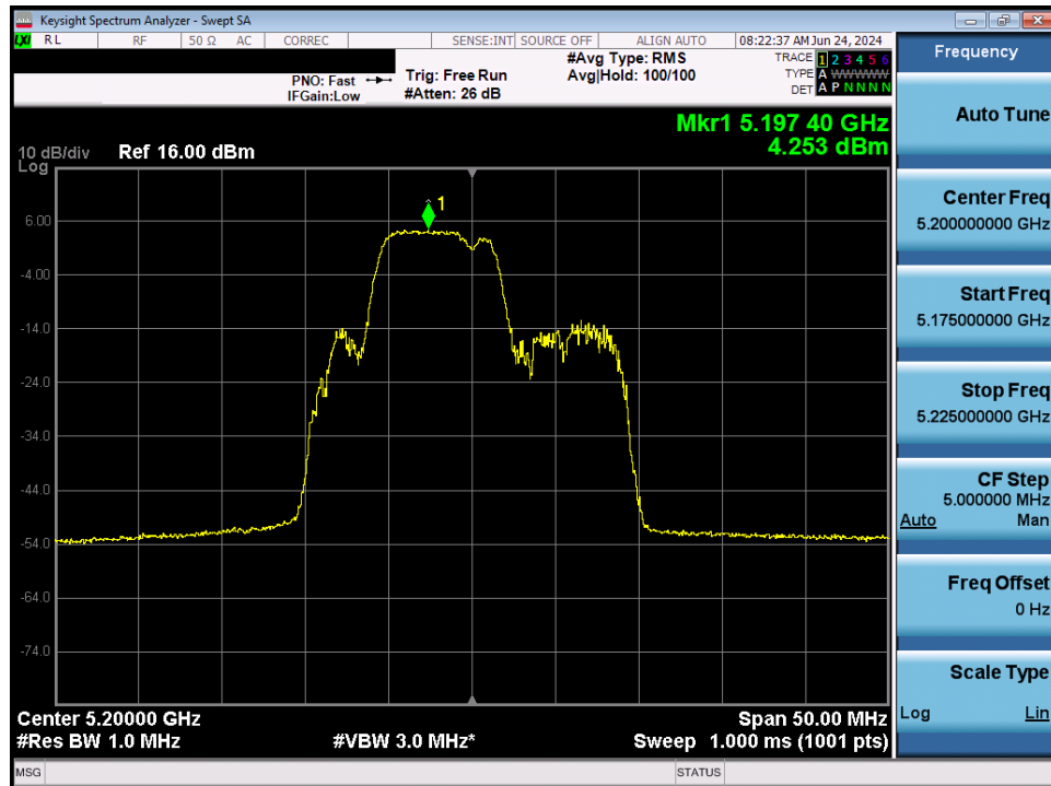
Plot 7-135. Power Spectral Density Plot MIMO ANT1 (20MHz BW 802.11be – 52+26 Tones (UNII Band 1) – Ch. 40)
