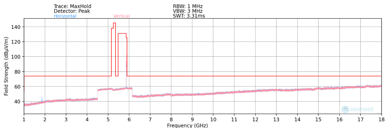
Plot 7-201. Radiated Spurious Plot above 1GHz MIMO (802.11be – UNII 4 Ch. 173)
