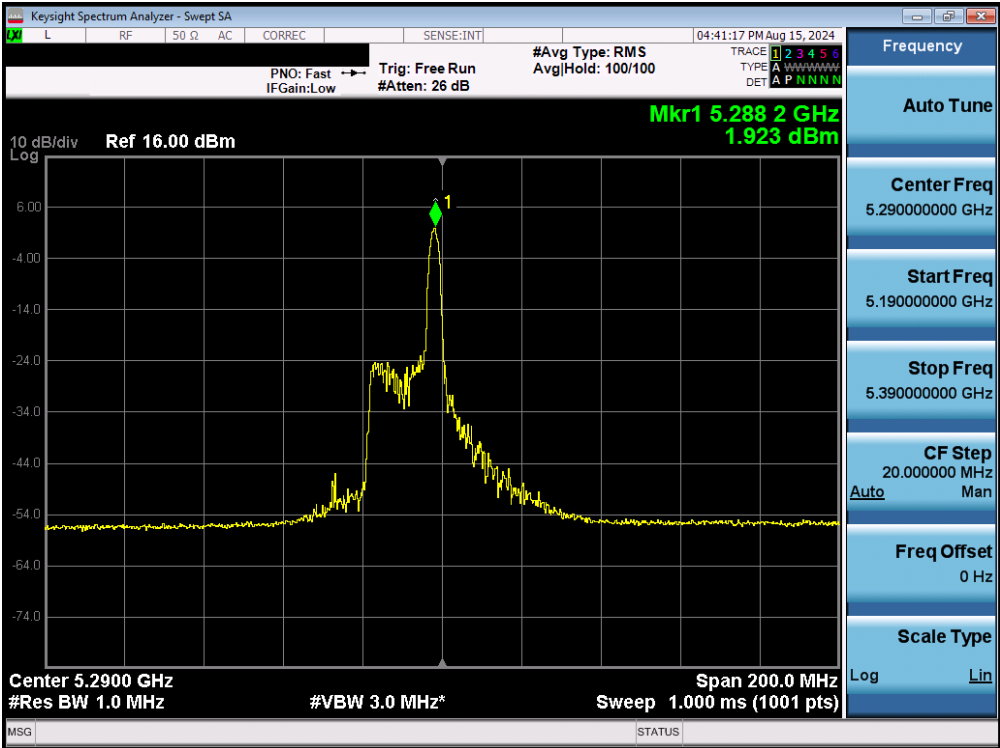
Plot 7-154. Power Spectral Density Plot MIMO ANT2 (80MHz BW 802.11be – 26 Tones (UNII Band 2A) – Ch. 58)
