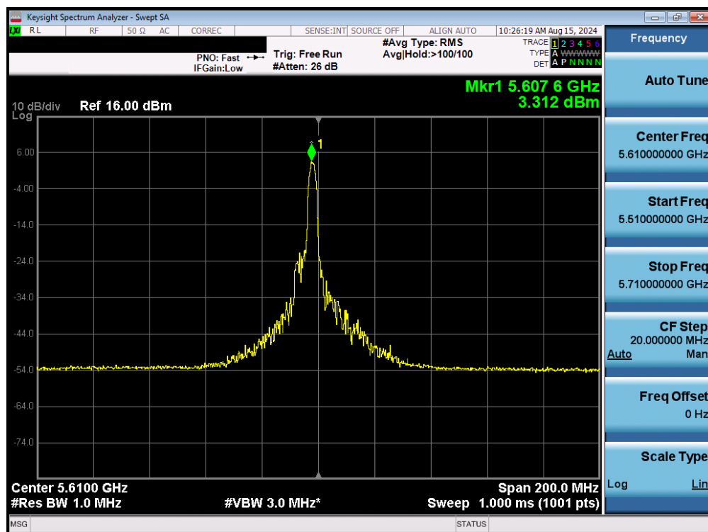
Plot 7-108. Power Spectral Density Plot MIMO ANT1 (80MHz BW 802.11be – 26 Tones (UNII Band 2C) – Ch. 122)
