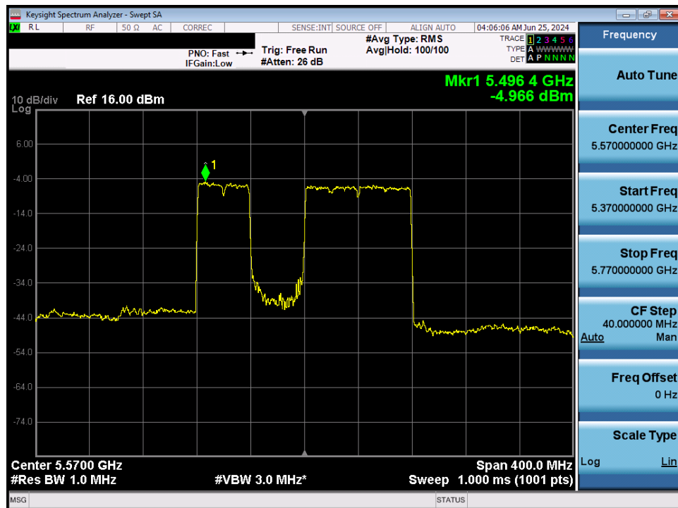
Plot 7-142. Power Spectral Density Plot MIMO ANT1 (160MHz BW 802.11be – 996+484 Tones (UNII Band 2C) – Ch. 114)
