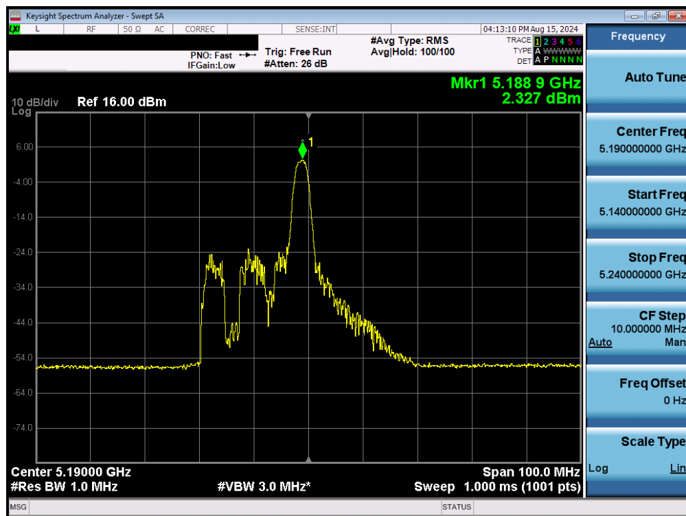
Plot 7-149. Power Spectral Density Plot MIMO ANT2 (40MHz BW 802.11be – 26 Tones (UNII Band 1) – Ch. 38)
