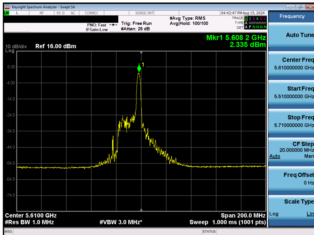
Plot 7-157. Power Spectral Density Plot MIMO ANT2 (80MHz BW 802.11be – 26 Tones (UNII Band 2C) – Ch. 122)
