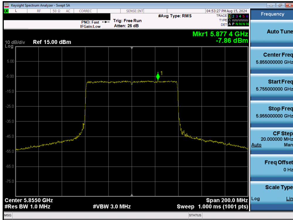
Plot 7-182. Power Spectral Density Plot MIMO ANT2 (80MHz BW 802.11be – 996 Tones (UNII Band 3/4) – Ch. 171)
