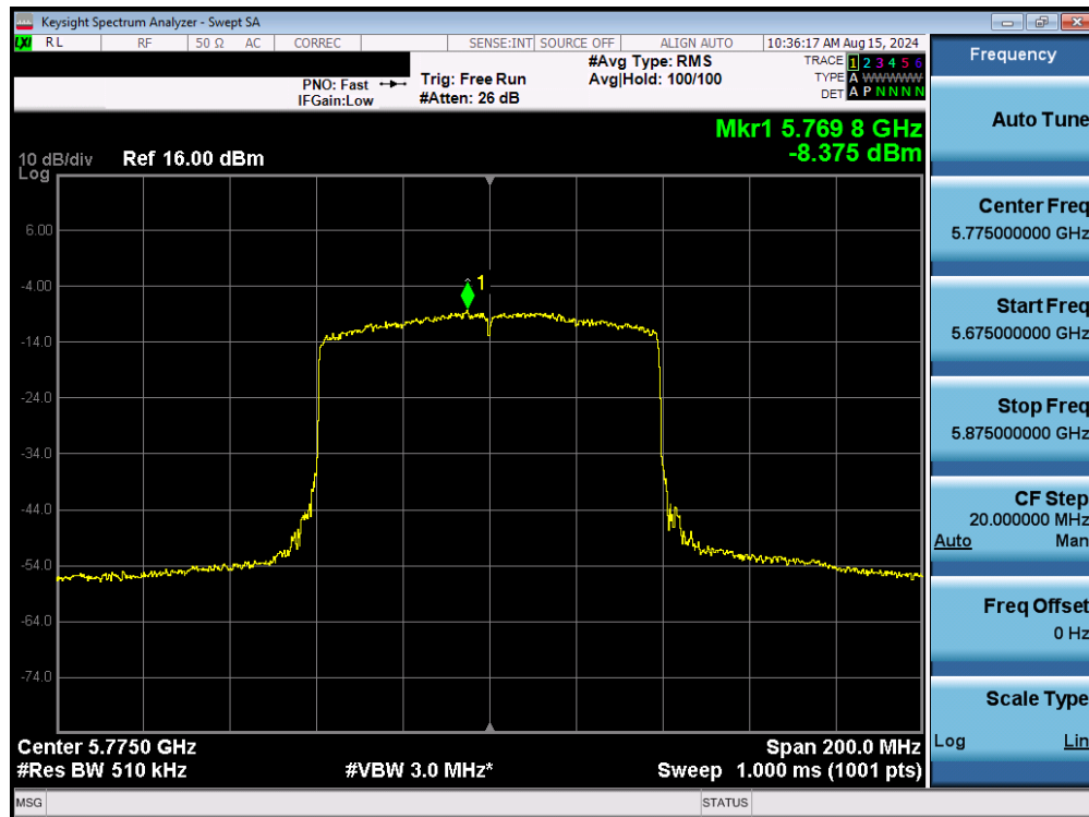
Plot 7-130. Power Spectral Density Plot MIMO ANT1 (80MHz BW 802.11be – 996 Tones (UNII Band 3) – Ch. 155)
