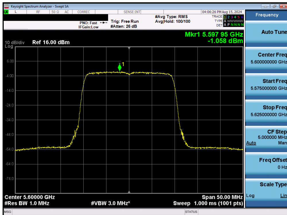
Plot 7-173. Power Spectral Density Plot MIMO ANT2 (20MHz BW 802.11be – 242 Tones (UNII Band 2C) – Ch. 120)
