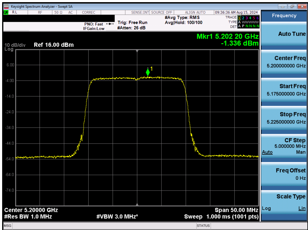
Plot 7-117. Power Spectral Density Plot MIMO ANT1 (20MHz BW 802.11be – 242 Tones (UNII Band 1) – Ch. 40)
