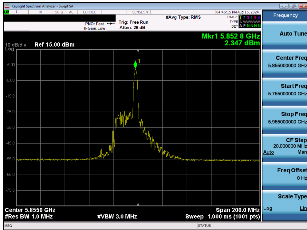
Plot 7-164. Power Spectral Density Plot MIMO ANT2 (80MHz BW 802.11be – 26 Tones (UNII Band 3/4) – Ch. 171)
