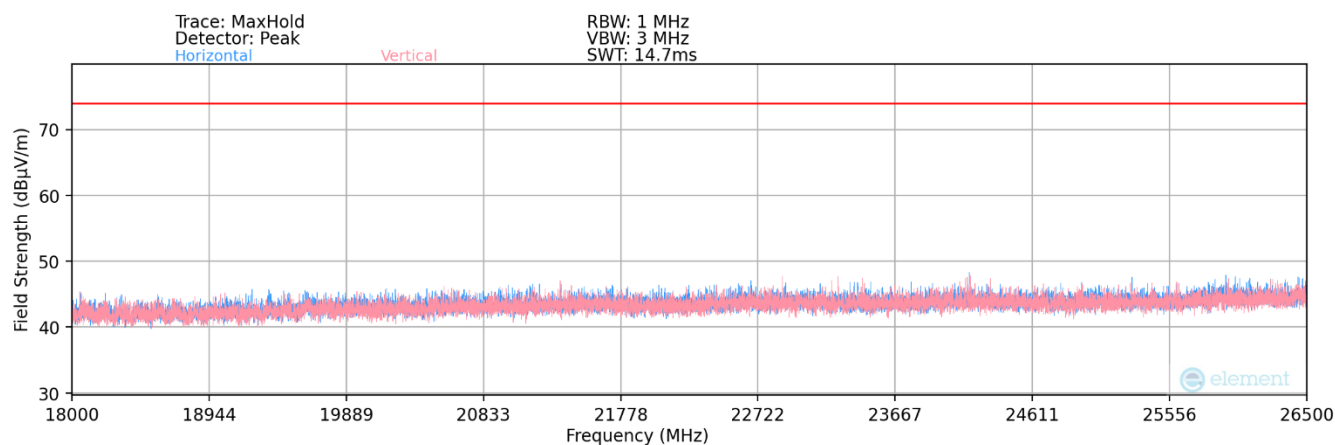
Plot 7-202. Radiated Spurious Plot 18GHz - 26.5GHz (802.11be)
