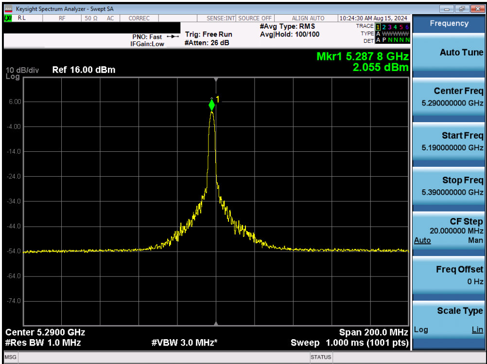
Plot 7-105. Power Spectral Density Plot MIMO ANT1 (80MHz BW 802.11be – 26 Tones (UNII Band 2A) – Ch. 58)
