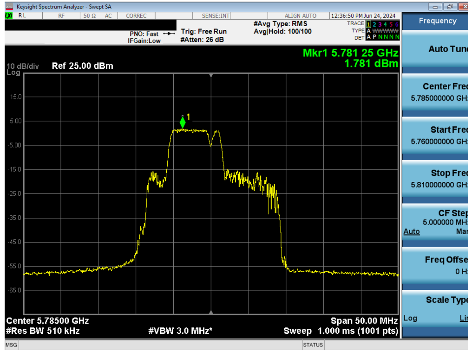
Plot 7-192. Power Spectral Density Plot MIMO ANT2 (20MHz BW 802.11be – 52+26 Tones (UNII Band 3) – Ch. 157)
