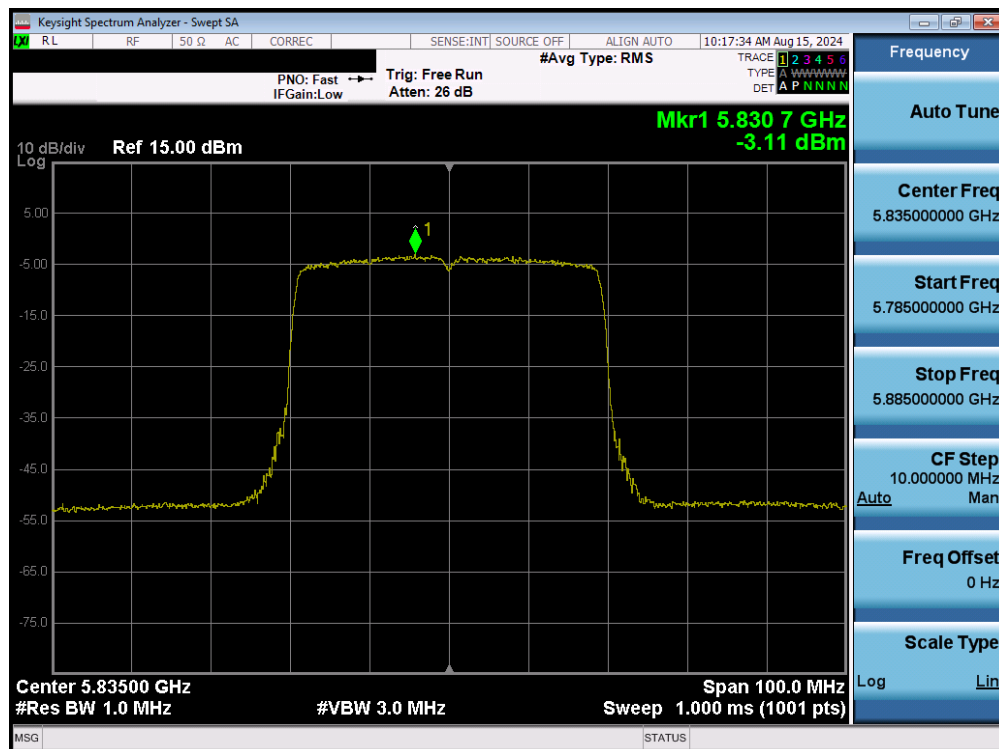
Plot 7-132. Power Spectral Density Plot MIMO ANT1 (40MHz BW 802.11be – 484 Tones (UNII Band 3/4) – Ch. 167)
