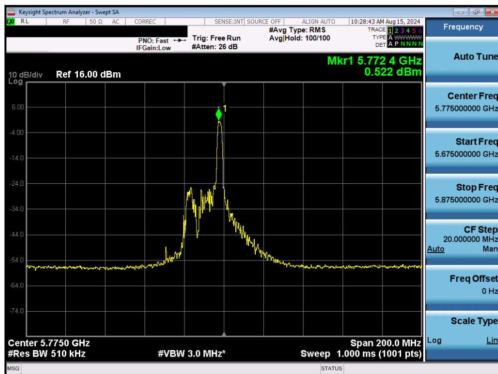
Plot 7-112. Power Spectral Density Plot MIMO ANT1 (80MHz BW 802.11be – 26 Tones (UNII Band 3) – Ch. 155)
