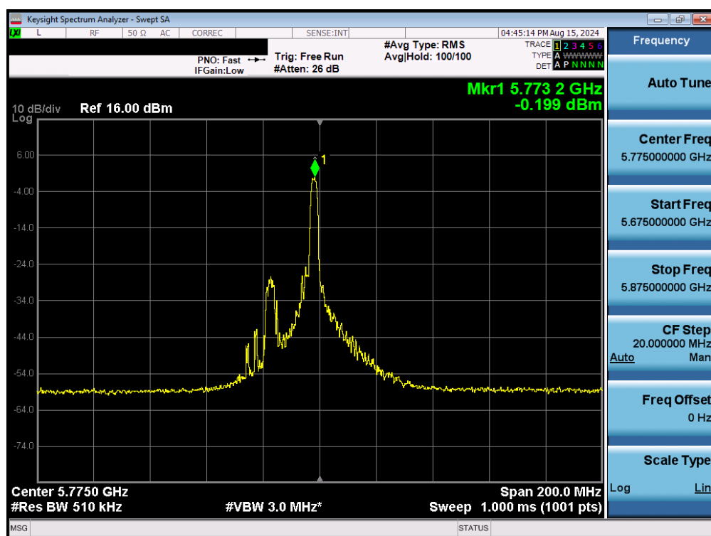
Plot 7-161. Power Spectral Density Plot MIMO ANT2 (80MHz BW 802.11be – 26 Tones (UNII Band 3) – Ch. 155)
