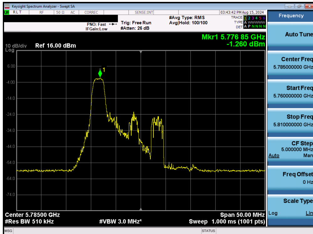
Plot 7-159. Power Spectral Density Plot MIMO ANT2 (20MHz BW 802.11be – 26 Tones (UNII Band 3) – Ch. 157)
