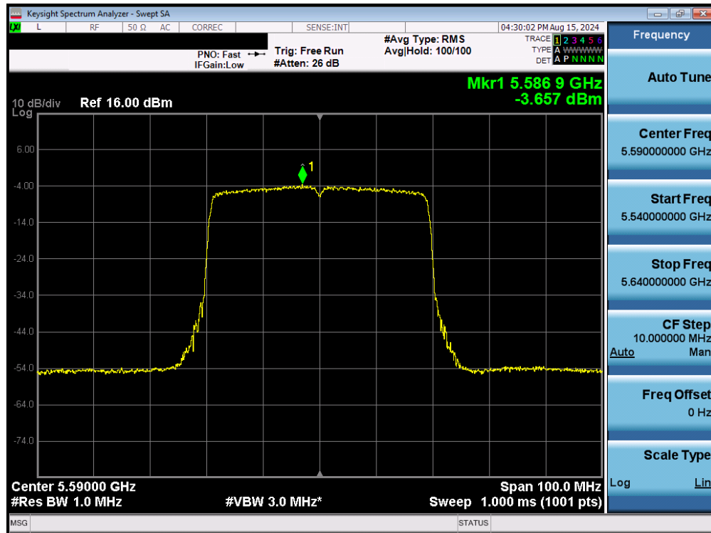
Plot 7-174. Power Spectral Density Plot MIMO ANT2 (40MHz BW 802.11be – 484 Tones (UNII Band 2C) – Ch. 118)
