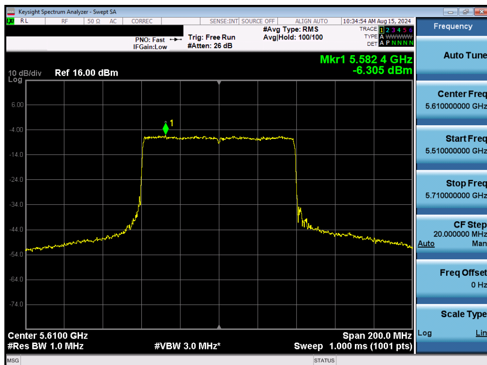
Plot 7-126. Power Spectral Density Plot MIMO ANT1 (80MHz BW 802.11be – 996 Tones (UNII Band 2C) – Ch. 122)
