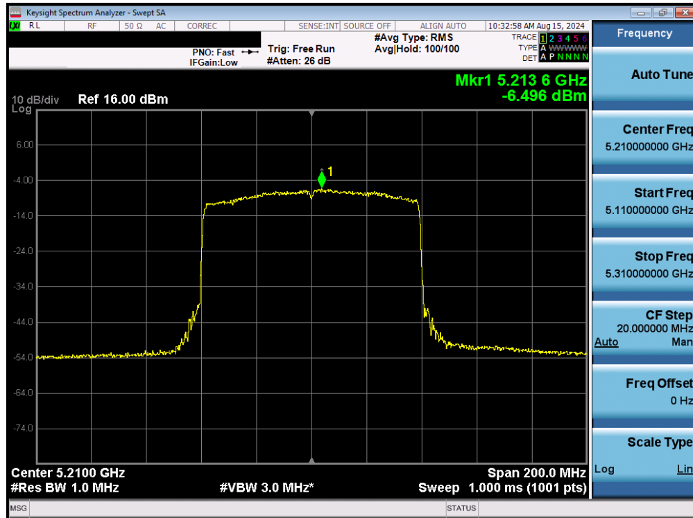
Plot 7-119. Power Spectral Density Plot MIMO ANT1 (80MHz BW 802.11be – 996 Tones (UNII Band 1) – Ch. 42)
