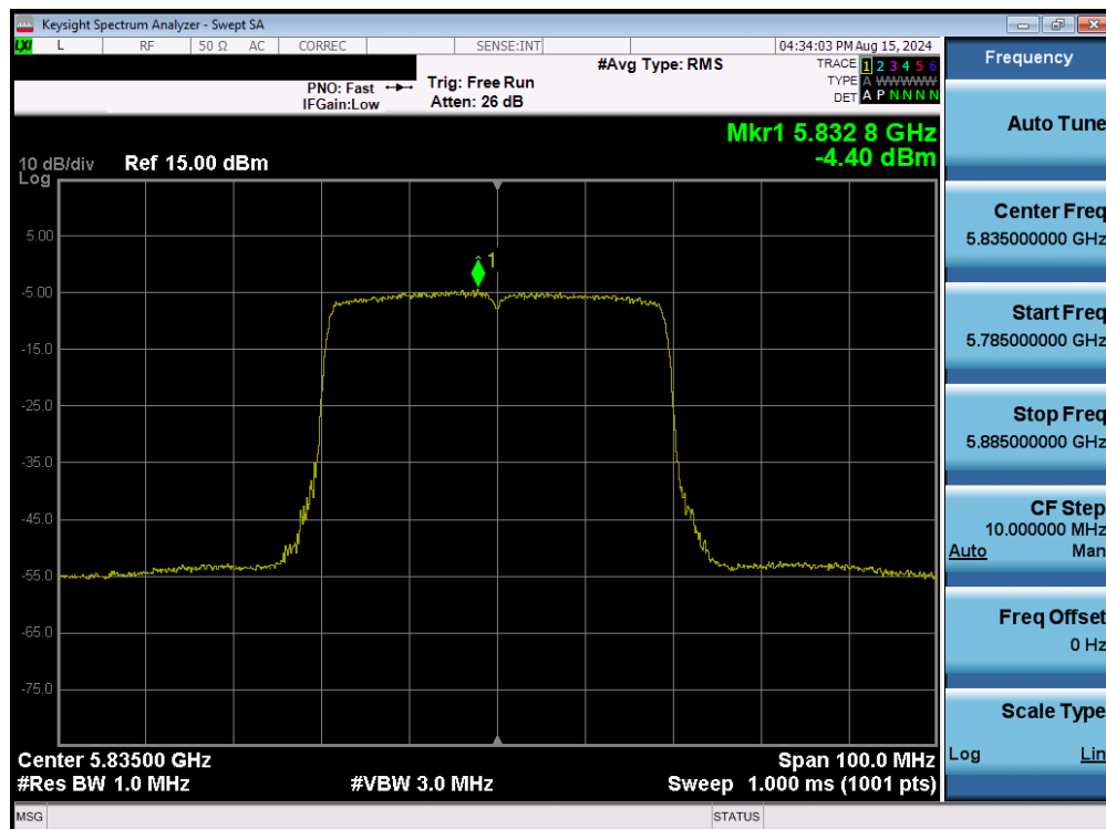
Plot 7-181. Power Spectral Density Plot MIMO ANT2 (40MHz BW 802.11be – 484 Tones (UNII Band 3/4) – Ch. 167)
