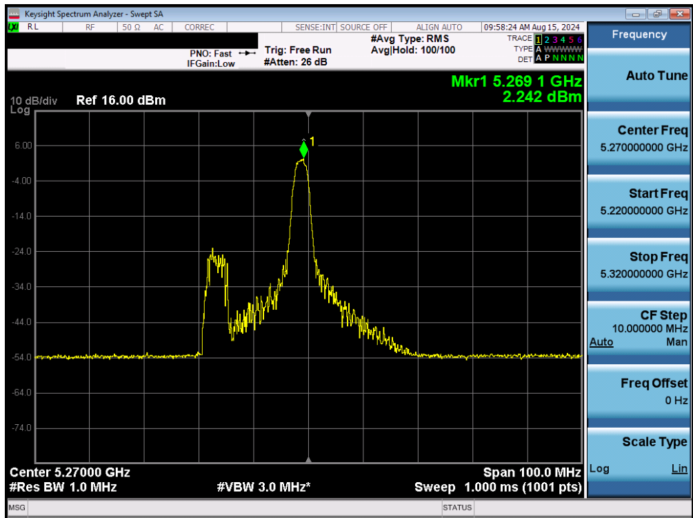
Plot 7-104. Power Spectral Density Plot MIMO ANT1 (40MHz BW 802.11be – 26 Tones (UNII Band 2A) – Ch. 54)
