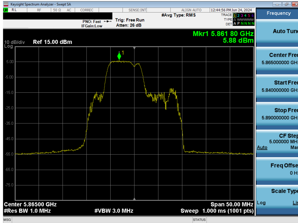
Plot 7-194. Power Spectral Density Plot MIMO ANT2 (20MHz BW 802.11be – 52+26 Tones (UNII Band 4) – Ch. 173)
