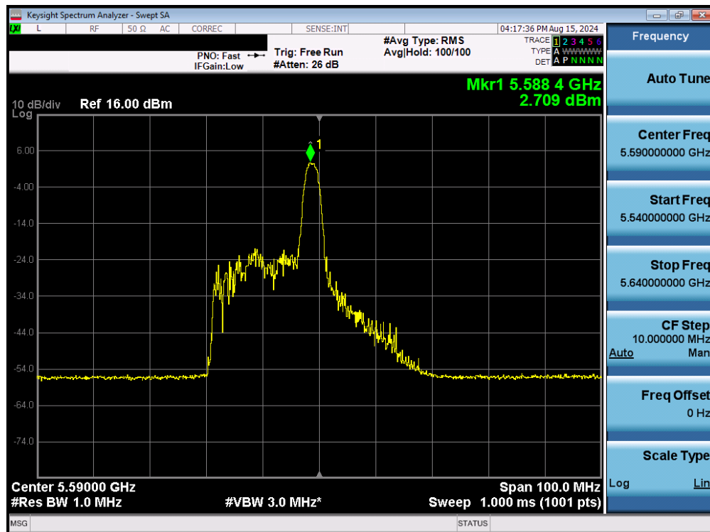
Plot 7-156. Power Spectral Density Plot MIMO ANT2 (40MHz BW 802.11be – 26 Tones (UNII Band 2C) – Ch. 118)
