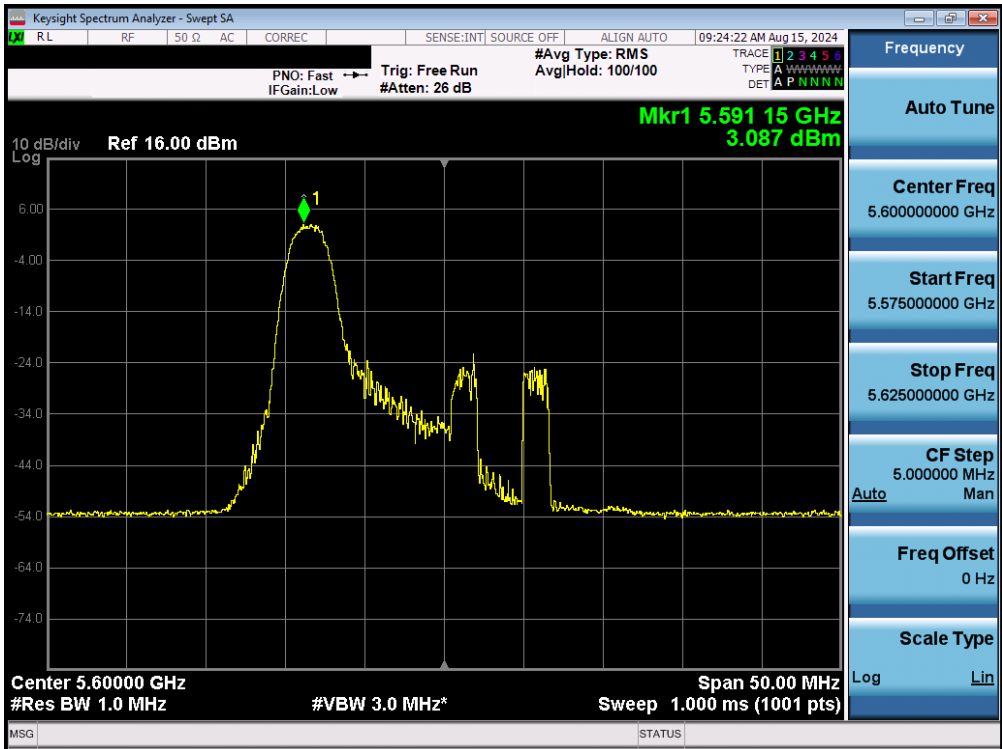
Plot 7-106. Power Spectral Density Plot MIMO ANT1 (20MHz BW 802.11be – 26 Tones (UNII Band 2C) – Ch. 120)
