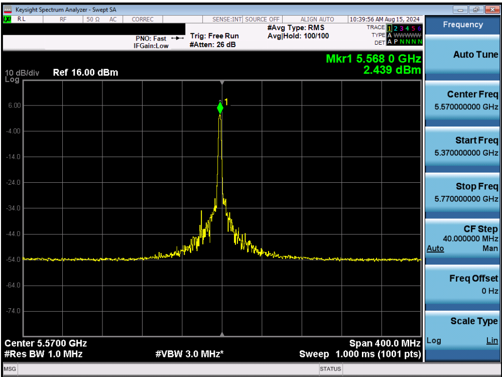
Plot 7-109. Power Spectral Density Plot MIMO ANT1 (160MHz BW 802.11be – 26 Tones (UNII Band 2C) – Ch. 114)
