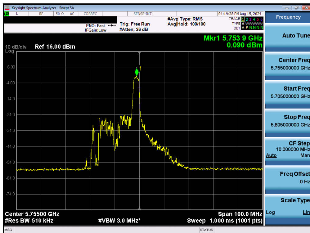
Plot 7-160. Power Spectral Density Plot MIMO ANT2 (40MHz BW 802.11be – 26 Tones (UNII Band 3) – Ch. 151)
