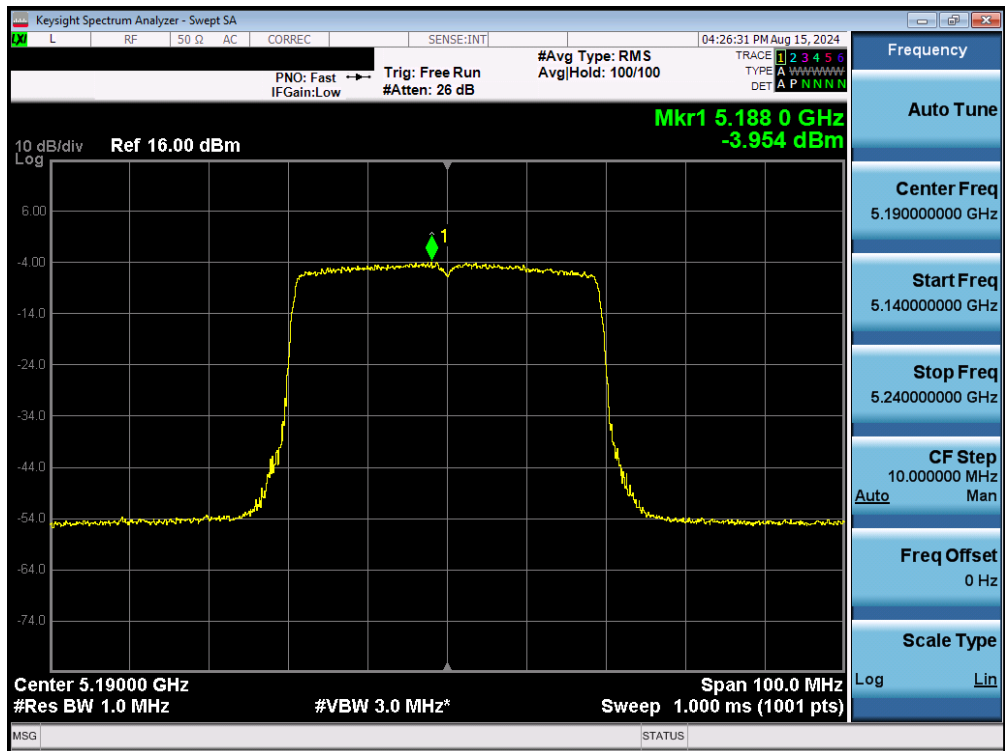
Plot 7-167. Power Spectral Density Plot MIMO ANT2 (40MHz BW 802.11be – 484 Tones (UNII Band 1) – Ch. 38)
