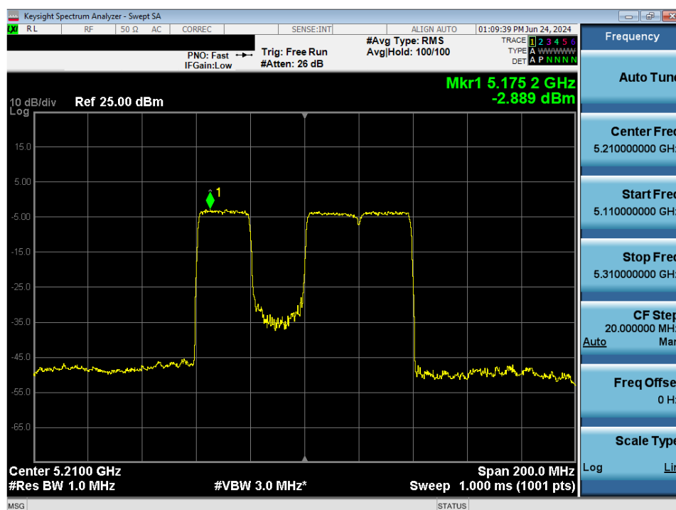
Plot 7-185. Power Spectral Density Plot MIMO ANT2 (80MHz BW 802.11be – 484+242Tones (UNII Band 1) – Ch. 42)
