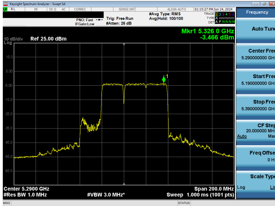
Plot 7-188. Power Spectral Density Plot MIMO ANT2 (80MHz BW 802.11be – 484+242Tones (UNII Band 2A) – Ch. 58)
