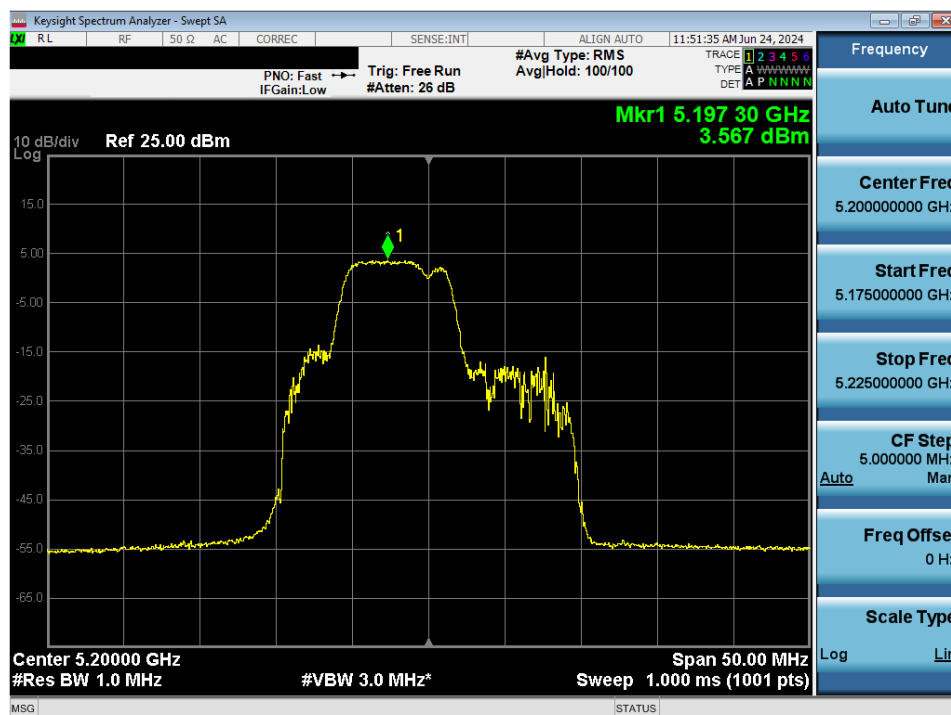
Plot 7-184. Power Spectral Density Plot MIMO ANT2 (20MHz BW 802.11be – 52+26 Tones (UNII Band 1) – Ch. 40)
