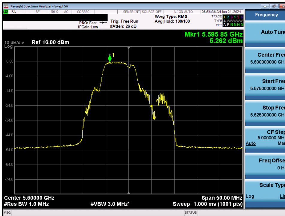
Plot 7-140. Power Spectral Density Plot MIMO ANT1 (20MHz BW 802.11be – 52+26 Tones (UNII Band 2C) – Ch. 120)
