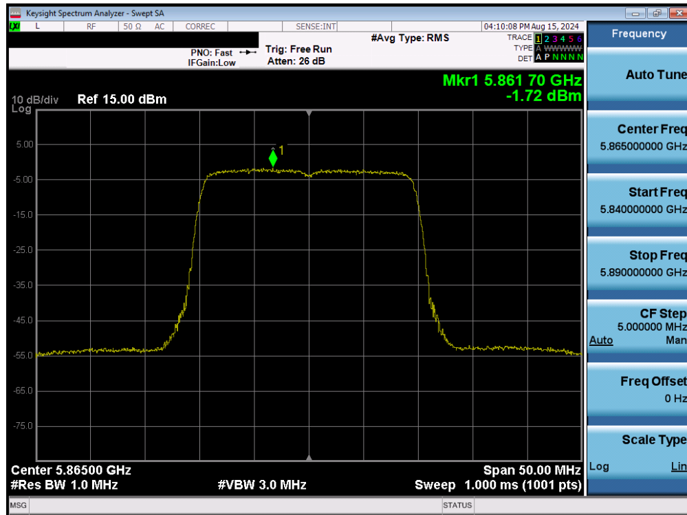
Plot 7-180. Power Spectral Density Plot MIMO ANT2 (20MHz BW 802.11be – 242 Tones (UNII Band 4) – Ch. 173)
