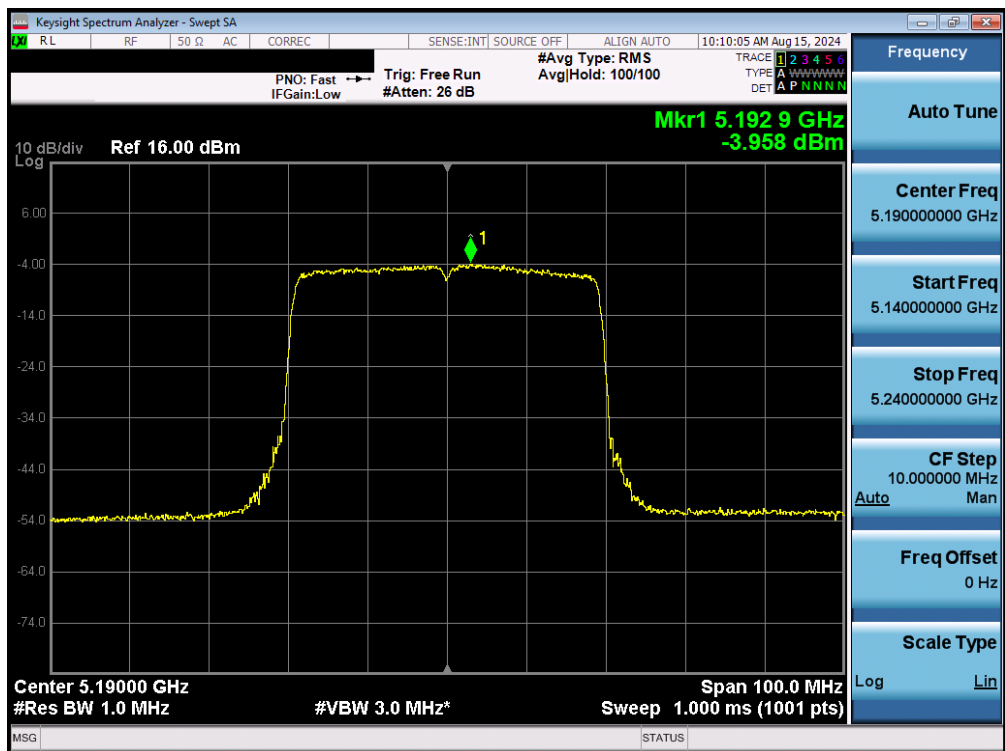
Plot 7-118. Power Spectral Density Plot MIMO ANT1 (40MHz BW 802.11be – 484 Tones (UNII Band 1) – Ch. 38)
