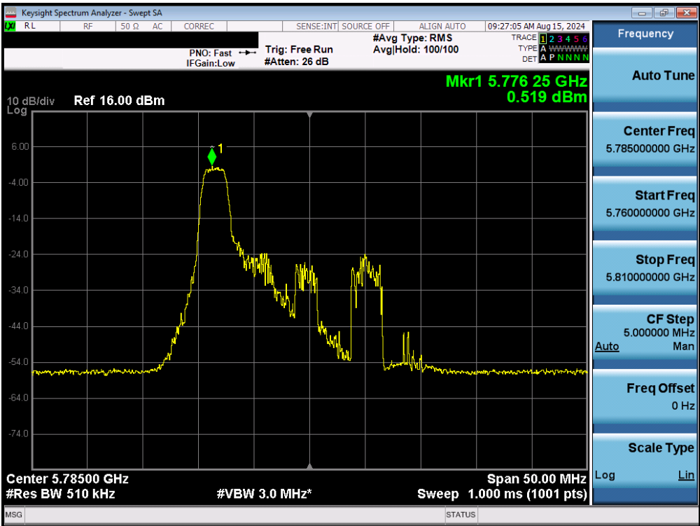
Plot 7-110. Power Spectral Density Plot MIMO ANT1 (20MHz BW 802.11be – 26 Tones (UNII Band 3) – Ch. 157)
