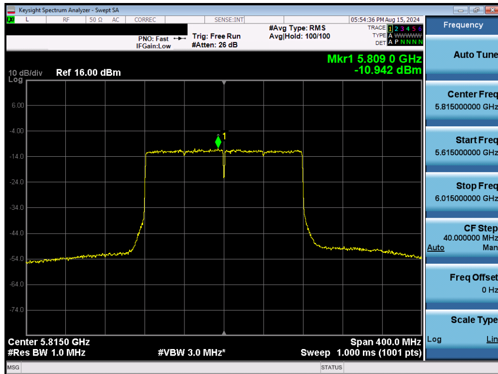
Plot 7-183. Power Spectral Density Plot MIMO ANT2 (160MHz BW 802.11be – 996*2 Tones (UNII Band 3/4) – Ch. 163)
