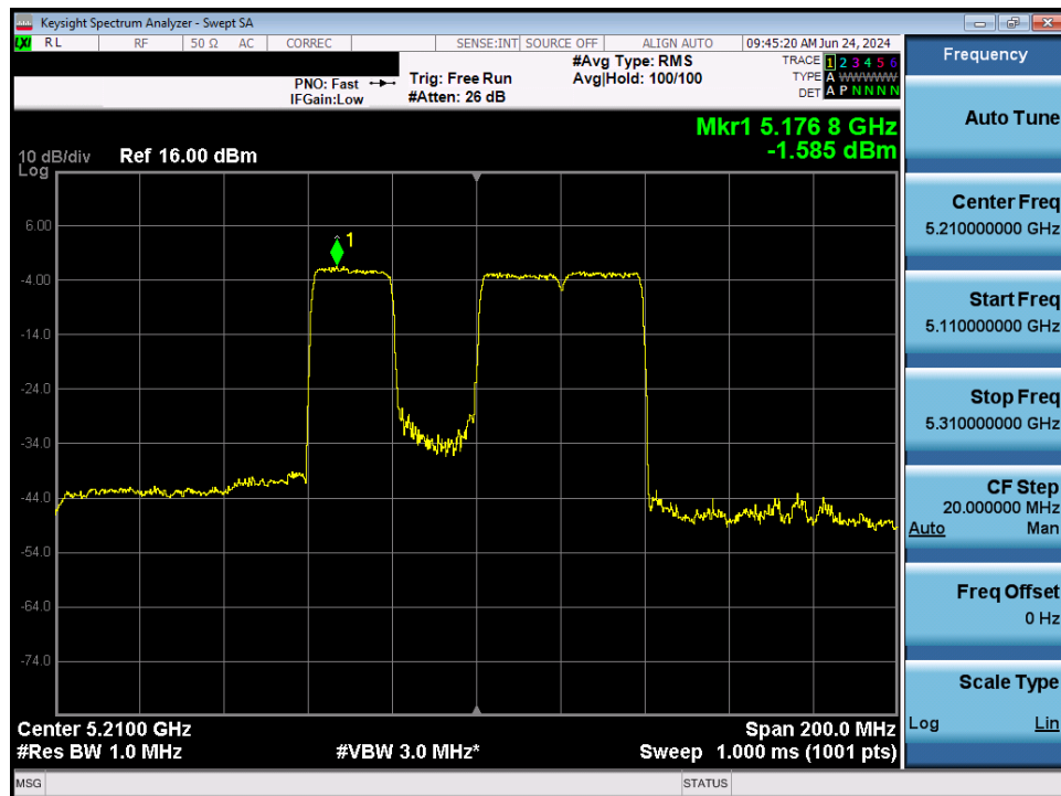
Plot 7-136. Power Spectral Density Plot MIMO ANT1 (80MHz BW 802.11be – 484+242Tones (UNII Band 1) – Ch. 42)
