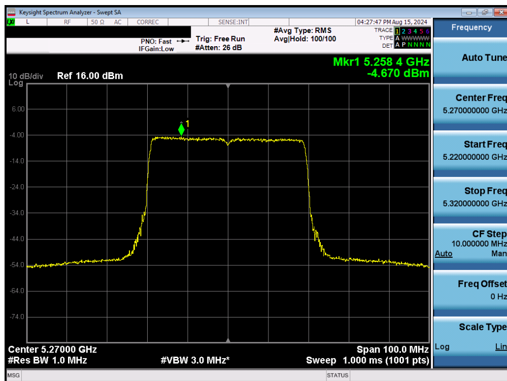
Plot 7-171. Power Spectral Density Plot MIMO ANT2 (40MHz BW 802.11be – 484 Tones (UNII Band 2A) – Ch. 54)
