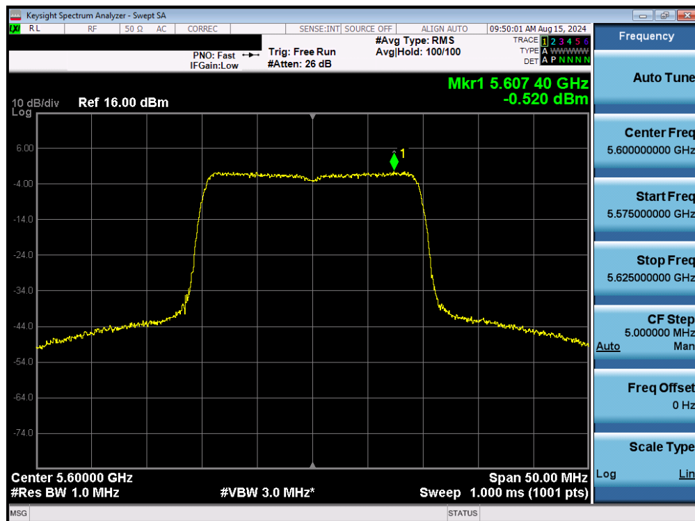
Plot 7-124. Power Spectral Density Plot MIMO ANT1 (20MHz BW 802.11be – 242 Tones (UNII Band 2C) – Ch. 120)
