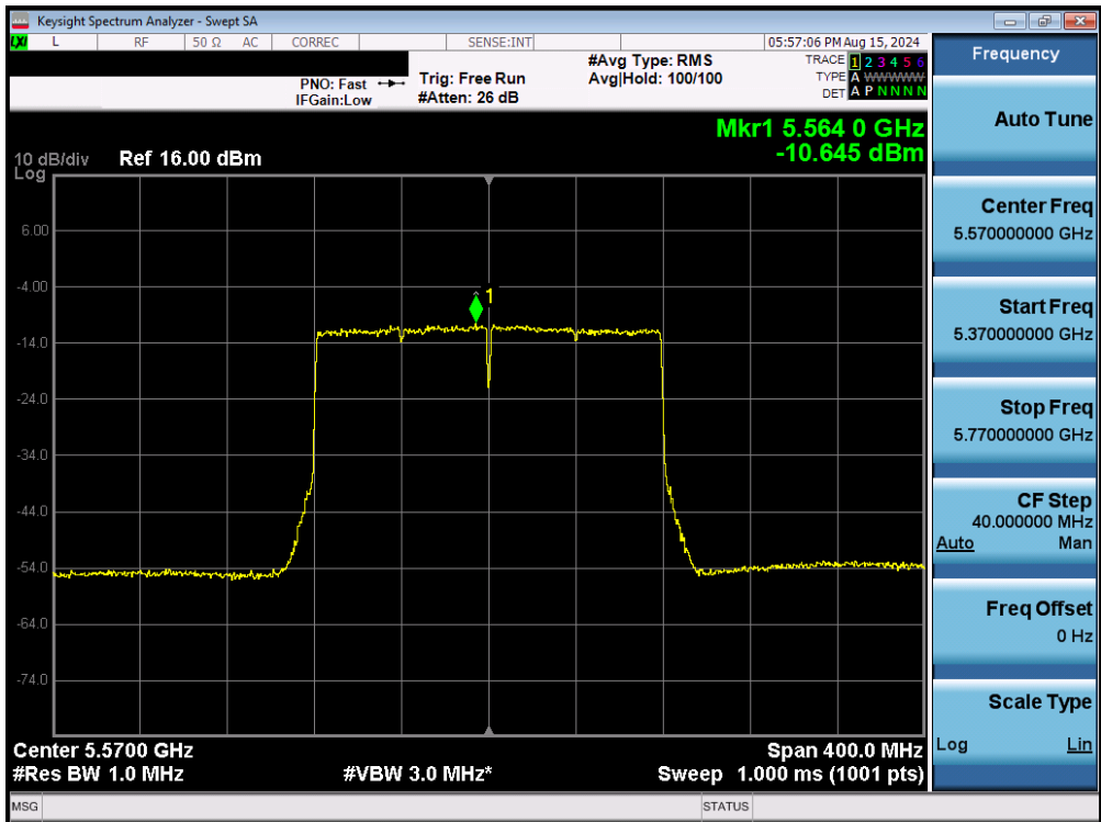
Plot 7-176. Power Spectral Density Plot MIMO ANT2 (160MHz BW 802.11be – 2x996 Tones (UNII Band 2C) – Ch. 114)
