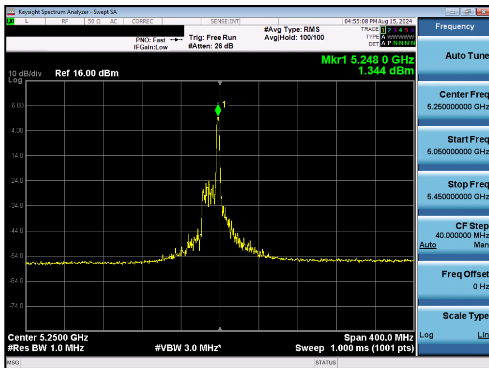
Plot 7-151. Power Spectral Density Plot MIMO ANT2 (160MHz BW 802.11be – 26 Tones (UNII Band 1/2A) – Ch. 50)
