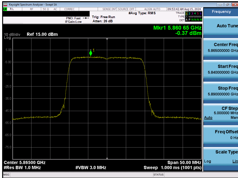
Plot 7-131. Power Spectral Density Plot MIMO ANT1 (20MHz BW 802.11be – 242 Tones (UNII Band 4) – Ch. 173)
