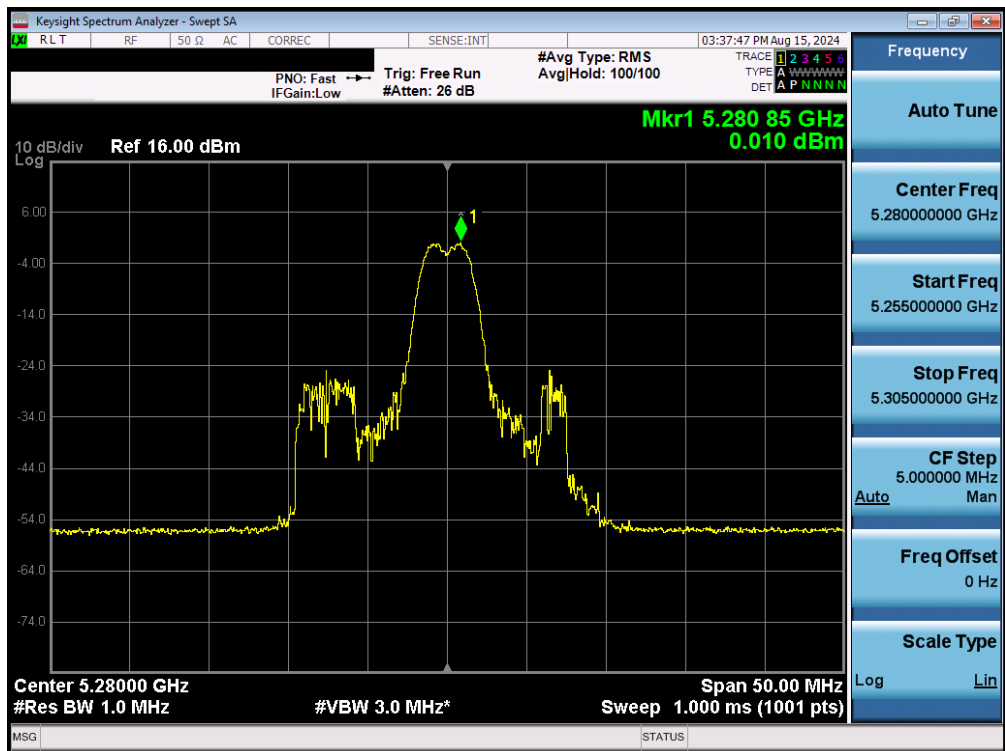
Plot 7-152. Power Spectral Density Plot MIMO ANT2 (20MHz BW 802.11be – 26 Tones (UNII Band 2A) – Ch. 56)
