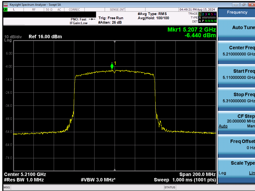
Plot 7-168. Power Spectral Density Plot MIMO ANT2 (80MHz BW 802.11be – 996 Tones (UNII Band 1) – Ch. 42)
