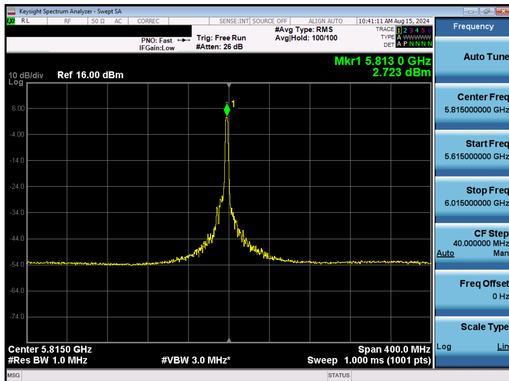
Plot 7-116. Power Spectral Density Plot MIMO ANT1 (160MHz BW 802.11be – 26 Tones (UNII Band 3/4) – Ch. 163)
