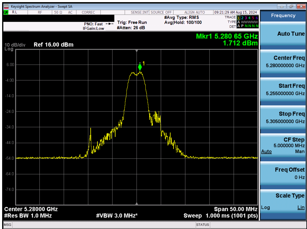
Plot 7-103. Power Spectral Density Plot MIMO ANT1 (20MHz BW 802.11be – 26 Tones (UNII Band 2A) – Ch. 56)
