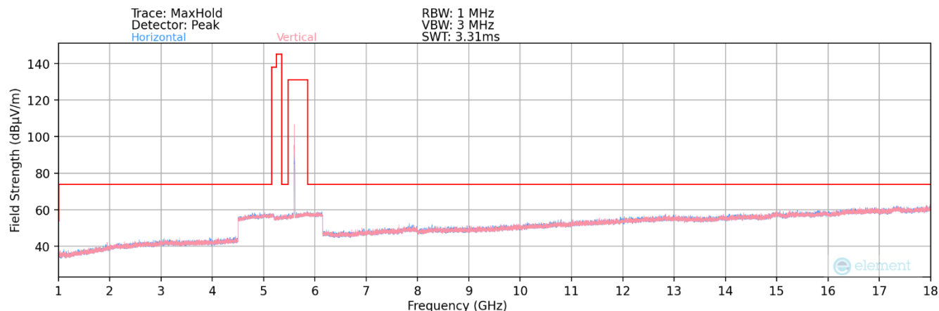
Plot 7-198. Radiated Spurious Plot above 1GHz MIMO (802.11be – UNII 2A Ch. 56)
