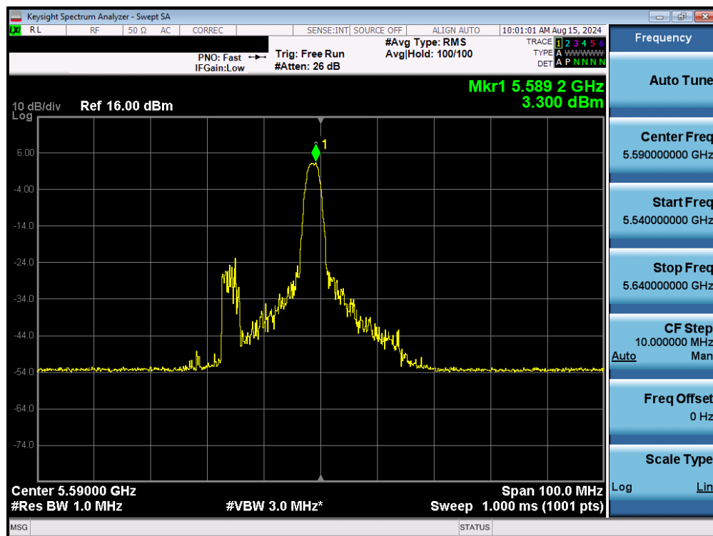
Plot 7-107. Power Spectral Density Plot MIMO ANT1 (40MHz BW 802.11be – 26 Tones (UNII Band 2C) – Ch. 118)
