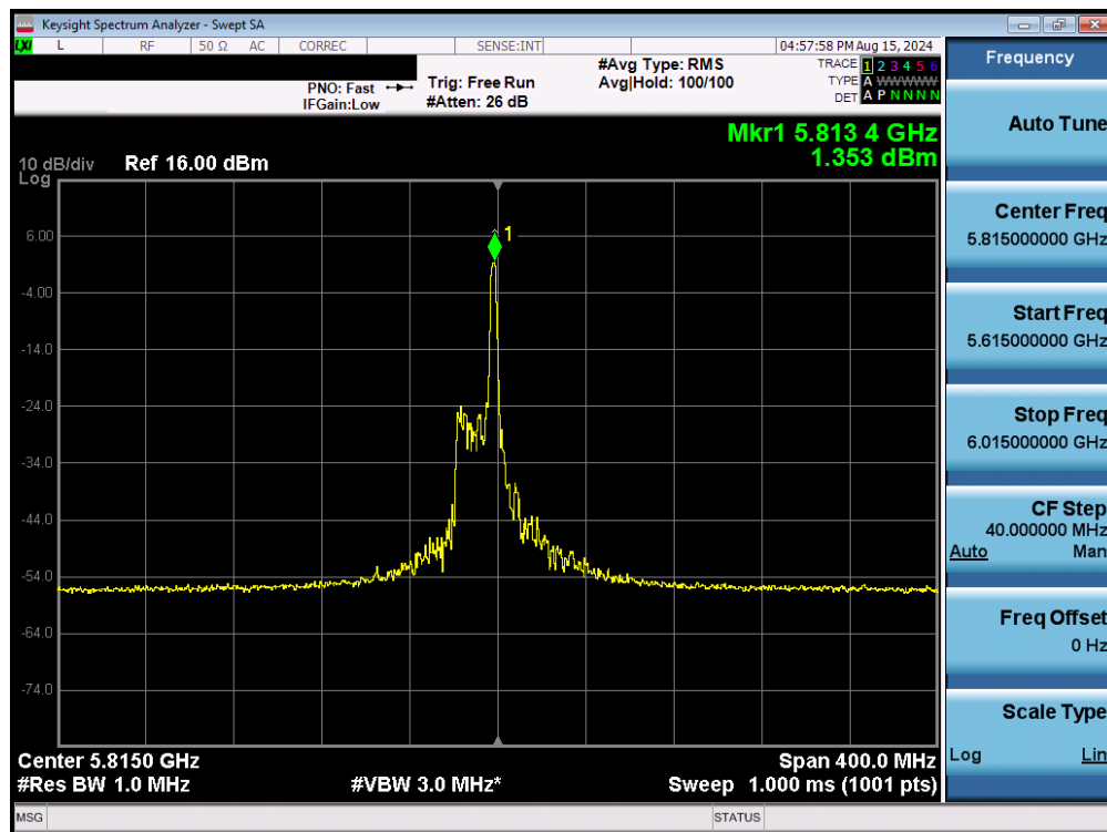
Plot 7-165. Power Spectral Density Plot MIMO ANT2 (160MHz BW 802.11be – 26 Tones (UNII Band 3/4) – Ch. 163)
