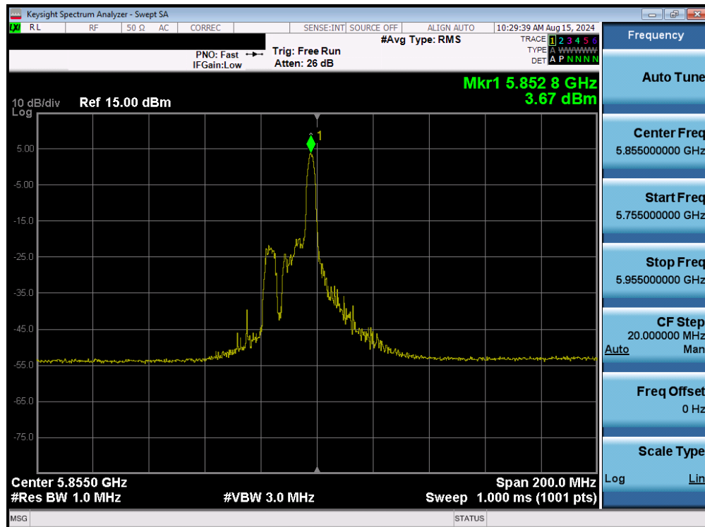
Plot 7-115. Power Spectral Density Plot MIMO ANT1 (80MHz BW 802.11be – 26 Tones (UNII Band 3/4) – Ch. 171)
