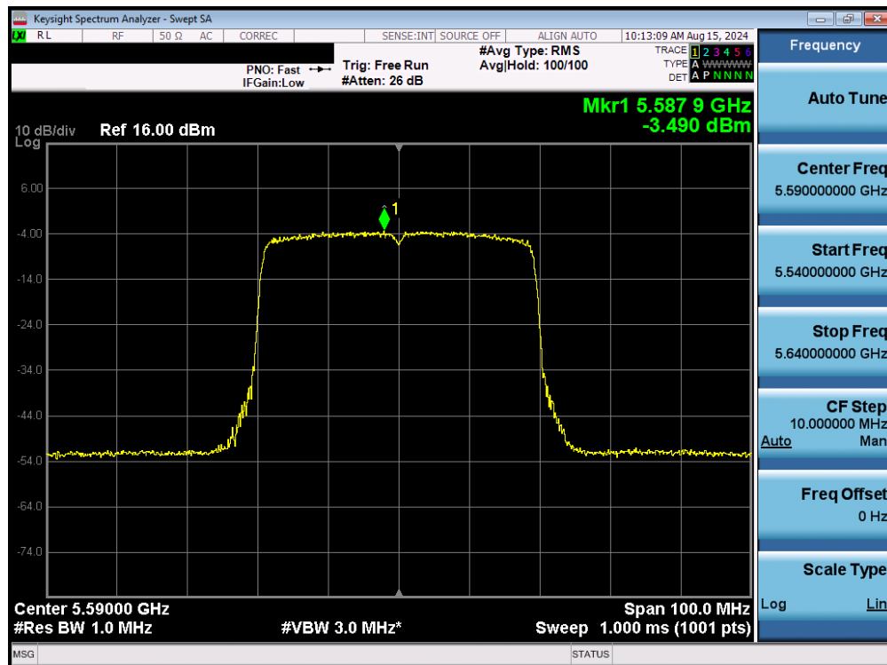
Plot 7-125. Power Spectral Density Plot MIMO ANT1 (40MHz BW 802.11be – 484 Tones (UNII Band 2C) – Ch. 118)
