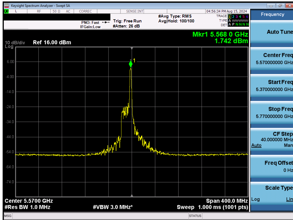
Plot 7-158. Power Spectral Density Plot MIMO ANT2 (160MHz BW 802.11be – 26 Tones (UNII Band 2C) – Ch. 114)
