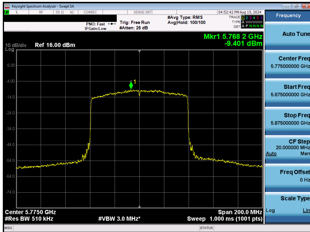
Plot 7-179. Power Spectral Density Plot MIMO ANT2 (80MHz BW 802.11be – 996 Tones (UNII Band 3) – Ch. 155)
