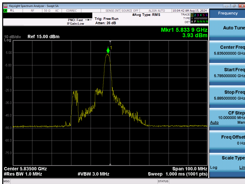
Plot 7-114. Power Spectral Density Plot MIMO ANT1 (40MHz BW 802.11be – 26 Tones (UNII Band 3/4) – Ch. 167)
