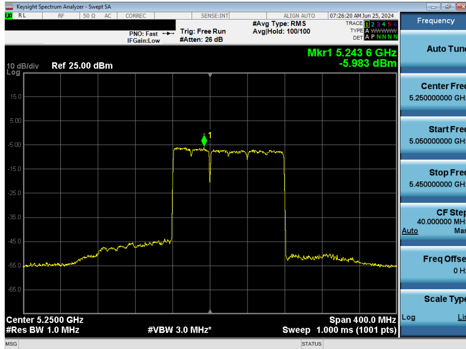
Plot 7-186. Power Spectral Density Plot MIMO ANT2 (160MHz BW 802.11be – 996+484 Tones (UNII Band 1/2A) – Ch. 50)
