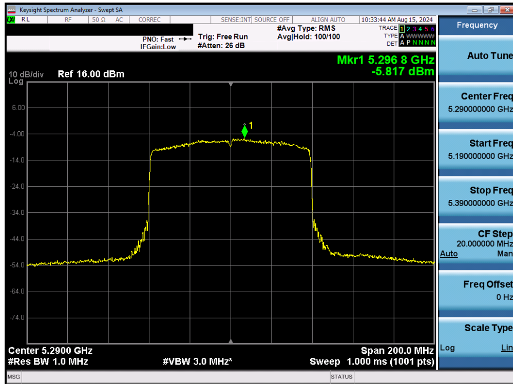
Plot 7-123. Power Spectral Density Plot MIMO ANT1 (80MHz BW 802.11be – 996 Tones (UNII Band 2A) – Ch. 58)
