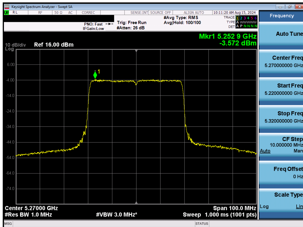
Plot 7-122. Power Spectral Density Plot MIMO ANT1 (40MHz BW 802.11be – 484 Tones (UNII Band 2A) – Ch. 54)
