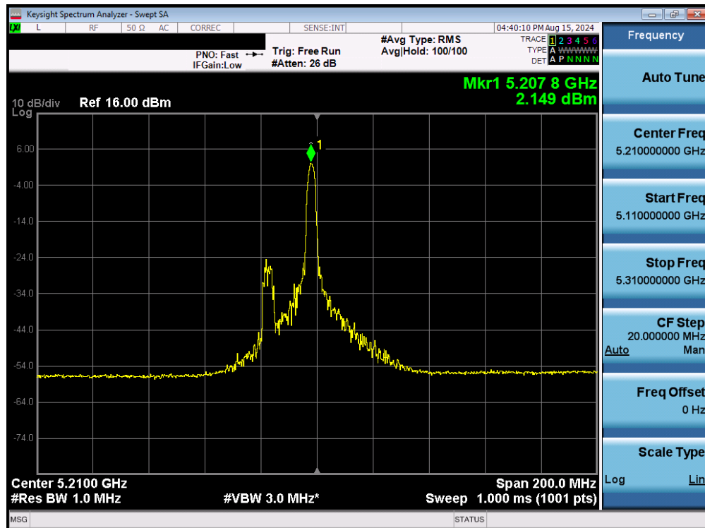
Plot 7-150. Power Spectral Density Plot MIMO ANT2 (80MHz BW 802.11be – 26 Tones (UNII Band 1) – Ch. 42)
