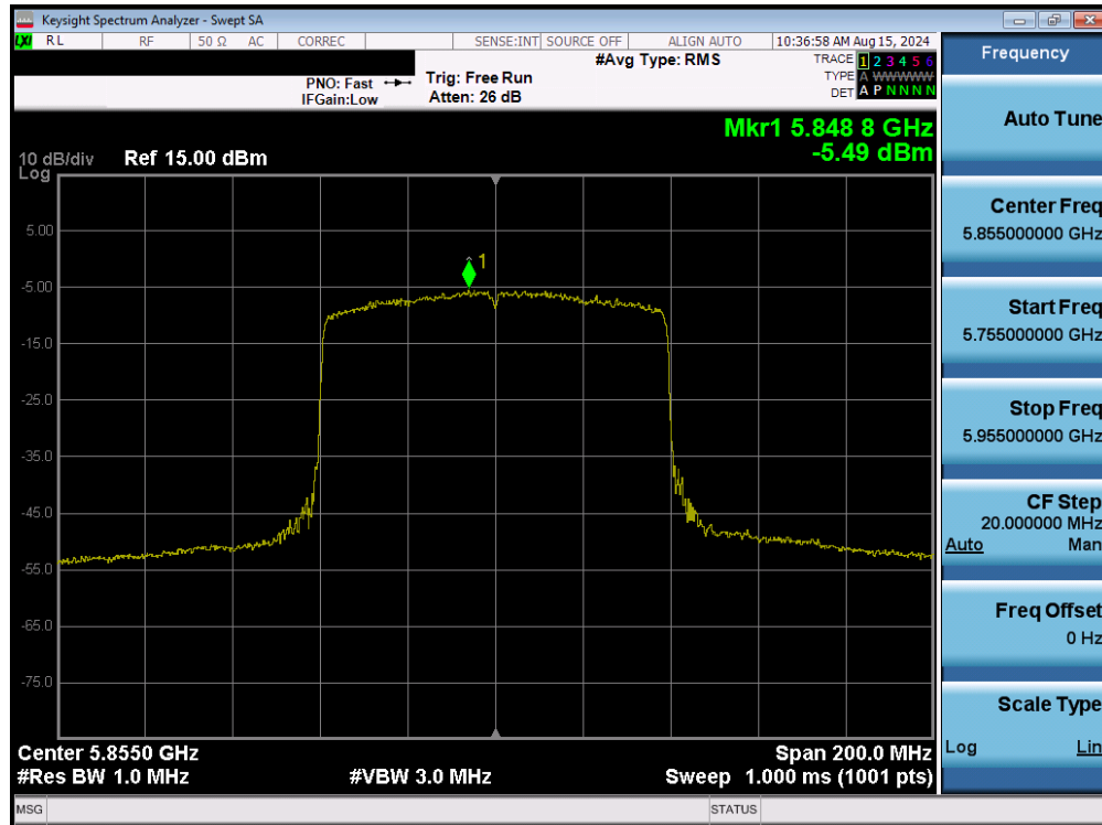
Plot 7-133. Power Spectral Density Plot MIMO ANT1 (80MHz BW 802.11be – 996 Tones (UNII Band 3/4) – Ch. 171)
