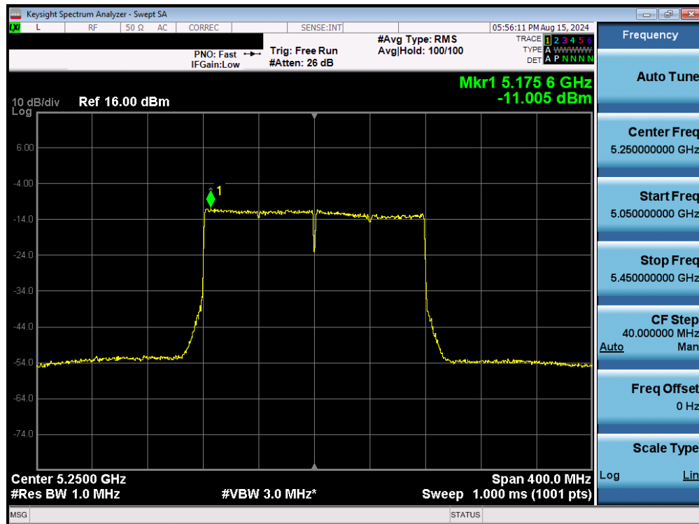
Plot 7-169. Power Spectral Density Plot MIMO ANT2 (160MHz BW 802.11be – 2x996 Tones (UNII Band 1/2A) – Ch. 50)
