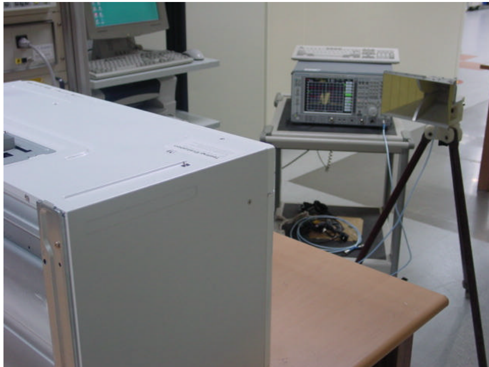
Fig. 2 Test Setup for Operating Frequency Measurements
