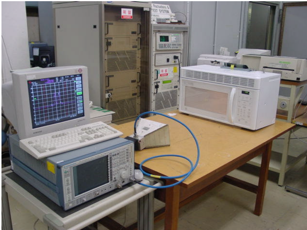
Fig. 5 Test Setup for Operating Frequency Measurements
