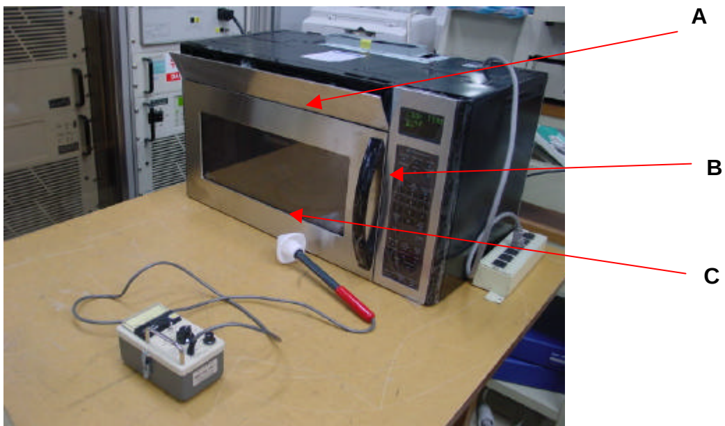
Fig. 1 Test Setup and the locations of maximum leakage
