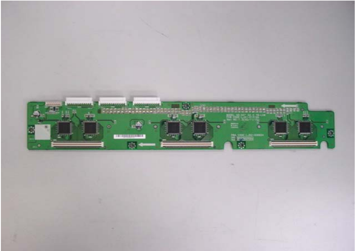
YB-LOW board top view
