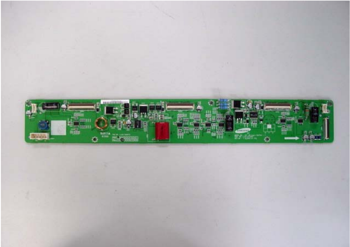
Logic buffer-I board top view
