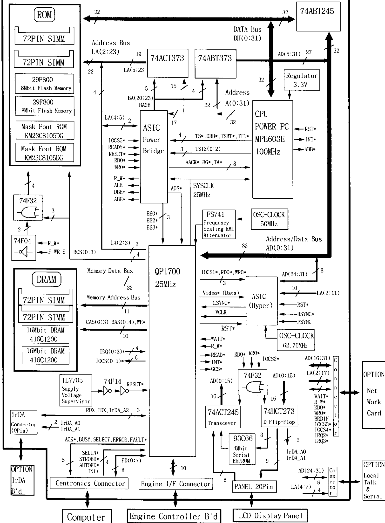
Video Controller Board Block Diagram
