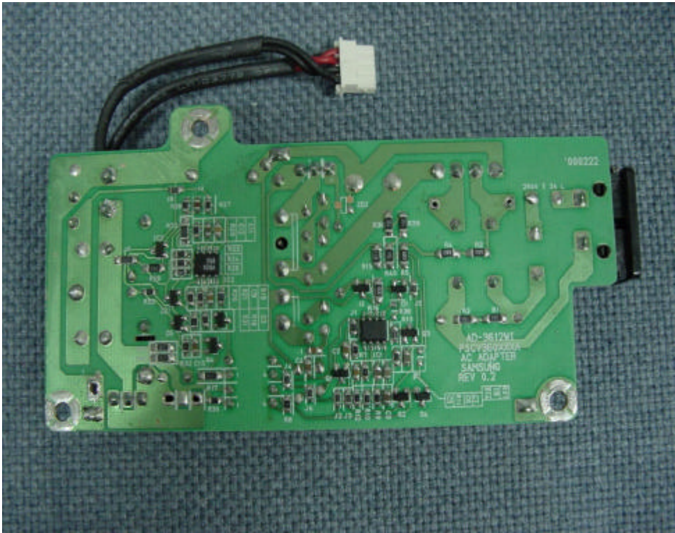
Rear view of internal adaptor PCB
