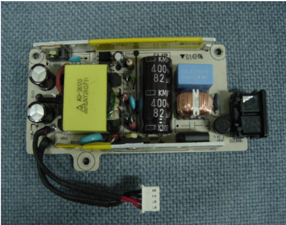
Front view of Internal adaptor PCB
