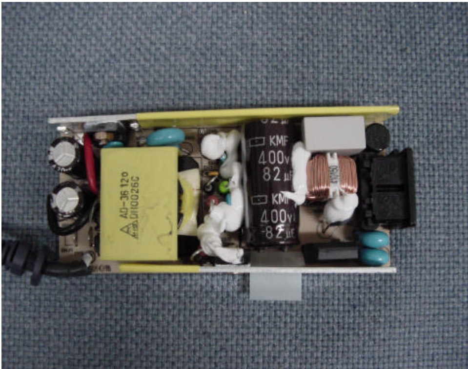
Front view of external adaptor PCB
