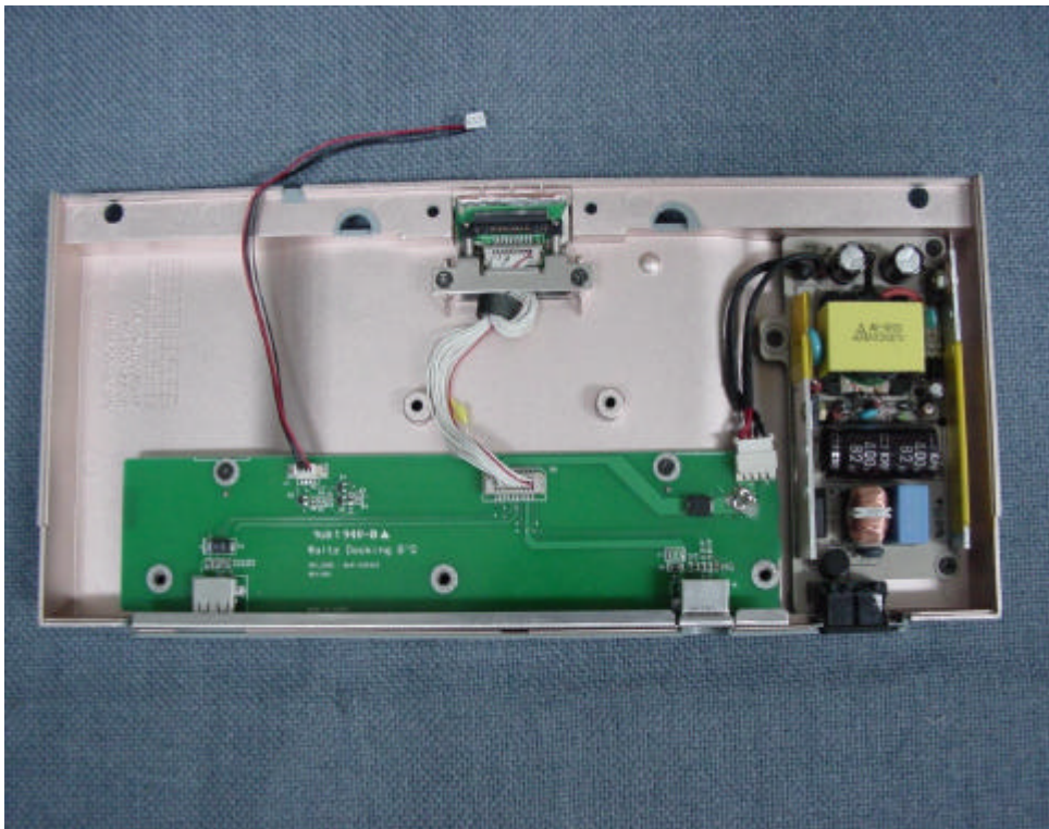
Inside View of Docking station
