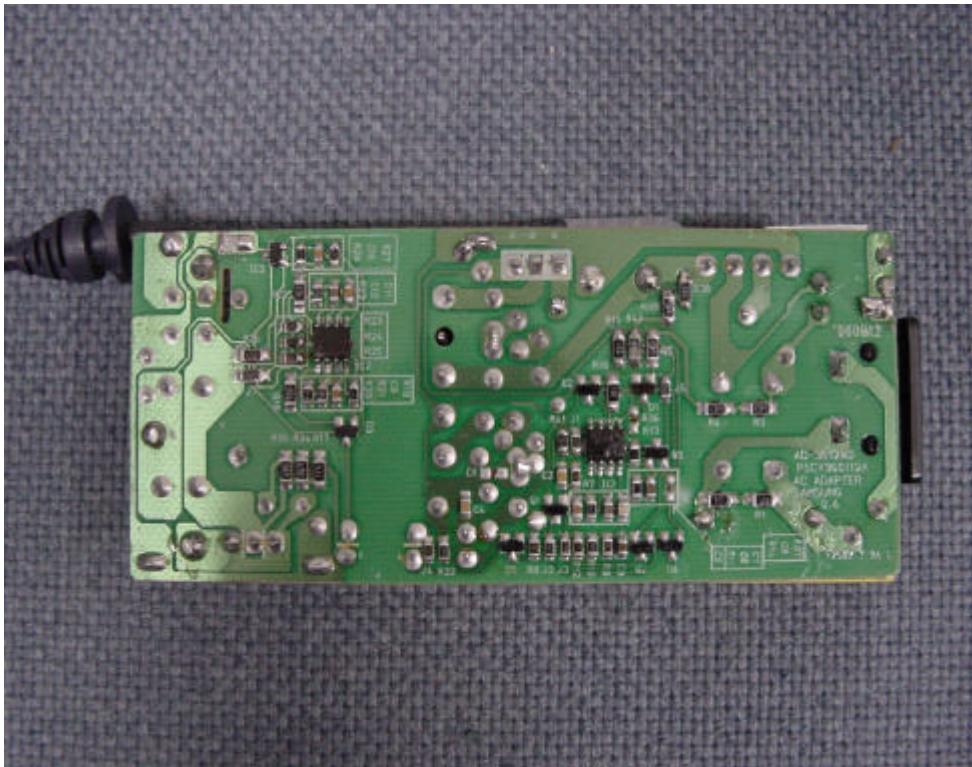
Rear view of external adaptor PCB
