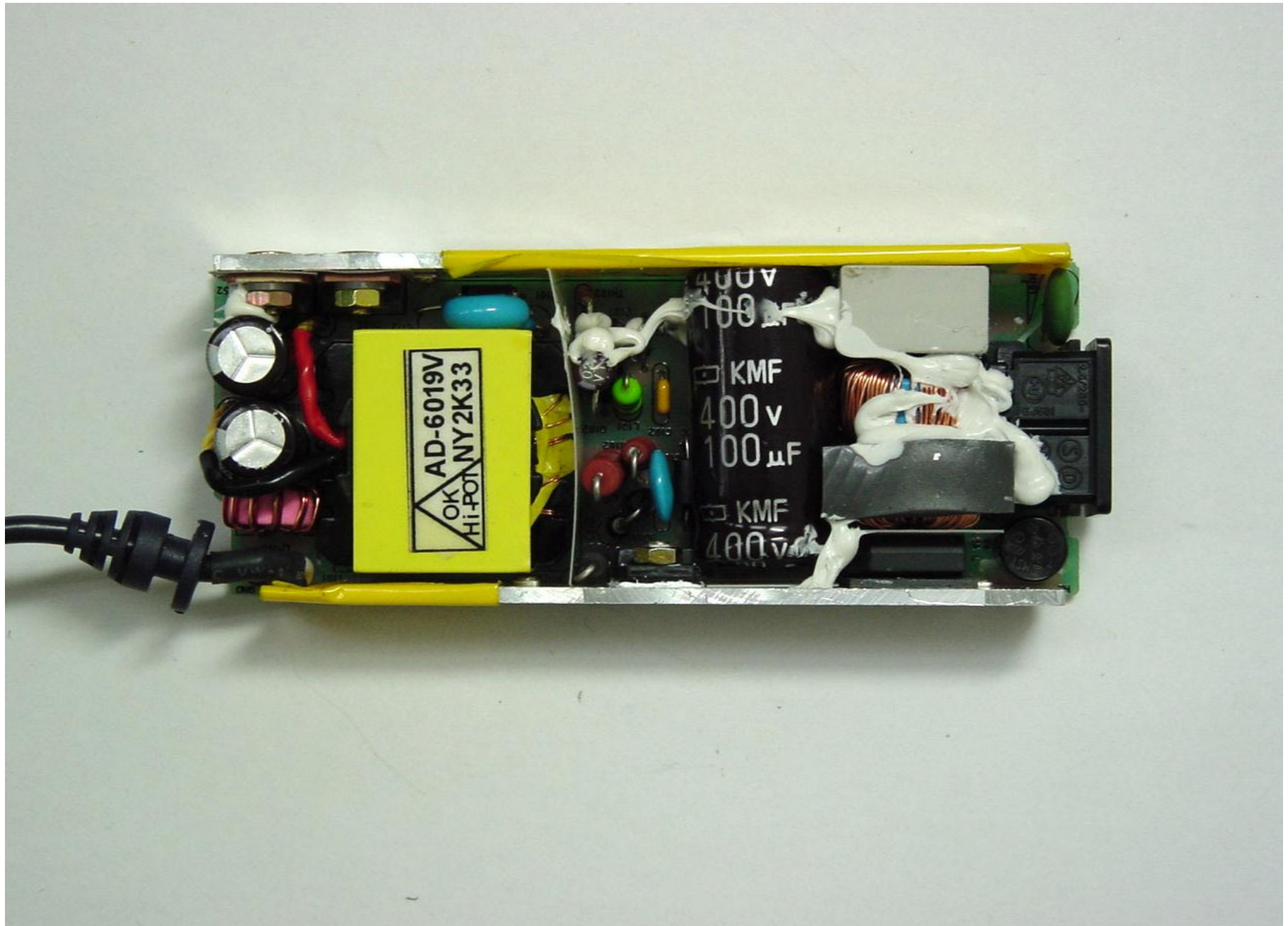
AC Adapter - Front
