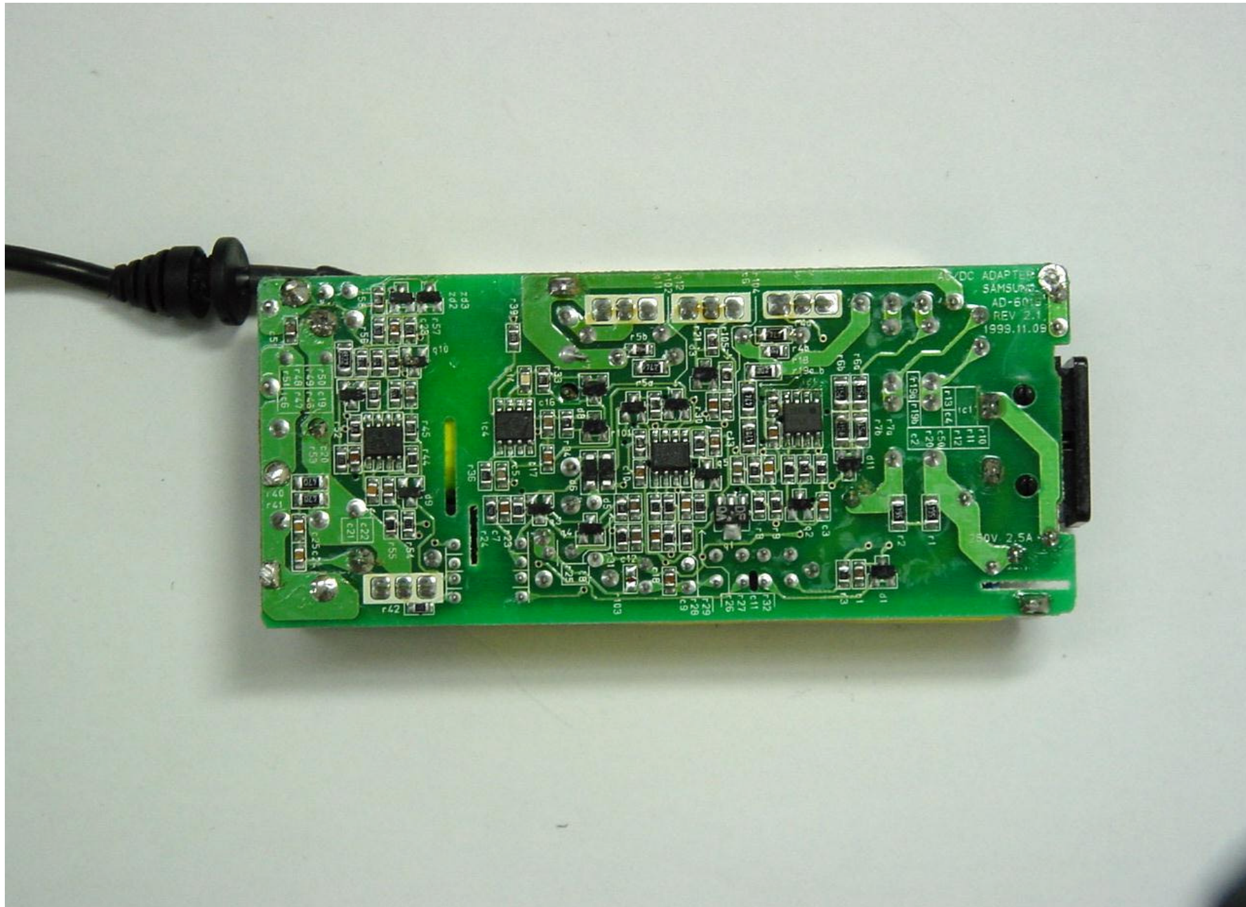
AC Adapter - Rear
