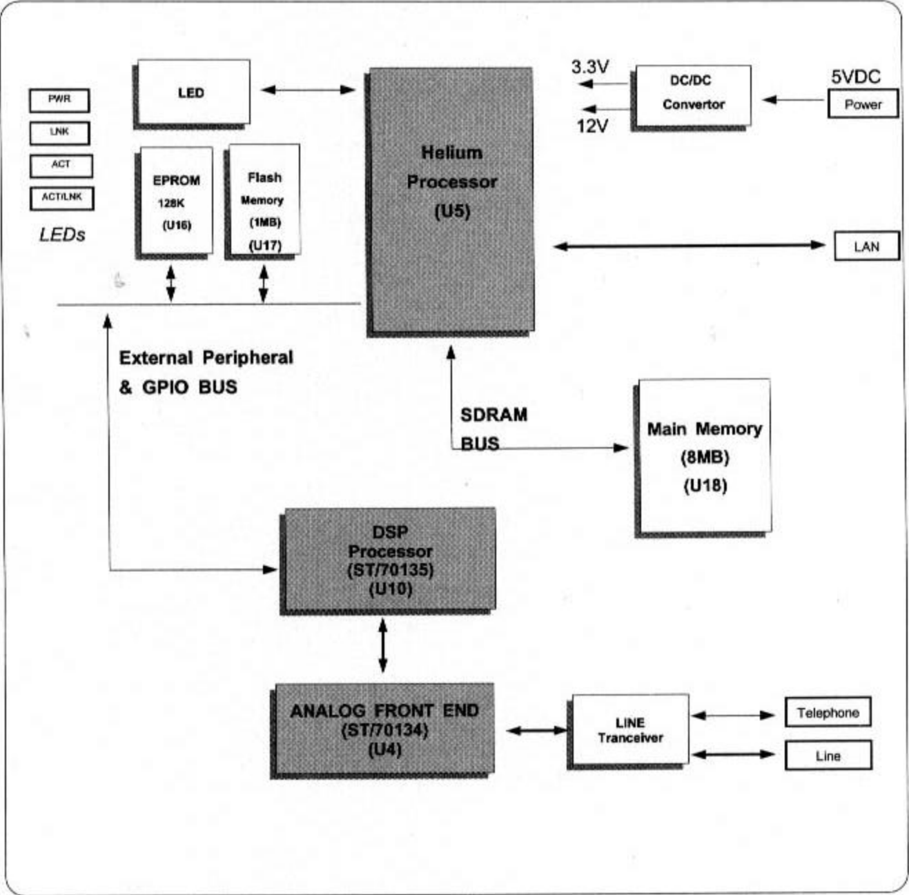
SAM-335A Block Diagram
