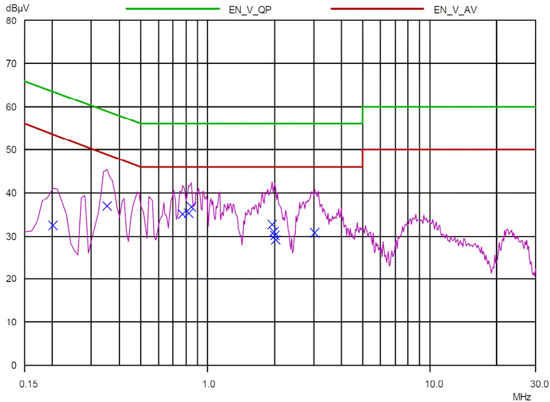
Neutral – PE (Quasi-Peak reading: 'x' mark)
