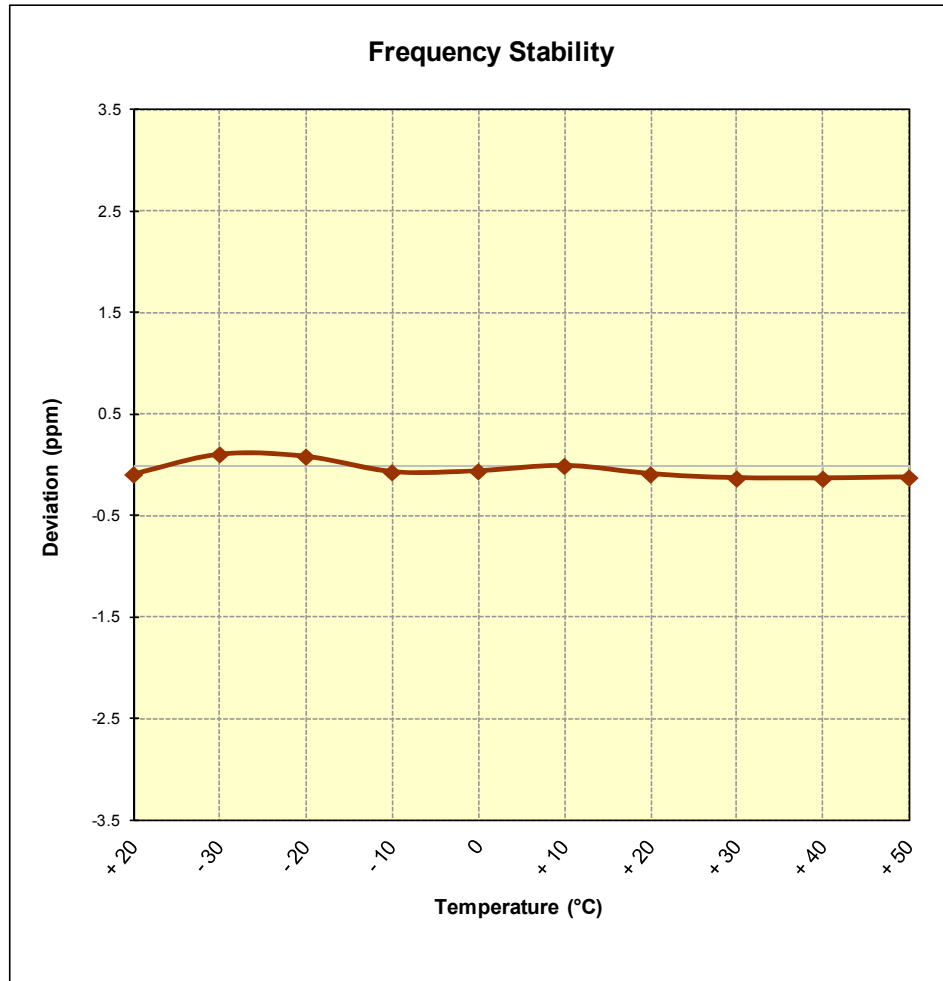
Figure 6-9. Frequency Stability Graph (PCS GSM Mode – Ch. 661)
