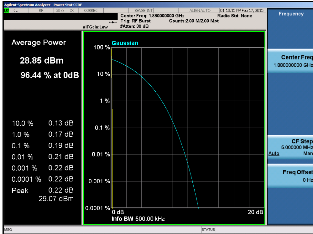
Plot 6-37. Peak-Average Ratio Plot (PCS GSM Mode – Ch. 661)
