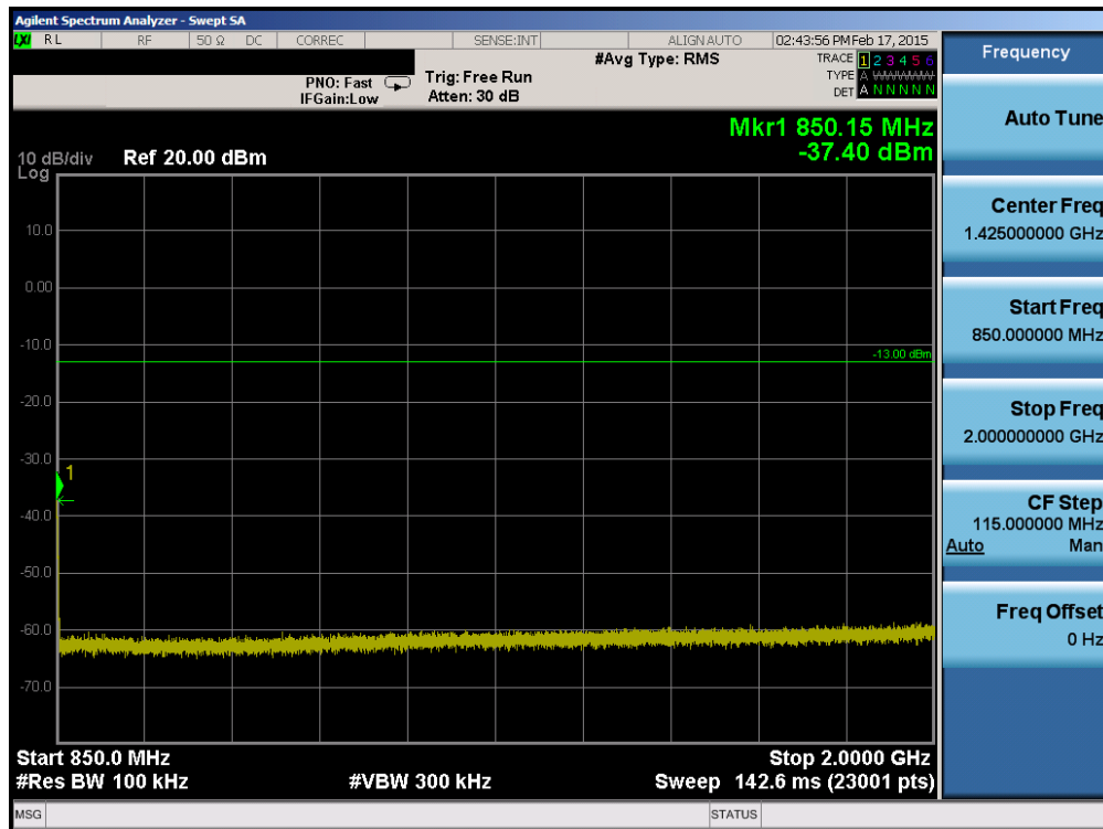
Plot 6-29. Conducted Spurious Plot (Cellular WCDMA Mode – Ch. 4233)
