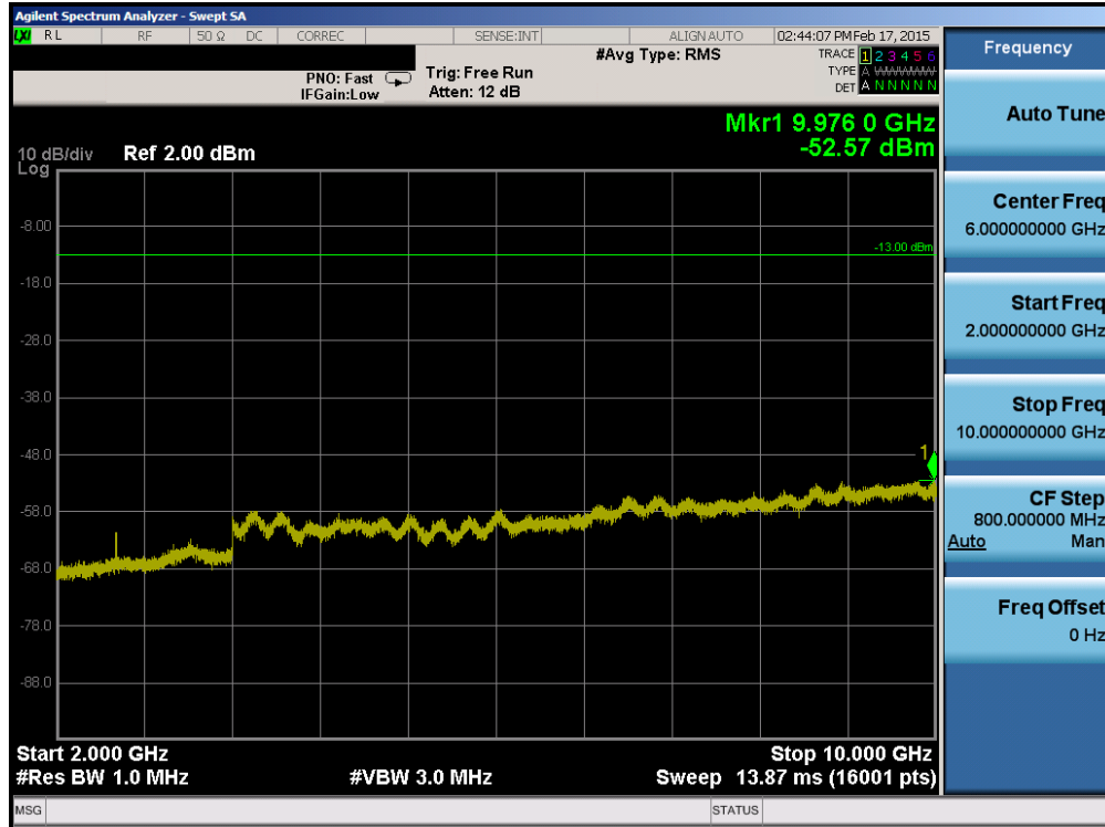
Plot 6-30. Conducted Spurious Plot (Cellular WCDMA Mode – Ch. 4233)
