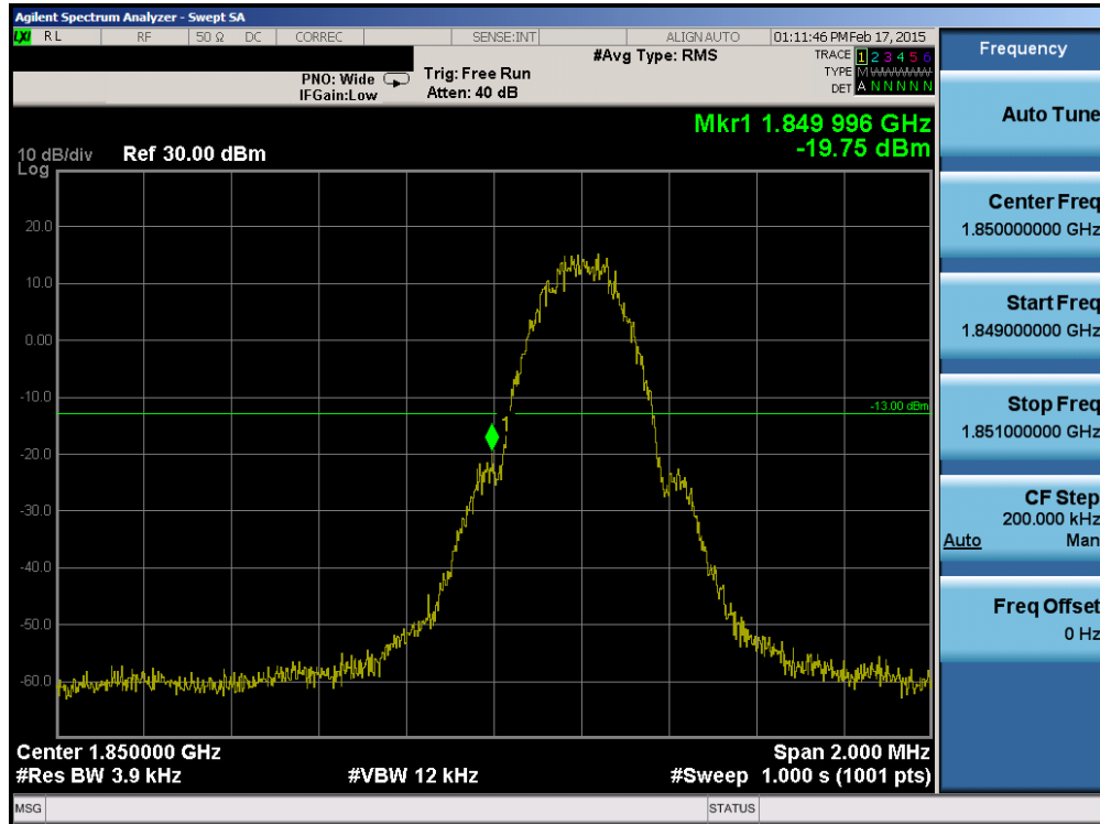
Plot 6-33. Band Edge Plot (PCS GSM Mode – Ch. 512)
