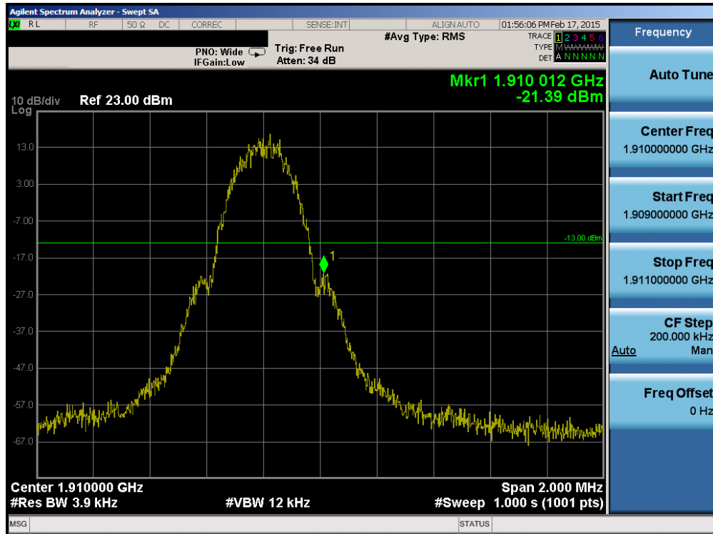
Plot 6-34. Band Edge Plot (PCS GSM Mode – Ch. 810)
