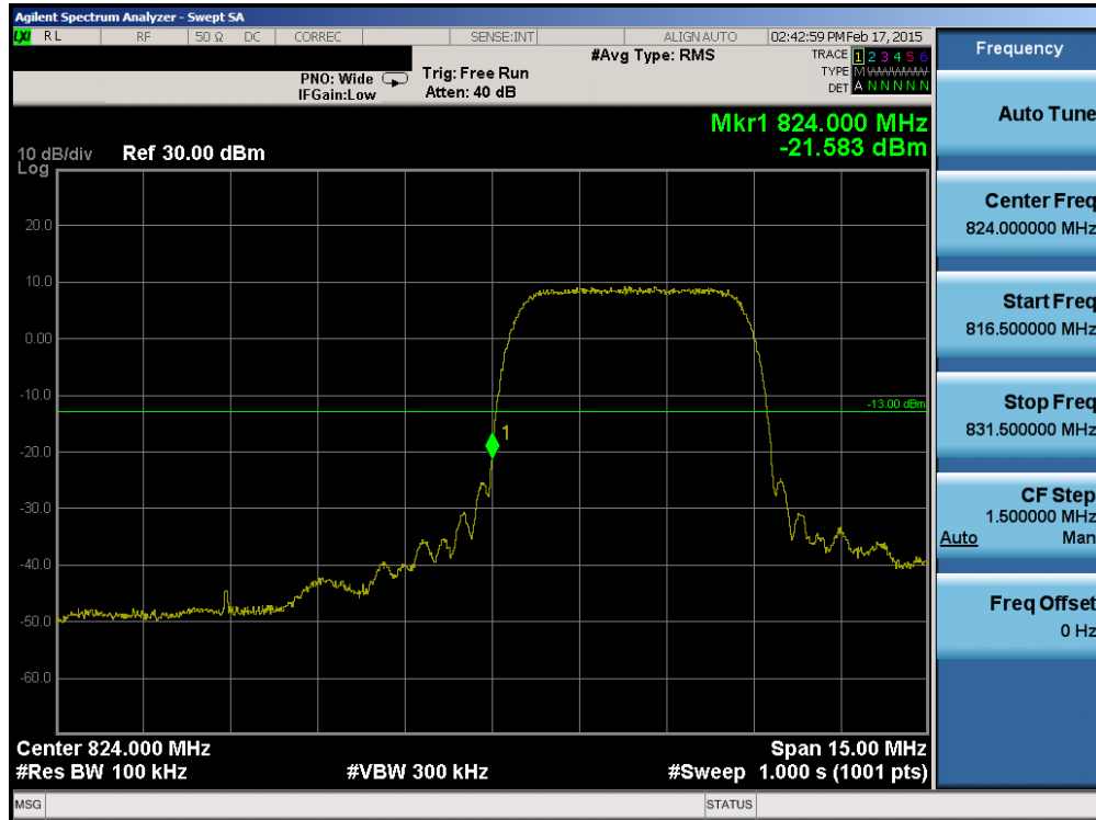
Plot 6-35. Band Edge Plot (Cellular WCDMA Mode – Ch. 4132)
