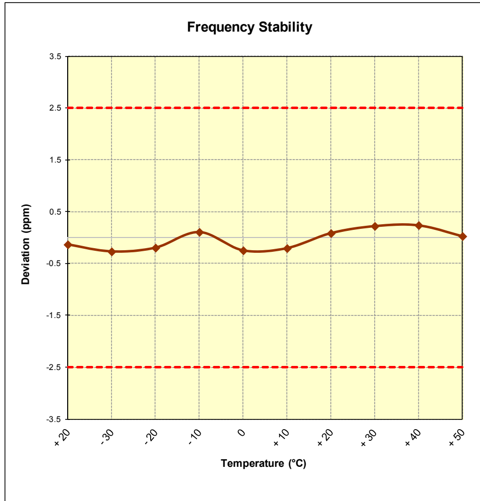
Figure 6-7. Frequency Stability Graph (Cellular GSM Mode – Ch. 190)
