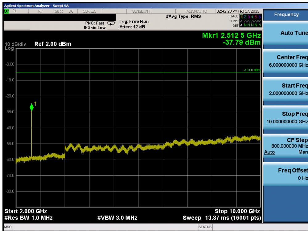
Plot 6-27. Conducted Spurious Plot (Cellular WCDMA Mode – Ch. 4183)
