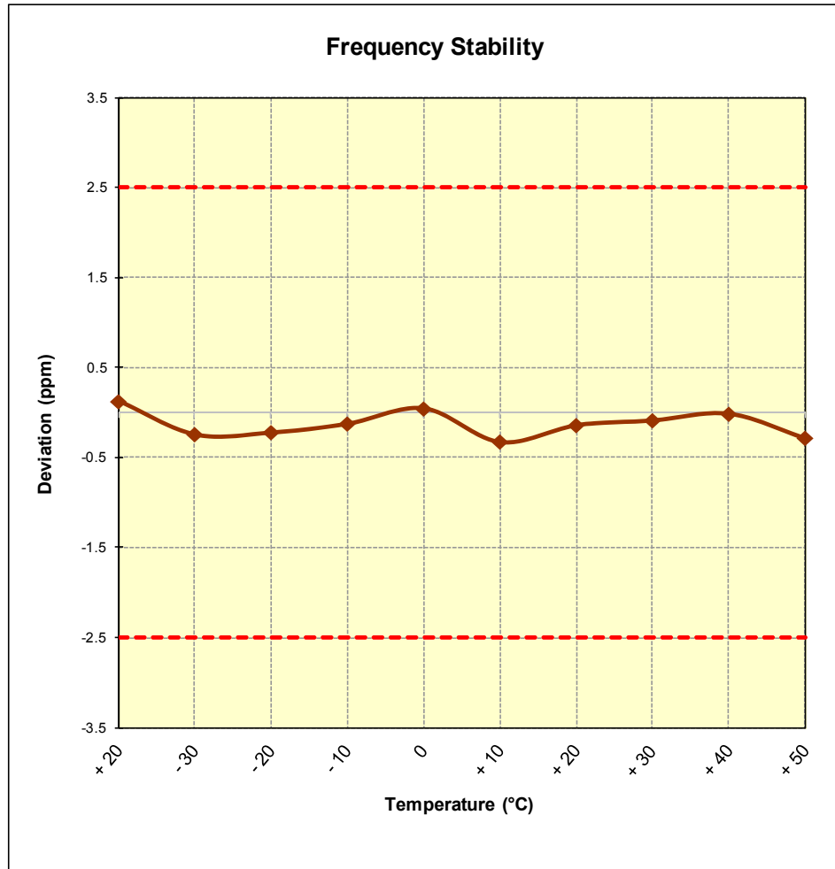
Figure 6-8. Frequency Stability Graph (Cellular WCDMA Mode – Ch. 4183)
