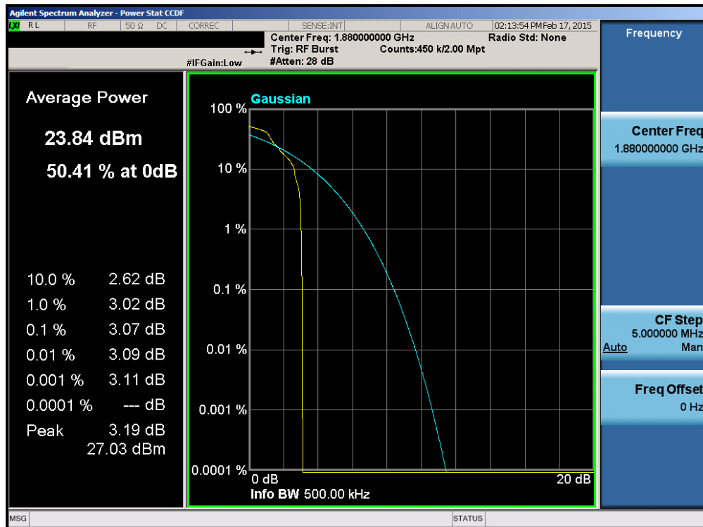
Plot 6-38. Peak-Average Ratio Plot (EDGE1900 Mode – Ch. 661)
