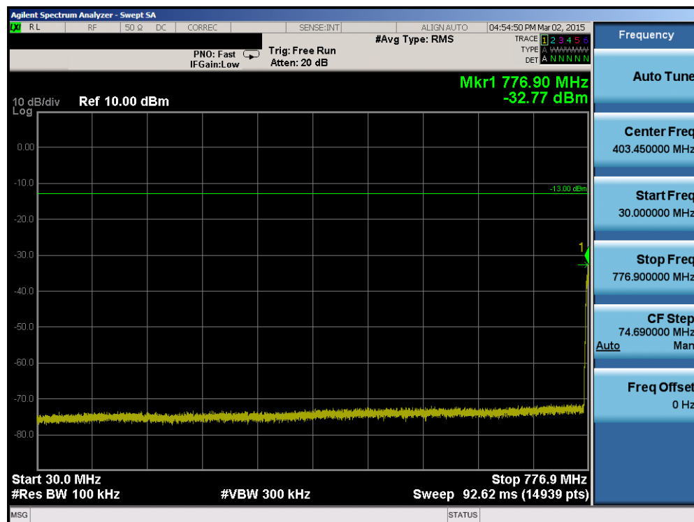
Plot 6-26. Conducted Spurious Plot (Band 13 – 5.0MHz QPSK – RB Size 1, RB Offset 0 – Low Channel)
