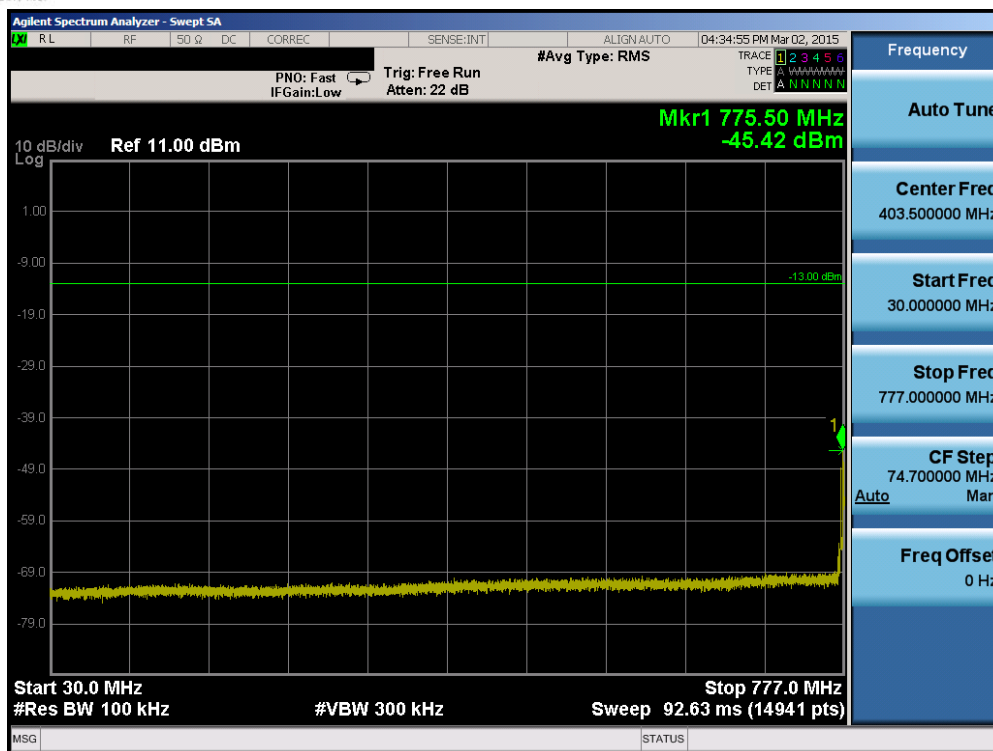
Plot 6-29. Conducted Spurious Plot (Band 13 – 5.0MHz QPSK – RB Size 1, RB Offset 0 – Mid Channel)
