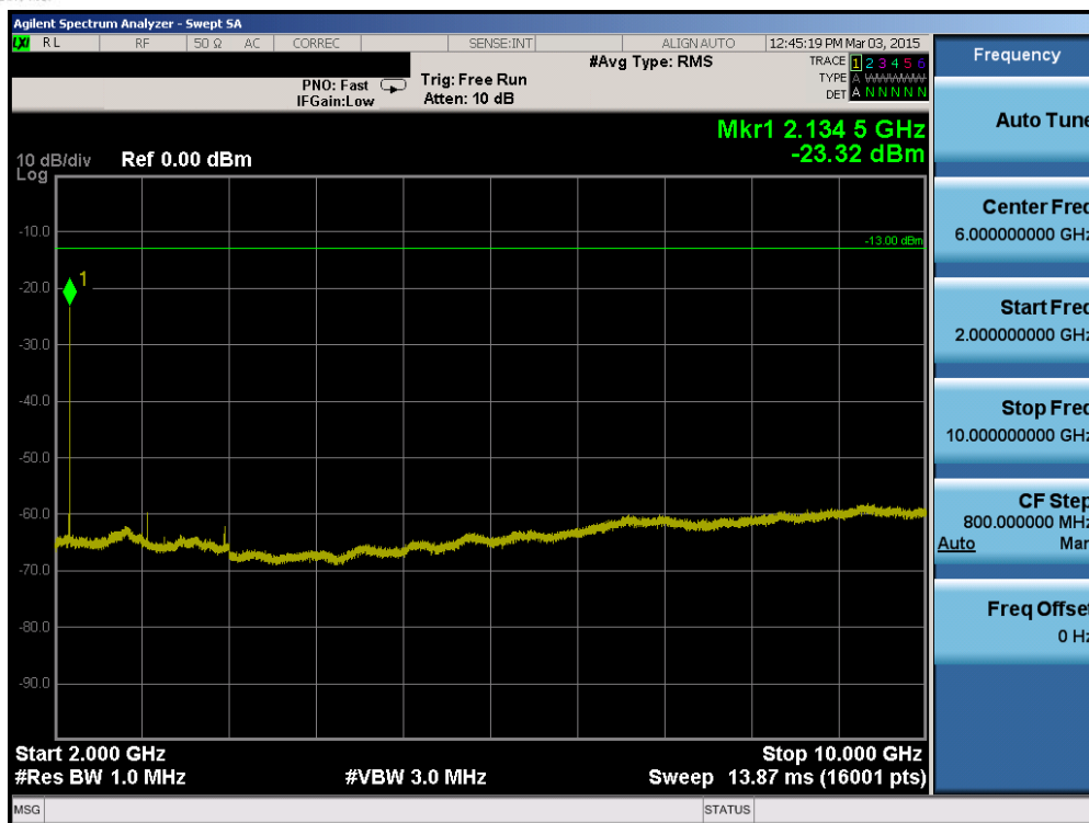
Plot 6-25. Conducted Spurious Plot (Band 17 – 5.0MHz QPSK – RB Size 1, RB Offset 0 – High Channel)
