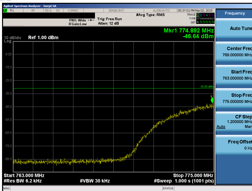
Plot 6-53. Lower Emission Mask Plot (Band 13 – 10.0MHz QPSK – RB Size 25)
