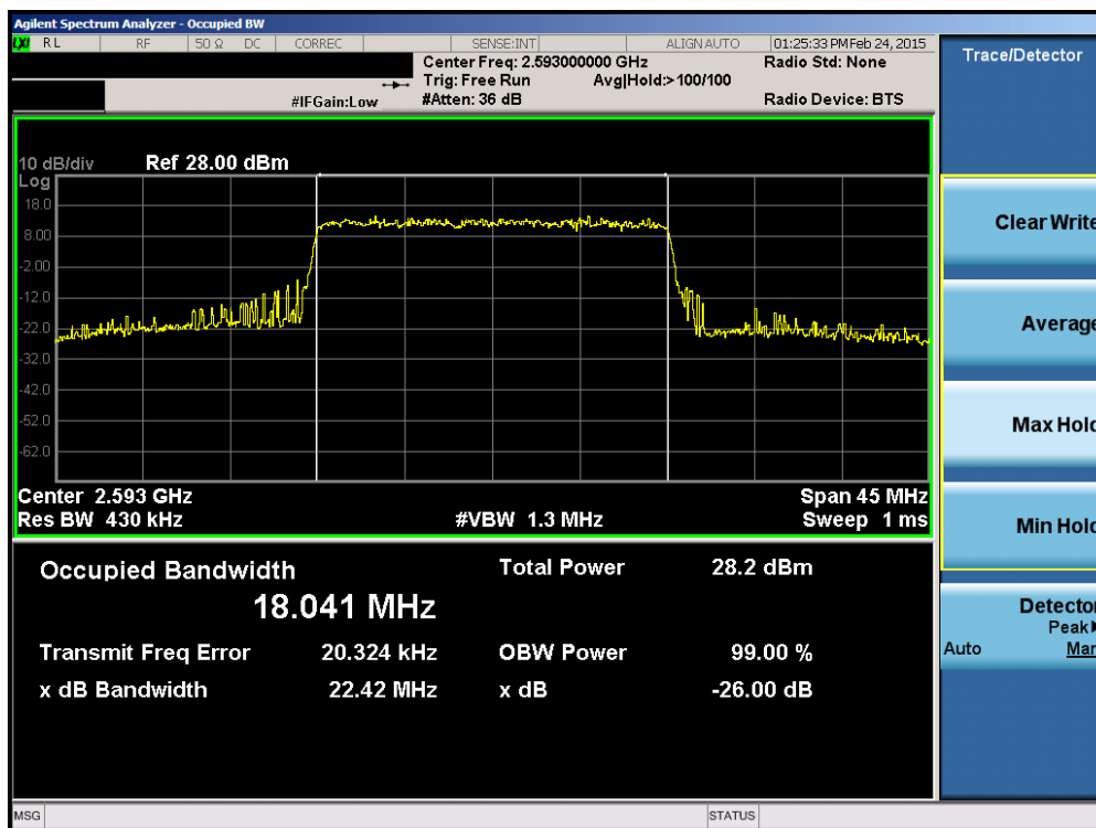
Plot 6-16. Occupied Bandwidth Plot (Band 41 – 20.0MHz 16-QAM – RB Size 100)
