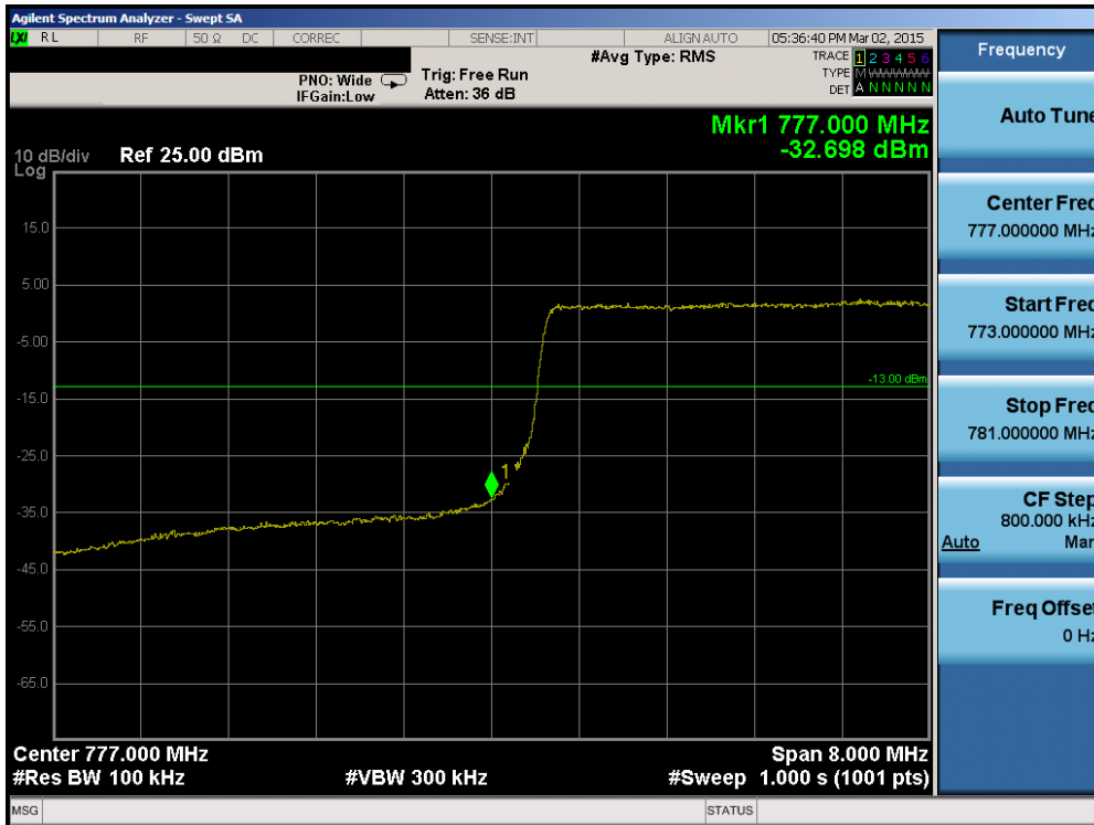
Plot 6-52. Lower Band Edge Plot (Band 13 – 10.0MHz QPSK – RB Size 50)
