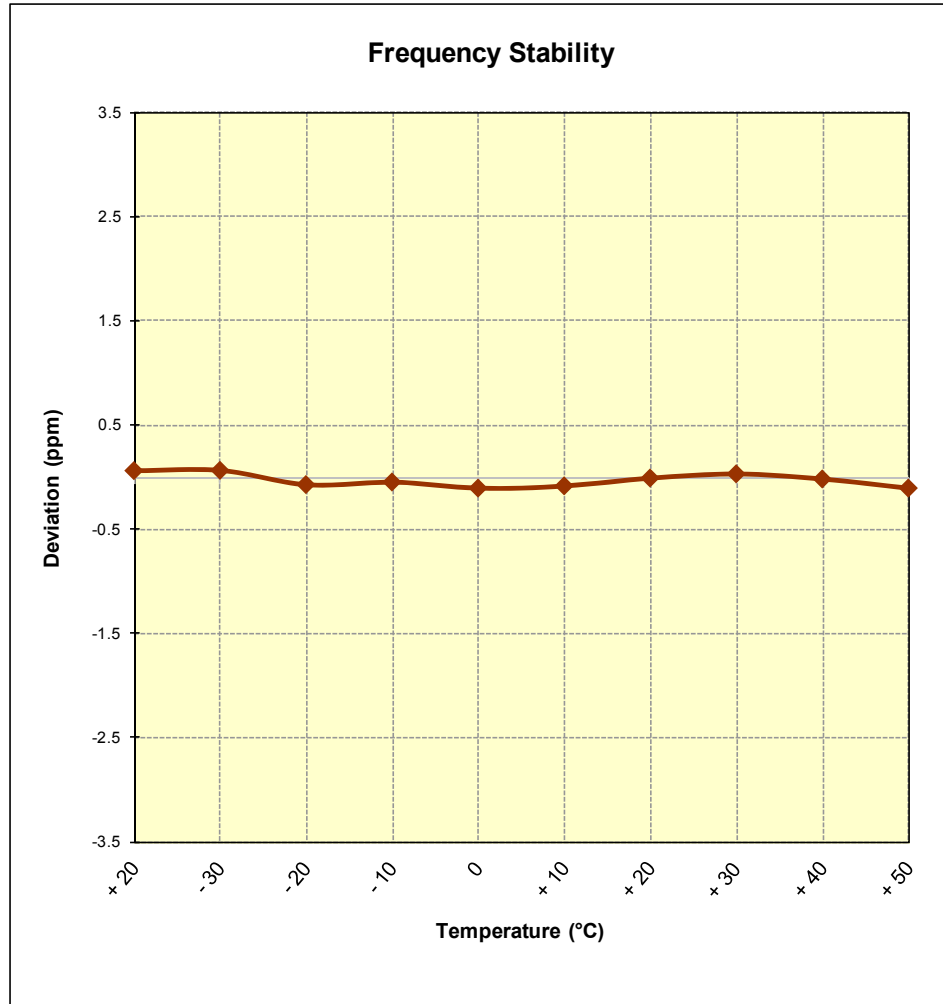
Figure 6-8. Frequency Stability Graph (Band 41)
