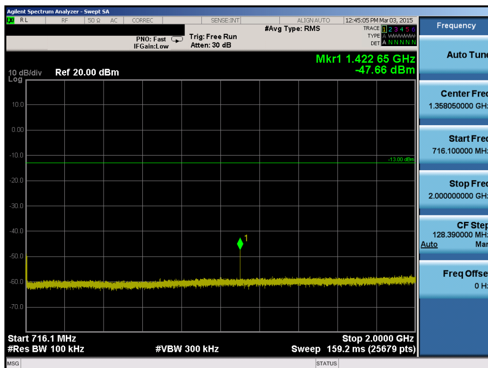
Plot 6-24. Conducted Spurious Plot (Band 17 – 5.0MHz QPSK – RB Size 1, RB Offset 0 – High Channel)
