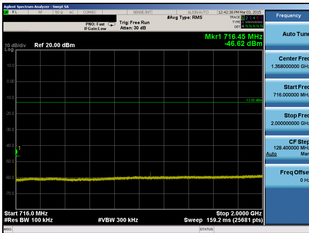
Plot 6-21. Conducted Spurious Plot (Band 17 – 5.0MHz QPSK – RB Size 1, RB Offset 0 – Mid Channel)
