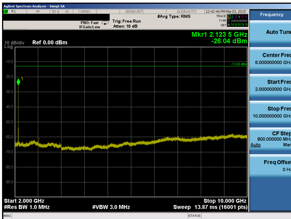
Plot 6-22. Conducted Spurious Plot (Band 17 – 5.0MHz QPSK – RB Size 1, RB Offset 0 – Mid Channel)
