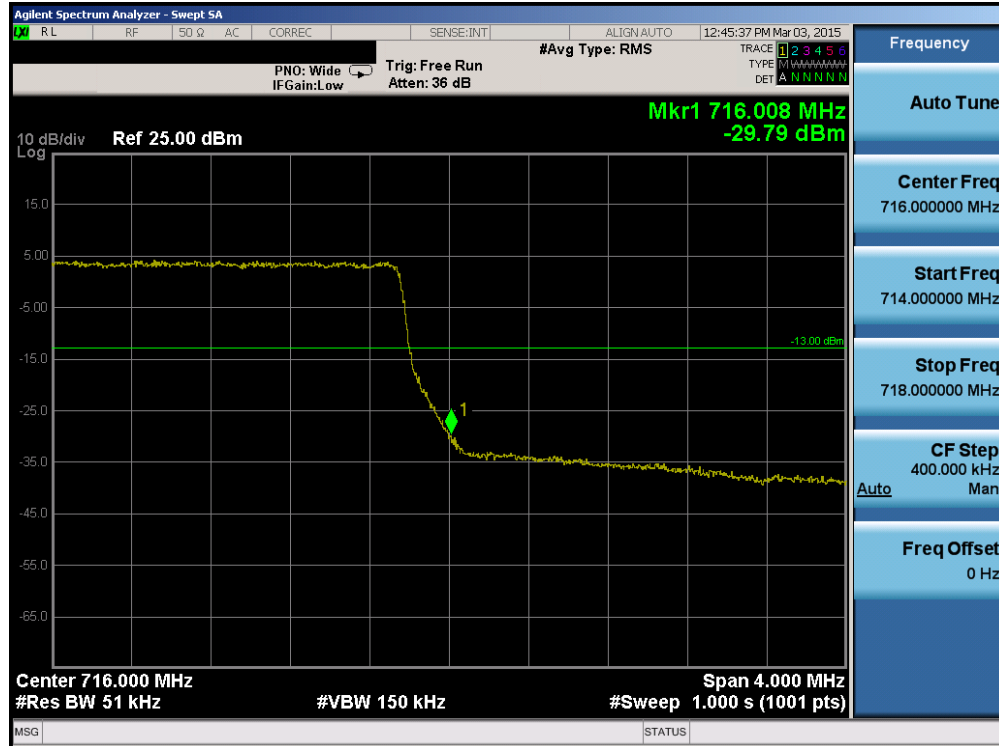
Plot 6-45. Upper Band Edge Plot (Band 17 – 5.0MHz QPSK – RB Size 25)
