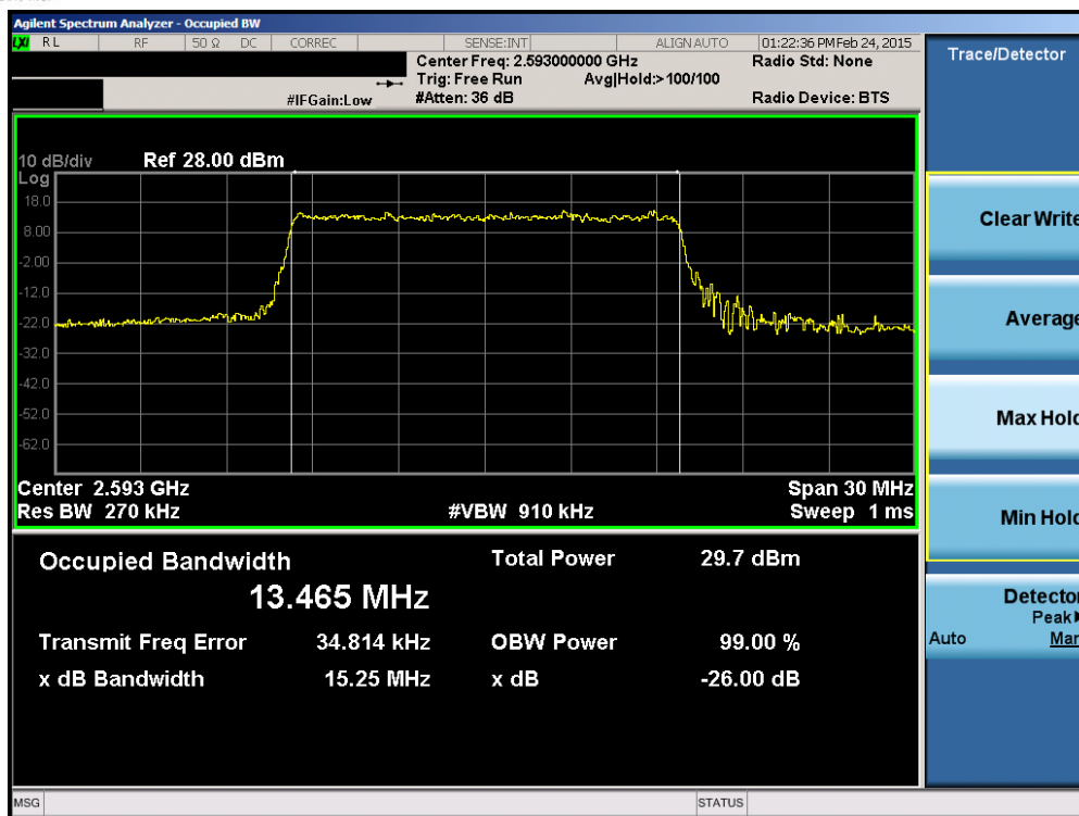
Plot 6-13. Occupied Bandwidth Plot (Band 41 – 15.0MHz QPSK – RB Size 75)
