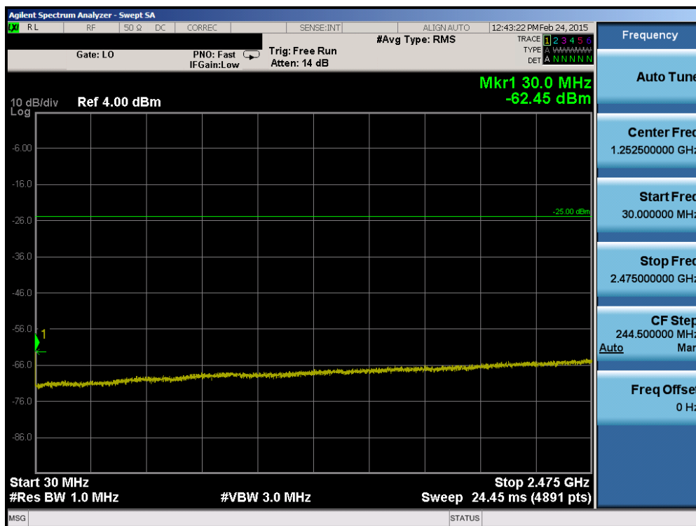
Plot 6-38. Conducted Spurious Plot (Band 41 – 5.0MHz QPSK – RB Size 1, RB Offset 0 – Mid Channel)
