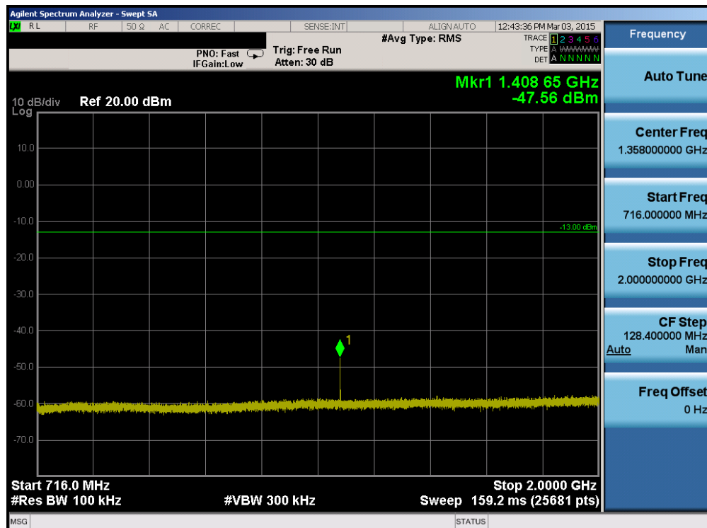
Plot 6-18. Conducted Spurious Plot (Band 17 – 5.0MHz QPSK – RB Size 1, RB Offset 0 – Low Channel)
