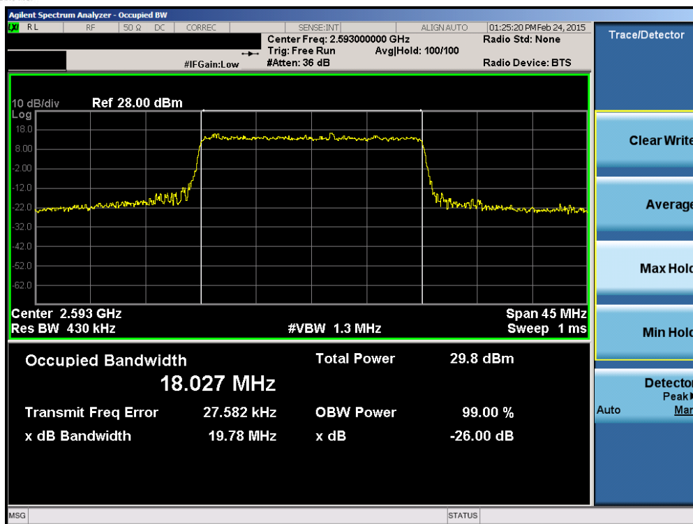
Plot 6-15. Occupied Bandwidth Plot (Band 41 – 20.0MHz QPSK – RB Size 100)
