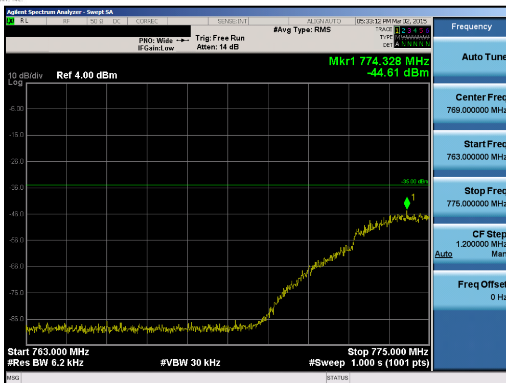
Plot 6-49. Lower Emission Mask Plot (Band 13 – 5.0MHz QPSK – RB Size 25)
