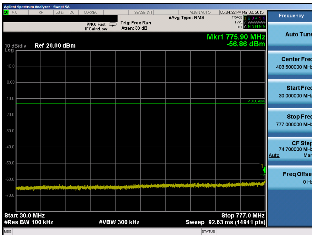
Plot 6-32. Conducted Spurious Plot (Band 13 – 5.0MHz QPSK – RB Size 1, RB Offset 0 – High Channel)
