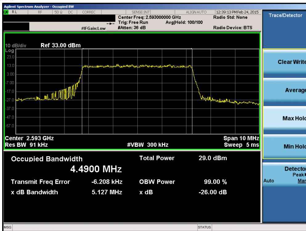
Plot 6-9. Occupied Bandwidth Plot (Band 41 – 5.0MHz QPSK – RB Size 25)
