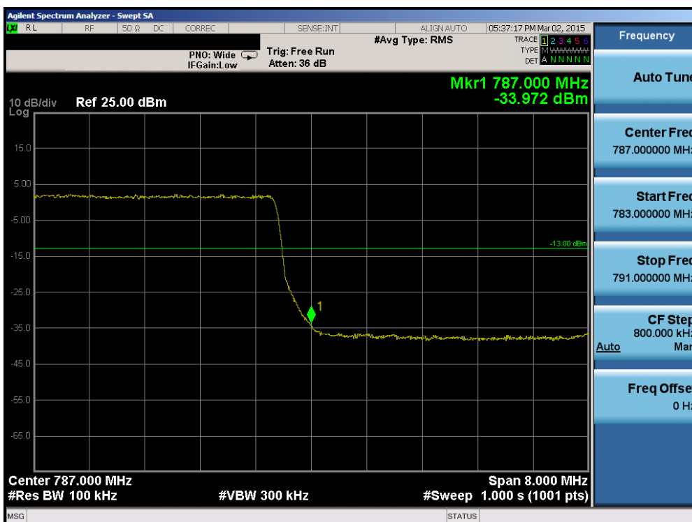
Plot 6-54. Upper Band Edge Plot (Band 13 – 10.0MHz QPSK – RB Size 50)
