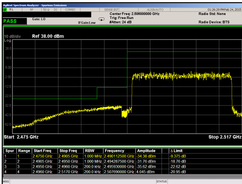
Plot 6-62. Lower ACP Plot (Band 41 – 20.0MHz QPSK – RB Size 100)
