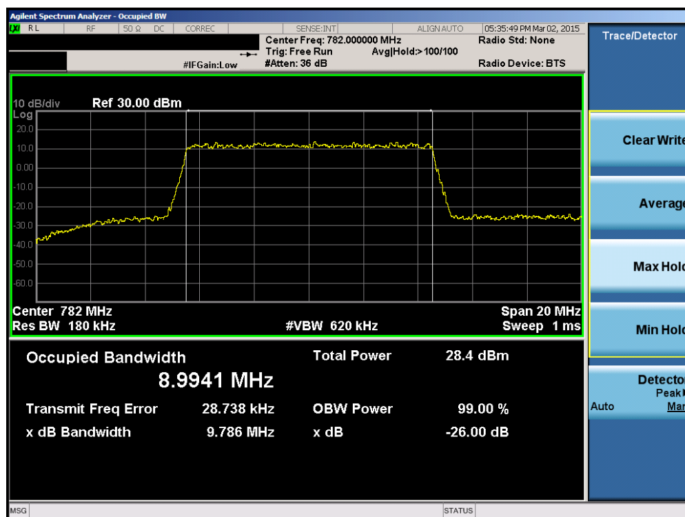
Plot 6-8. Occupied Bandwidth Plot (Band 13 – 10.0MHz 16-QAM – RB Size 50)
