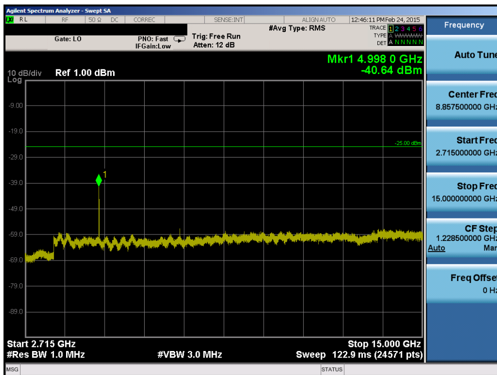
Plot 6-36. Conducted Spurious Plot (Band 41 – 5.0MHz QPSK – RB Size 1, RB Offset 0 – Low Channel)
