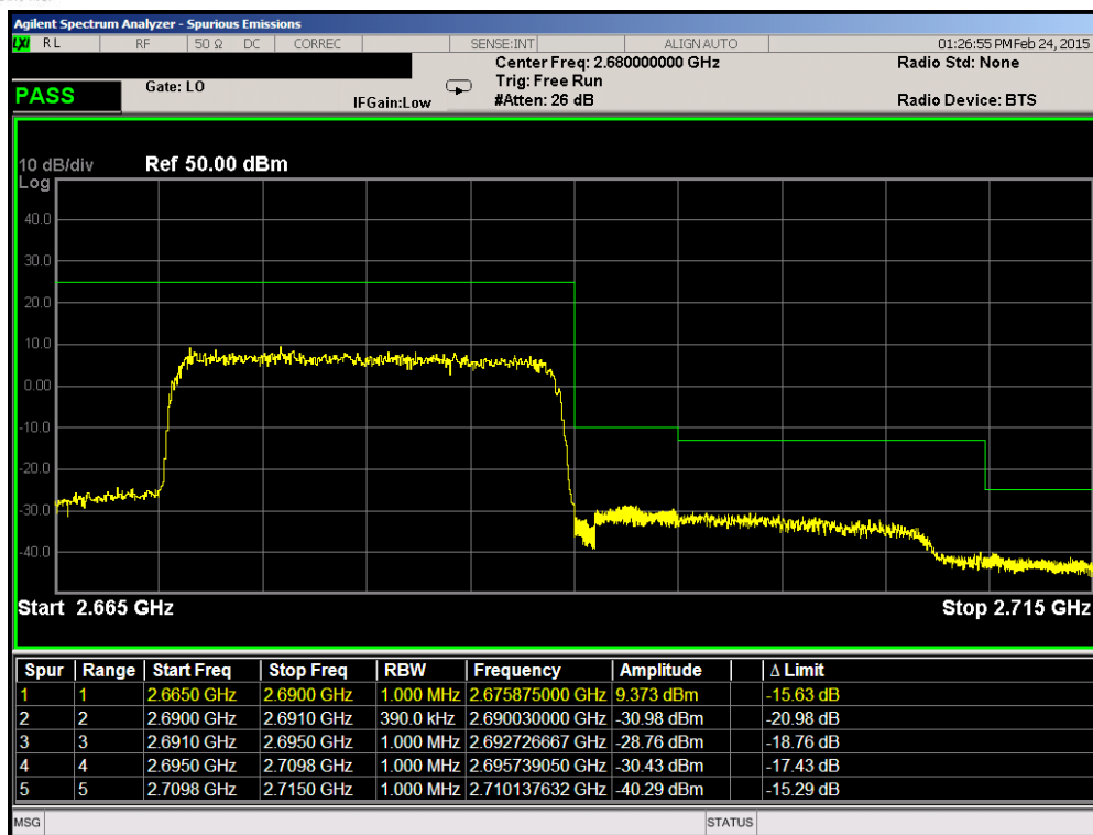
Plot 6-63. Upper ACP Plot (Band 41 – 20.0MHz QPSK – RB Size 100)
