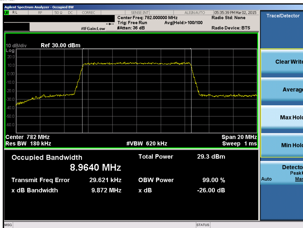
Plot 6-7. Occupied Bandwidth Plot (Band 13 – 10.0MHz QPSK – RB Size 50)
