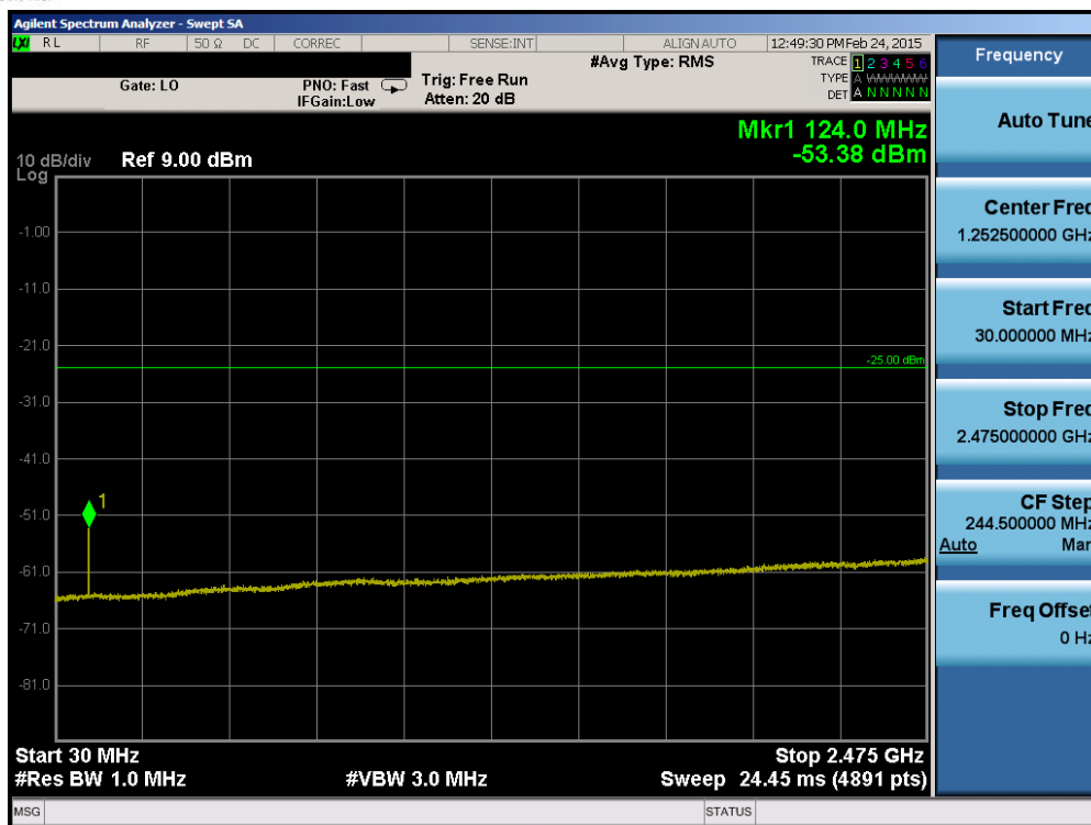
Plot 6-41. Conducted Spurious Plot (Band 41 – 5.0MHz QPSK – RB Size 1, RB Offset 0 – High Channel)
