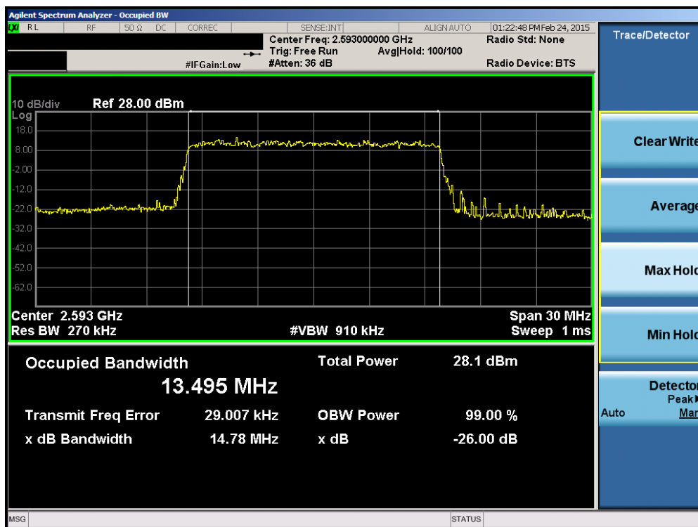
Plot 6-14. Occupied Bandwidth Plot (Band 41 – 15.0MHz 16-QAM – RB Size 75)
