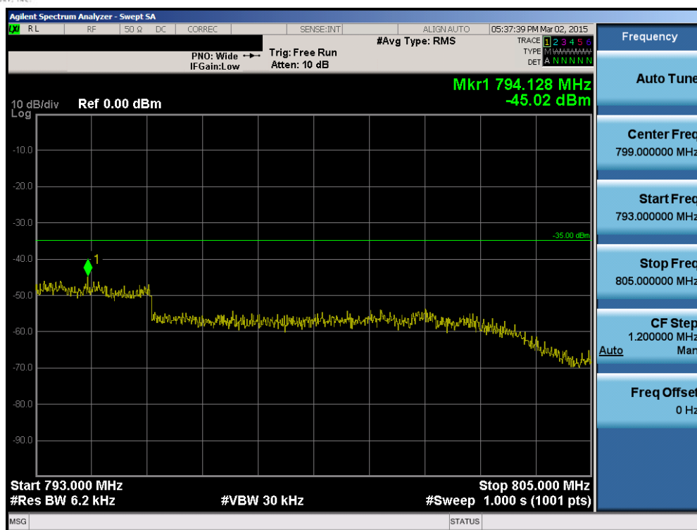
Plot 6-55. Upper Emission Mask Plot (Band 13 – 10.0MHz QPSK – RB Size 25)
