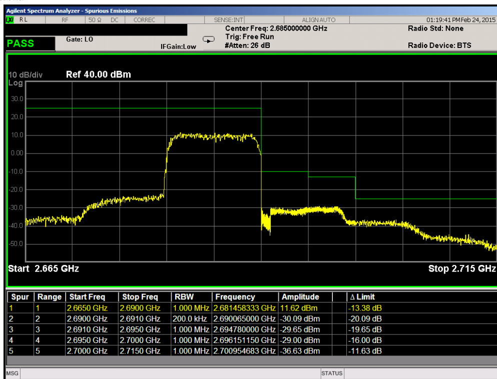
Plot 6-59. Upper ACP Plot (Band 41 – 10.0MHz QPSK – RB Size 50)
