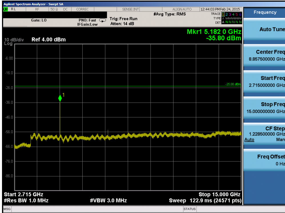
Plot 6-39. Conducted Spurious Plot (Band 41 – 5.0MHz QPSK – RB Size 1, RB Offset 0 – Mid Channel)
