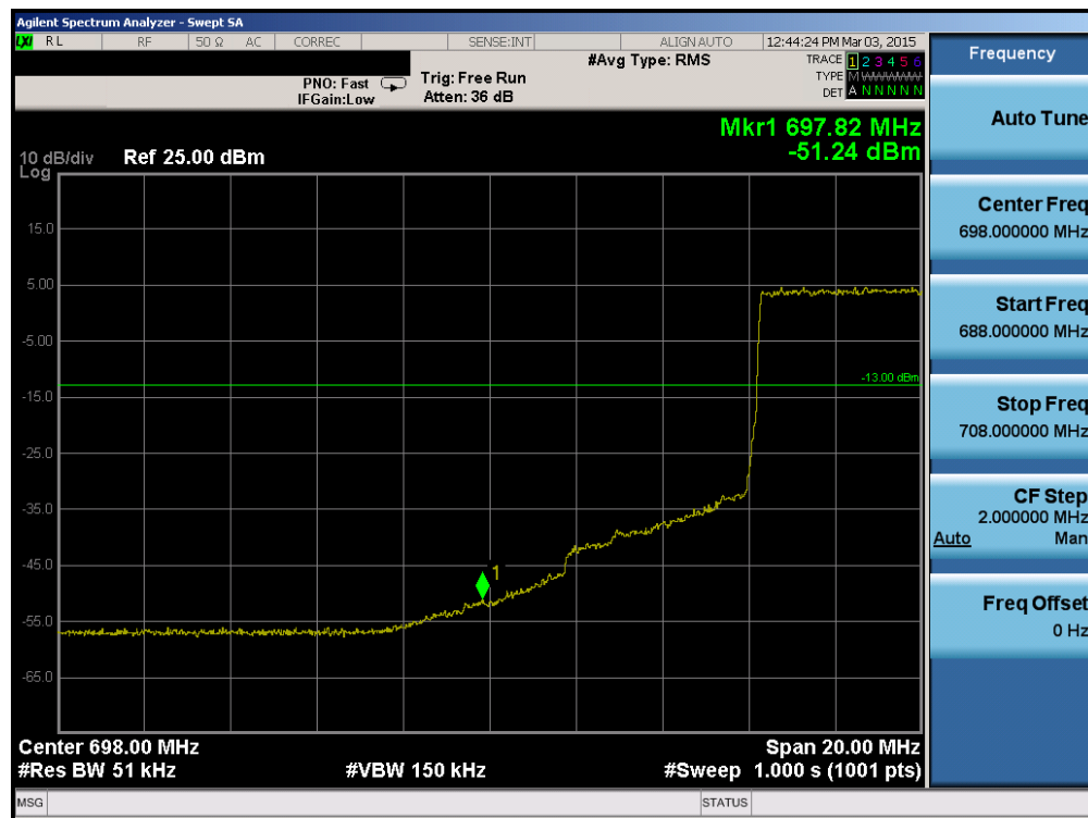
Plot 6-44. Lower Band Edge Plot (Band 17 – 5.0MHz QPSK – RB Size 25)
