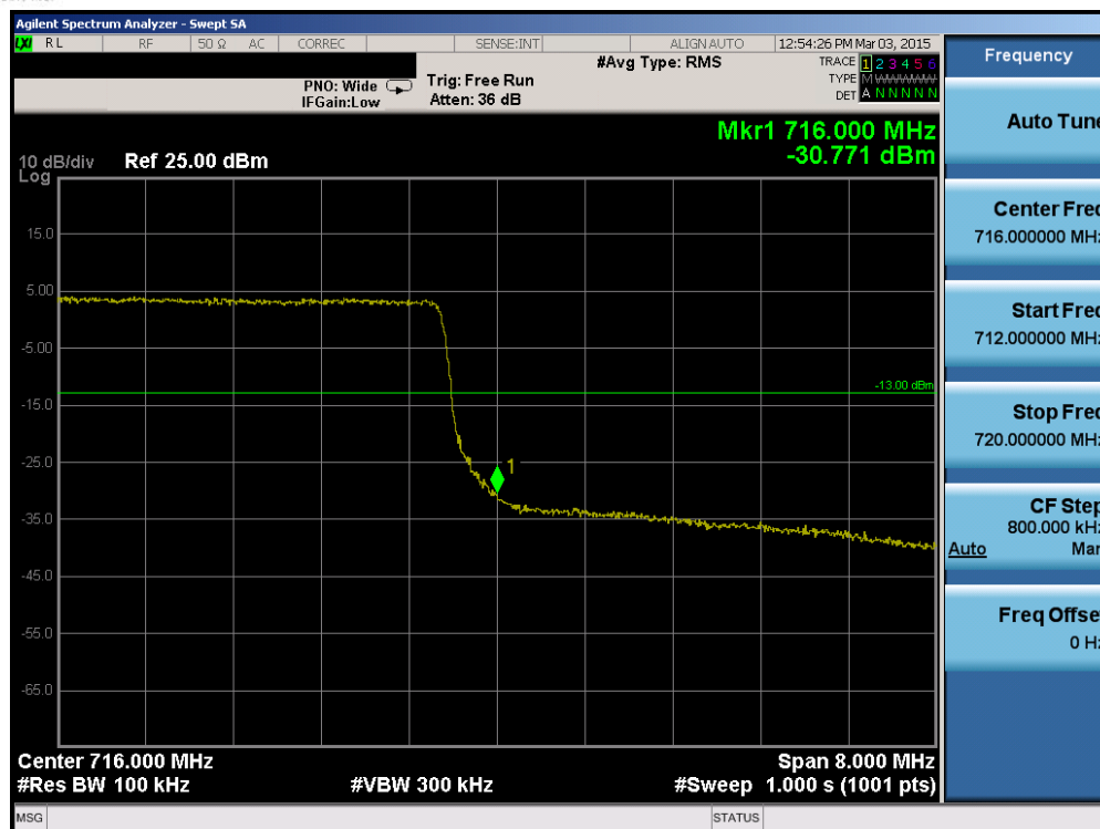
Plot 6-47. Upper Band Edge Plot (Band 17 – 10.0MHz QPSK – RB Size 50)
