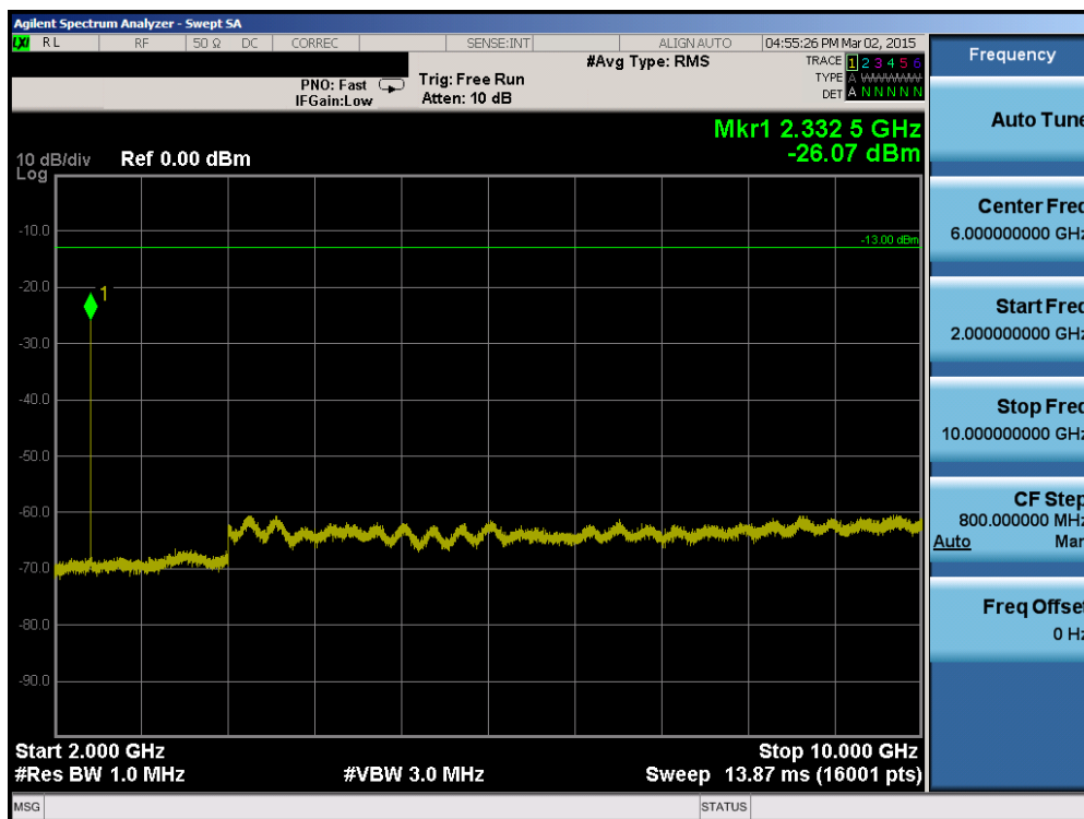
Plot 6-28. Conducted Spurious Plot (Band 13 – 5.0MHz QPSK – RB Size 1, RB Offset 0 – Low Channel)
