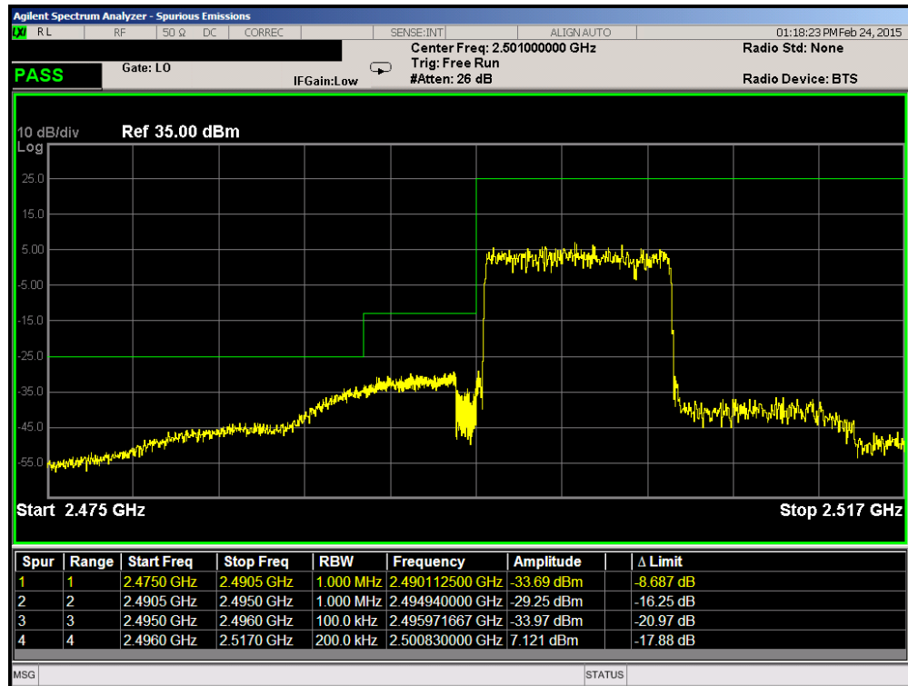
Plot 6-58. Lower ACP Plot (Band 41 – 10.0MHz QPSK – RB Size 50)
