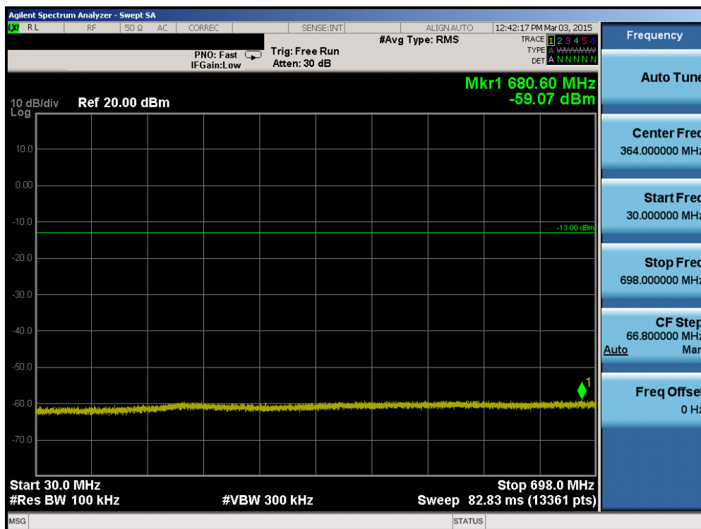
Plot 6-20. Conducted Spurious Plot (Band 17 – 5.0MHz QPSK – RB Size 1, RB Offset 0 – Mid Channel)
