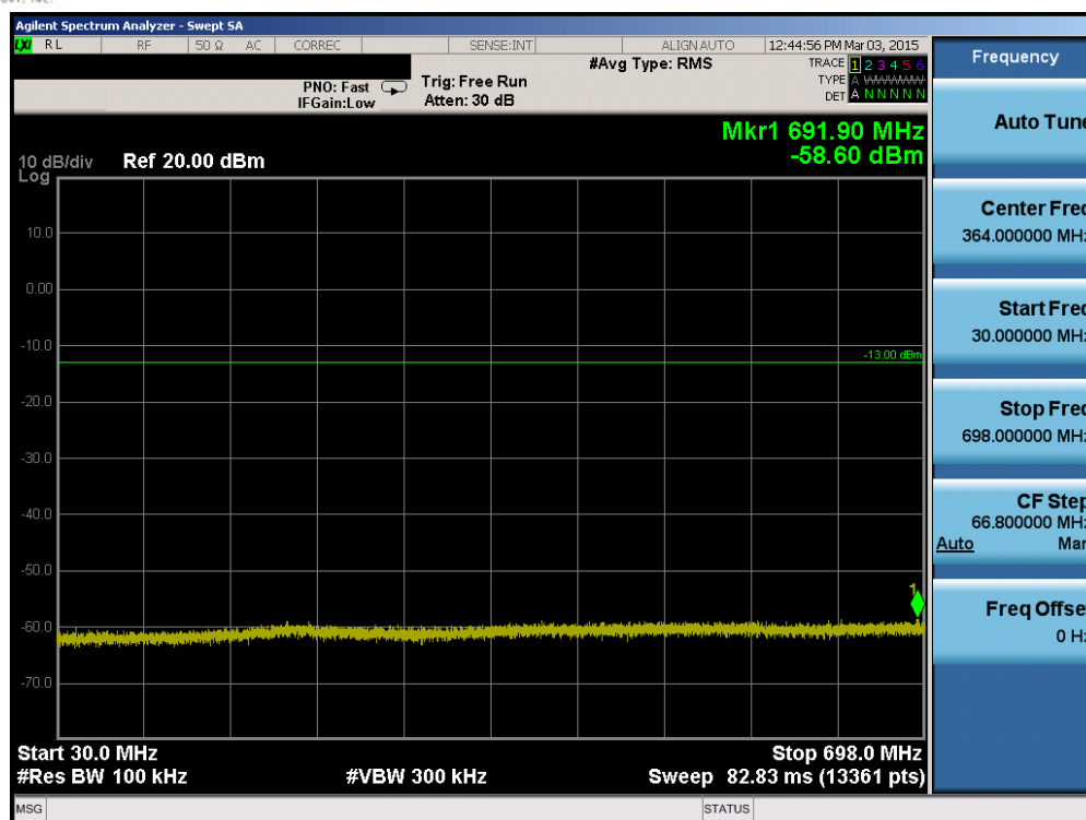
Plot 6-23. Conducted Spurious Plot (Band 17 – 5.0MHz QPSK – RB Size 1, RB Offset 0 – High Channel)
