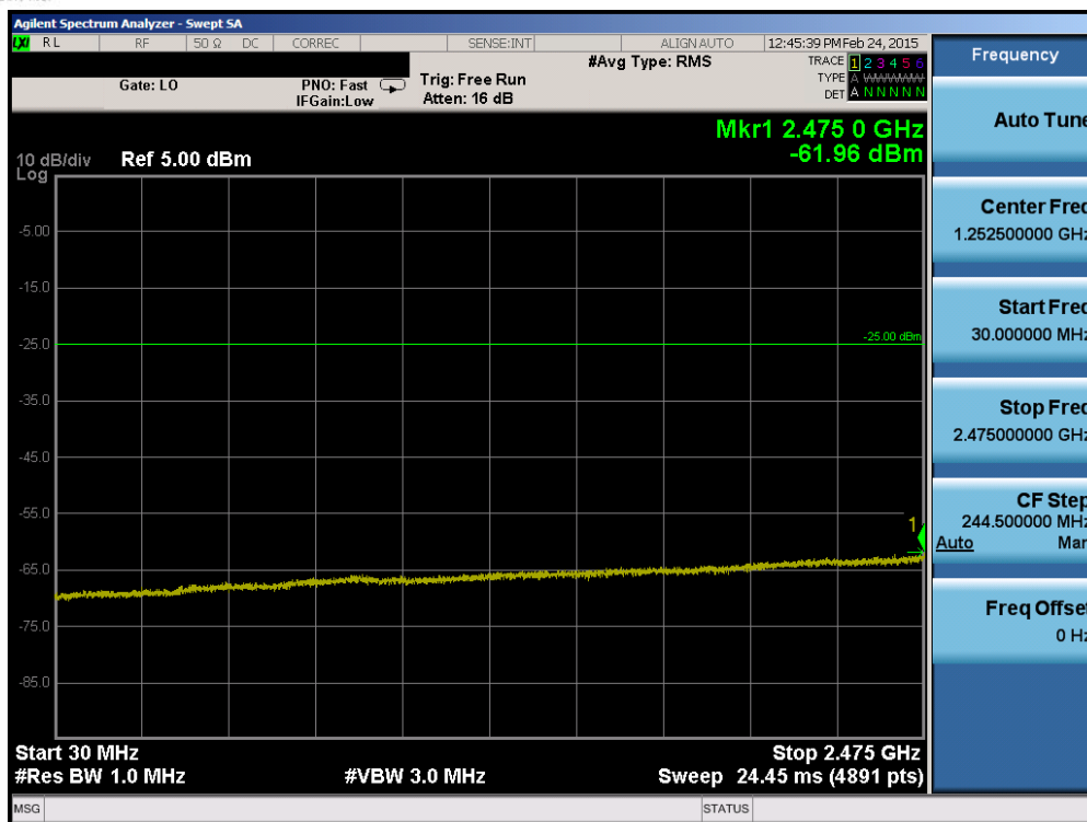
Plot 6-35. Conducted Spurious Plot (Band 41 – 5.0MHz QPSK – RB Size 1, RB Offset 0 – Low Channel)
