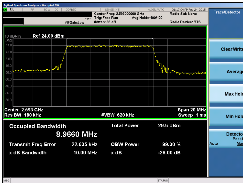
Plot 6-11. Occupied Bandwidth Plot (Band 41 – 10.0MHz QPSK – RB Size 50)
