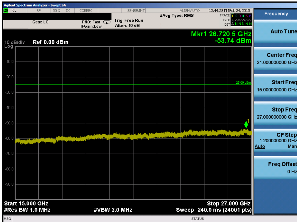
Plot 6-40. Conducted Spurious Plot (Band 41 – 5.0MHz QPSK – RB Size 1, RB Offset 0 – Mid Channel)
