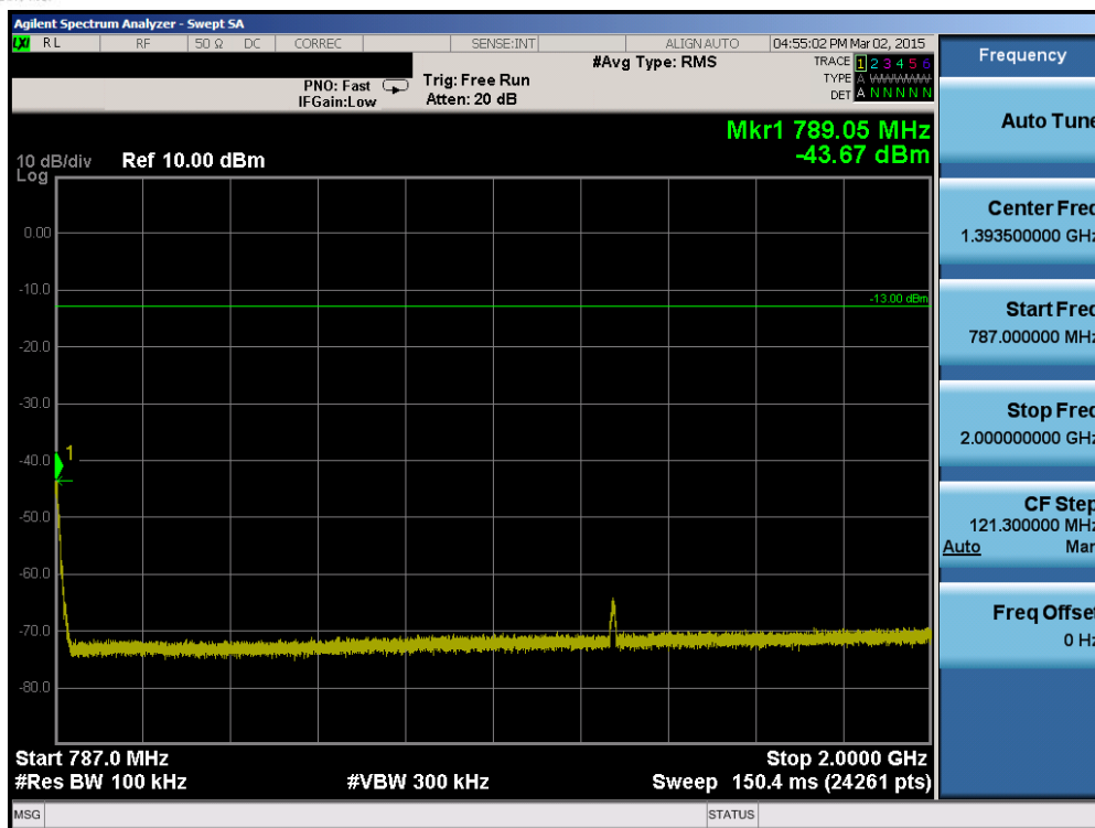
Plot 6-27. Conducted Spurious Plot (Band 13 – 5.0MHz QPSK – RB Size 1, RB Offset 0 – Low Channel)
