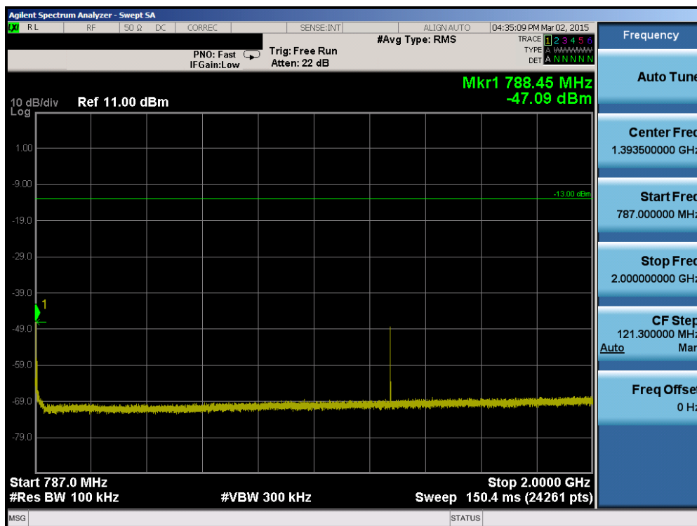
Plot 6-30. Conducted Spurious Plot (Band 13 – 5.0MHz QPSK – RB Size 1, RB Offset 0 – Mid Channel)
