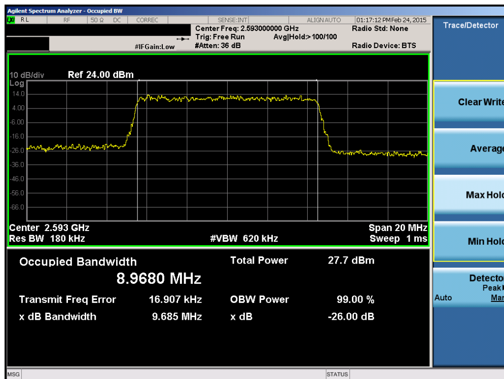
Plot 6-12. Occupied Bandwidth Plot (Band 41 – 10.0MHz 16-QAM – RB Size 50)
