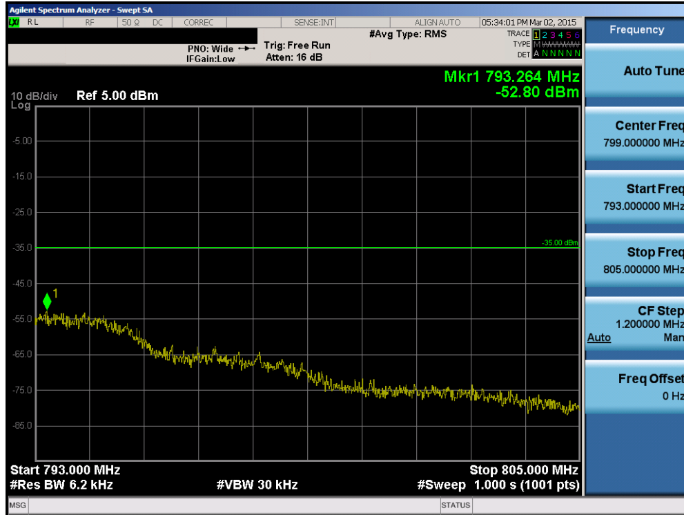
Plot 6-51. Upper Emission Mask Plot (Band 13 – 5.0MHz QPSK – RB Size 25)
