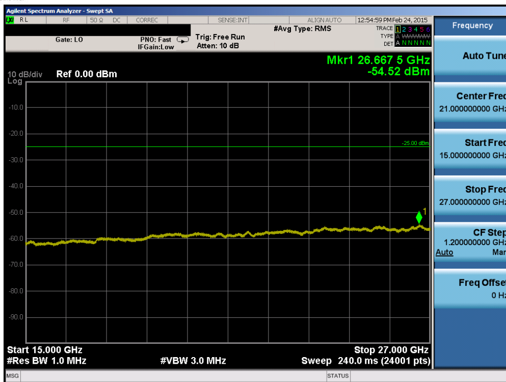
Plot 6-43. Conducted Spurious Plot (Band 41 – 5.0MHz QPSK – RB Size 1, RB Offset 0 – High Channel)
