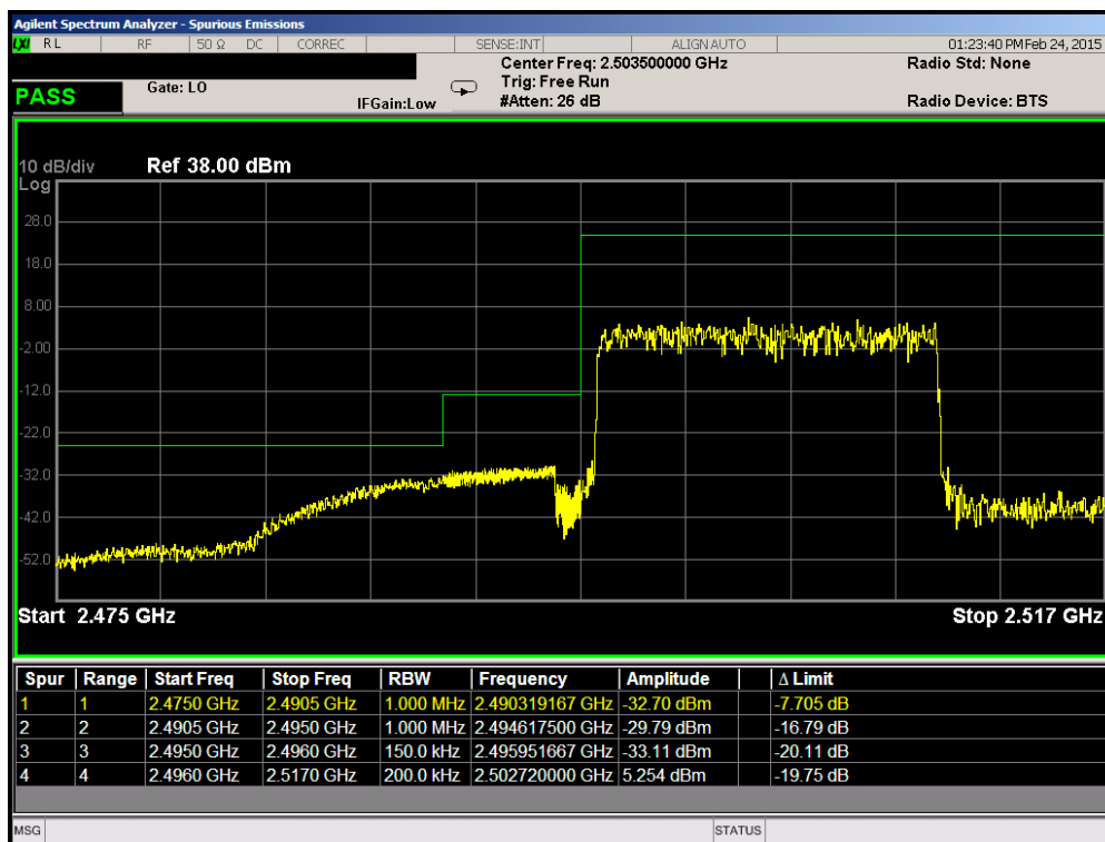
Plot 6-60. Lower ACP Plot (Band 41 – 15.0MHz QPSK – RB Size 75)
