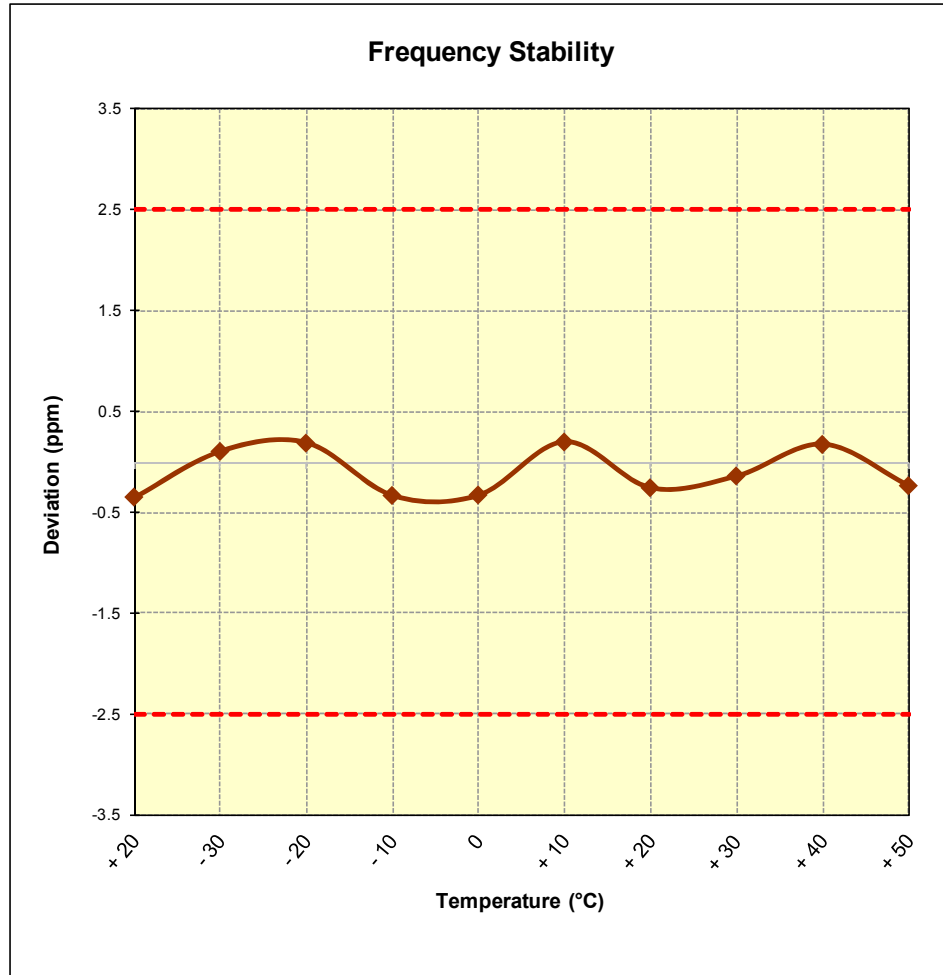
Figure 6-7. Frequency Stability Graph (Band 13)
