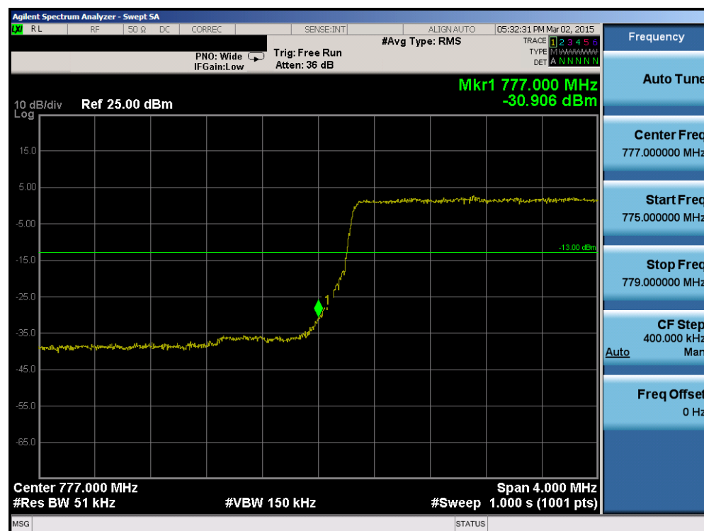
Plot 6-48. Lower Band Edge Plot (Band 13 – 5.0MHz QPSK – RB Size 25)
