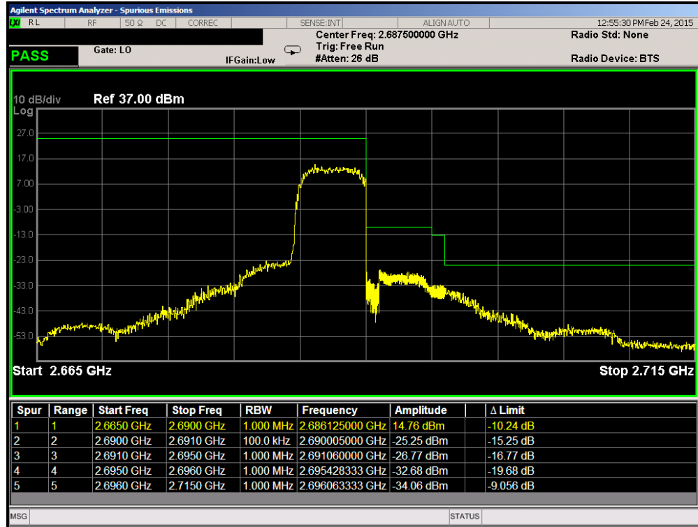
Plot 6-57. Upper ACP Plot (Band 41 – 5.0MHz QPSK – RB Size 25)
