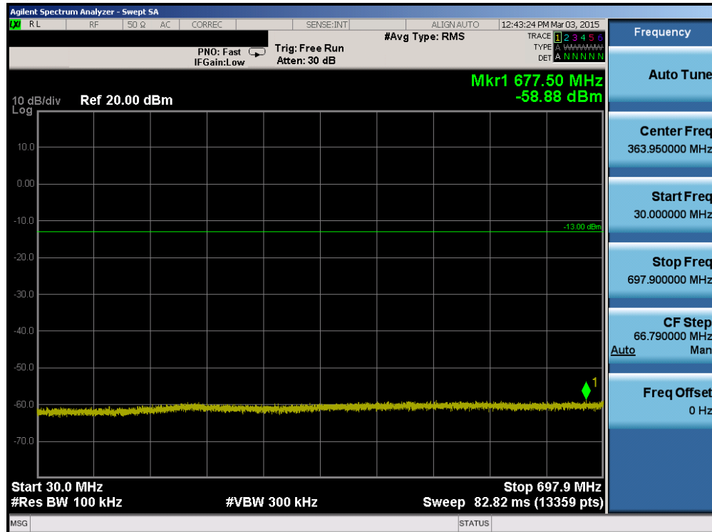
Plot 6-17. Conducted Spurious Plot (Band 17 – 5.0MHz QPSK – RB Size 1, RB Offset 0 – Low Channel)
