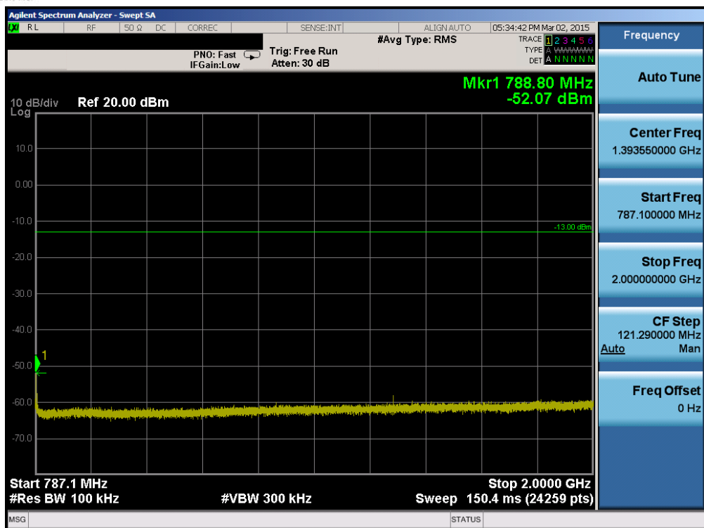
Plot 6-33. Conducted Spurious Plot (Band 13 – 5.0MHz QPSK – RB Size 1, RB Offset 0 – High Channel)
