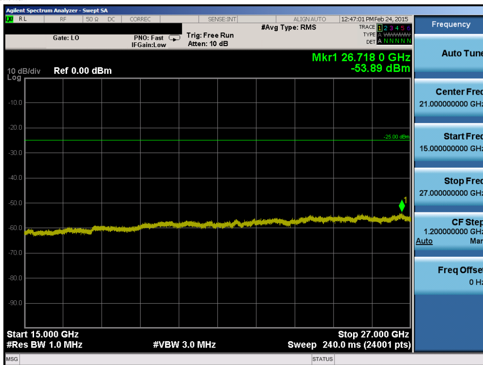
Plot 6-37. Conducted Spurious Plot (Band 41 – 5.0MHz QPSK – RB Size 1, RB Offset 0 – Low Channel)
