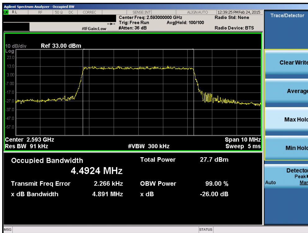
Plot 6-10. Occupied Bandwidth Plot (Band 41 – 5.0MHz 16-QAM – RB Size 25)
