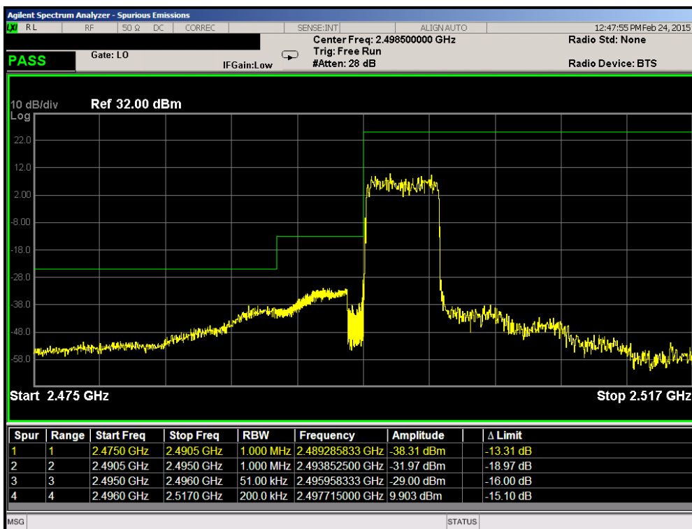
Plot 6-56. Lower ACP Plot (Band 41 – 5.0MHz QPSK – RB Size 25)
