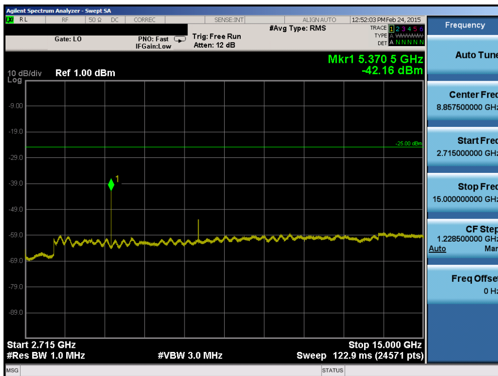
Plot 6-42. Conducted Spurious Plot (Band 41 – 5.0MHz QPSK – RB Size 1, RB Offset 0 – High Channel)
