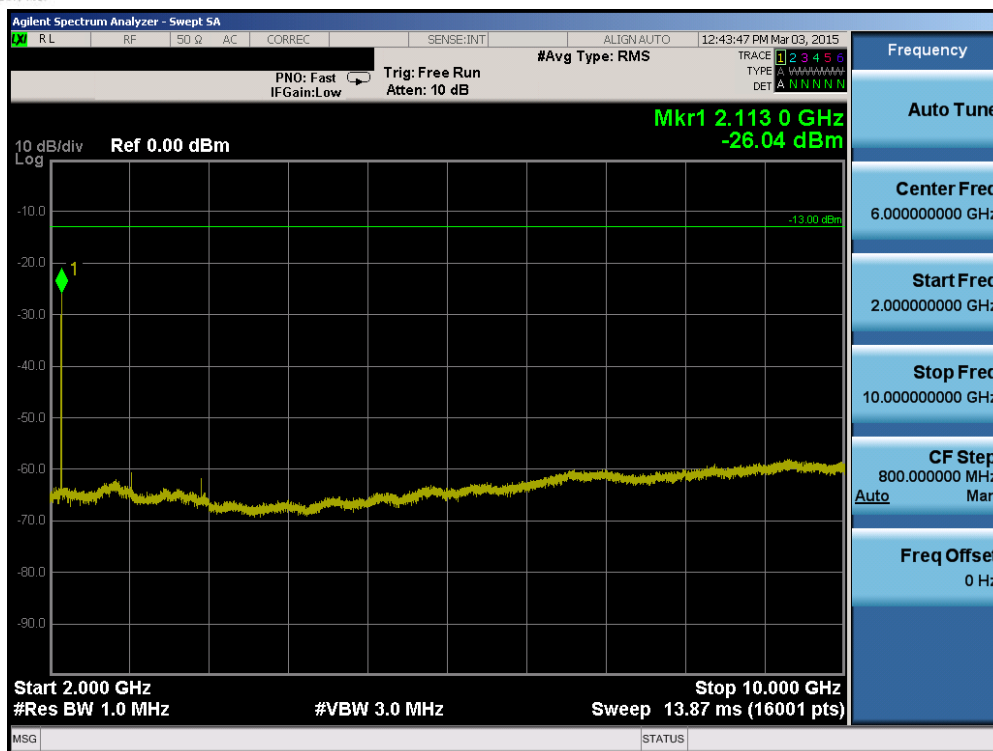
Plot 6-19. Conducted Spurious Plot (Band 17 – 5.0MHz QPSK – RB Size 1, RB Offset 0 – Low Channel)
