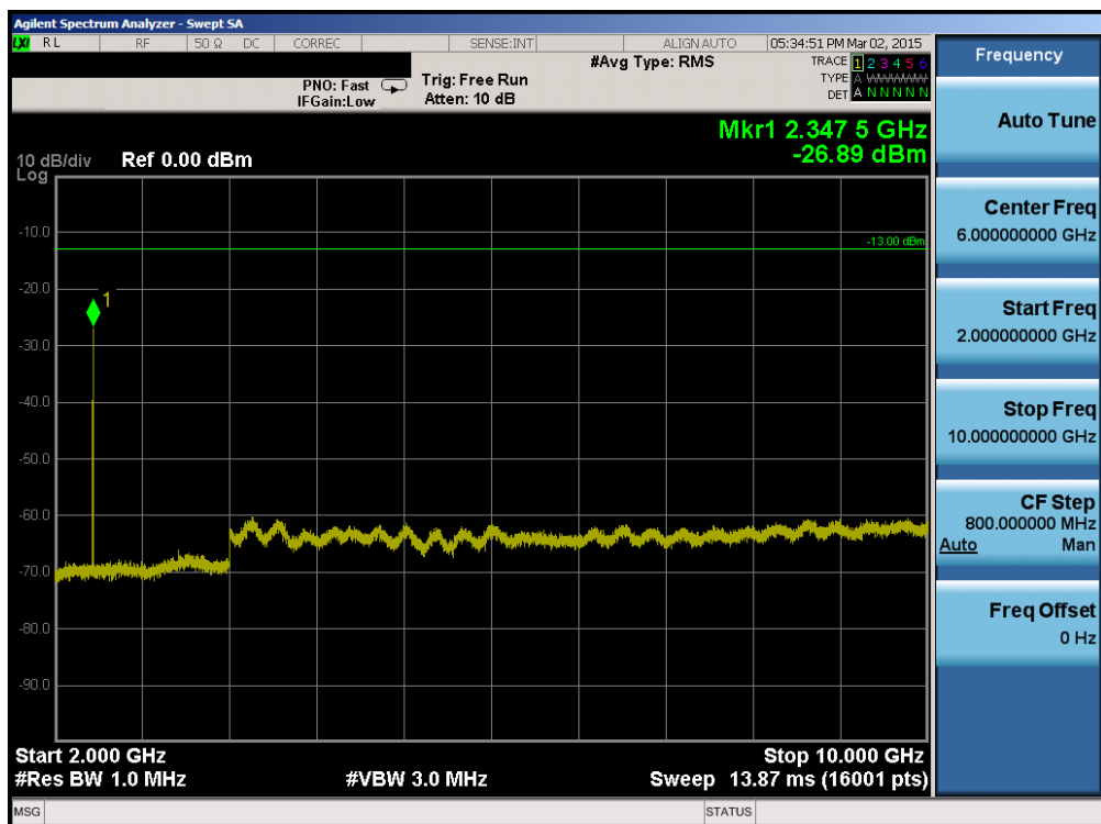
Plot 6-34. Conducted Spurious Plot (Band 13 – 5.0MHz QPSK – RB Size 1, RB Offset 0 – High Channel)
