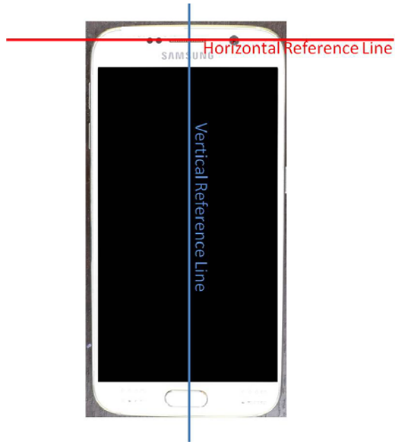
SAR Test Setup Photo 11 – Vertical & Horizontal Reference Lines.
