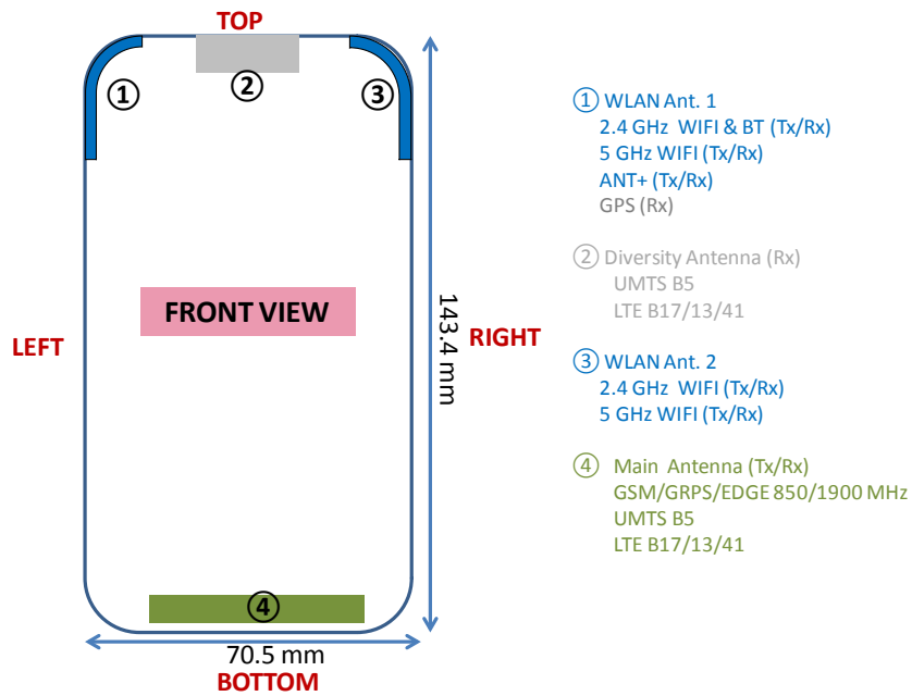
Figure F-1 DUT Antenna Locations
