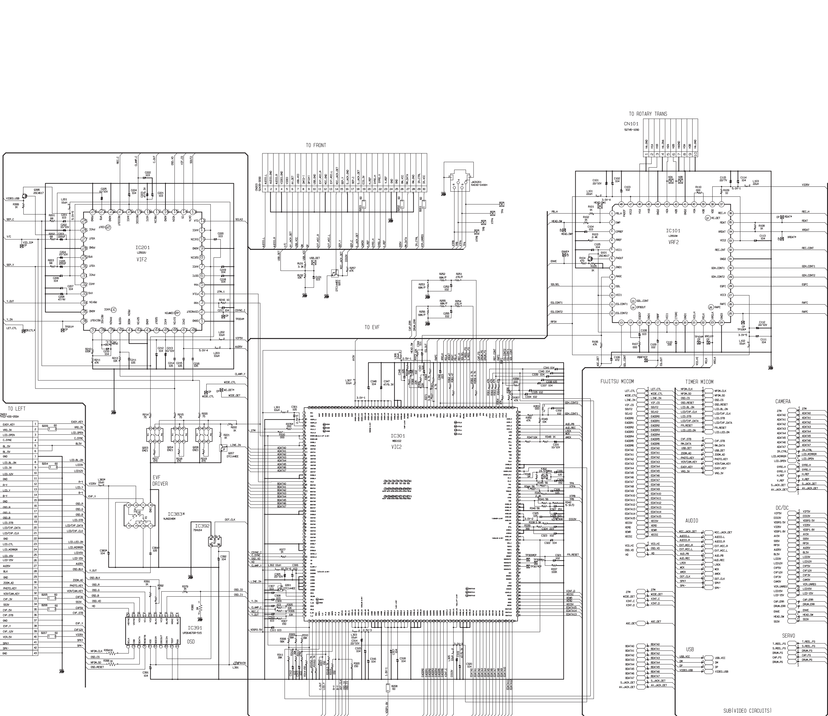
SUB(VIDEO CIRCUITS)
