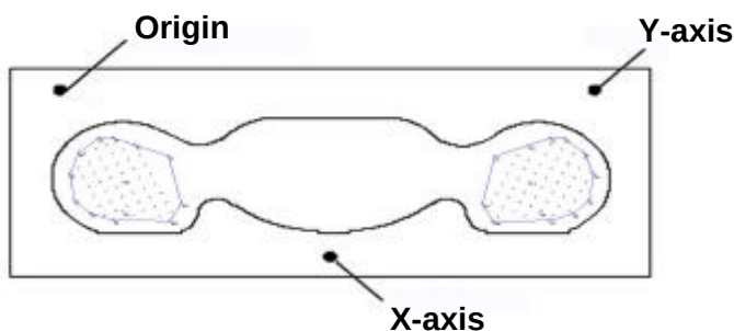
Fig 10. SAR Measurement Points in Area Scan
