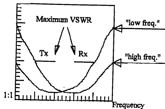
Figure 3.4.1 Reference antennas defining the lowest and highest allowable resonance frequencies for a single band antenna.
