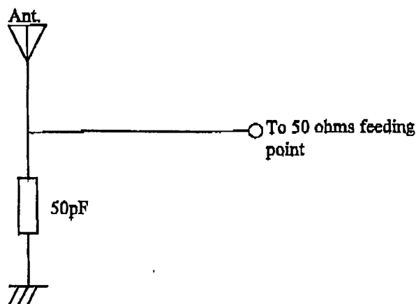
Figure 3.3.1 Matching circuit
