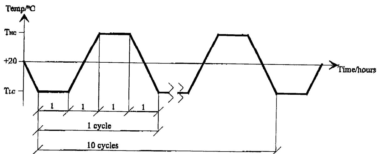
Figure 5.2.1 Temperature cycling
