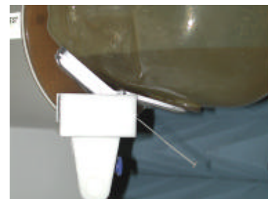
Figure 16. Head SAR Test Setup
