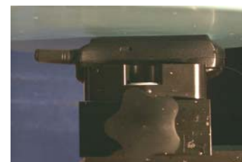
Figure 15. Shirt Pocket Configuration
