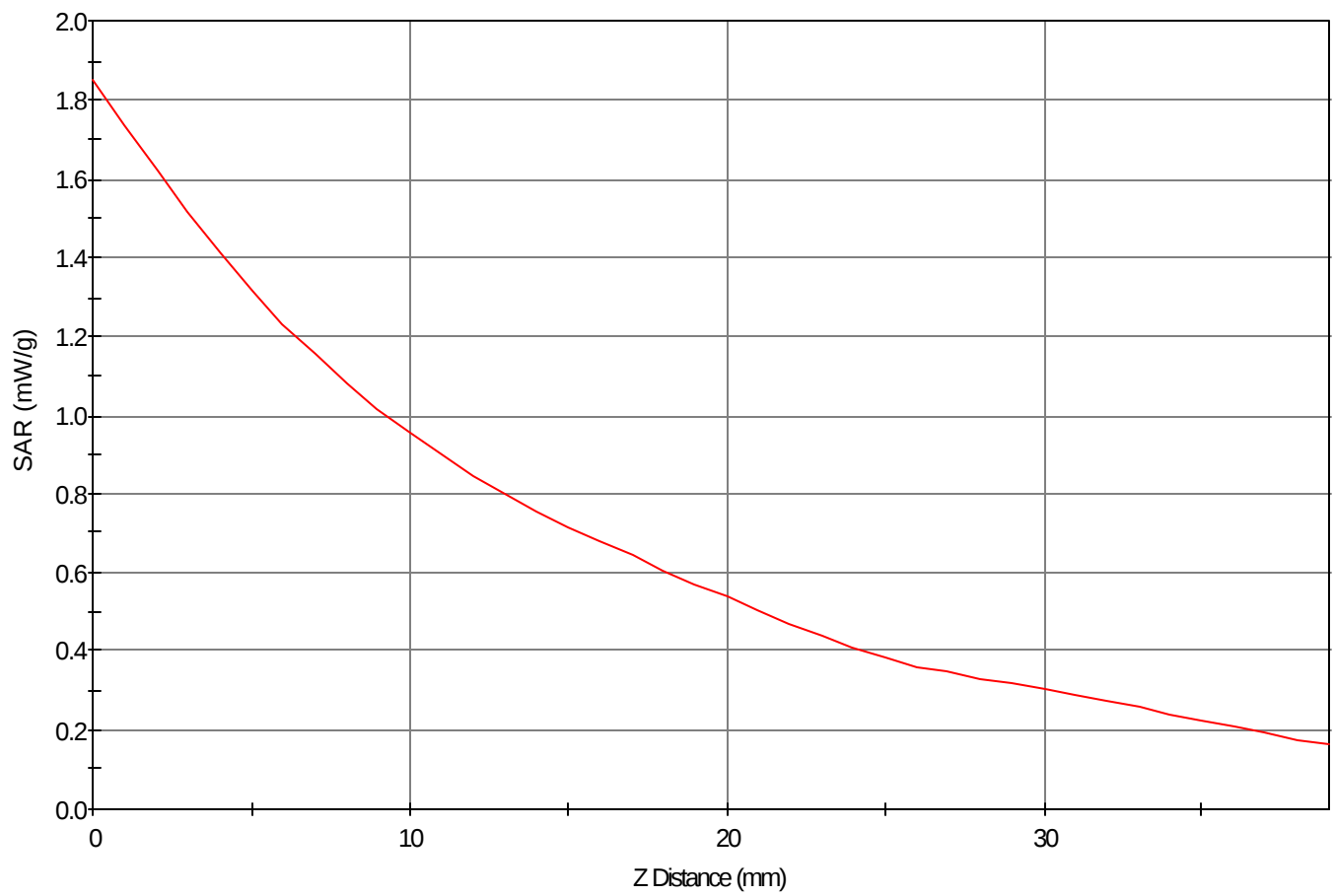
SAR - Z Axis at Hotspot x:68.0 y:12.0
