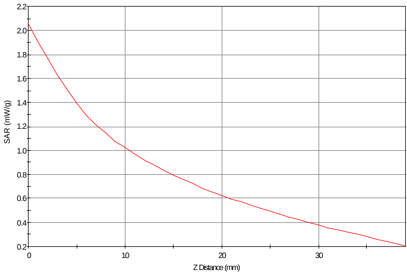
SAR - Z Axis at Hotspot x:62.0 y:12.0
