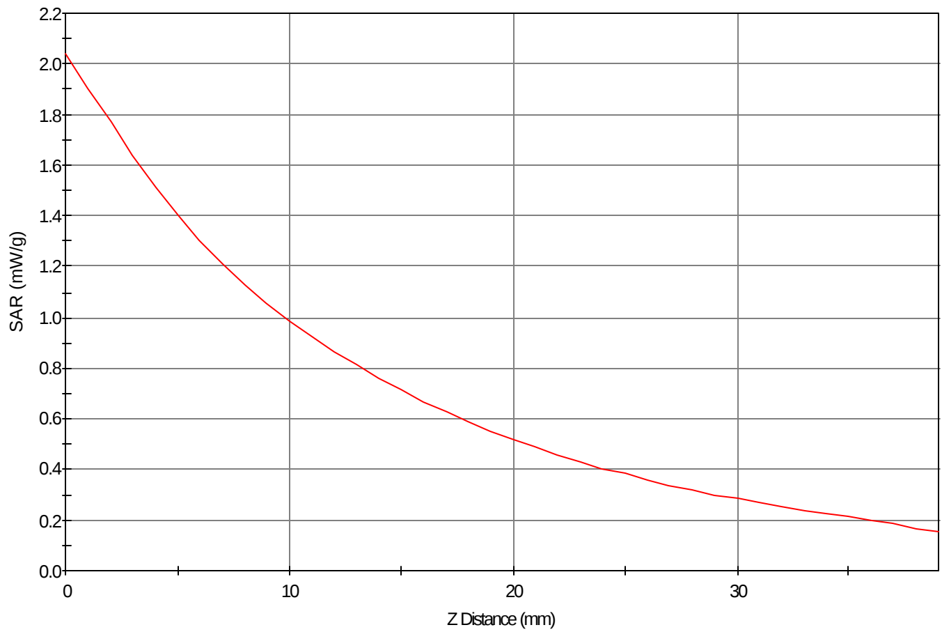
SAR - Z Axis at Hotspot x:2.0 y:-8.0
