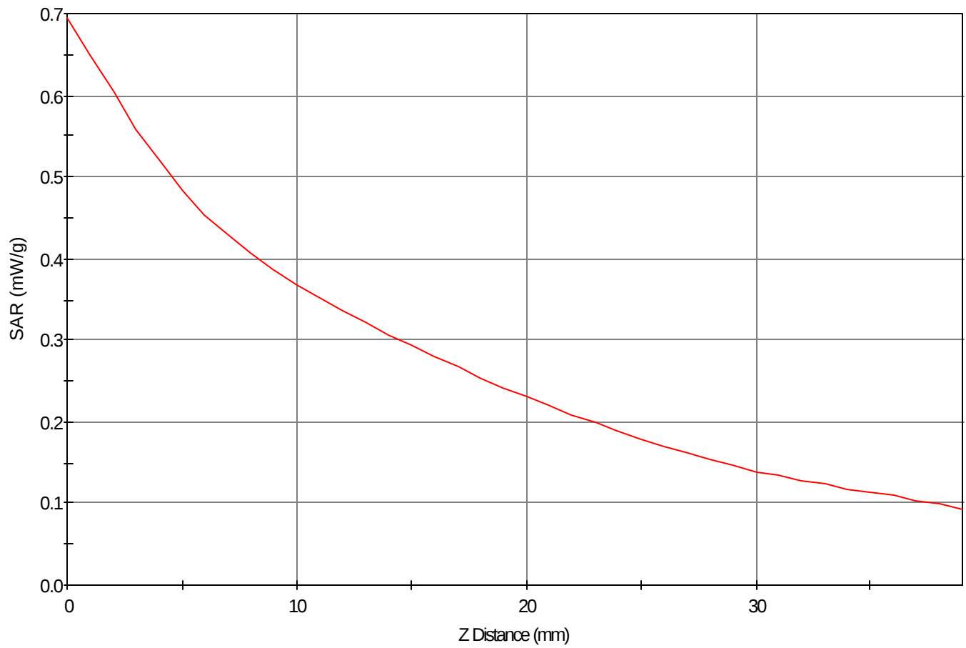
SAR - Z Axis at Hotspot x:52.0 y:6.0
