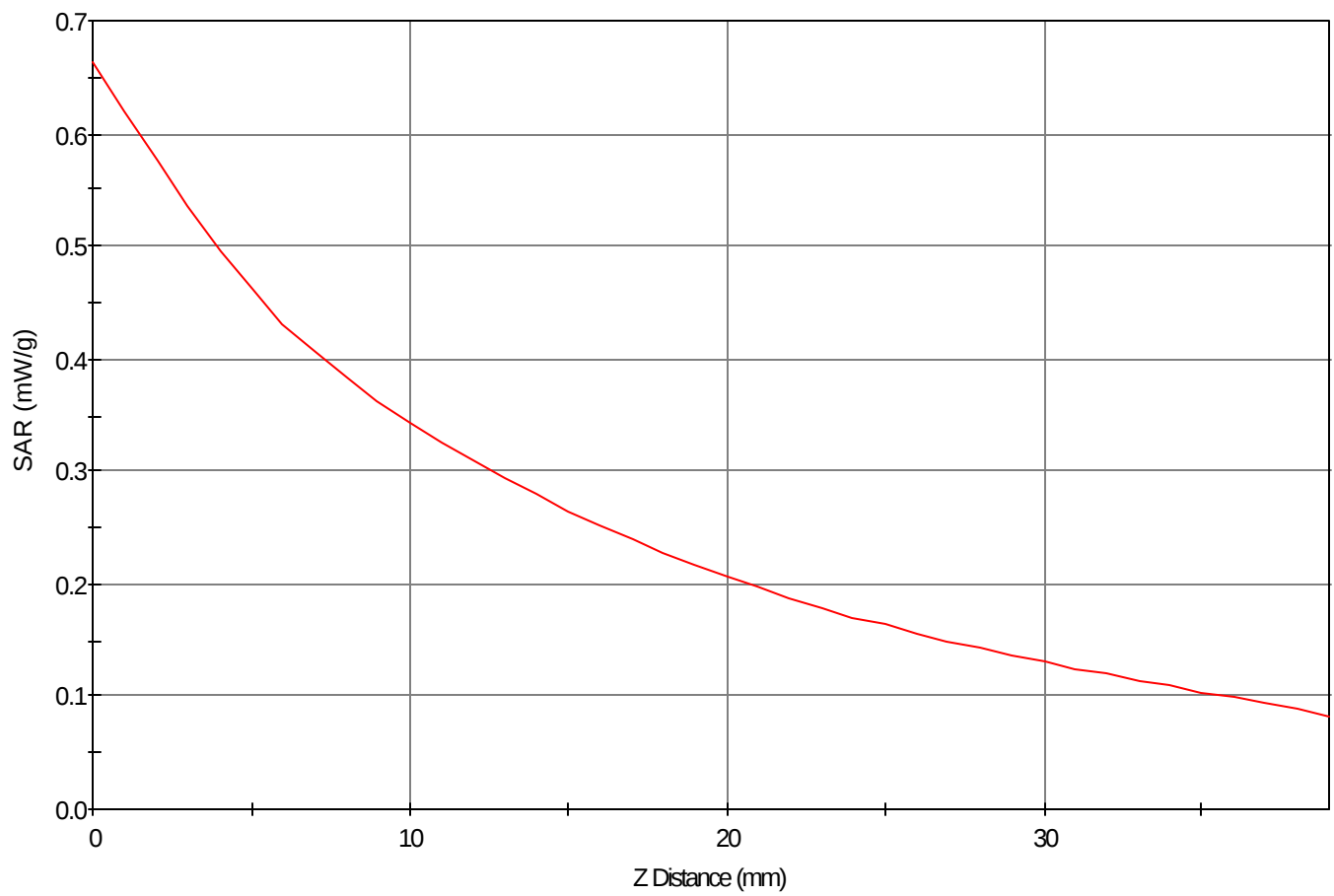
SAR - Z Axis at Hotspot x:42.0 y:7.0
