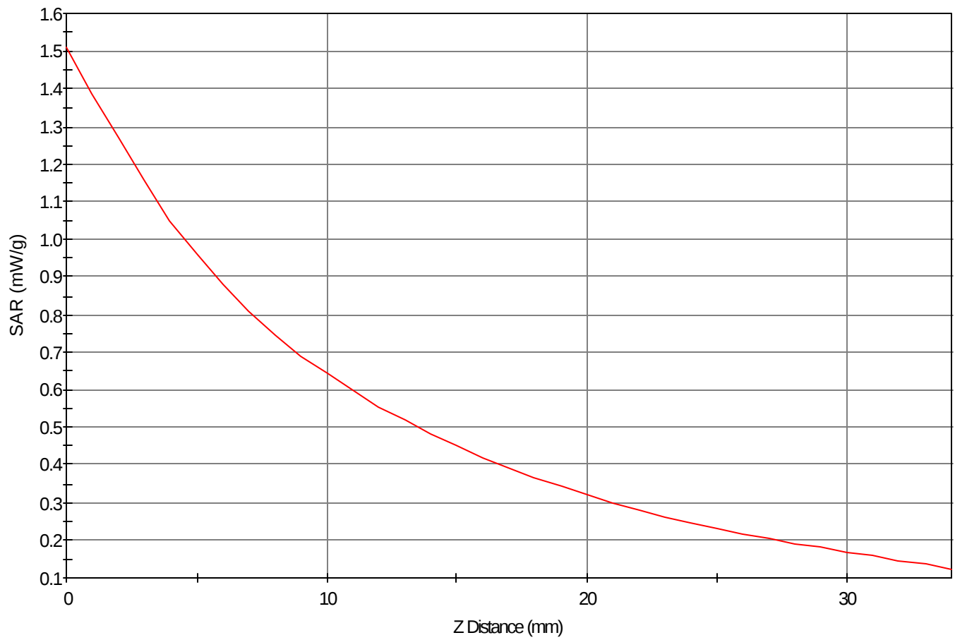
SAR - Z Axis at Hotspot x:74.0 y:12.0
