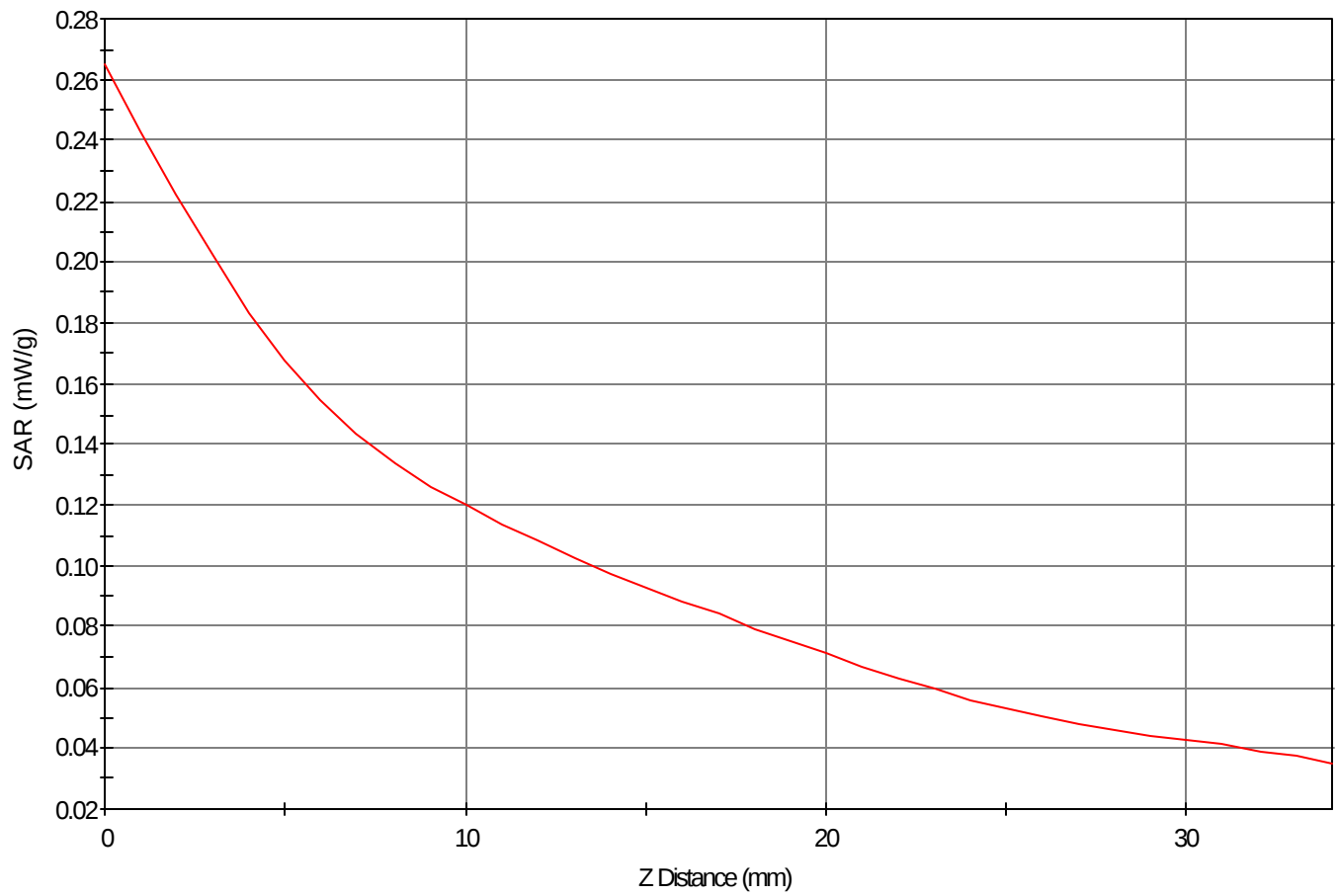
SAR - Z Axis at Hotspot x:63.0 y:10.0
