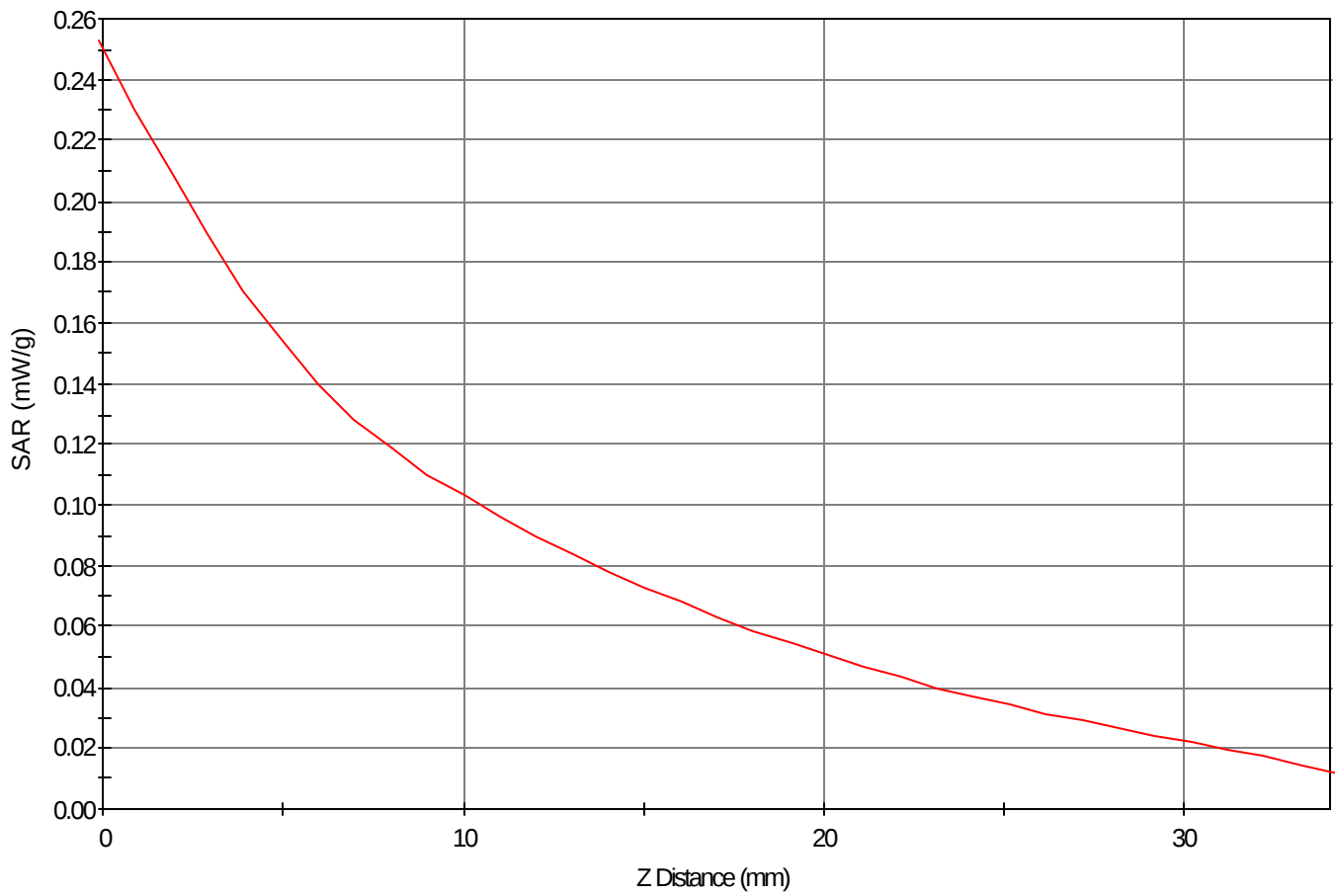
SAR - Z Axis at Hotspot x:48.0 y:4.0
