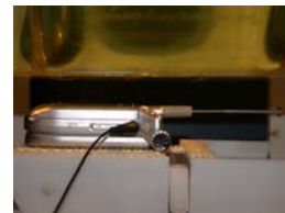
Figure 14.10 Body SAR Test Setup -- w/o Holster --
