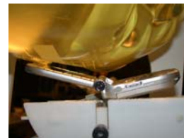
Figure 14.6 Right Head SAR Test Setup -- Tilt Position --
