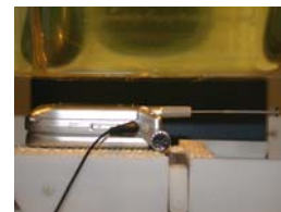
Figure 14.9 Body SAR Test Setup -- w/o Holster --
