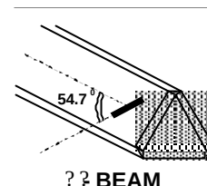
Figure 3.3 Triangular Probe Configuration
