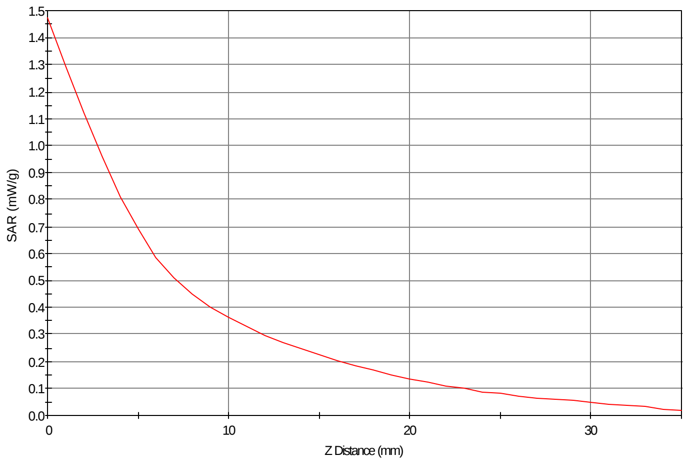
SAR - Z Axis at Hotspot x:-8.0 y:25.0
