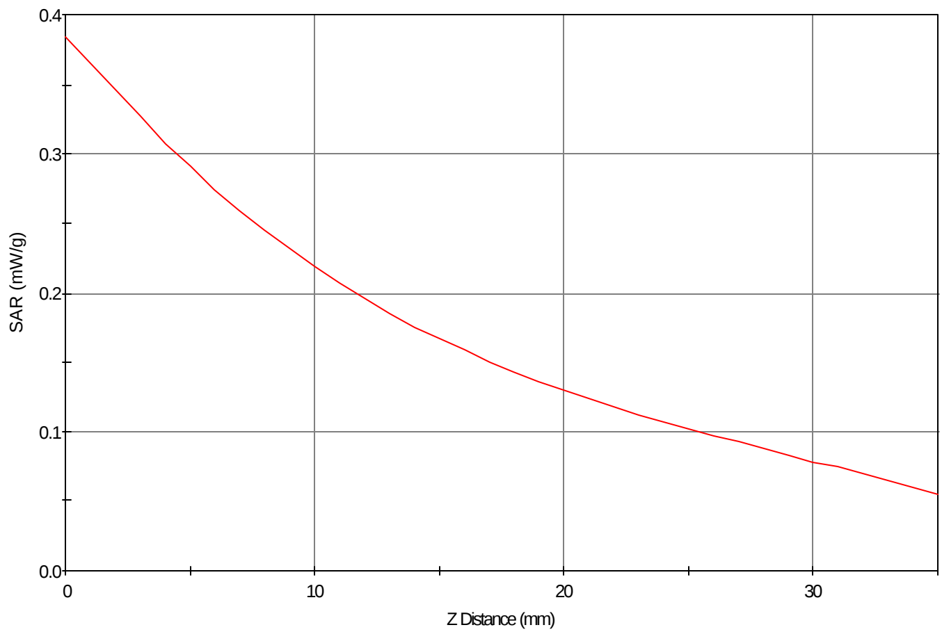
SAR - Z Axis at Hotspot x:65.0 y:27.0
