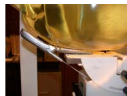
Figure A.7 Left Head SAR Test Setup -- Cheek / Touch Position --
