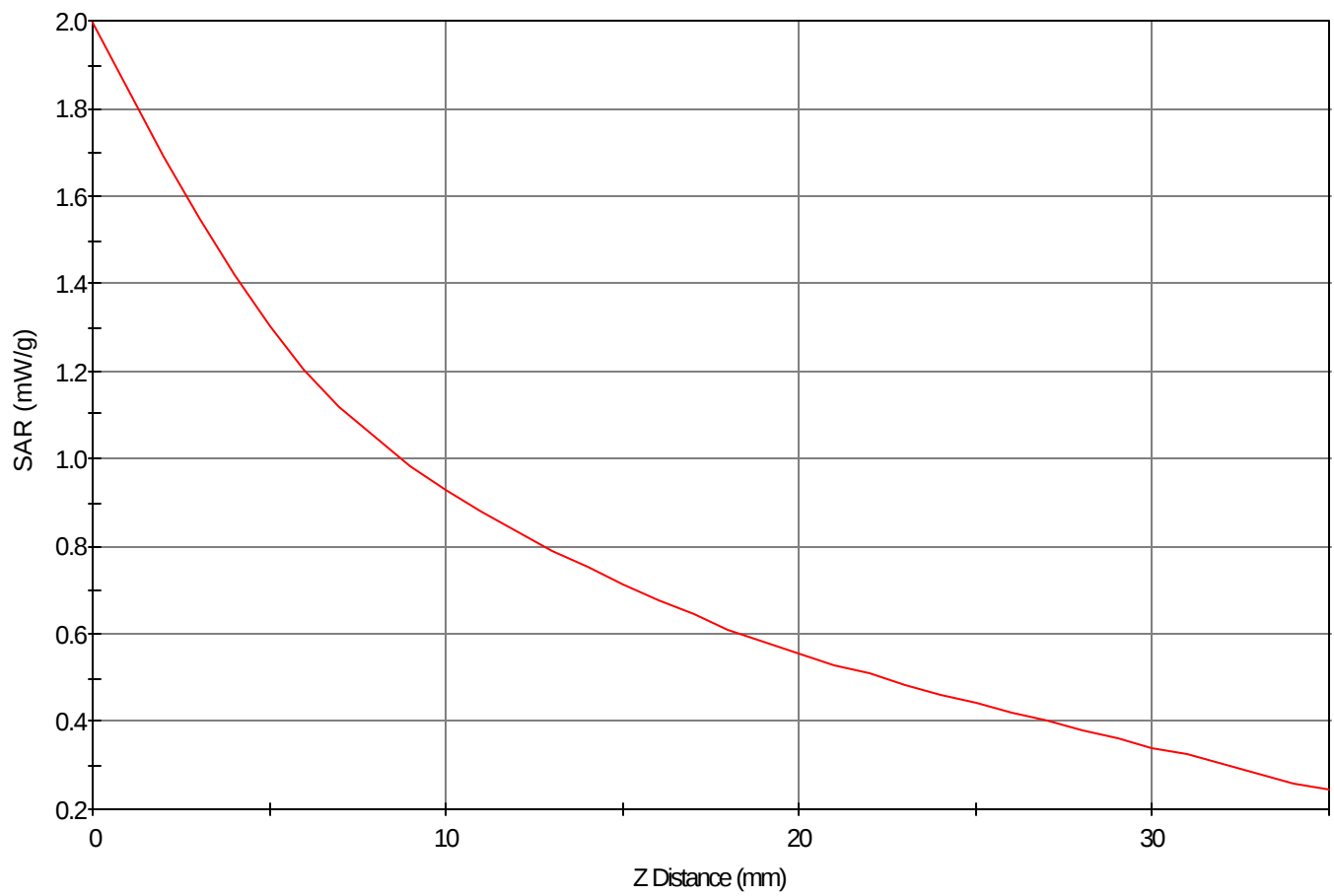
SAR - Z Axis at Hotspot x:69.0 y:18.0
