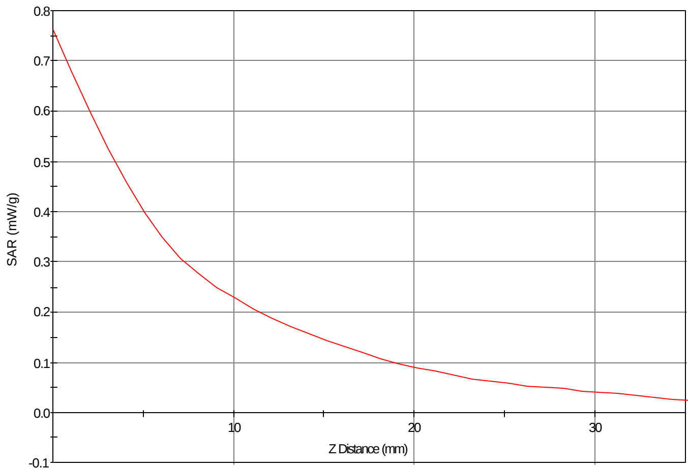
SAR - Z Axis at Hotspot x:13.0 y:7.0
