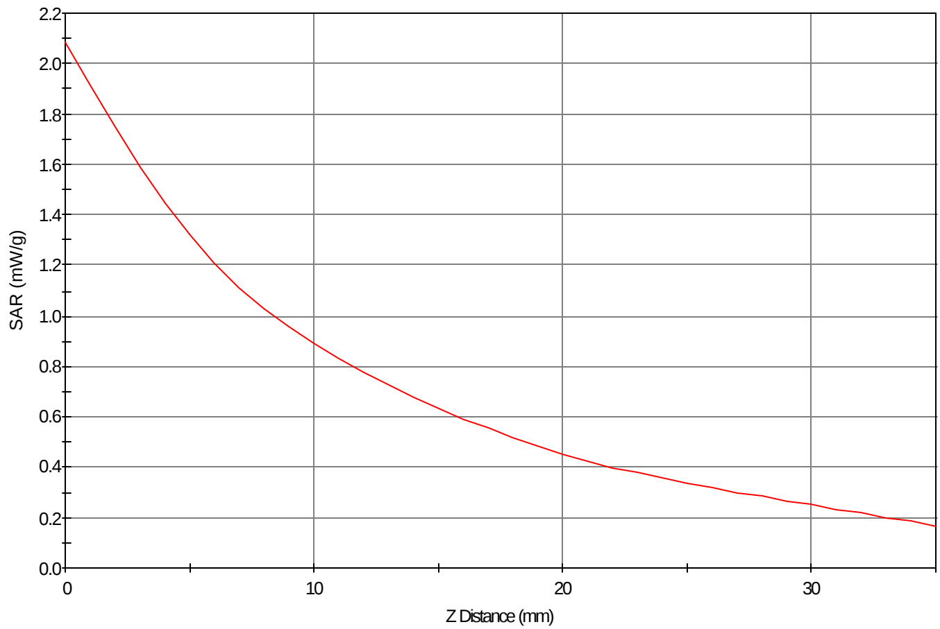
SAR - Z Axis at Hotspot x:72.0 y:25.0
