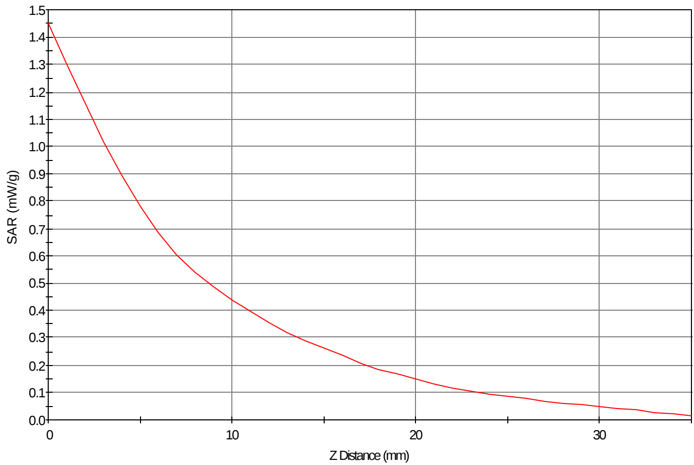
SAR - Z Axis at Hotspot x:68.0 y:19.0
