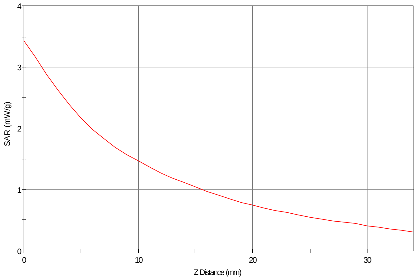
SAR - Z Axis at Hotspot x:-9.0 y:-2.0
