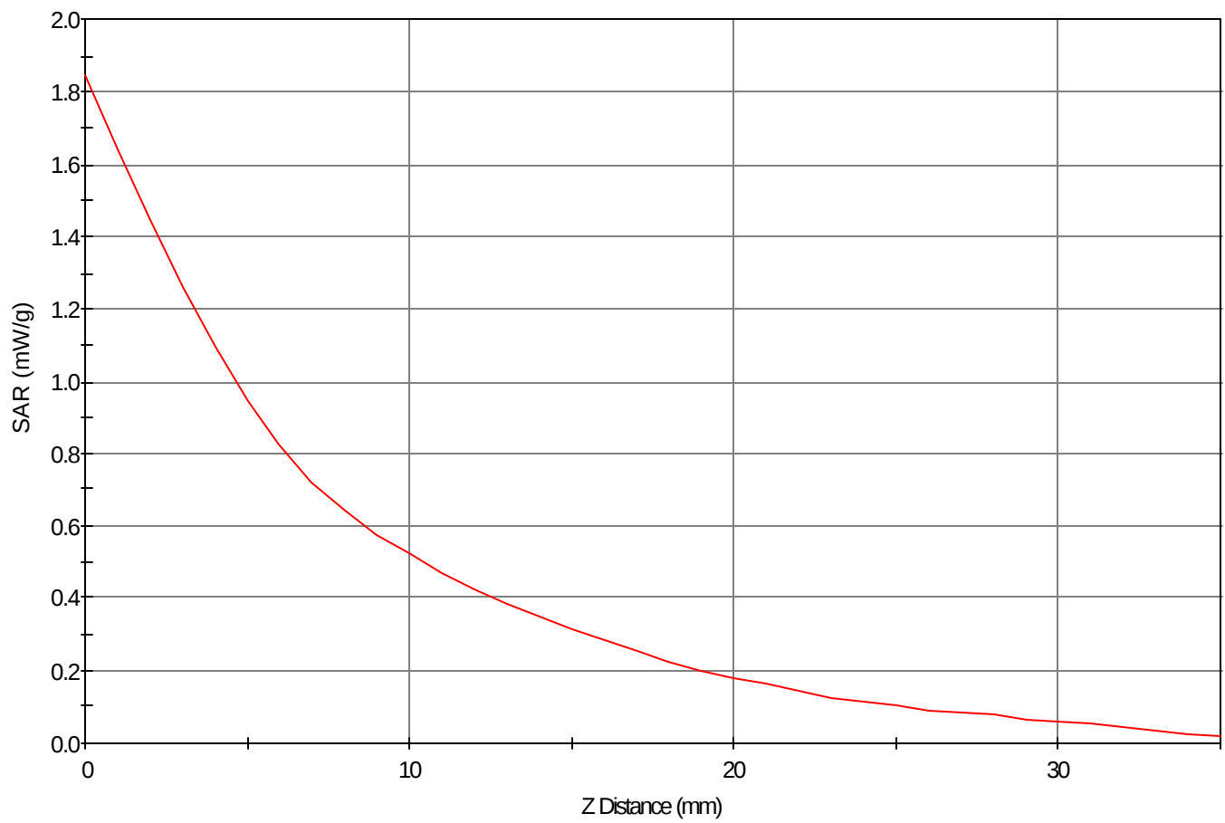
SAR - Z Axis at Hotspot x:67.0 y:19.0
