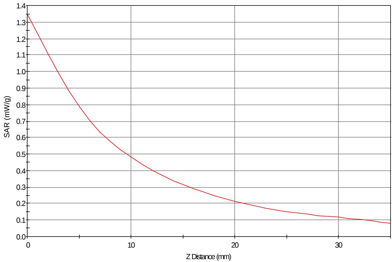
SAR - Z Axis at Hotspot x:67.0 y:14.0
