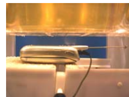
Figure A.10 Body SAR Test Setup -- w/o Holster --
