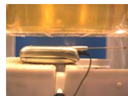
Figure A.9 Body SAR Test Setup -- w/o Holster --
