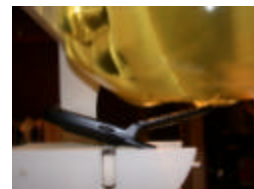
Figure 14.8 Left Head SAR Test Setup -- Ear / 15° Tilt Position --
