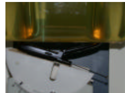
Figure 14.10.2 Face SAR Test Setup -- Open Position --
