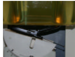
Figure 14.9.2 Face SAR Test Setup -- Open Position --
