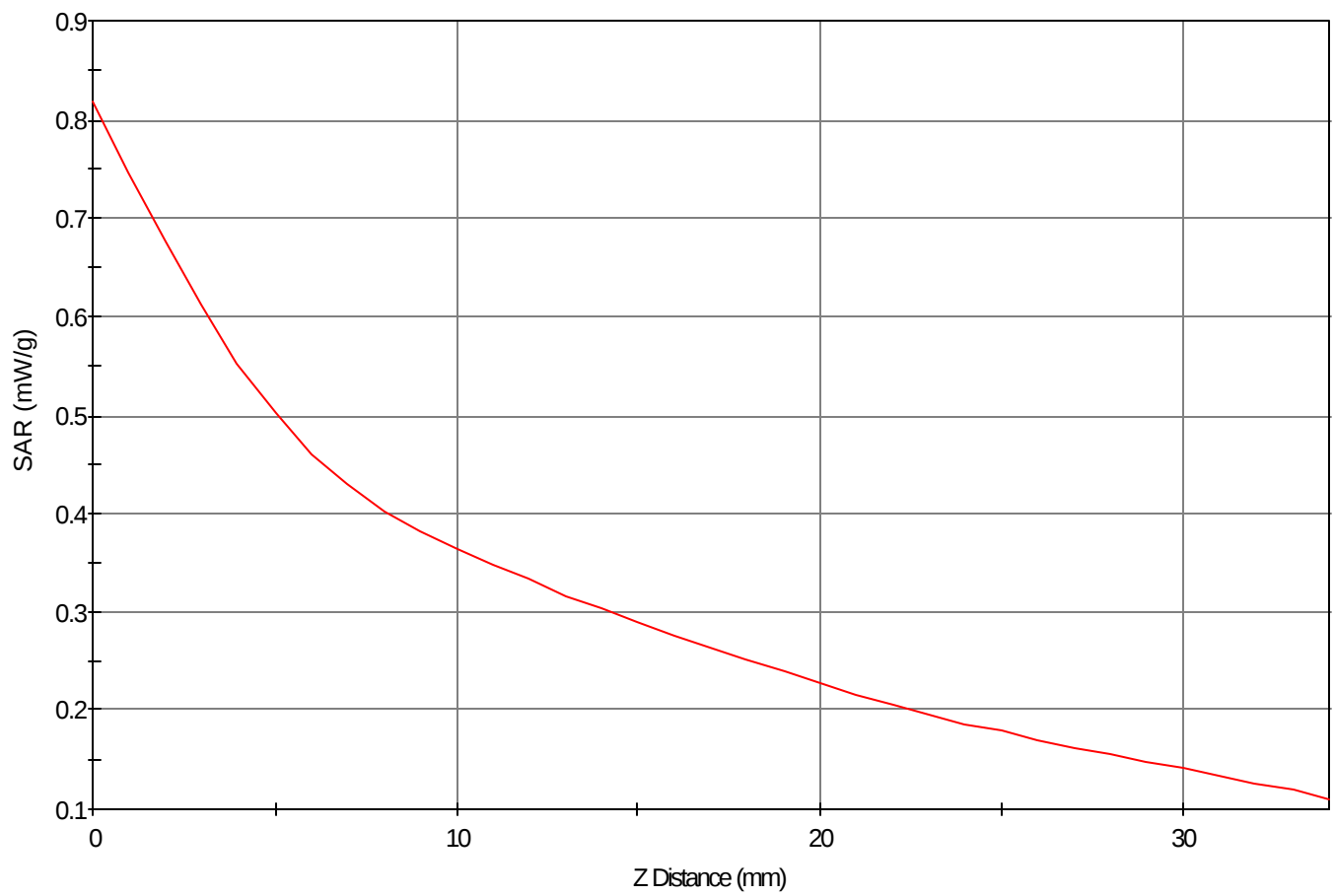
SAR - Z Axis at Hotspot x:59.0 y:16.0
