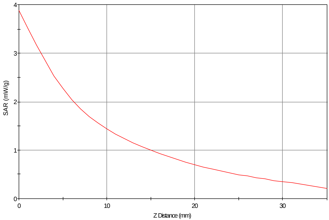
SAR - Z Axis at Hotspot x:-14.0 y:-3.0
