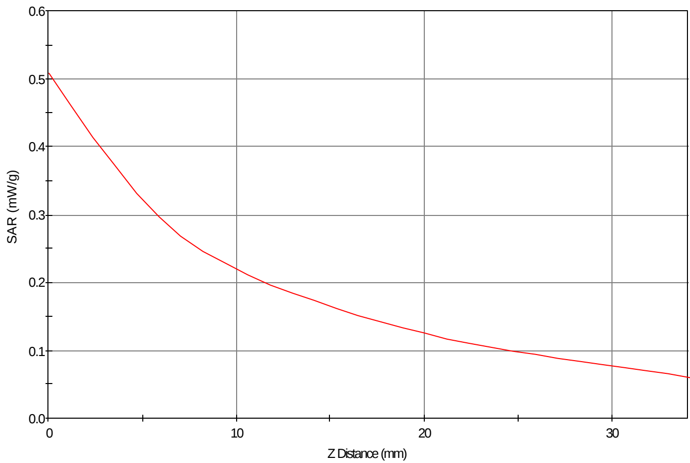
SAR - Z Axis at Hotspot x:59.0 y:36.0
