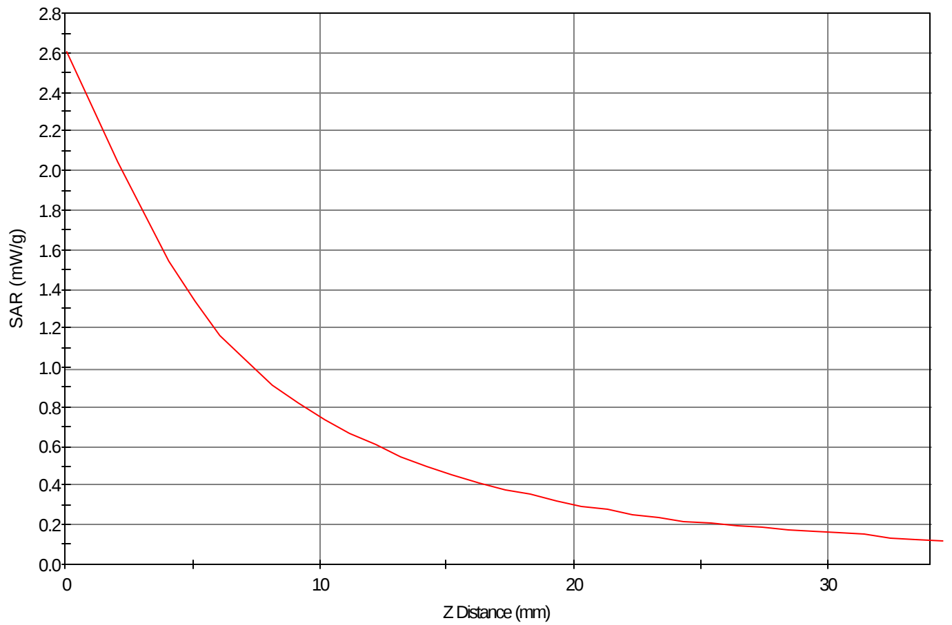
SAR - Z Axis at Hotspot x:88.0 y:24.0
