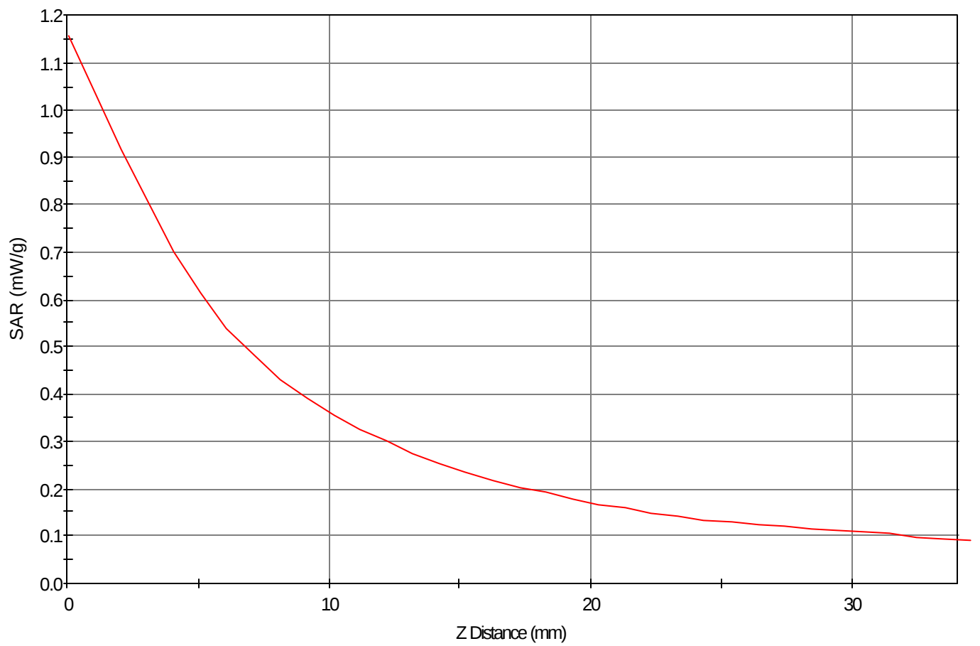
SAR - Z Axis at Hotspot x:93.0 y:-10.0
