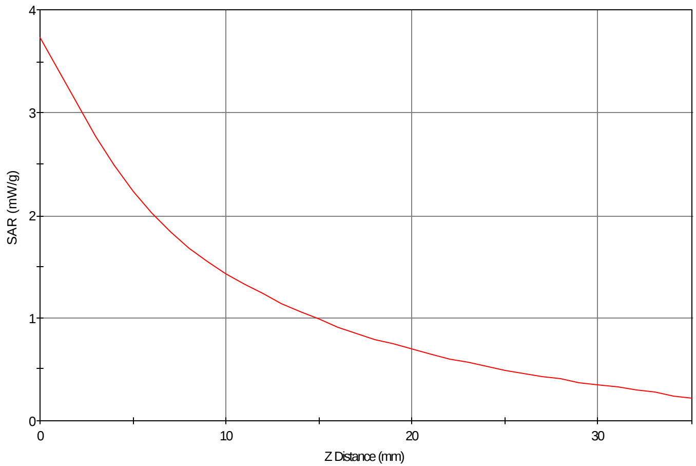
SAR - Z Axis at Hotspot x:-15.0 y:-3.0
