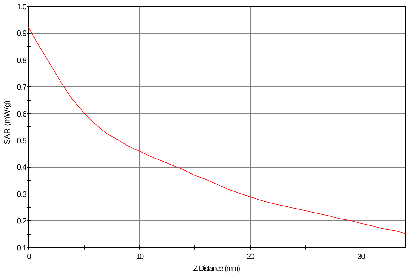
SAR - Z Axis at Hotspot x:60.0 y:8.0
