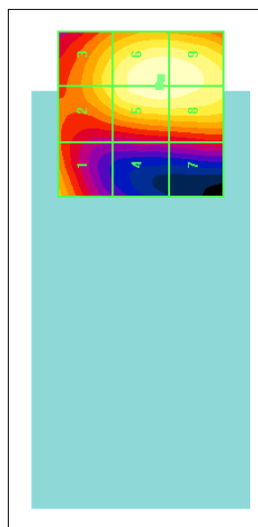
Figure 10-1 Sample E-field Scan Overlay
