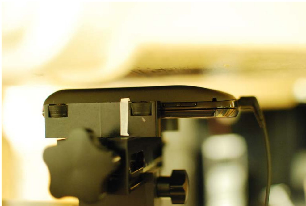
SAR Test Setup Photo 12 – Body-Worn at 1.0 cm (Extended Battery)
