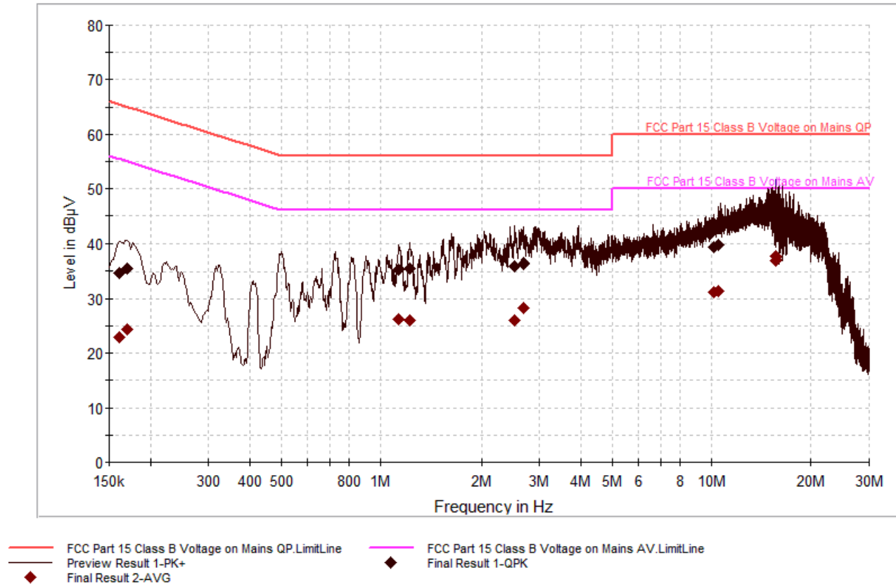
Plot 6-57. Line Conducted Plot with 802.11b (N)
