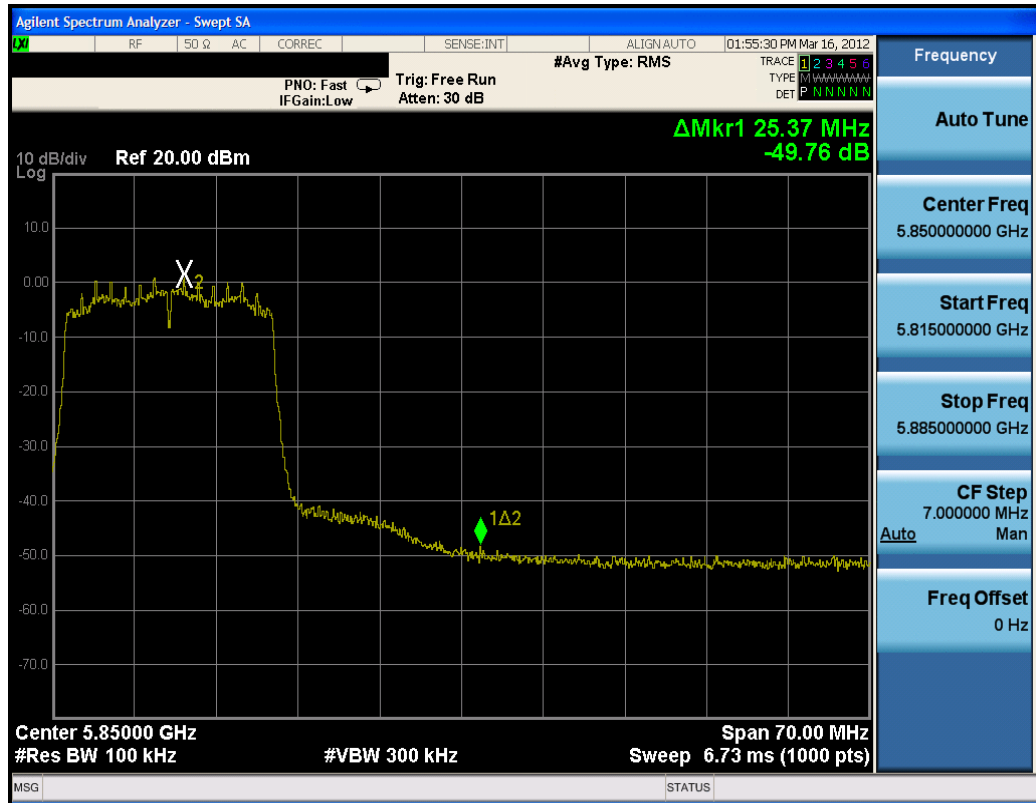
Plot 6-40. Band Edge Plot (802.11n (5.8GHz) – Ch. 165)
