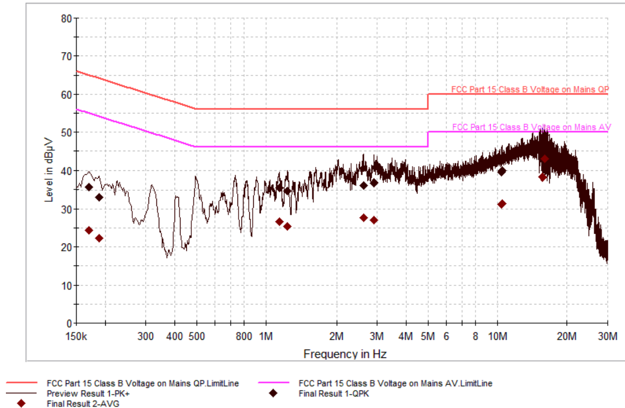
Plot 6-59. Line Conducted Plot with 802.11a (N)
