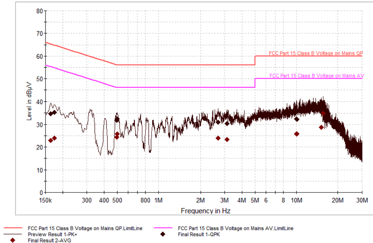
Plot 6-56. Line Conducted Plot with 802.11b (Line 1)
