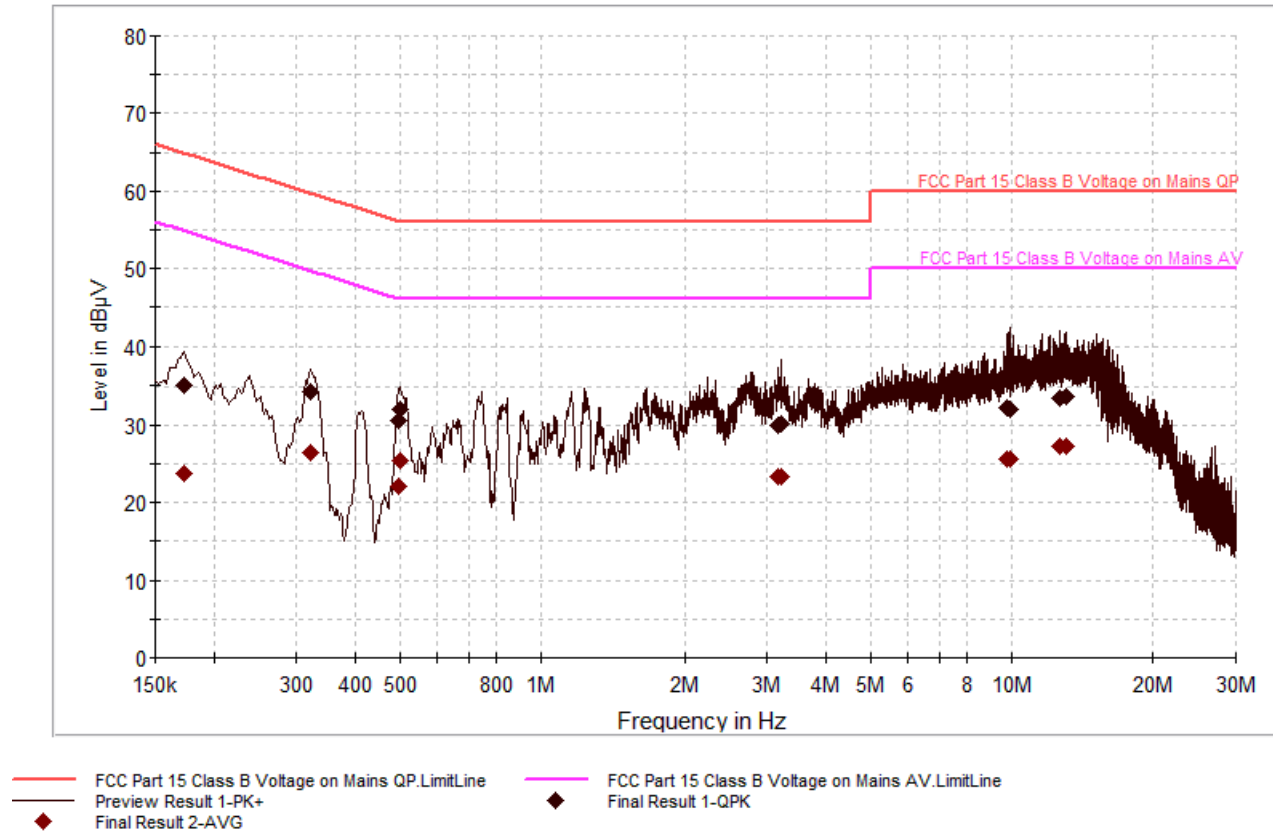
Plot 6-58. Line Conducted Plot with 802.11a (Line 1)
