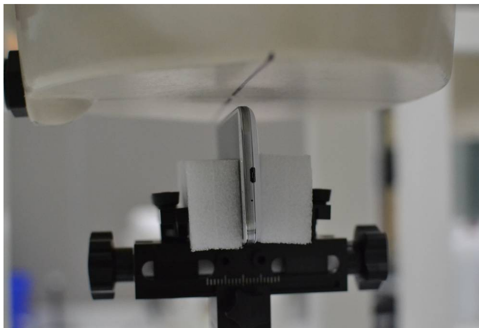
SAR Test Setup Photo 13 – Right Edge with Wireless Charging Cover at 1.0 cm
