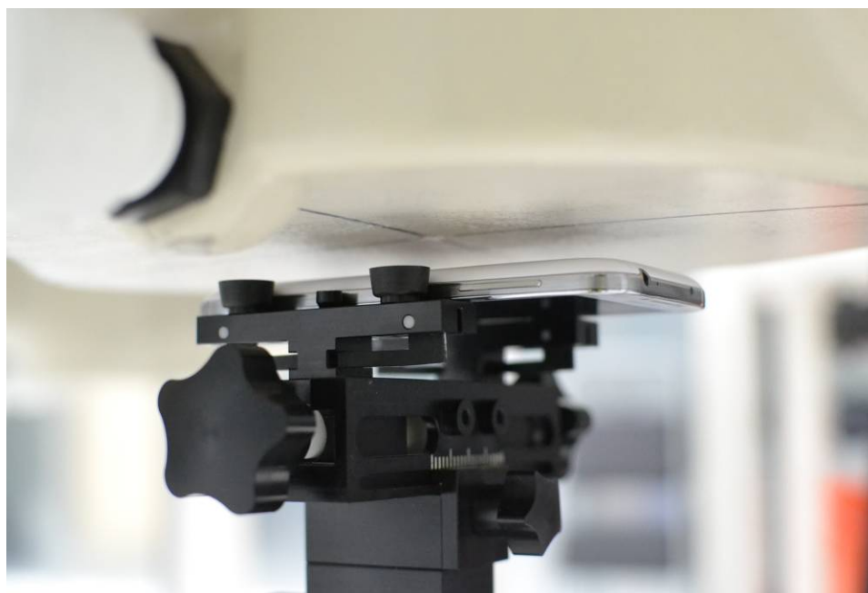
SAR Test Setup Photo 8 – Back side with Wireless Charging Cover at 1.0 cm
