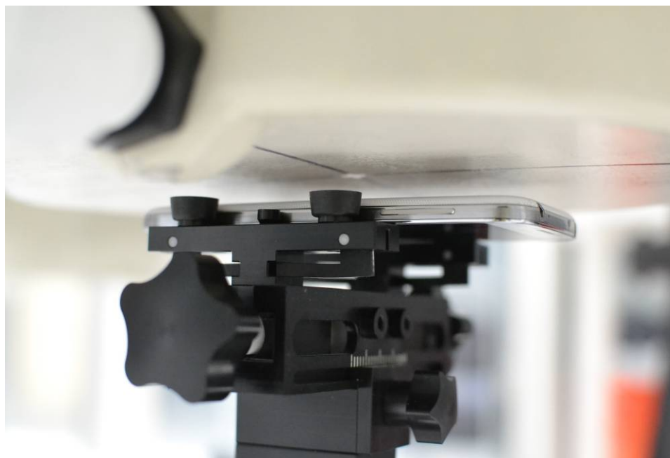
SAR Test Setup Photo 7 – Back side at 1.0 cm
