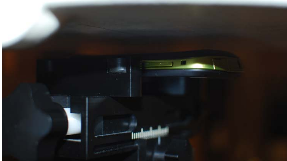
Figure 21-5 SAR Test Setup Photo 5 – Body Back, 1.0 cm
