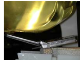
Figure 14.6 Right Head SAR Test Setup -- Ear / 15° Tilt Position --
