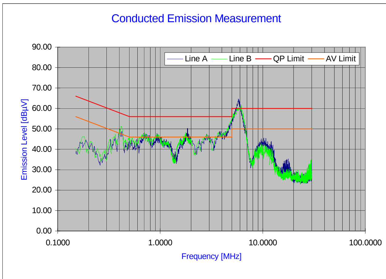
Plot 6-17. Line Conducted Plot with 802.11b
