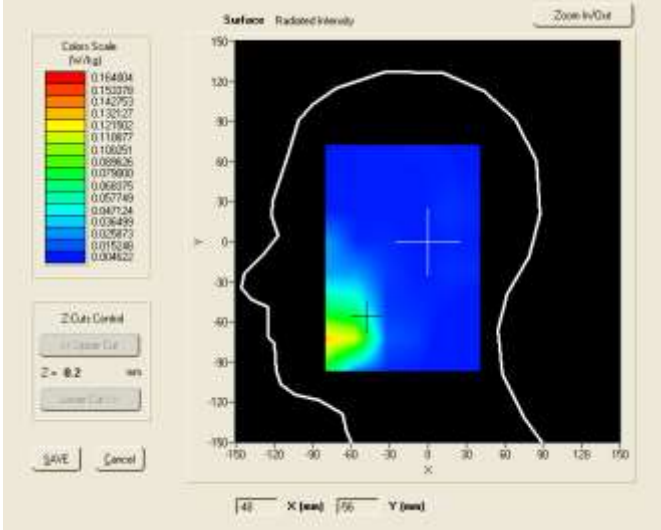
SURFACE SAR
