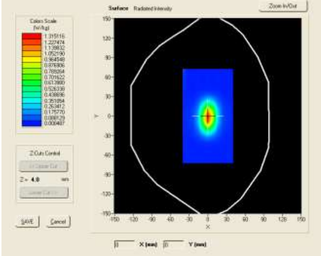
SURFACE SAR
