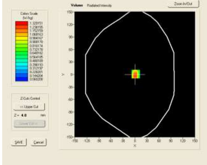
VOLUME SAR
