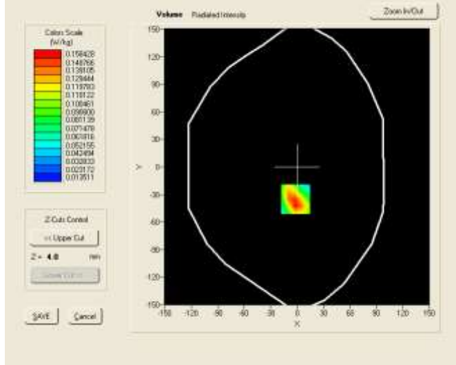
VOLUME SAR
