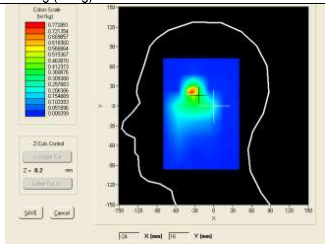
SURFACE SAR
