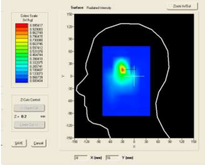
SURFACE SAR
