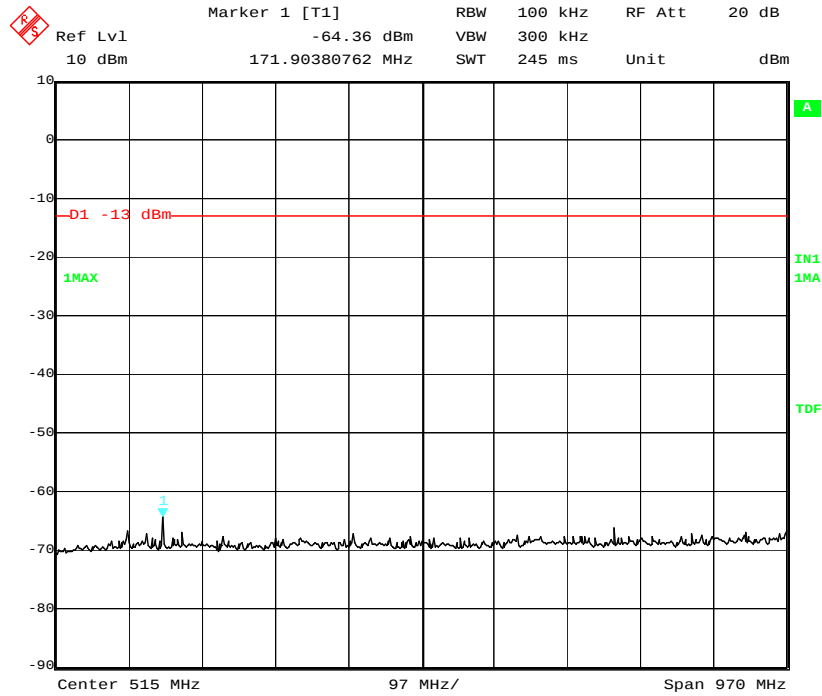
Low channel 30MHz-1GHz
