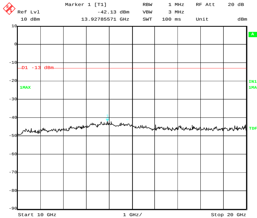
Low channel 10GHz-20GHz
