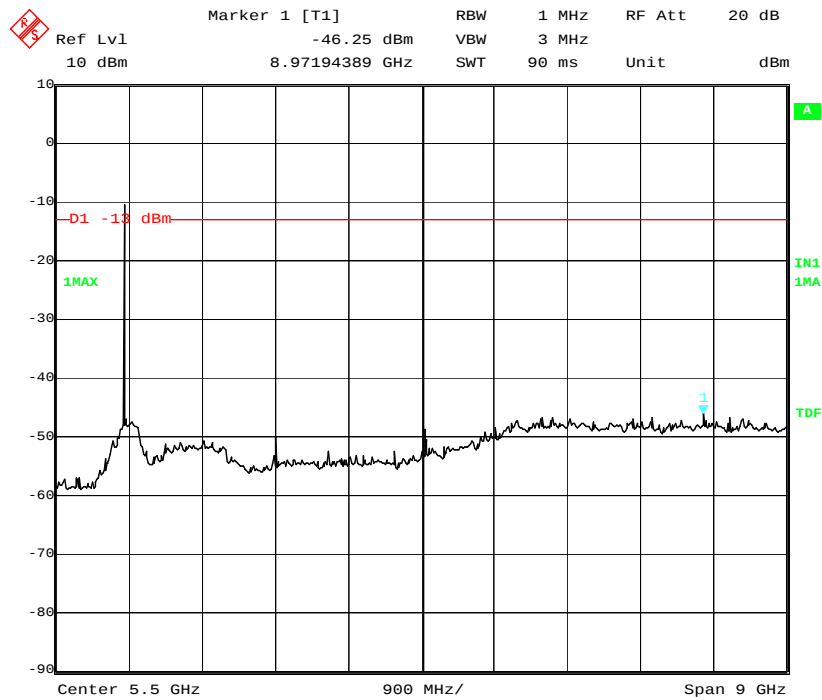
Low channel 1GHz-10GHz
