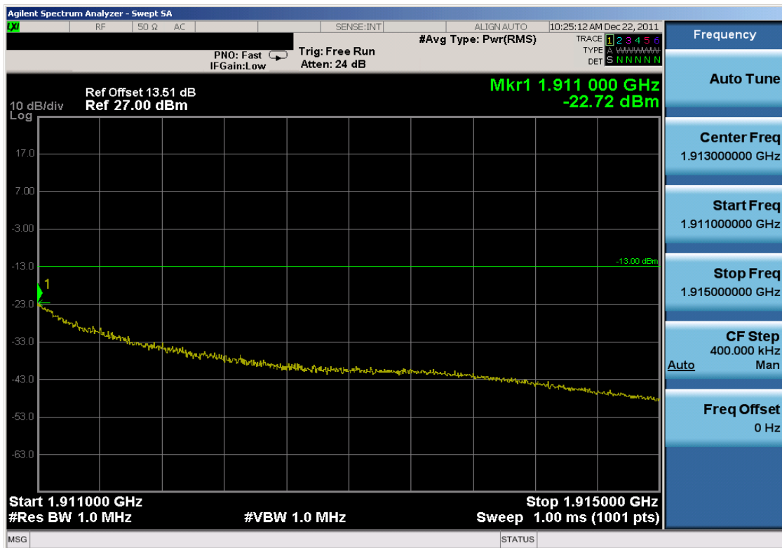
Plot 7-24. 4MHz Span Plot (PCS CDMA Mode - Ch. 1175)
