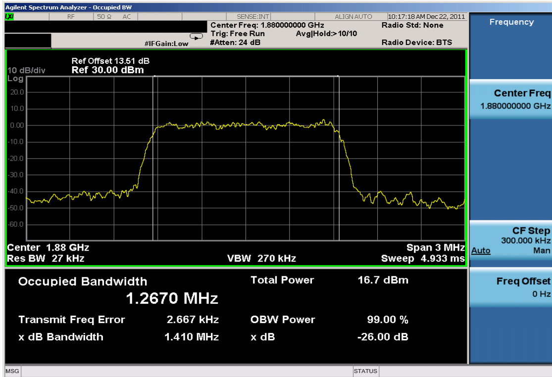
Plot 7-19. Occupied Bandwidth Plot (PCS CDMA Mode – Ch. 600)
