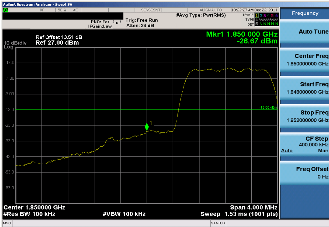
Plot 7-15. Band Edge Plot (PCS CDMA Mode – Ch. 25)
