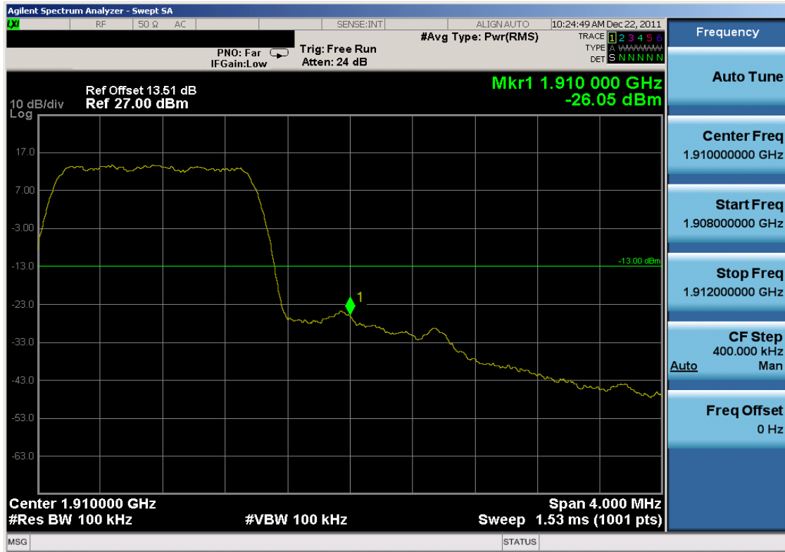
Plot 7-23. Band Edge Plot (PCS CDMA Mode - Ch. 1175)
