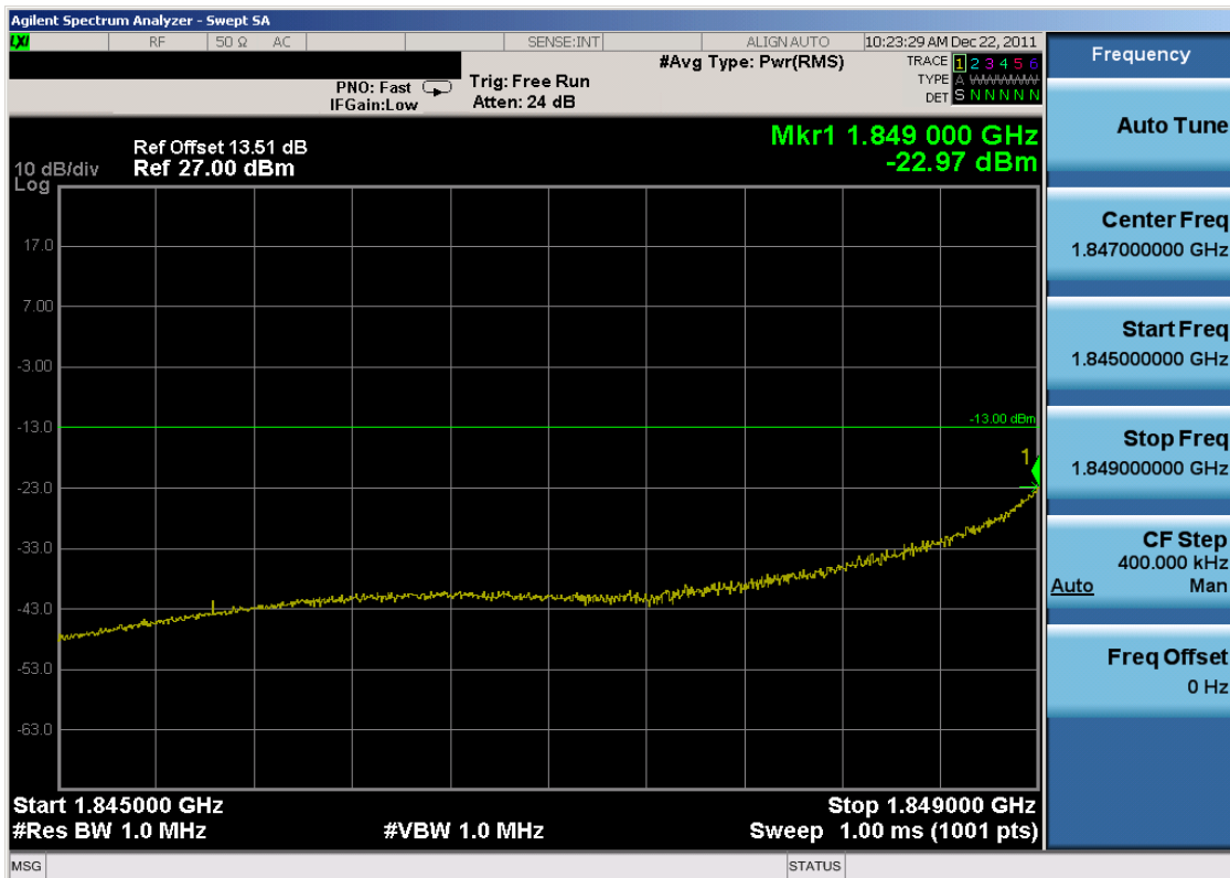
Plot 7-16. 4MHz Span Plot (PCS CDMA Mode – Ch. 25)
