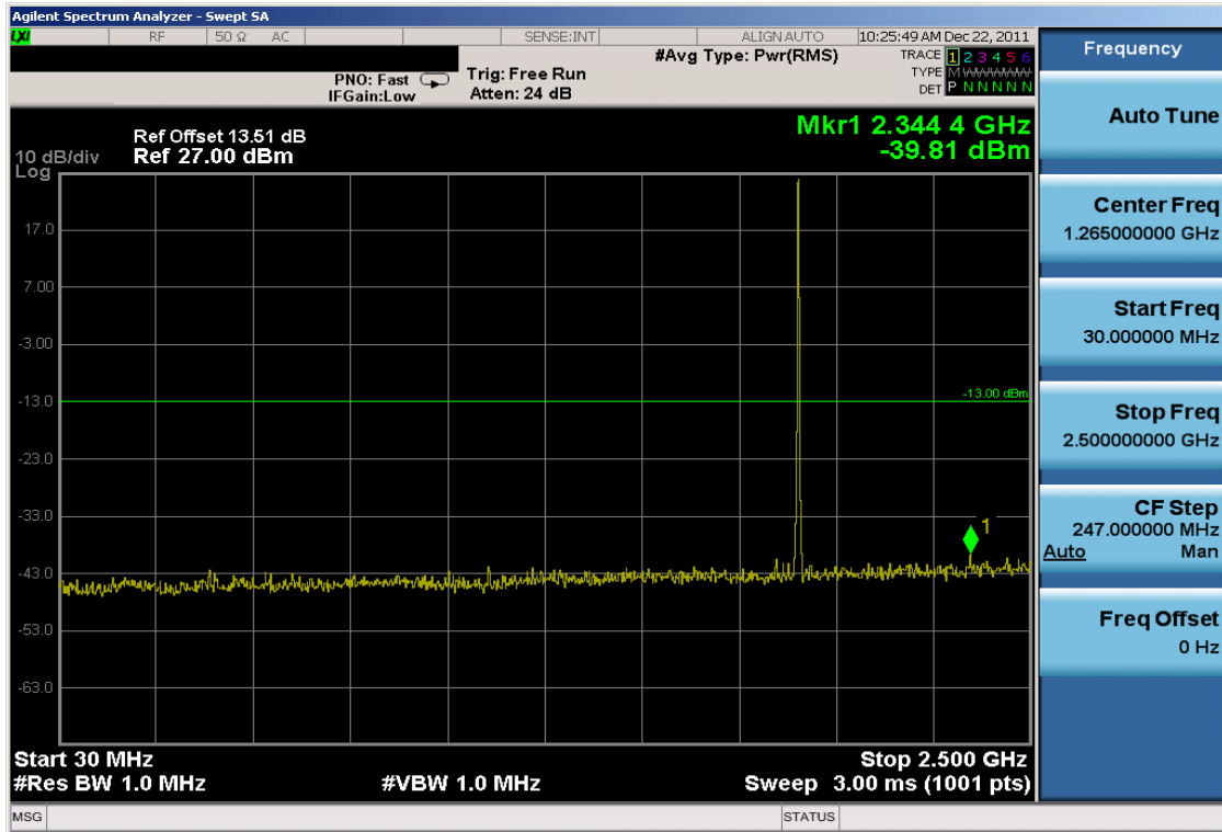
Plot 7-21. Conducted Spurious Plot (PCS CDMA Mode – Ch. 1175)
