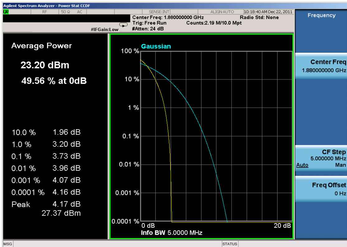
Plot 7-20. Peak-Average Ratio Plot (PCS CDMA Mode – Ch. 600)
