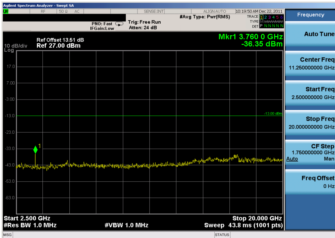
Plot 7-18. Conducted Spurious Plot (PCS CDMA Mode – Ch. 600)
