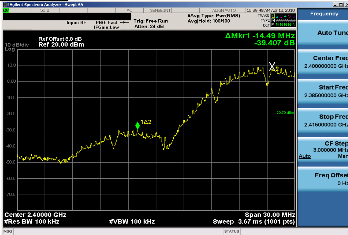
Plot 6-13. Band Edge Plot (802.11b – Ch. 1)
