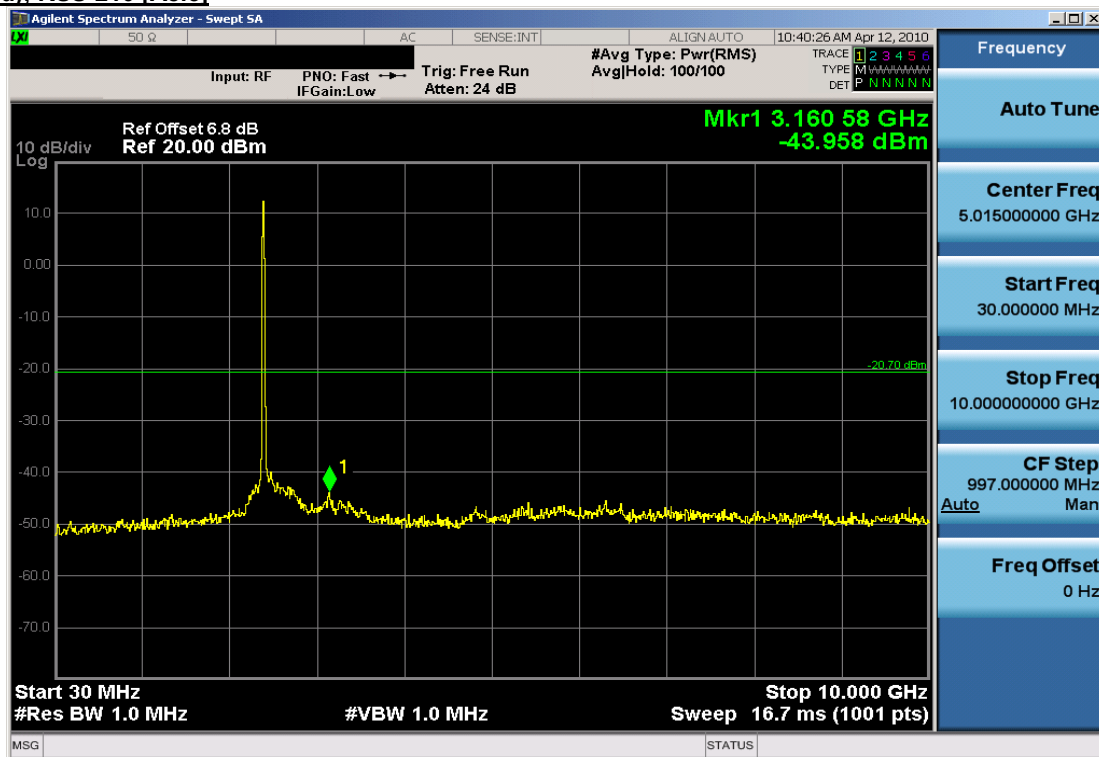
Plot 6-17. Conducted Spurious Plot (802.11b – Ch. 1)
