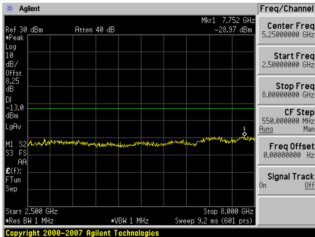
Plot 7-6. Conducted Spurious Plot (QPSK – RB Size 1, RB Offset 0)
