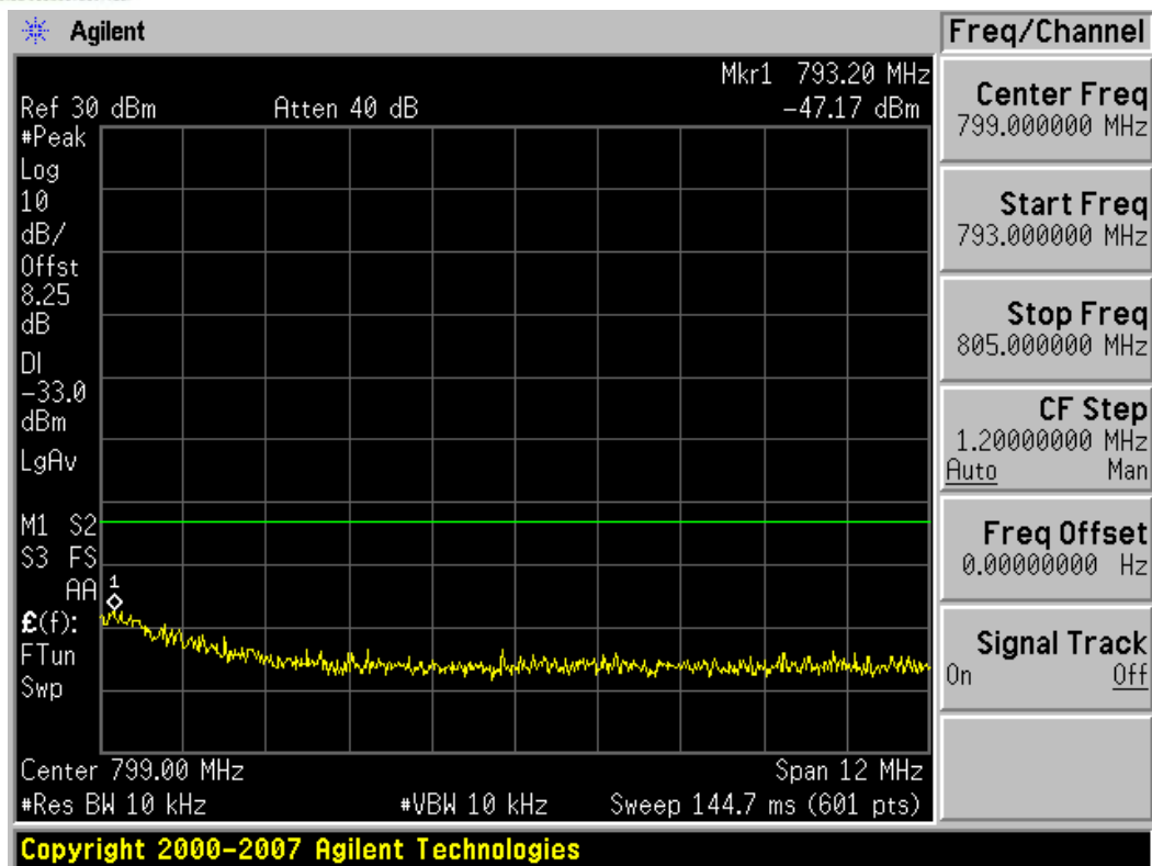
Plot 7-8. Upper Emission Mask (793 – 805MHz) Plot (QPSK – RB Size 50)
