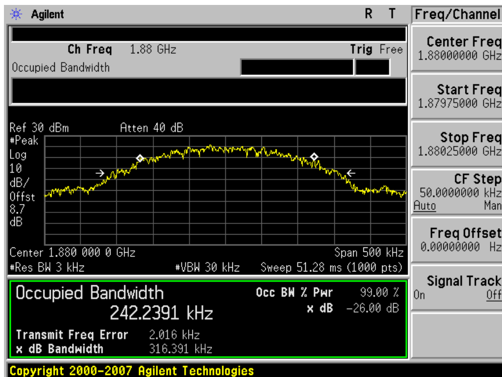
Plot 7-29. Occupied Bandwidth Plot (PCS GSM Mode – Ch. 661)
