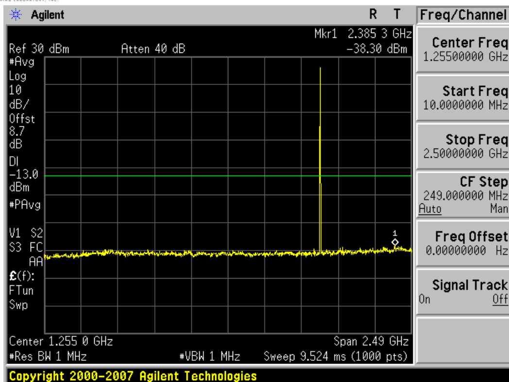
Plot 7-27. Conducted Spurious Plot (PCS GSM Mode – Ch. 661)
