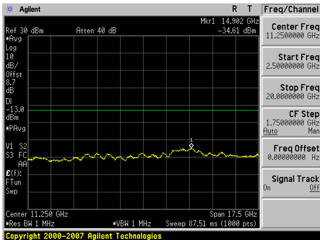
Plot 7-28. Conducted Spurious Plot (PCS GSM Mode – Ch. 661)
