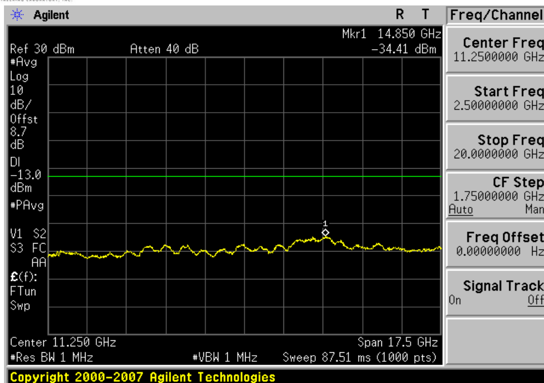
Plot 7-25. Conducted Spurious Plot (PCS GSM Mode – Ch. 512)
