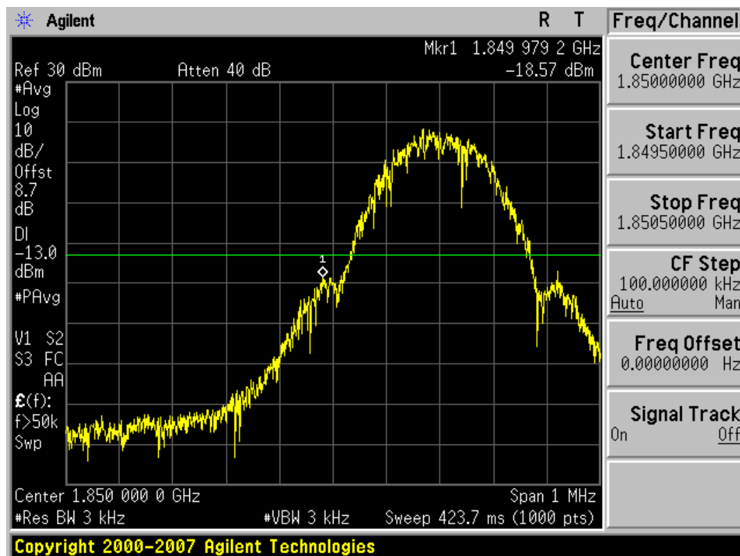
Plot 7-26. Band Edge Plot (PCS GSM Mode – Ch. 512)
