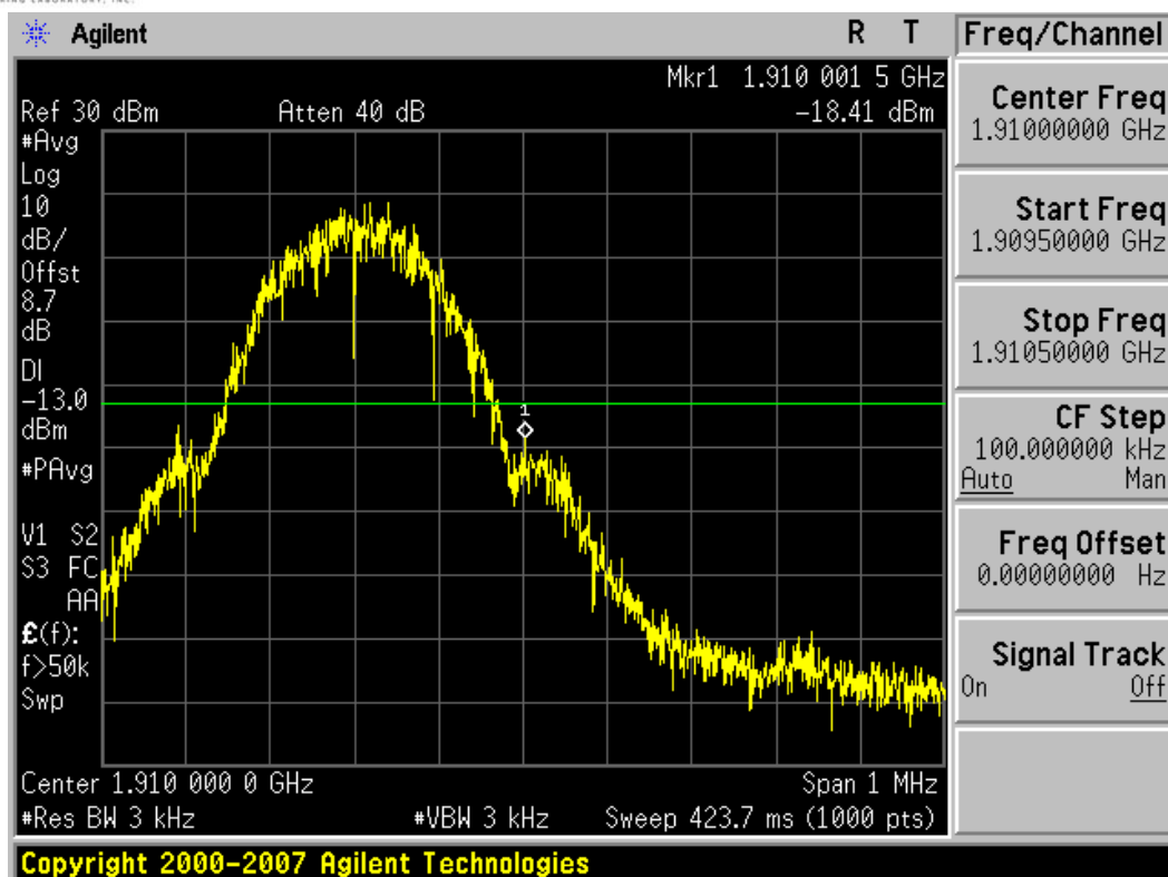
Plot 7-33. Band Edge Plot (PCS GSM Mode – Ch. 810)
