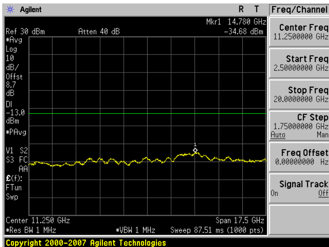
Plot 7-32. Conducted Spurious Plot (PCS GSM Mode – Ch. 810)
