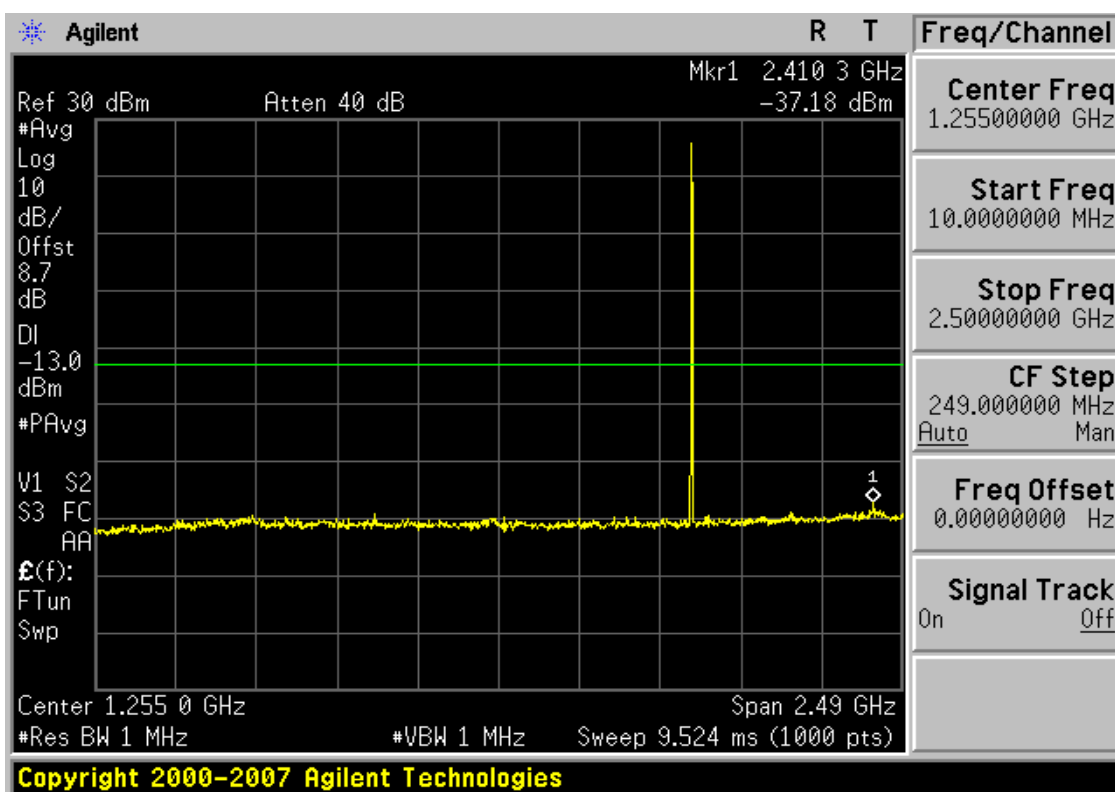
Plot 7-24. Conducted Spurious Plot (PCS GSM Mode – Ch. 512)
