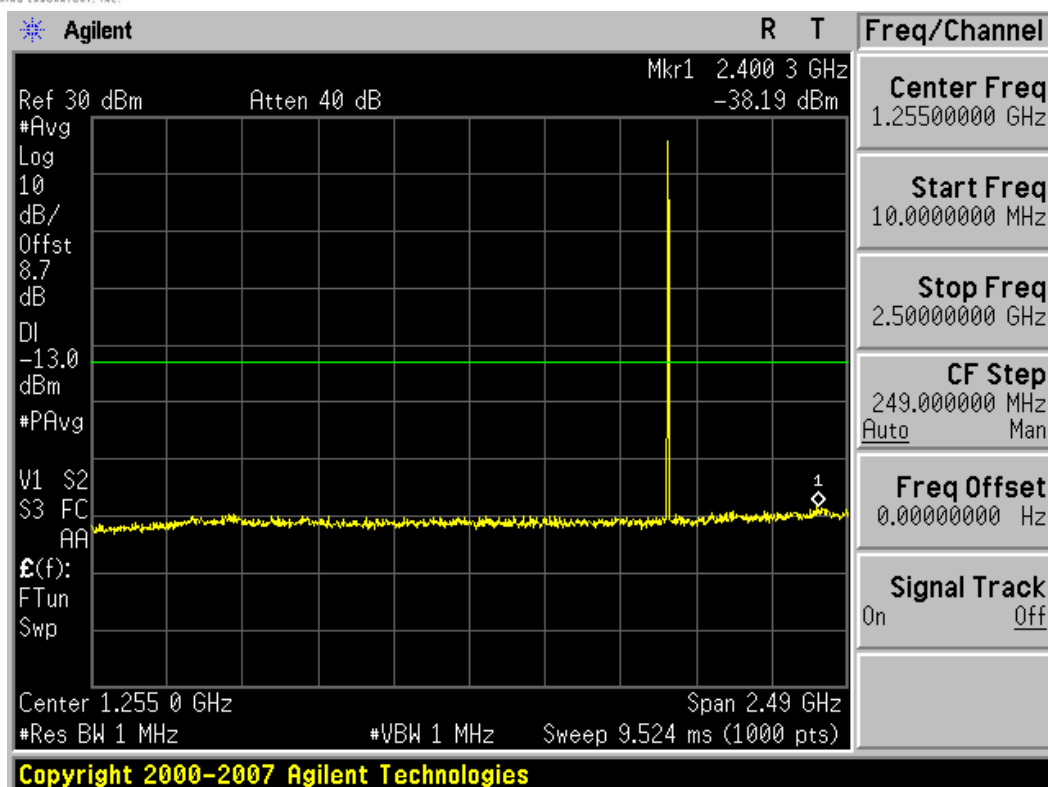
Plot 7-31. Conducted Spurious Plot (PCS GSM Mode – Ch. 810)
