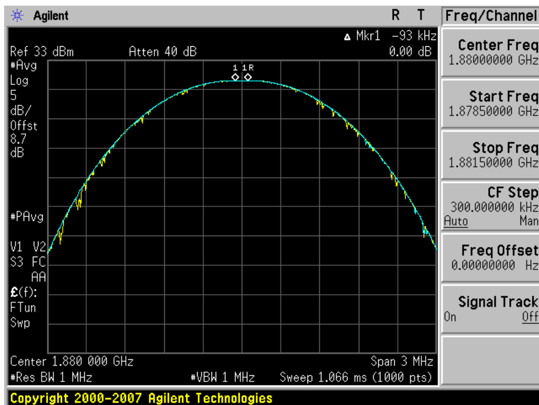
Plot 7-30. Peak-Average Ratio Plot (PCS GSM Mode – Ch. 661)
