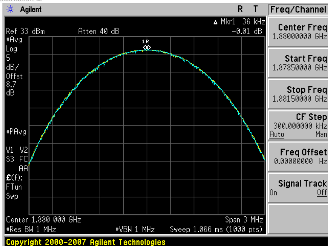
Plot 7-35. Peak-Average Ratio Plot (EDGE1900 Mode – Ch. 661)
