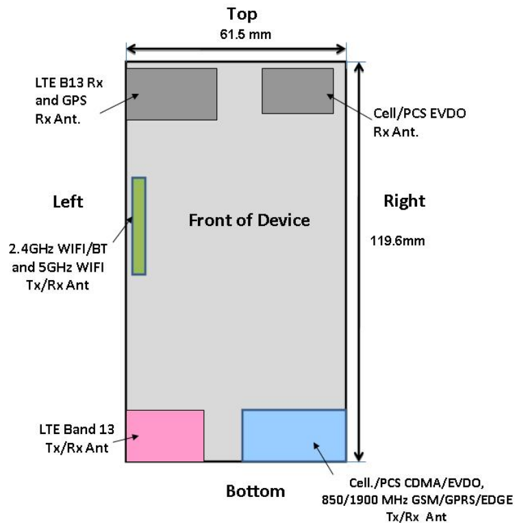
Figure 1-2 EUT Antenna Locations
