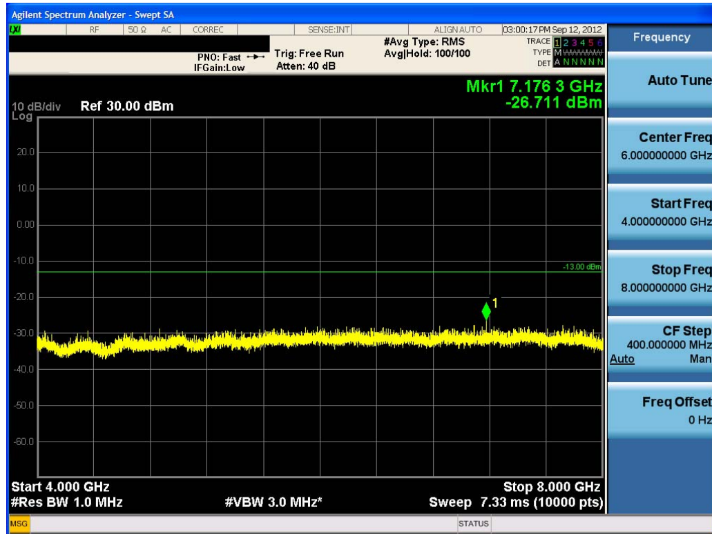
Plot 7-10. Conducted Spurious Plot (QPSK - RB Size 1, RB Offset 0)
