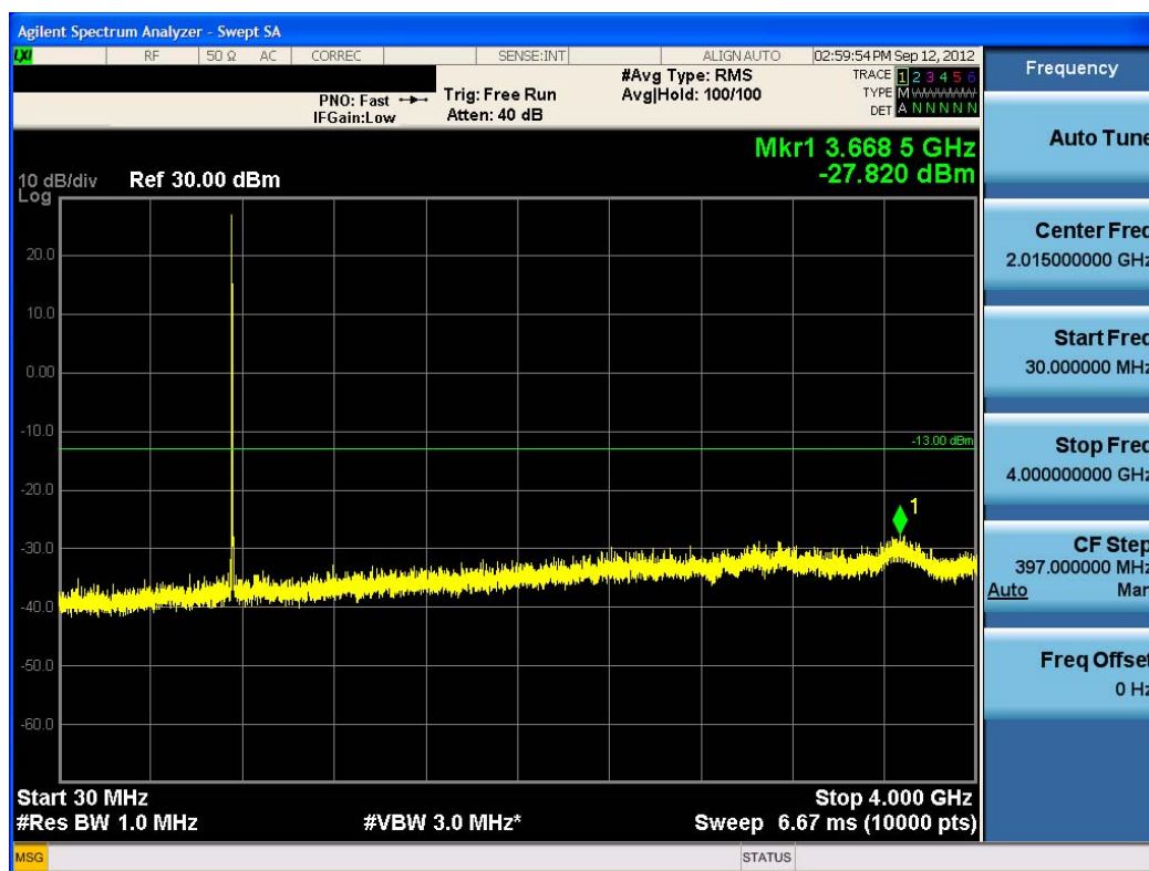
Plot 7-9. Conducted Spurious Plot (QPSK – RB Size 1, RB Offset 0)
