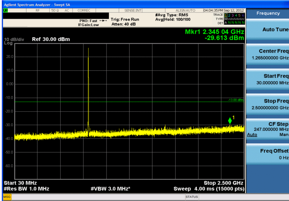
Plot 7-23. Conducted Spurious Plot (Cellular CDMA Mode – Ch. 1013)
