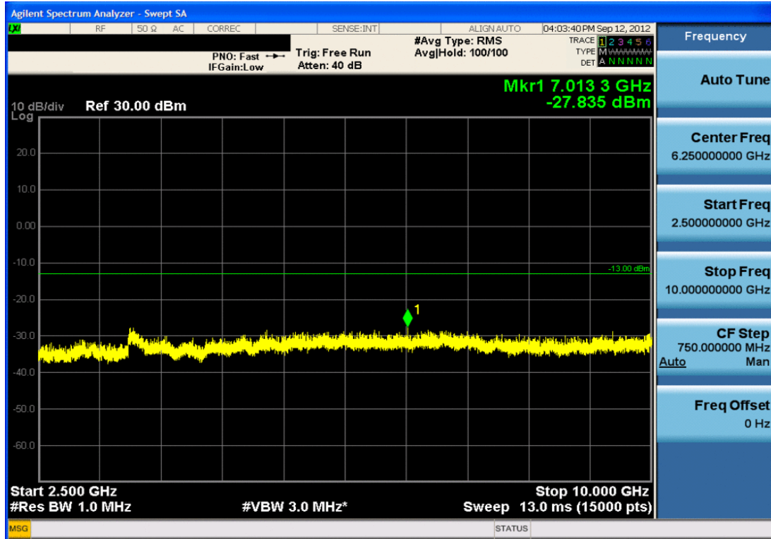
Plot 7-31. Conducted Spurious Plot (Cellular CDMA Mode – Ch. 777)
