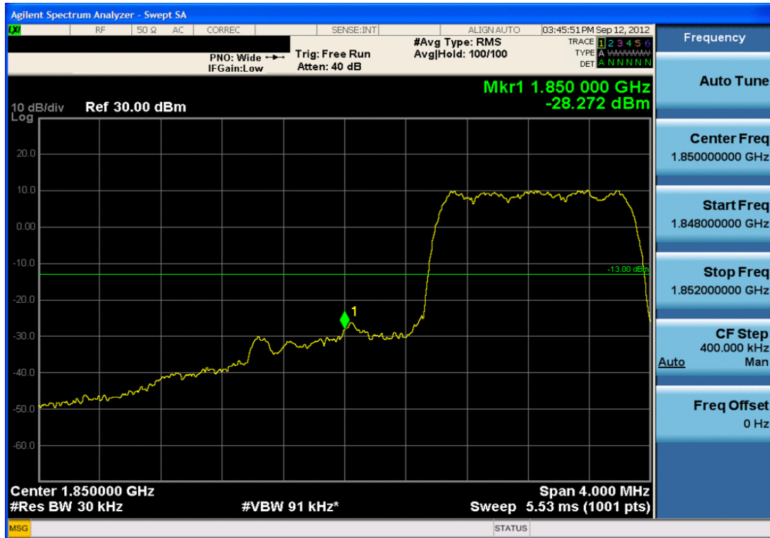
Plot 7-36. Band Edge Plot (PCS CDMA Mode – Ch. 25)
