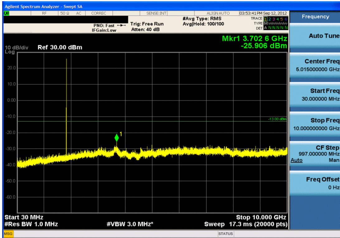
Plot 7-34. Conducted Spurious Plot (PCS CDMA Mode – Ch. 25)
