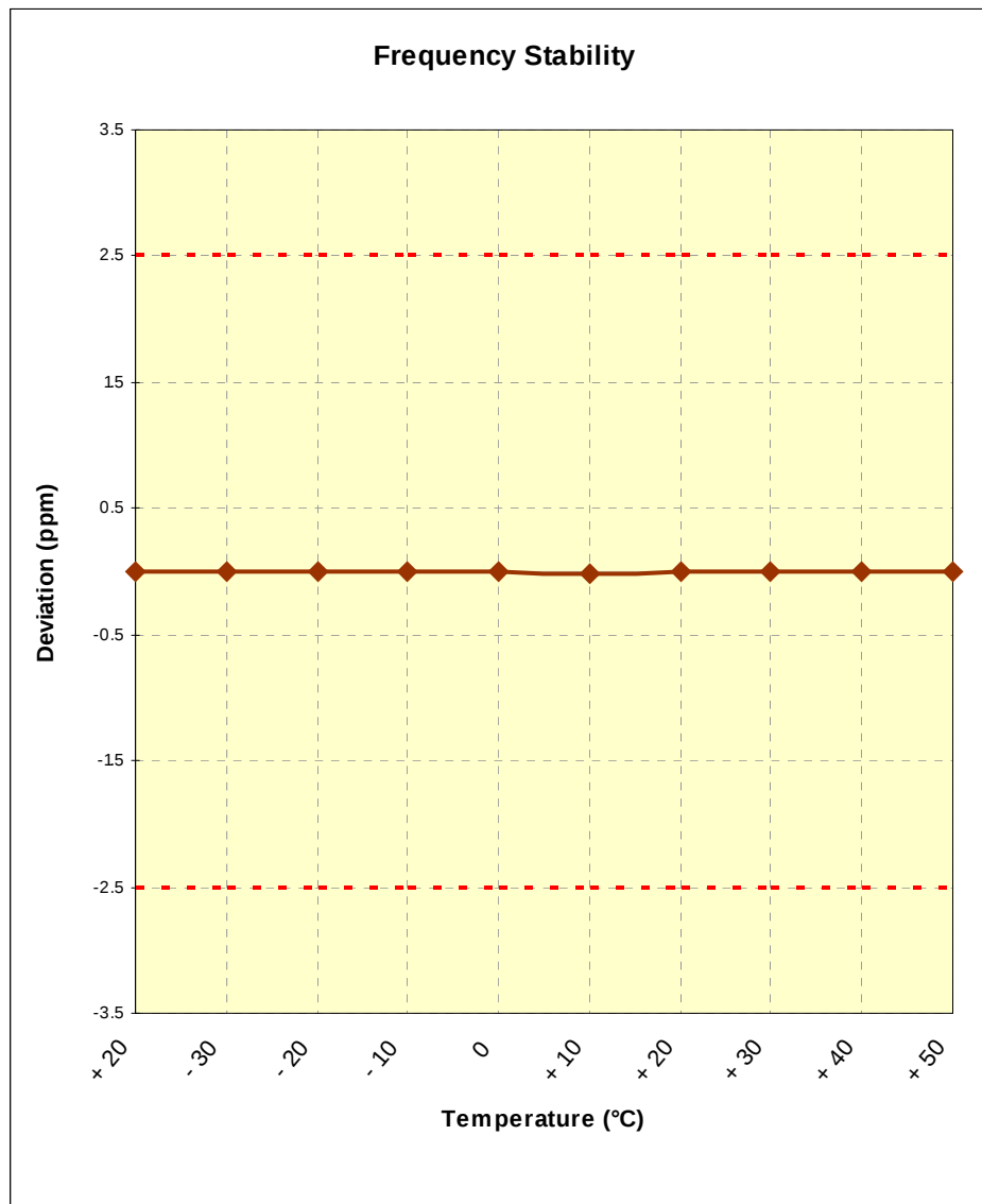
Figure 6-4. Frequency Stability Graph (PCS CDMA Mode – Ch. 600)
