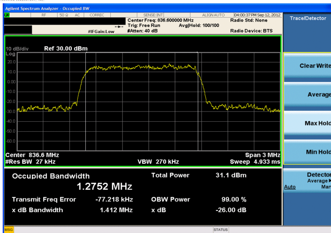
Plot 7-29. Occupied Bandwidth Plot (Cellular CDMA Mode – Ch. 384)
