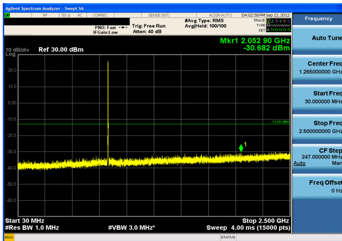
Plot 7-30. Conducted Spurious Plot (Cellular CDMA Mode – Ch. 777)
