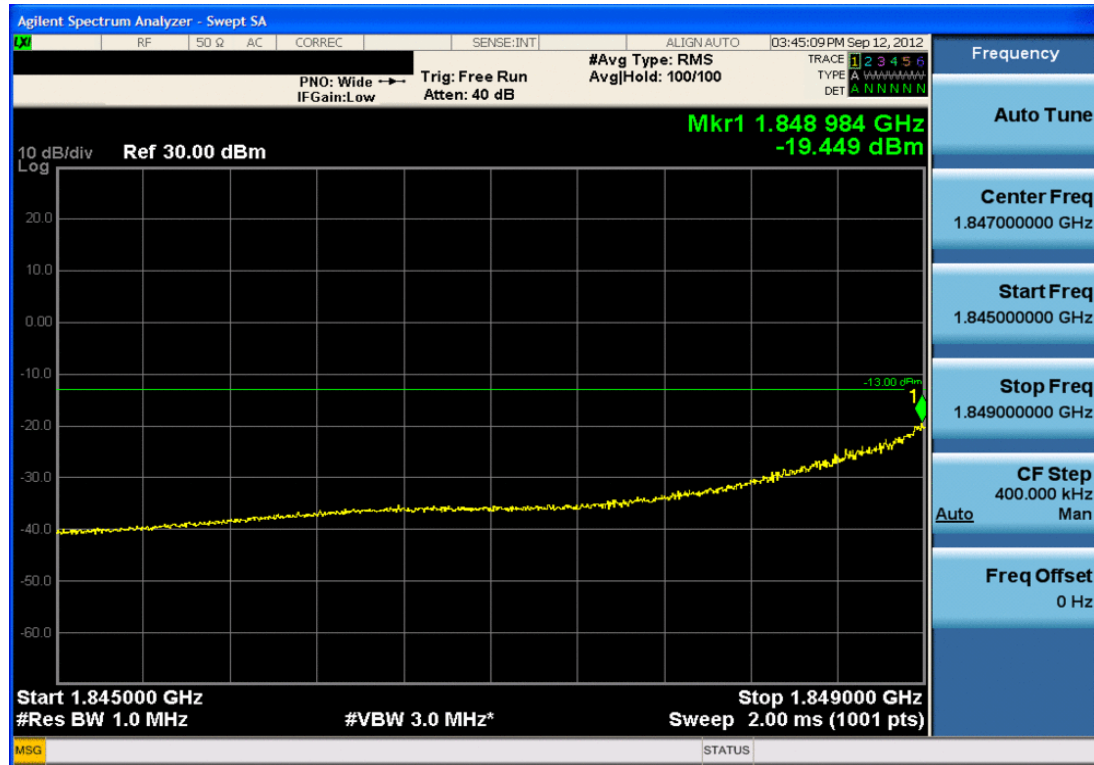
Plot 7-37. 4MHz Span Plot (PCS CDMA Mode – Ch. 25)
