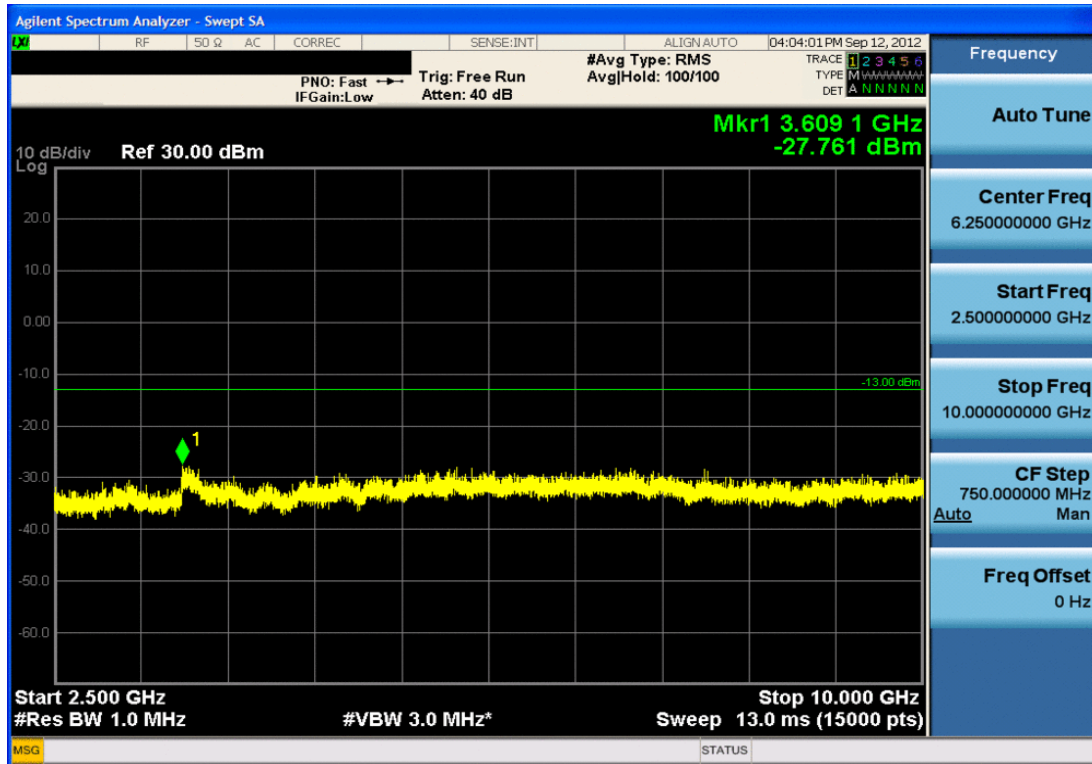
Plot 7-28. Conducted Spurious Plot (Cellular CDMA Mode – Ch. 384)
