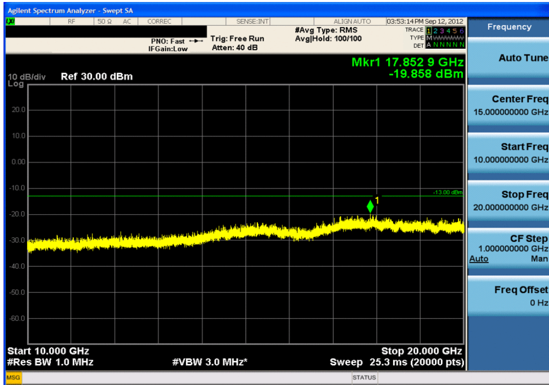
Plot 7-39. Conducted Spurious Plot (PCS CDMA Mode – Ch. 600)
