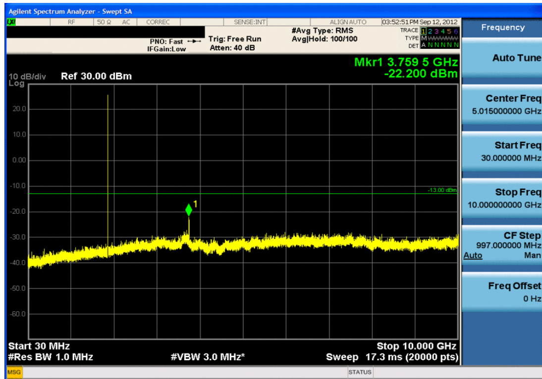
Plot 7-38. Conducted Spurious Plot (PCS CDMA Mode – Ch. 600)
