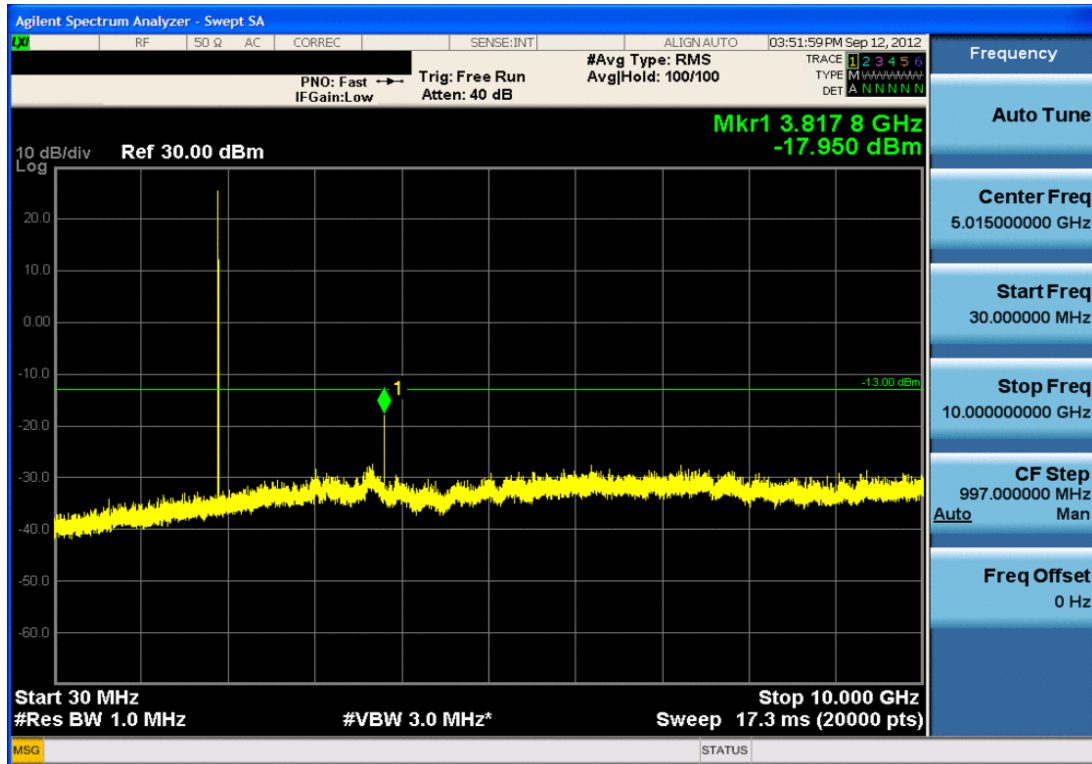
Plot 7-42. Conducted Spurious Plot (PCS CDMA Mode – Ch. 1175)
