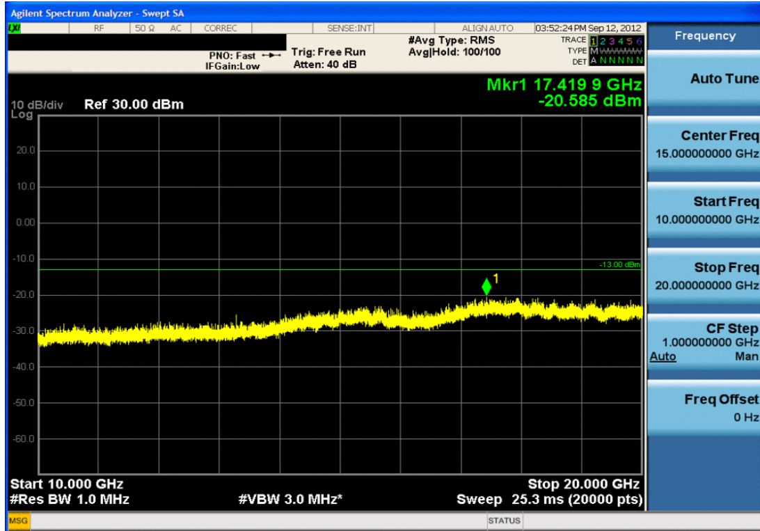
Plot 7-43. Conducted Spurious Plot (PCS CDMA Mode – Ch. 1175)
