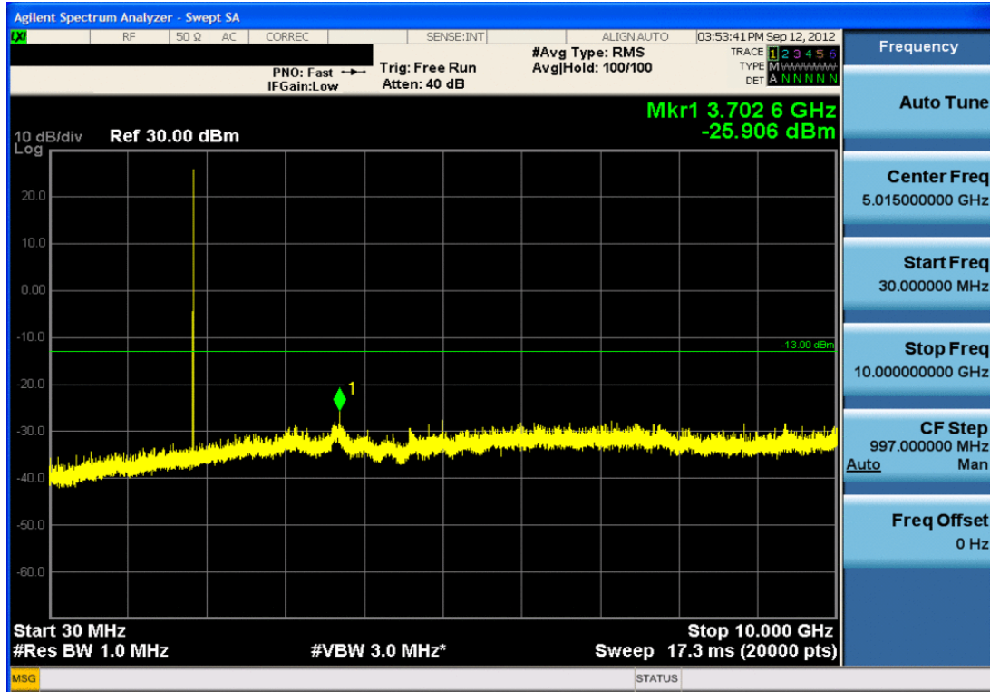
Plot 7-35. Conducted Spurious Plot (PCS CDMA Mode – Ch. 25)
