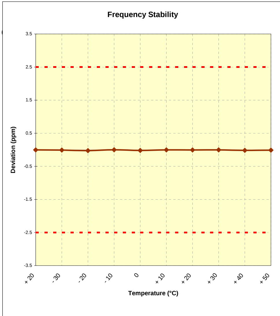
Figure 6-2. Frequency Stability Graph (Cellular CDMA Mode – Ch. 384)
