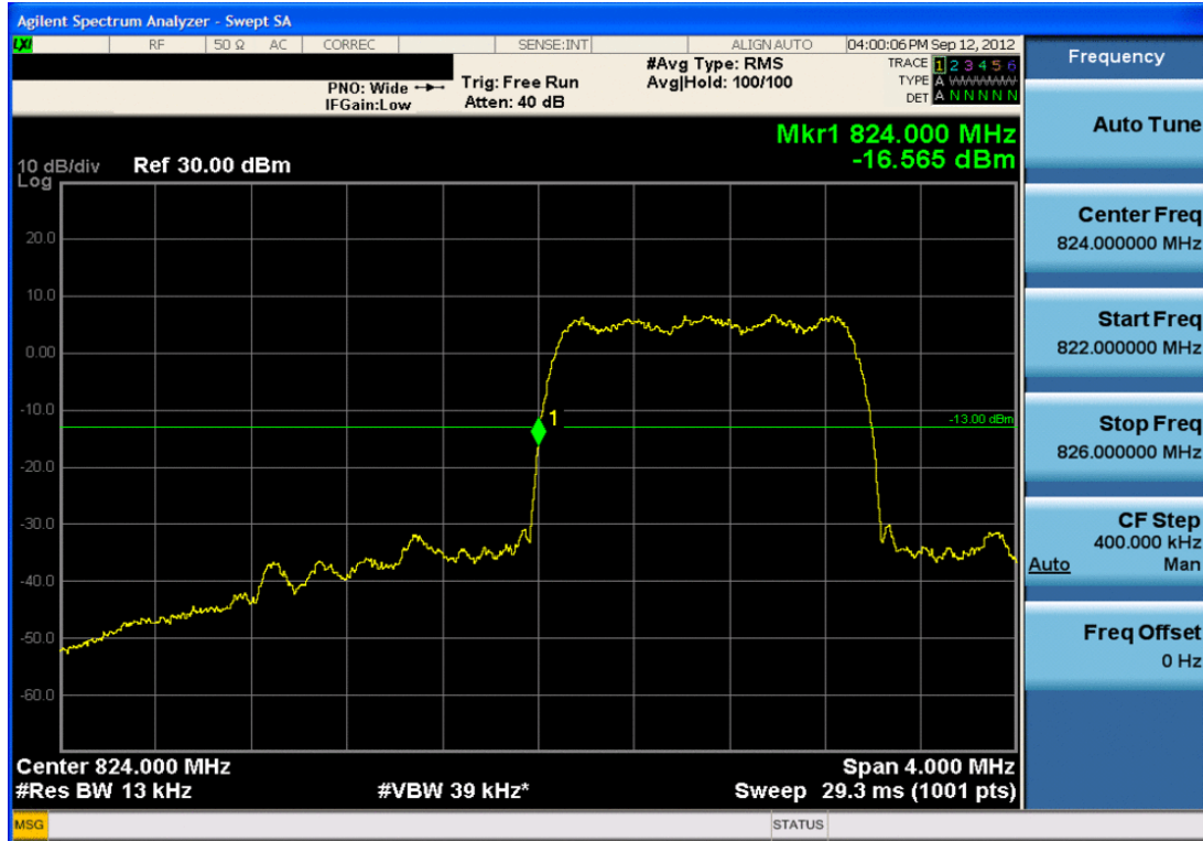
Plot 7-25. Band Edge Plot (Cellular CDMA Mode – Ch. 1013)
