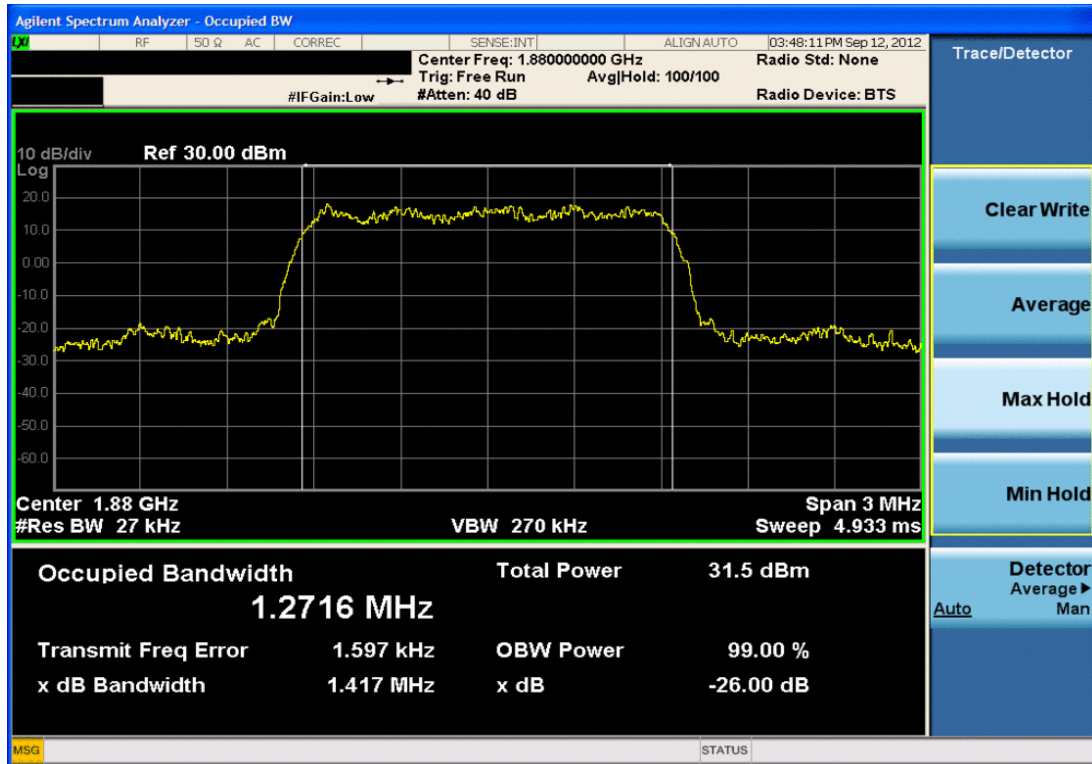
Plot 7-40. Occupied Bandwidth Plot (PCS CDMA Mode – Ch. 600)
