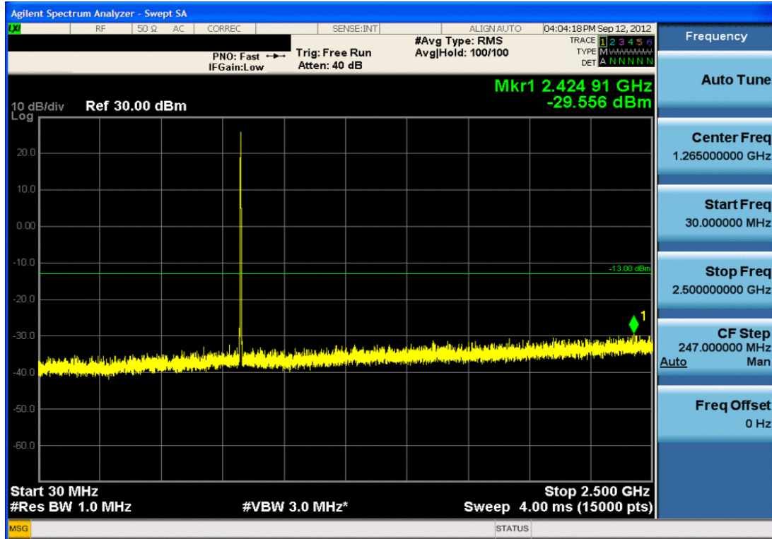
Plot 7-27. Conducted Spurious Plot (Cellular CDMA Mode – Ch. 384)
