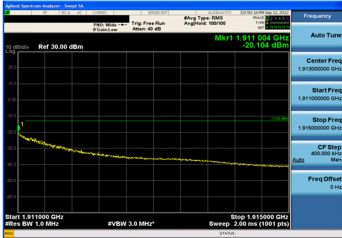
Plot 7-45. 4MHz Span Plot (PCS CDMA Mode – Ch. 1175)
