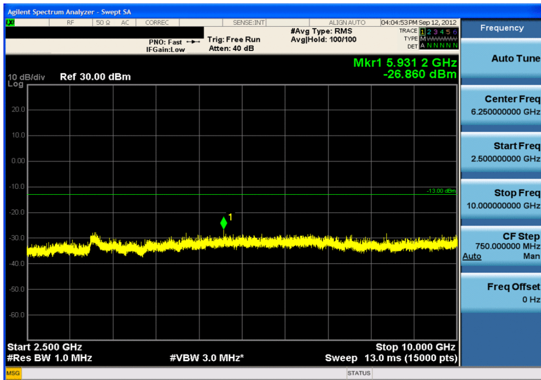
Plot 7-24. Conducted Spurious Plot (Cellular CDMA Mode – Ch. 1013)
