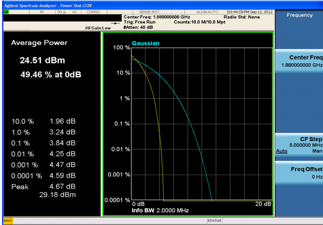
Plot 7-41. Peak-Average Ratio Plot (PCS CDMA Mode – Ch. 600)
